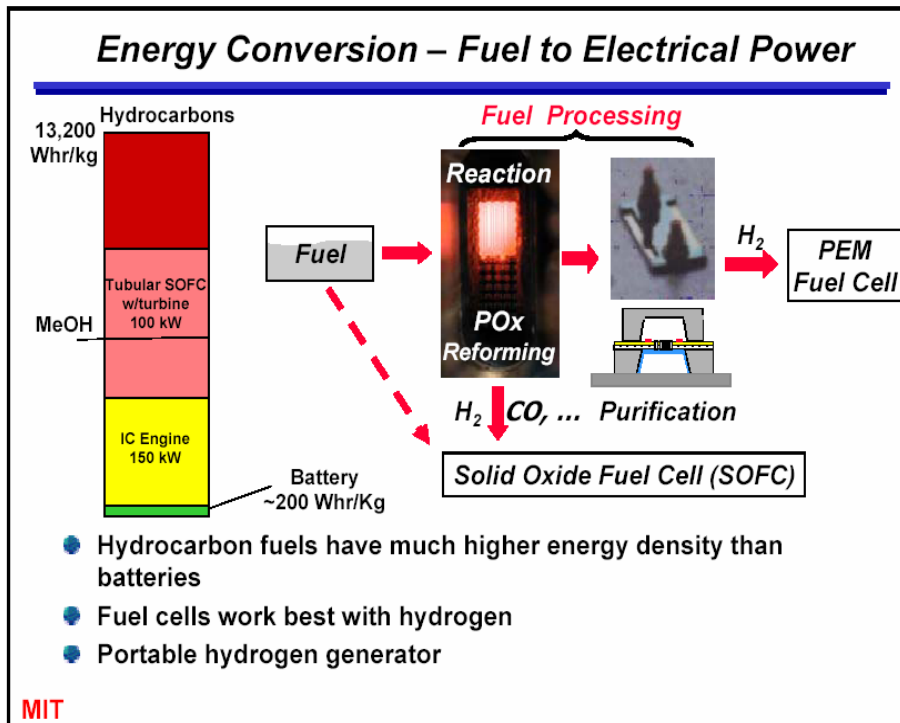
Figure 10 : Energy conversion comparison (Batteries, IC Engines, SOFC)
