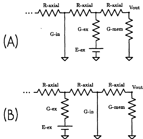
Figure 4.4: The effect of inhibition on tip output is dependent on the relative positions of the excitation and inhibition with respect to the output. To illustrate, we use an extreme case in which the inhibitory battery is equal to the resting potential, and the activated inhibitory conductance is infinite. In (A) the excitatory input is closer to the tip than the inhibitory input. Although the membrane potential at the site of inhibition is clamped to the resting potential (short-circuited), the axial resistance of the cable partially isolates the excitatory location, and the tip ( V_{out} ) is depolarized. In (B) the interposed inhibitory input clamps the cable between the excitatory input and the output to the resting potential, so that the output stays at rest. Adding membrane capacitance, a finite conductance to the activated inhibitory synapse, or making the inhibitory reversal potential not exactly equal to the resting potential does not change the basic interaction. However, a non-zero R_{axial} is crucial.
