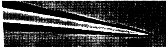
Figure B.1: Whole-cell patch electrode made with pull sequence in text (magnification 570\times ). R_{electrode} = 4M\Omega when filled with solution described in text. Tip diameter \approx 2\mu m .
