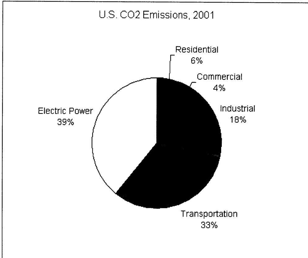
Figure 1.1: Anthropogenic CO 2 Emissions, 2001 [Energy Information Agency, 2002]
