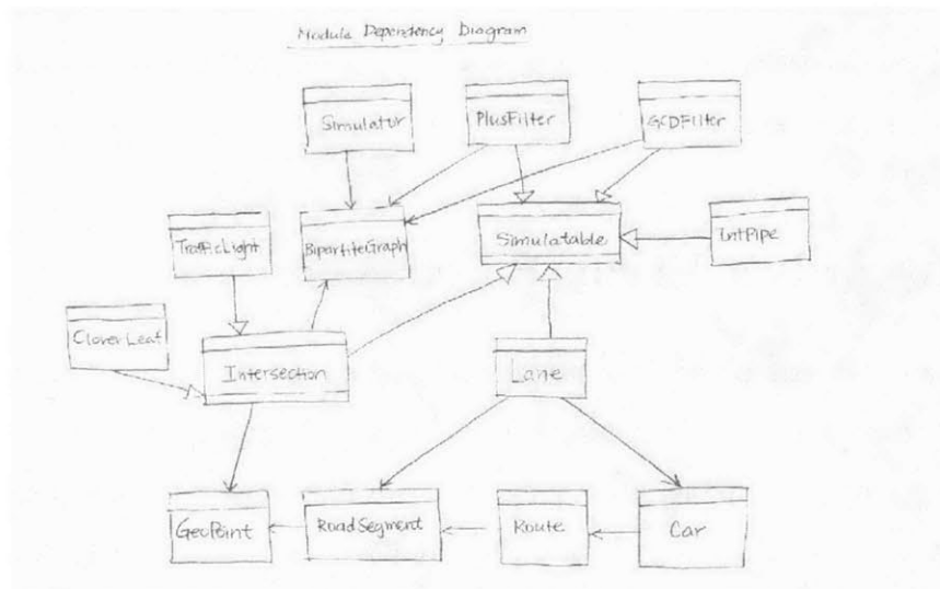
Figure 3-5: Module dependency diagram sketched by hand.
