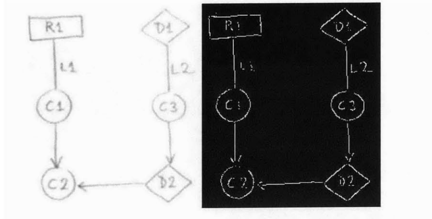
Figure 5-3: Result of Canny line detection. Line pixels are shown in white in image at right; at left, the input (Gaussian smoothed) image.
