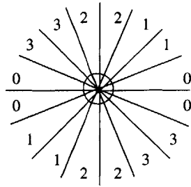
Figure 5-2: Converting gradient values to sectors.
