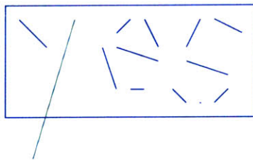
Figure 5-14: The “line segments cannot intersect text rectangles” heuristic filter.
