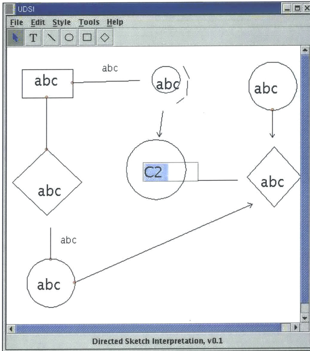
Figure 1-2: User editing a recognized sketch in UDSI
