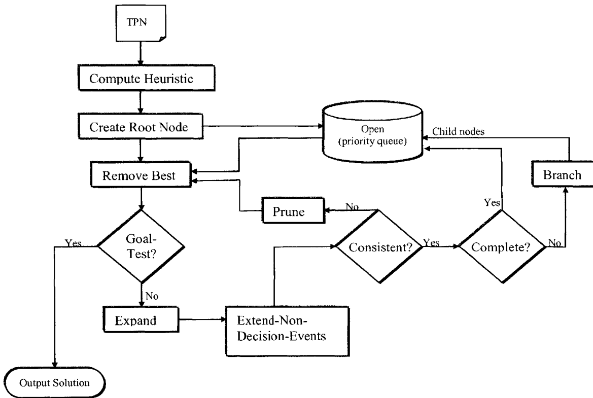
Figure 65: Flow chart for the optimal pre-planning process.
