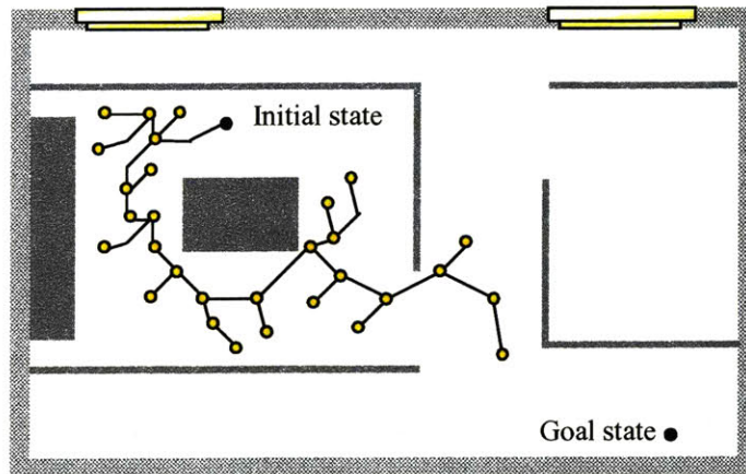
Figure 9: Example of an RRT exploring the state space.
