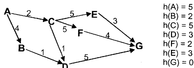
Figure 29: Example of a weighted graph (on the left) and the corresponding heuristic cost for each vertex to the goal G (on the right). The graph can be considered a state space search problem, where each vertex represents a state and each arc represents a specific action that takes the problem from one state to the next. The initial state is A and the goal state is G . Each vertex in the graph is analogous to a decision point in a TPN.
