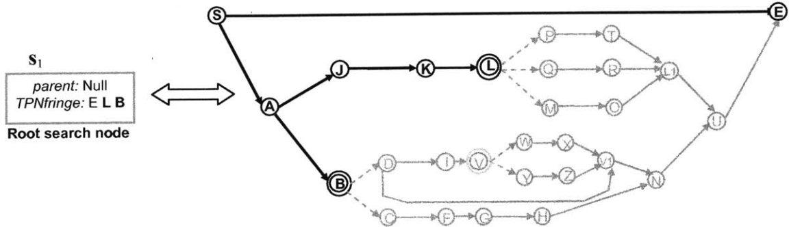
Figure 34: Root search node for the AtHome program (on the left) and its equivalent partial execution (on the right). The TPNfringe contains events E, L, and B. L and B in s_1 (shown in bold) are decision points that can be expanded further and E is the event signifying the end of that particular thread.
