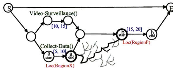
Figure 68: High-level example of a RMTPN growing an RRT from RegionX to RegionP.
