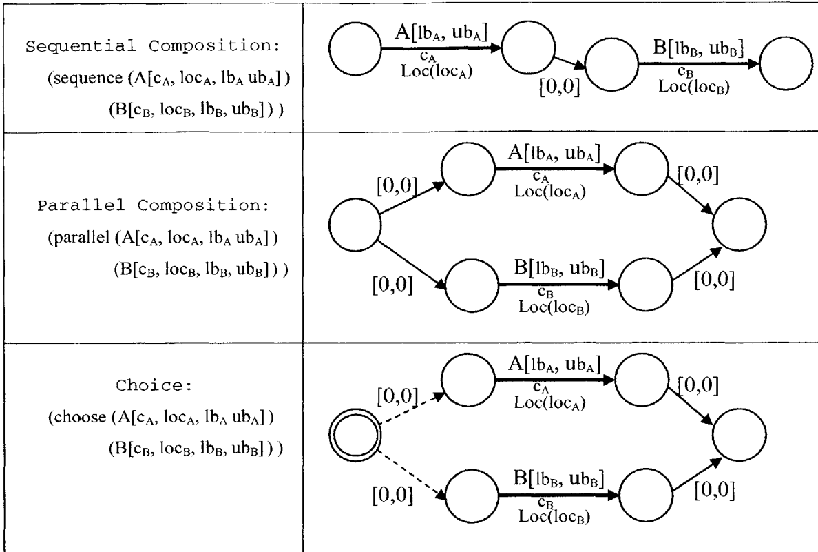
Figure 19: Mapping from ACLC combinators to TPN sub-networks.
