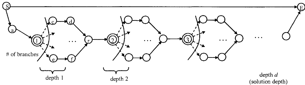
Figure 80: Example of type of problem instance analyzed.
