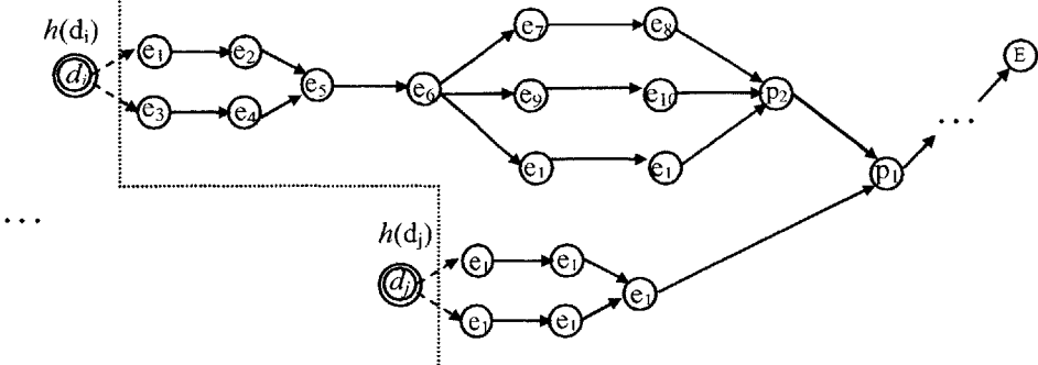
Figure 60: Example of the fringe of a search state with decision points d_i and d_j . Thread from the choices of either decision point will re-converge at p_1 .
