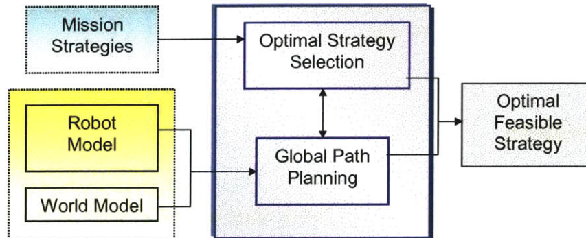
Figure 4: Overall unified activity and path planning system.
