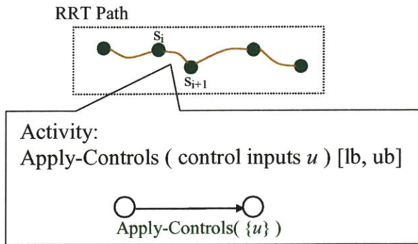
Figure 78: Example of mapping from a path sequence with nodes and edges to a sequence of activities. Each activity refers to the action of navigating to a location by applying the control inputs u for the duration of the activity.
