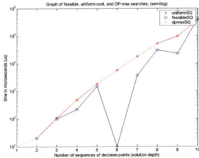
Figure 82: Semi-log plot of the graph in Figure 81.
