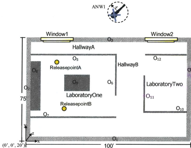
Figure 12: The world in which ANW1 will navigate in order to execute a strategy from the Enter-Building control program. The occluded regions are shown in gray. ANW1's dimensions are estimated by a sphere of radius r .
