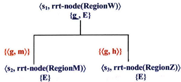
Figure 72: Search tree Path-Strategy in Figure 69.
