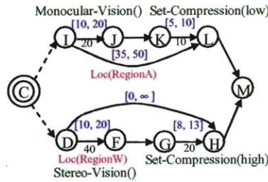
Figure 6: TPN representation of the program in Figure 5. There are two strategies for the AV to execute. The AV can either execute the Stereo-Vision activity and the Set-Compression activity, or the Monocular-Vision and the Set-Compression activity.
