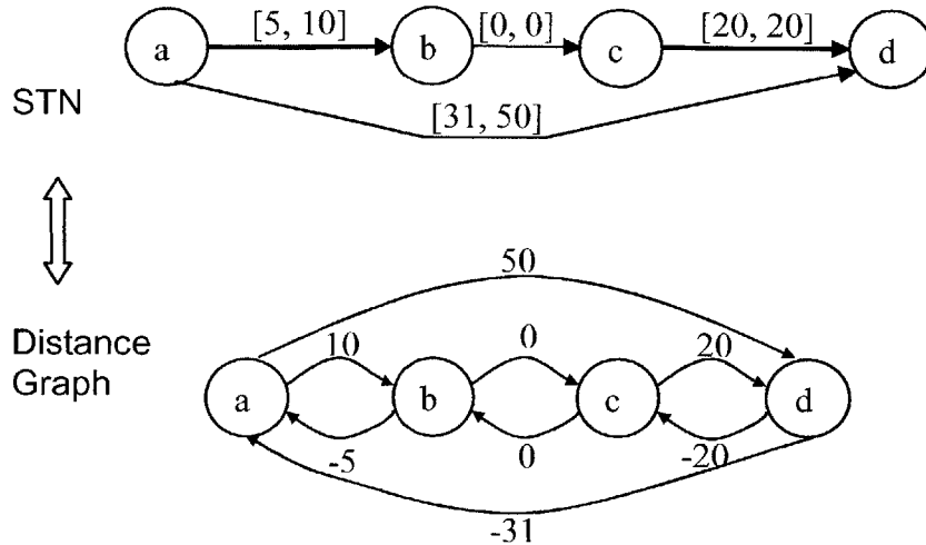
Figure 21: Example of STN and its corresponding distance graph.
