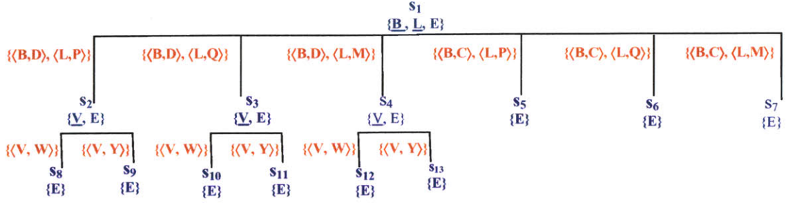
Figure 35: The complete search tree for the AtHome program. Each search node is labeled with a state name s_i and its corresponding TPN fringe events. The branches are labeled by choices. The choices for a node's state are the union of the branch choices along the path from the root to that node. The tree contains nine leaf nodes ( s_5 - s_{13} ), each referring to the nine complete (not necessarily consistent) plans in the AtHome search space. The underlined TPN events are decision points that are expanded, in order to generate a node's children. Each set of TPN fringe events that contain E marks the end of another thread of execution from S to E . Node s_8 denotes the optimal execution.
