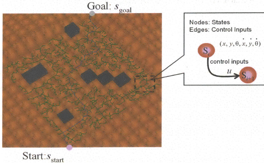
Figure 10: Example of an RRT growing from the start state to the goal state.
