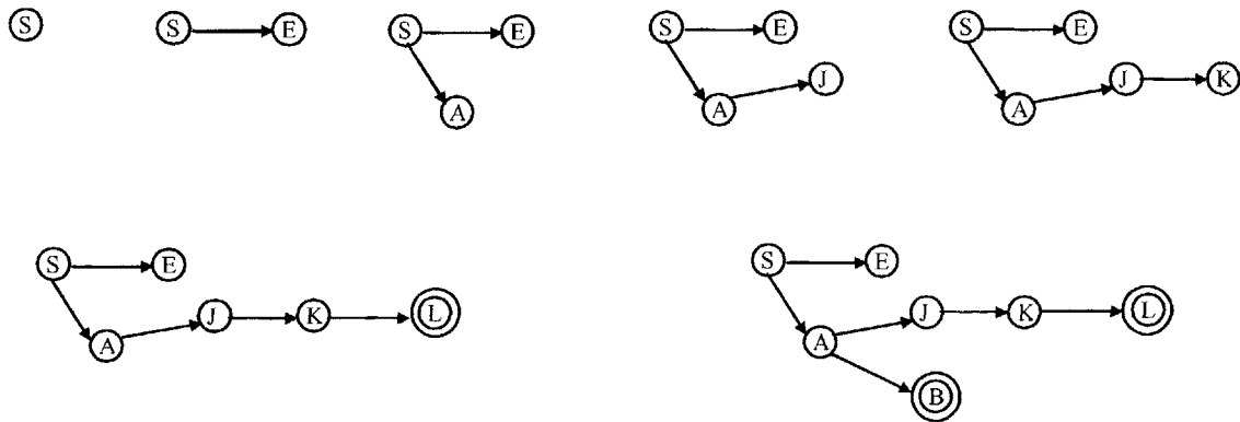
Figure 44: Example of Phase One, Extend-Non-Decision-Events, applied to the initial root tree node.
