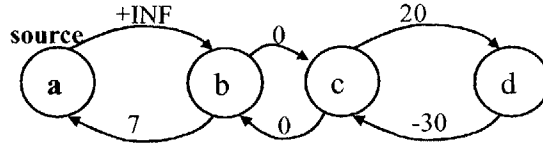
Figure 22: Distance graph from a sequence of STN constraints.
