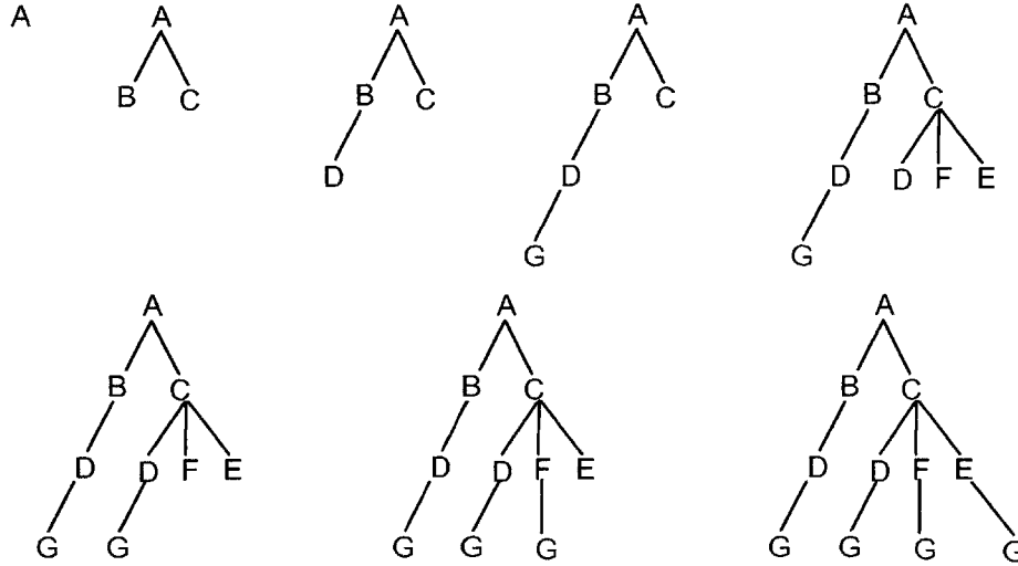
Figure 46: Progression of depth-first search applied to the graph in Figure 29. The start vertex is A and the goal vertex is G. The final tree shows the four possible paths from A to G.
