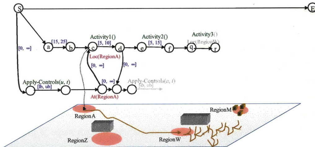
Figure 76: Attempting to satisfy the location constraint Loc(RegionM) by growing an RRT from the current region, RegionW .
