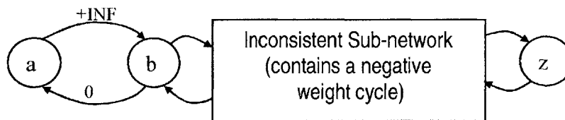
Figure 23: A sequence that starts with a +INF arc and contains a sub-network that is temporally inconsistent. The +INF arc gets propagated forward when applying the single-source shortest path algorithm and the shortest path between nodes in the graph all become +INF, and thus, a temporally inconsistent plan is mistakenly declared temporally consistent.
