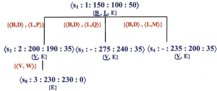
Figure 64: Search process for TPNA* applied to the AtHome control program. Each search tree node is denoted by \langle s : \text{iteration\#} : f(s) : g(s) : h(s) \rangle . The heuristic cost of s_1 is \max(h(B), h(L)) = 50 .
