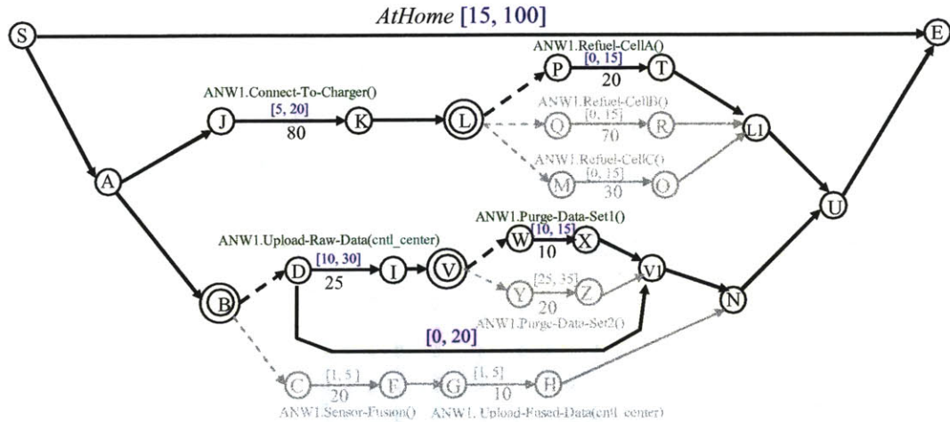
Figure 31: The bold portion of the TPN denotes the optimal plan for the AtHome program. We use a default arc cost of 5 units (not including arc S→E).
