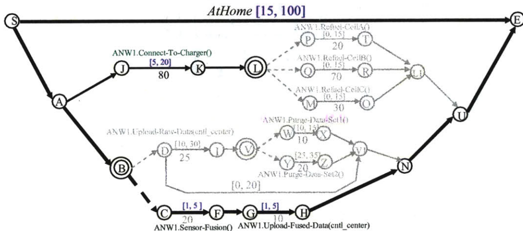
Figure 48: A cycle is formed at when search tree node s_5 is expanded. The cycle, between the partial execution of s_1 and s_5 , is shown in thick bold. Temporal consistency is checked on the current partial execution, and it fails. Thus, expansion of s_5 is terminated and the node is pruned from the search tree.
