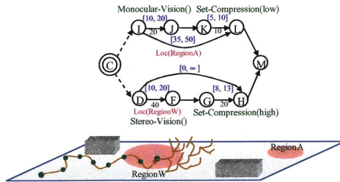
Figure 7: Unified activity and path planning space. The RMPTPN model is used to reason on the combined search spaces.
