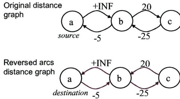
Figure 24: By framing the problem as a single-destination shortest path problem all negative weight cycles in a distance graph can be found.
