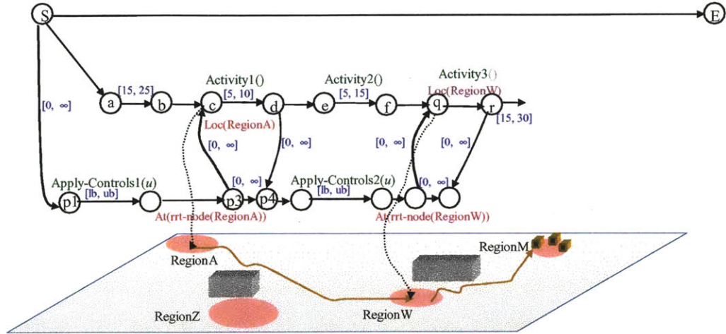
Figure 77: After the location constraint Loc(RegionW) is satisfied.
