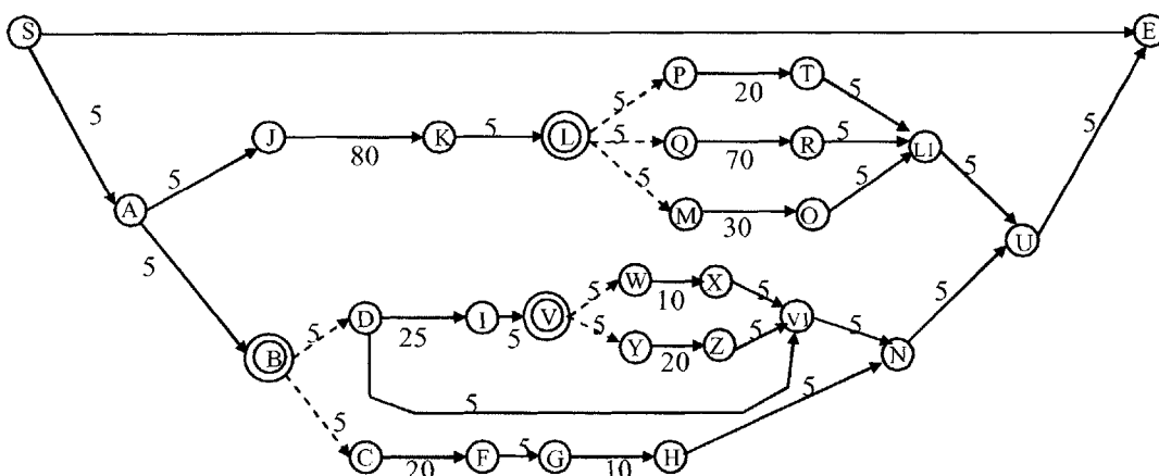
Figure 59: TPN for the AtHome strategy with all its arc costs.
