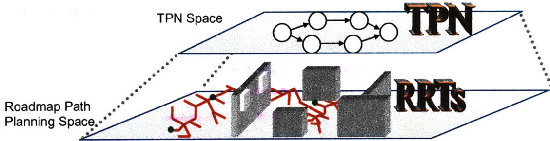
Figure 70: Unified search space - Illustrates the two spaces in which the unified planner searches. The circles points in the TPN represent regions where the AV will navigate to.
