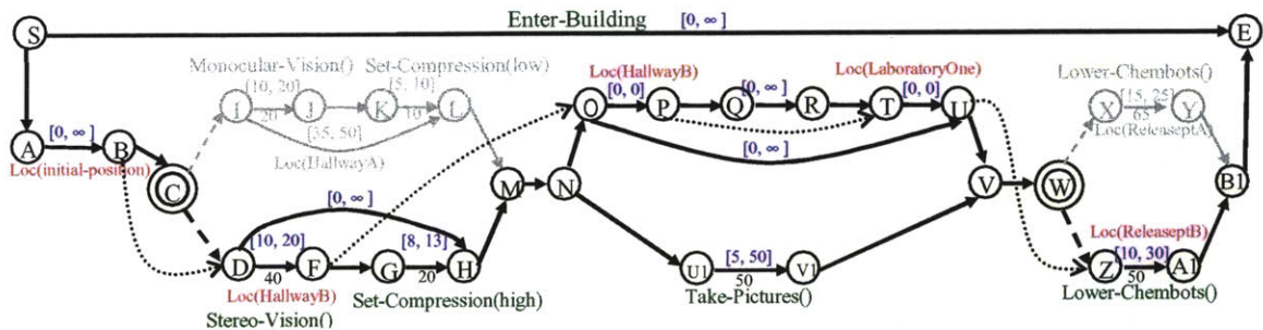
Figure 20: Example of an optimal, complete and consistent plan for the Enter-Building activity. The dotted arrows from location to location enforce the order in which each location is visited by ANW.
