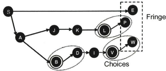
Figure 32: Example of a partial execution from the AtHome program TPN. The terminal events are E, P, and W and make-up the fringe of this partial execution. The choices are B \rightarrow D , V \rightarrow W , and L \rightarrow P .
