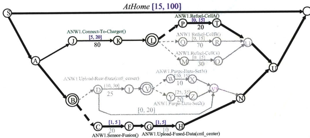
Figure 49: Extend-Non-Decision-Events applied to s_5 and the event U is reached by the threads from B and L.
