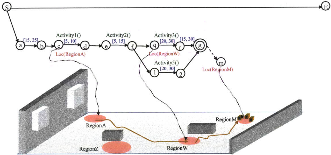
Figure 71: Example of a RMTPN partial execution with a path from RegionA to RegionW to RegionM.
