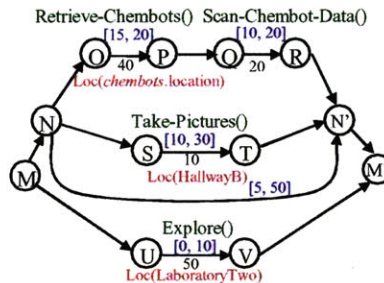
Figure 83: Snapshot of the parallel sub-network in the Exit-Building TPN (Figure 67). The location constraints within a parallel sub-network must have an order that specifies the order in which regions are visited.
