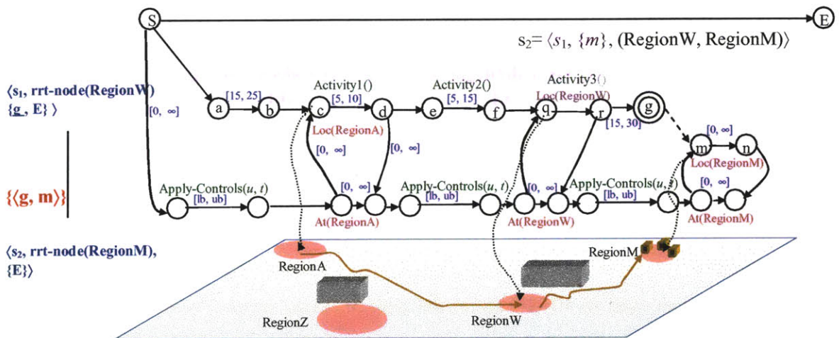
Figure 74: Example of partial execution for the search tree node s_2 (Figure 72) after satisfying location constraint \text{Loc}(\text{RegionM}) during expansion.
