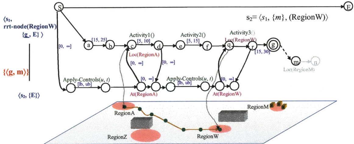
Figure 73: Example of an RMTPN partial execution for the search tree node s_2 (Figure 72) before satisfying location constraint \text{Loc}(\text{RegionM}) during expansion. The corresponding search tree is shown on the left, and the partial execution is shown on the top right.
