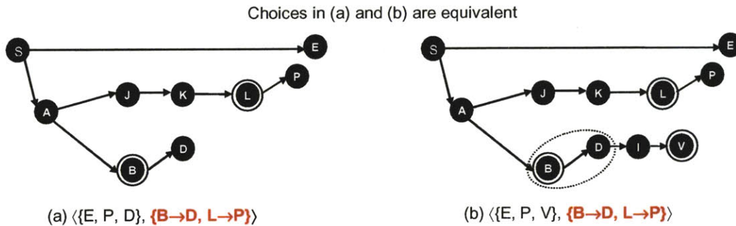
Figure 33: Two partial executions, (a) and (b), with equivalent choices \{B \rightarrow D, L \rightarrow P\} . Thus (a) and (b) map to the same state.
