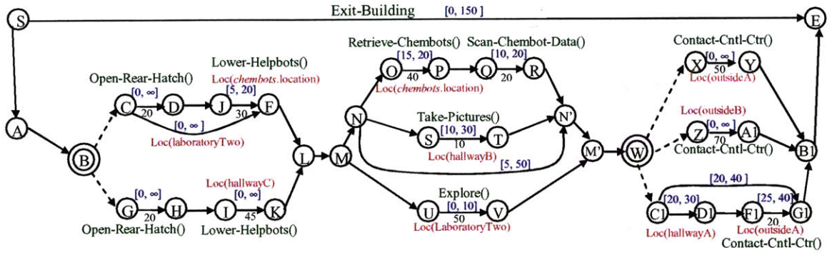
Figure 67: TPN representation of the Exit-Building strategy.
