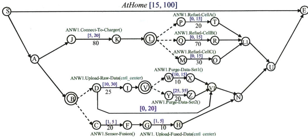
Figure 27: Corresponding TPN representation of the AtHome program in Figure 26. Decision points are marked with double circles. Arcs without an explicit time bound have a [0, 0] time bound. Arcs without an explicit cost are assumed to have a default cost of 5 units. There are no location constraints in this example, thus, they are not included on the arcs.
