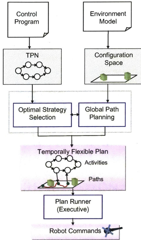
Figure 16: Overview of the unified activity and path planning system.
