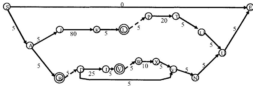
Figure 51: The partial execution denoted by search node s_8 . The network contains a default arc cost of 5 units for all arcs without activity costs. The path cost for g(s_8) = 210 units.
