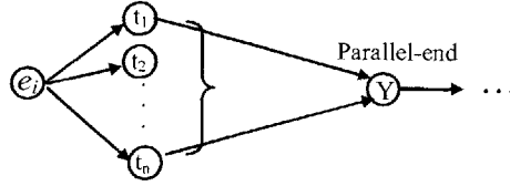
Figure 55: Example of a generalized parallel sub-network. The heuristic cost of a parallel start event e_i is the sum of each thread within the parallel sub-network, plus the heuristic cost of the parallel end.
