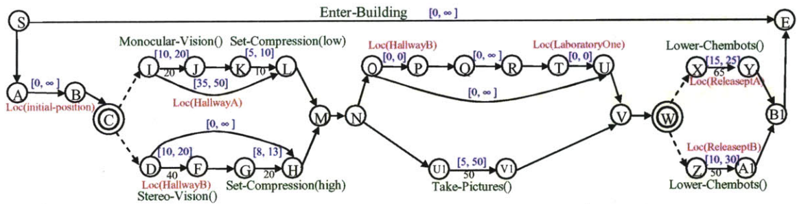
Figure 17: Example Temporal Plan Network for the Enter Building control program. In the figure, the name of the autonomous vehicle ANW1 involved in the mission is omitted and the activity names are abbreviated for clarity. In Figure 17, arcs without an explicitly labeled temporal constraint are assumed to have [0, 0] bounds and arcs without explicit location constraints are assumed to not be constrained by location.
