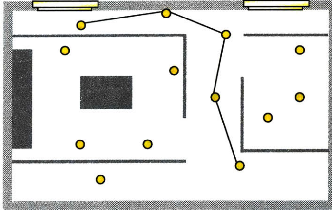
Figure 8: Example of randomly generated roadmap nodes used to find collision free paths in a space.
