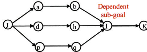
Figure 53: The additive heuristic applied to J results in an admissible heuristic for J. The heuristics for a, d, and p, each include the cost from their dependent sub-goal I \rightarrow K . The max heuristic does result in an admissible heuristic for J, however, it is not informative.
