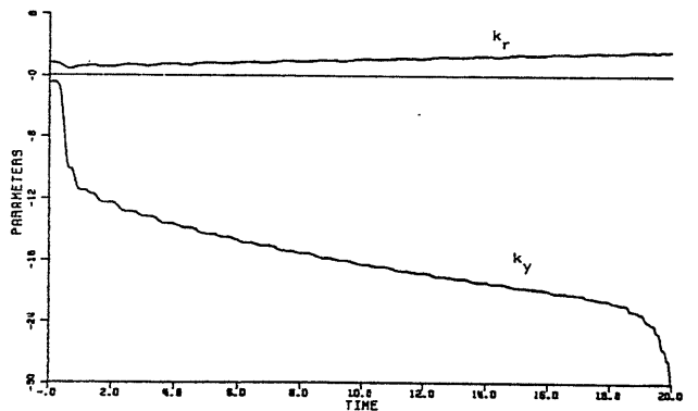
Figure 8: Simulation of CAL with unmodeled dynamics, r(t)=0.3 , and d(t)=8.0 \times 10^{-6} \sin 5.0t . (System eventually becomes unstable).
