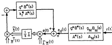
Figure 2: Error System for CAL.
