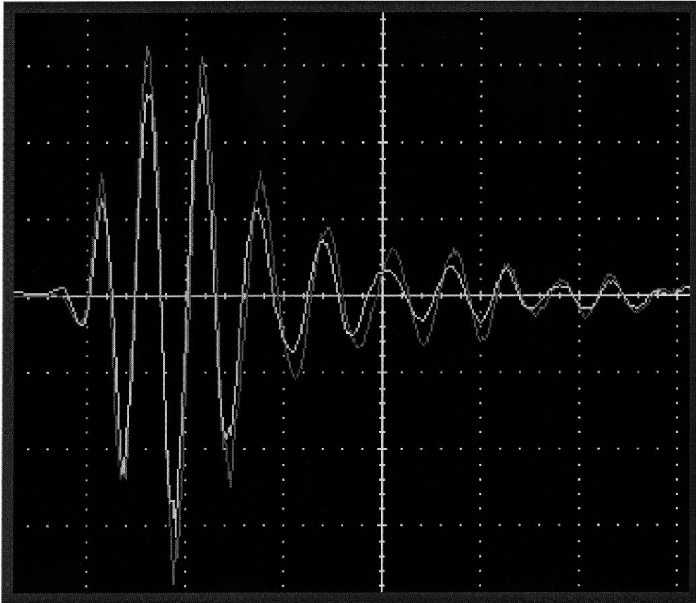
Figure 46. Received pulse (light) over Transmit pulse (dark) for Loaded SEA.
