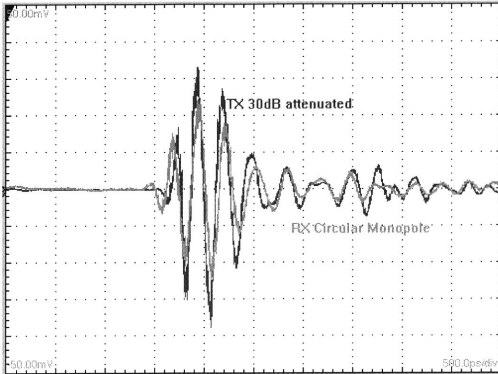
Figure 39. Time Domain pulse characteristics of CDM. Transmit pulse (dark) vs. Receive pulse (light).
