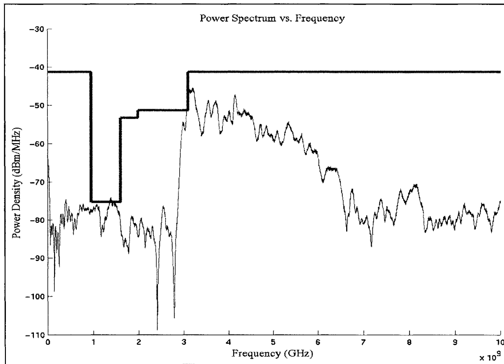
Figure 17. Power spectrum of the transmitted pulse plotted against the FCC spectral mask.
