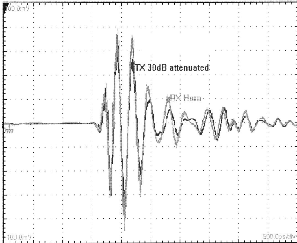
Figure 22. Transmitted Pulse (Dark) Superimposed on Received Pulse (Light). Measured directly at antenna terminals.
