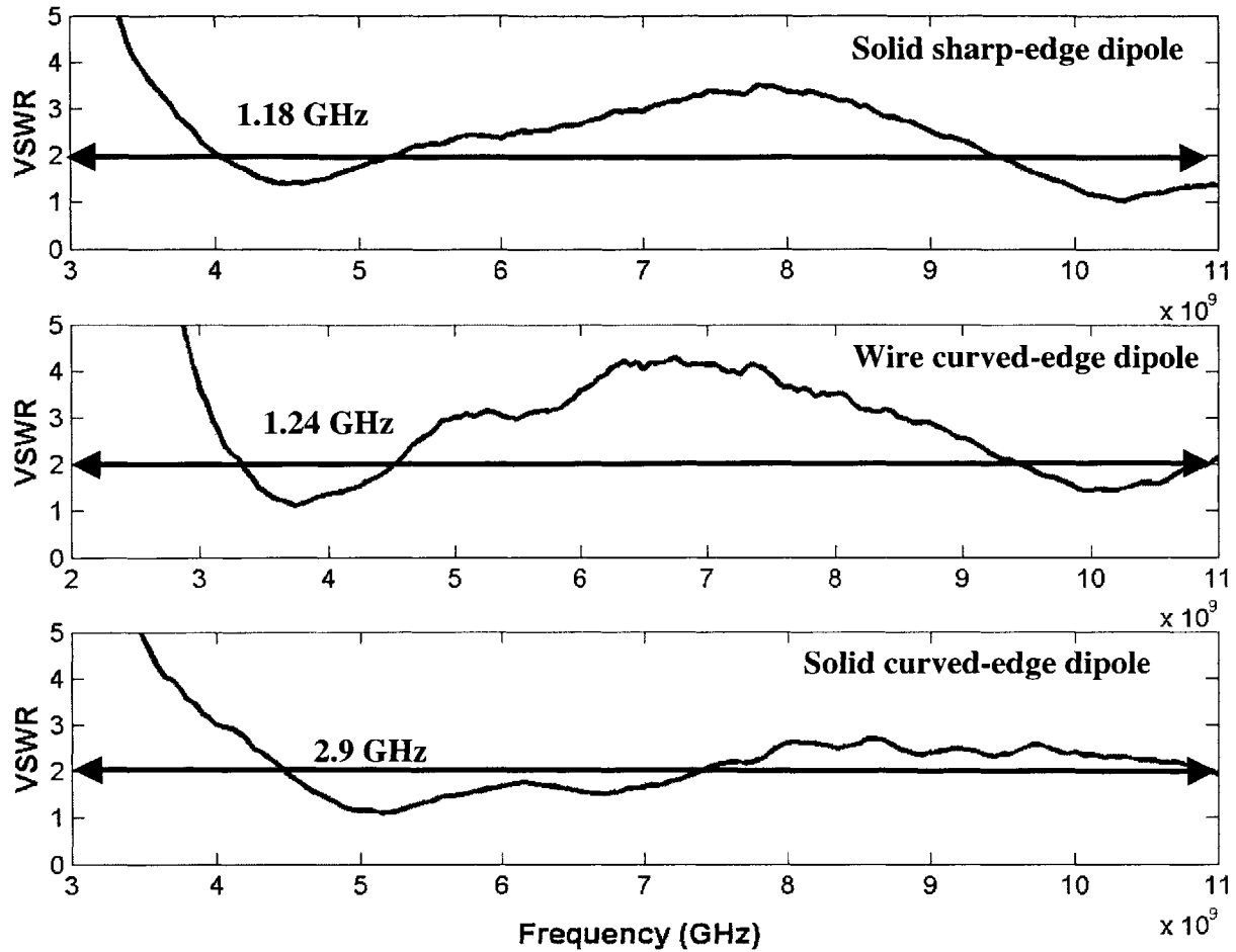
Figure 36. VSWR plots for Diamond Dipole Configurations.
