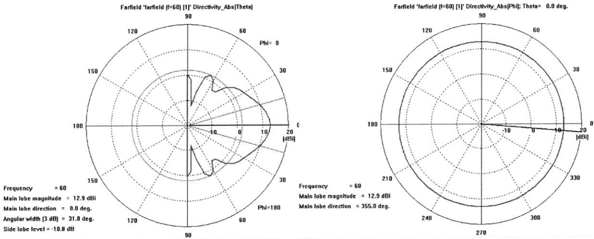
Figure 7. CST MW Studio simulated radiation pattern. Varying \theta , \phi=0^\circ (left). Varying \phi , \theta = 0^\circ (right).
