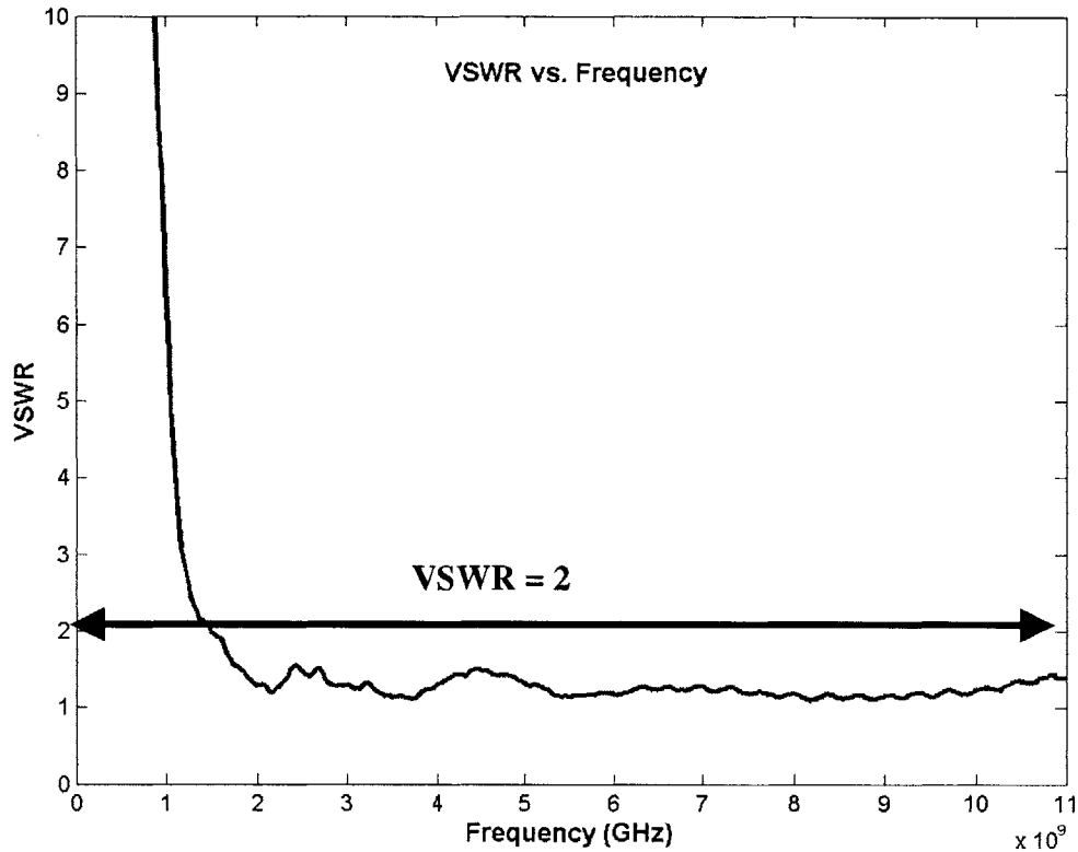
Figure 38. VSWR plot for the CDM.
