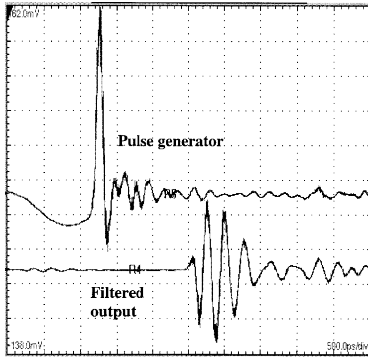
Figure 15. Output pulse from impulse generator (top) and pulse output from high pass filter.
