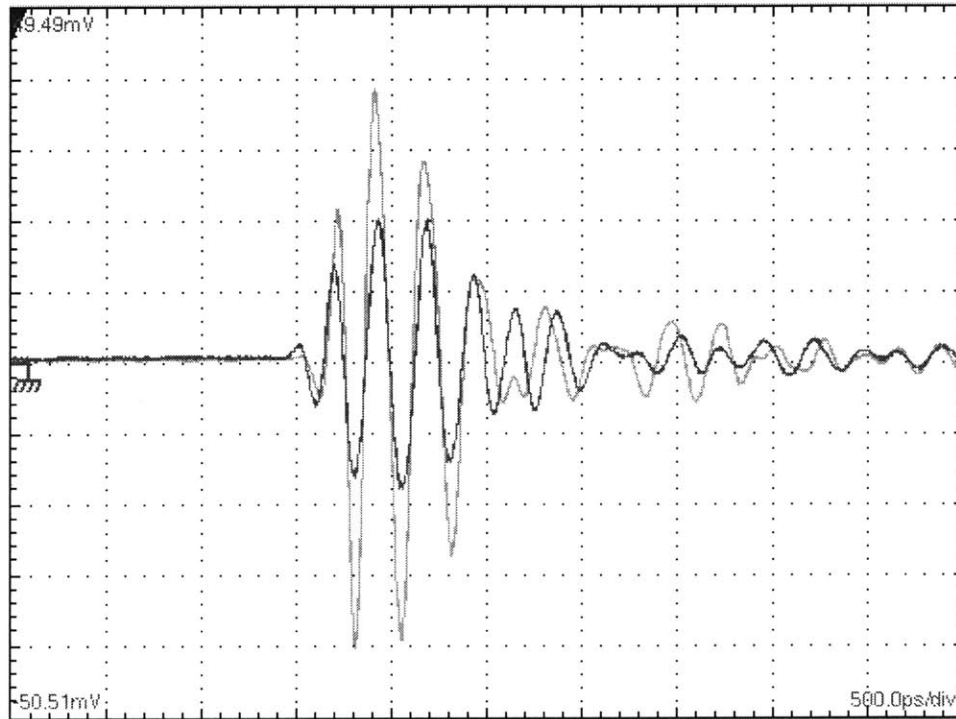
Figure 29. Time Domain Pulse. Received Pulse from spiral antenna superimposed on transmitted pulse. Transmit pulse is light, and receive pulse is dark.
