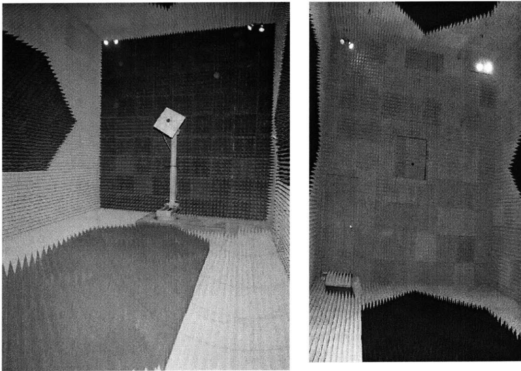
Figure 49. Photos of mm wavelength anechoic chambers. Courtesy David Bruno, Lincoln Laboratory.
