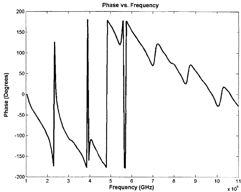
Figure 32. Measured Phase vs. Frequency for Narrowband Wire Antenna.
