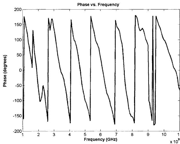
Figure 20. Phase vs. Frequency for Horn Antenna.
