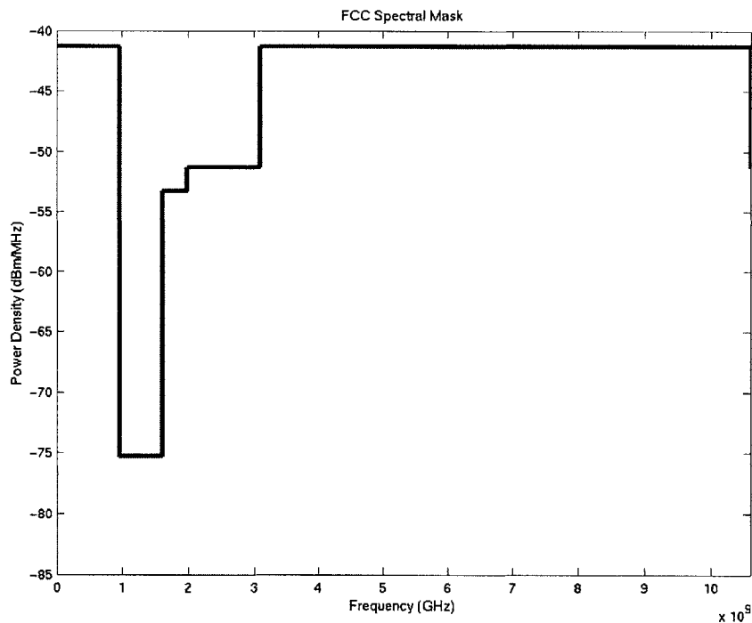
Figure 2. FCC Spectral Mask for indoor unlicensed UWB transmission. [1].
