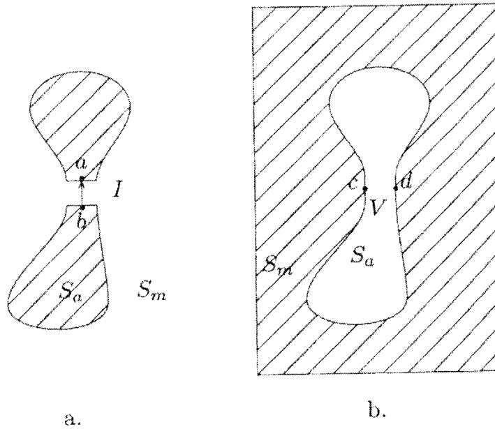
Figure 12. Complementary antennas illustrating Babinet's Equivalence Principle [14]
