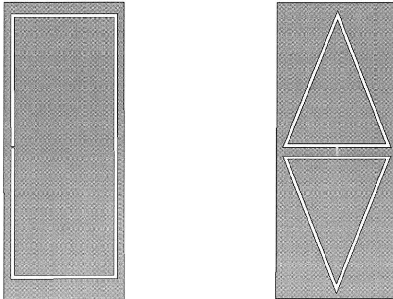
Figure 11. Rectangular loop antenna model (left) [9,10,13] and diamond dipole antenna model (right) [12].
