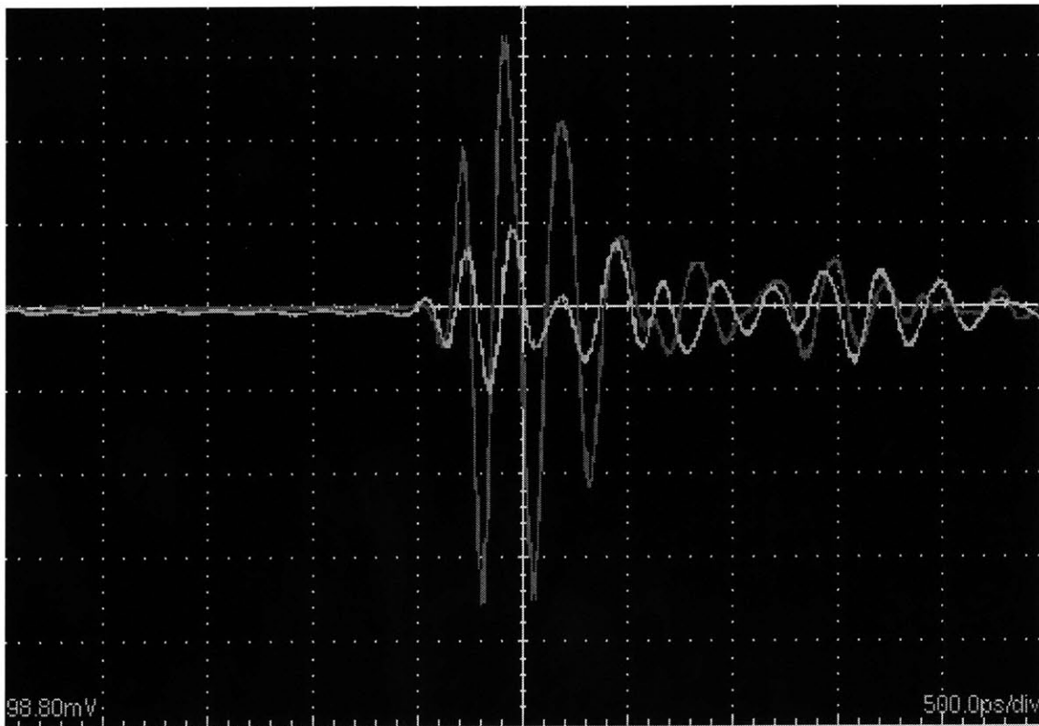
Figure 34. Time Domain plot of wire antenna received pulse superimposed over transmitted pulse. Transmit pulse is dark, and receive pulse is light.
