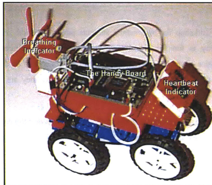
Figure 9 The LEGO carriage robot
