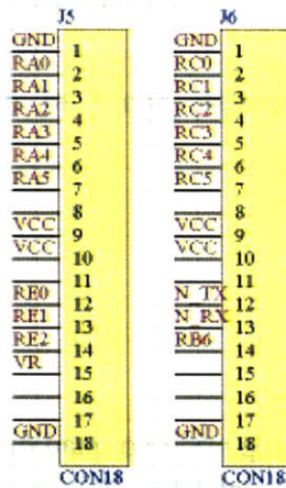
Figure 23 The Hoarder board add-on-board connectors
