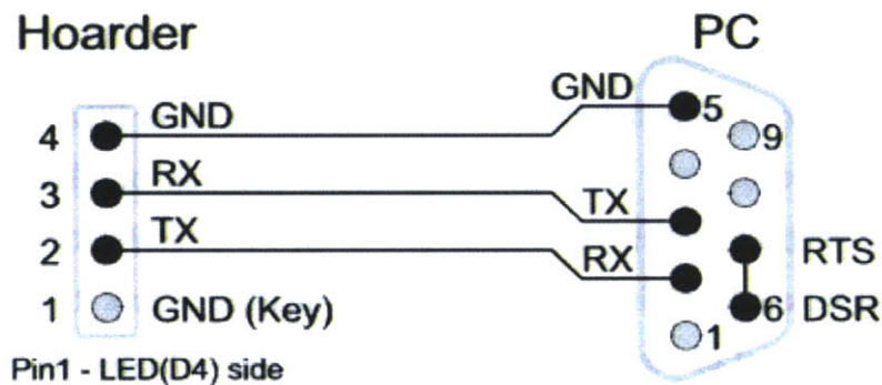
Figure 18 The Hoarder board serial-cable pinout
