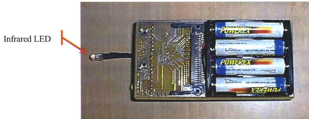
Figure 35 The Hoarder board in the Heartball
