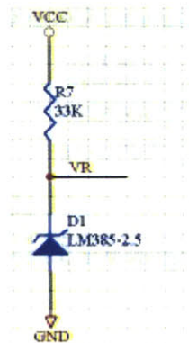
Figure 22 The Hoarder board voltage reference
