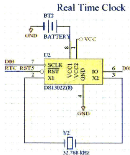
Figure 17 The Hoarder board real-time clock chip
