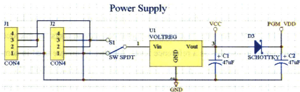
Figure 21 The Hoarder board power-supply circuit
