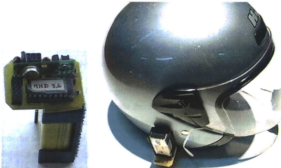
Figure 5 The HHD device and the biosensor helmet. The HHD device is mounted on the side of the helmet while four sensors are mounted inside.
