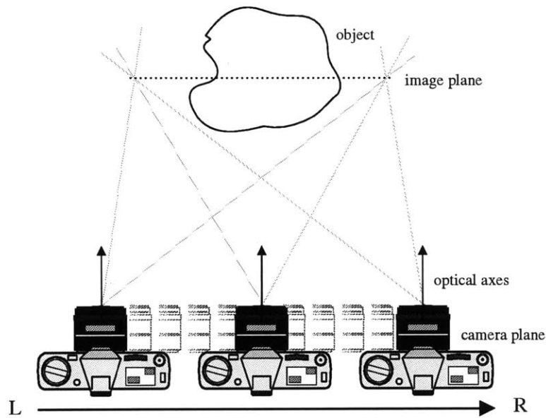
Figure 5-2: A two-dimensional view of the PRS camera geometry.
