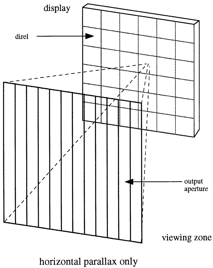
Figure 3-5: An HPO parallax display projects a one-dimensional grid of long, thin view apertures.
