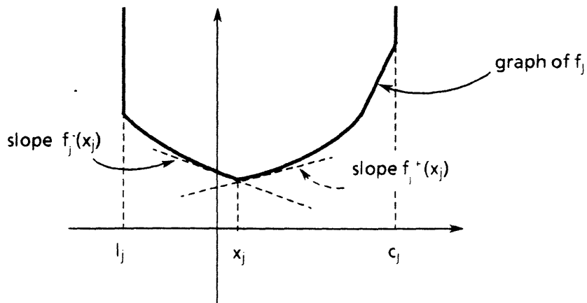
Figure 1 The left and right derivatives of f_j .
