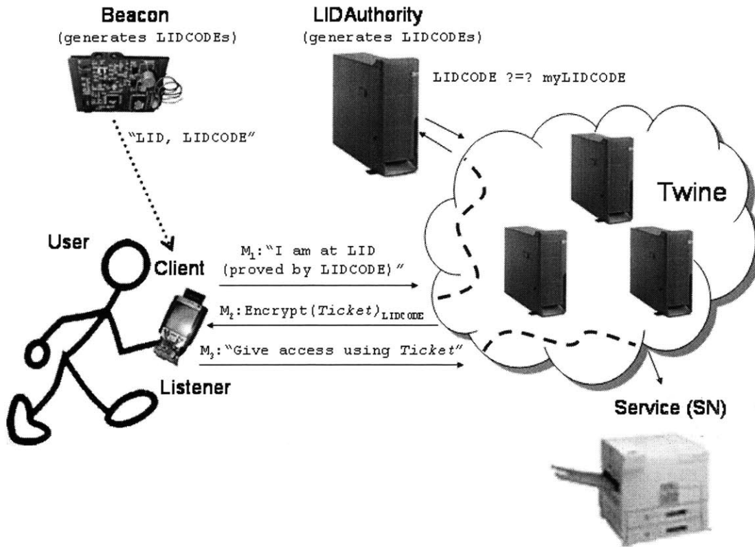
Figure 1-1: How a user accesses a service using PAC.
