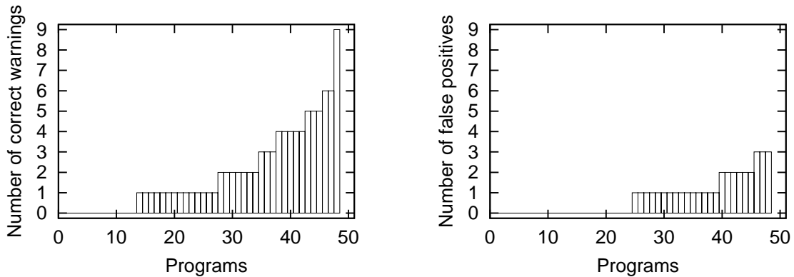
Figure 8-2: Reported incompatibilities between C library versions 2.1.3 and 2.3.2 for 48 subject programs. The left graph shows incompatibilities that we have verified by hand. The right graph shows warnings that are probably false positives. The numbering of programs is different in the two graphs.
