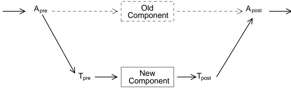
Figure 2-8: The behavioral subtyping rule. A new component whose specification guarantees T_{\text{pre}} \Rightarrow T_{\text{post}} may replace an old component whose specification guaranteed A_{\text{pre}} \Rightarrow A_{\text{post}} (dashed), if A_{\text{pre}} \Rightarrow T_{\text{pre}} and T_{\text{post}} \Rightarrow A_{\text{post}} (solid). Arrows represent both program control flow and logical implication between specifications. This rule is sufficient but too strong for validating component upgrades. Section 2.3.1 presents our alternate rule.
