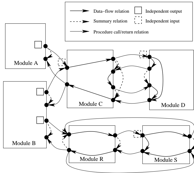
Figure 3-2: Examples of modules and relations
