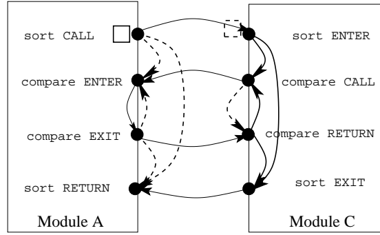
Figure 4-5: A system with a module C that calls back to the using module A .
