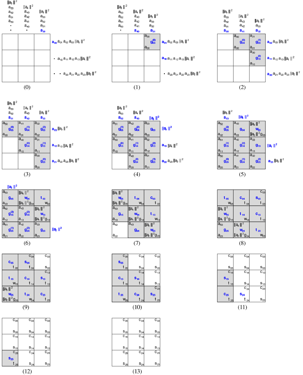
Figure 6: Systolic rotation computation for two R \times N row blocks with R = 3 and N = 4 . Values g_{ij} = a_i^T a_j , w_{ij} = \|a_i\|^2 \|a_j\|^2 / g_{ij} , and t_{ij} = \text{sign}(w_{ij}) / (|w_{ij}| + \sqrt{1 + w_{ij}^2}) are the intermediate values of Procedure 2 used to compute the rotation c_{ij} and s_{ij} of rows i and j .
