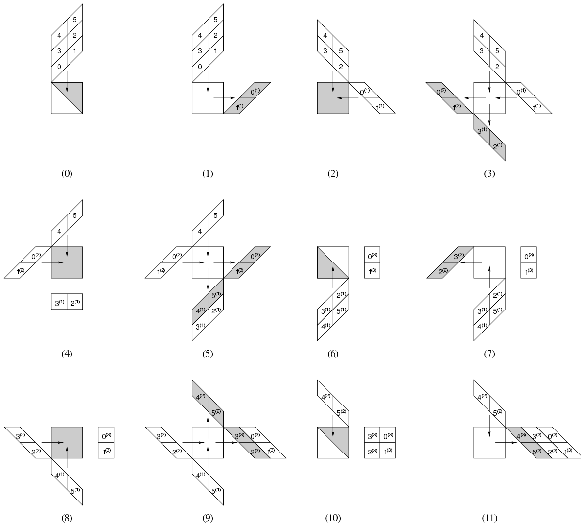
Figure 10: One block sweep of a stream SVD of M \times N matrix A on an R \times R array of compute processors with R = 2 and M = 6 . Matrix A is partitioned into three row blocks \{0, 1\} , \{2, 3\} , and \{4, 5\} . Even numbered phases denote rotation computations, and odd numbered phases rotation applications. Grey shaded areas hold newly computed values.
