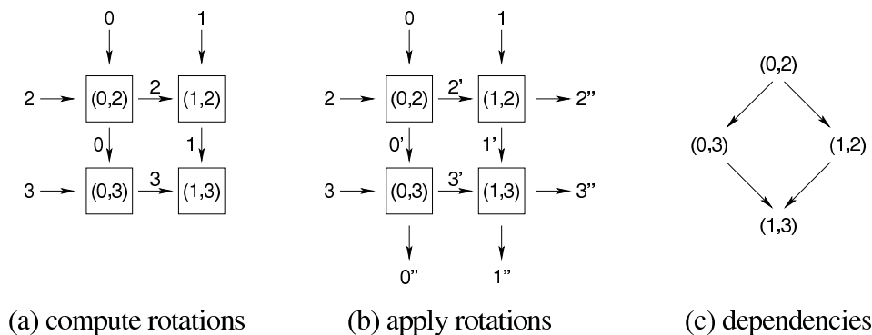
Figure 4: A block transformation of our parallel Hestenes-Jacobi method. In a first phase (a) we compute the rotations (0, 2) , (1, 2) , (0, 3) , and (1, 3) , and store them locally. During the second phase (b) rows 0 to 3 are streamed into the array once again, this time in order to apply the rotations.
