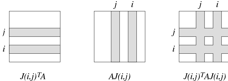
Figure 2: Jacobi transformation J(i, j) modifies rows and columns i and j of matrix A . Premultiplication J(i, j)^T A effects rows i and j , and postmultiplication AJ(i, j) columns i and j .
