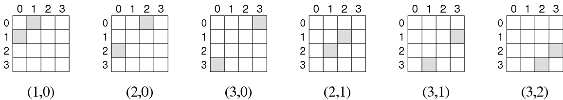
Figure 1: Sweep of Jacobi transformations for a symmetric 4 \times 4 matrix. We use the index pair (i, j) as a shorthand for the notation J(i, j, \theta) .
