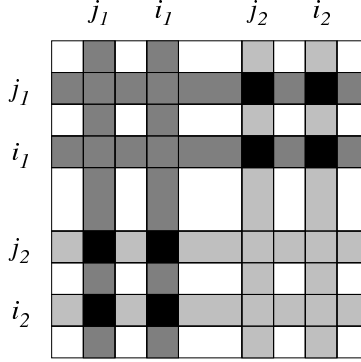
Figure 3: Two Jacobi transformations J(i_1, j_1) and J(i_2, j_2) are nearly independent with the exception of the eight black elements that are modified by both Jacobi updates.
