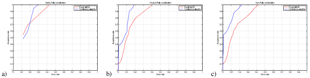
Figure 3: ROC curves for a single trial showing three different classifier combination strategies with and without confidence weighting. a) voting combination rule; b) product rule; c) sum rule. In all cases the top curve is generated by a weighted rule
