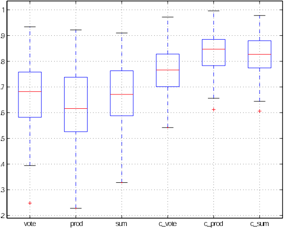
Figure 4: Performance of the Bayesian combination scheme as compared to the traditional combination techniques. The first three boxes correspond to voting, product and sum rules. The next group of three corresponds to the same rules but applied to the weighted classifier scores. Each box represents the data within 25th and 75th percentile, with the mean marked as a horizontal line. The whiskers of the plot relate to the variance of the accuracy of the classifiers over the set of trials
