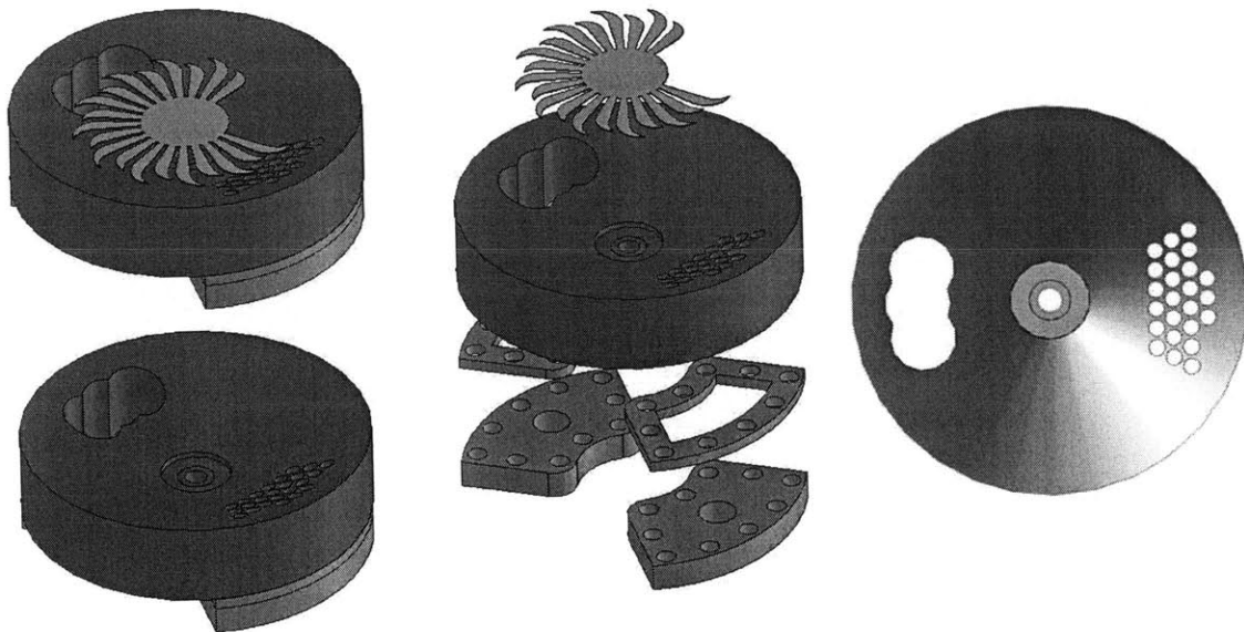
(Figure 5.2: different views of solid models of test valve)
