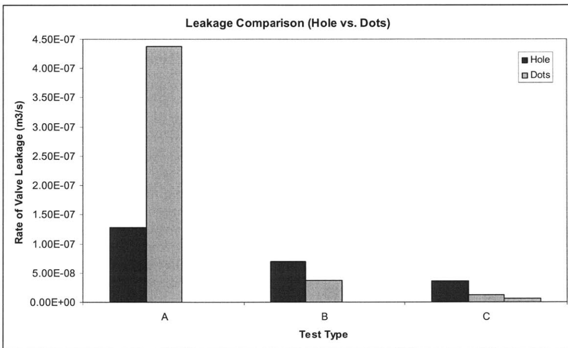
(Figure 5.7: valve leak comparison for meshed and unmeshed ports)
