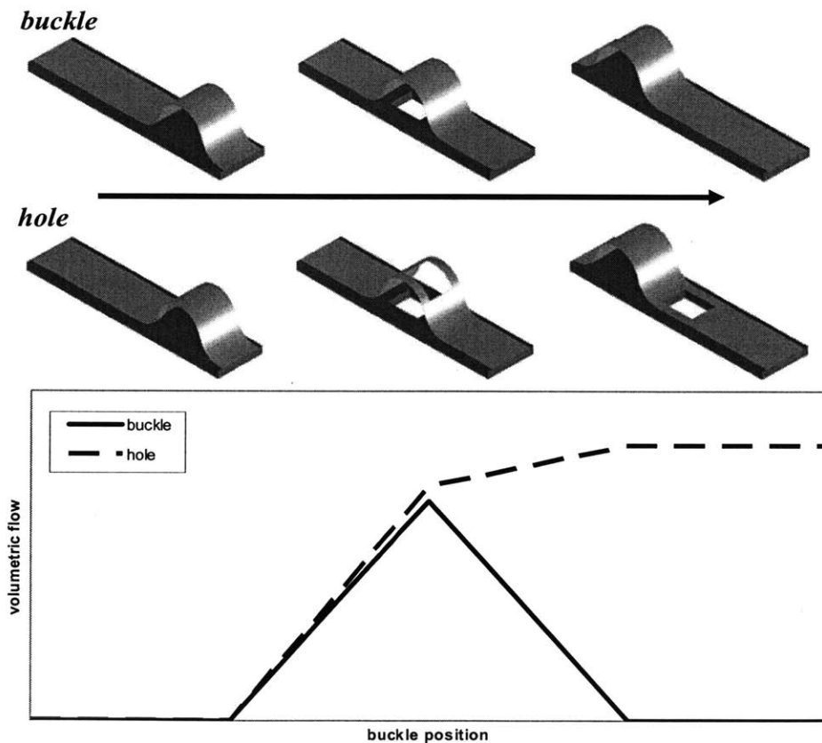
(Figure 3.14: WaveFlex opening modes & effect on flow)
