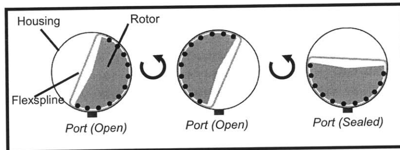
(Figure 3.6: WaveFlex system sketch)
