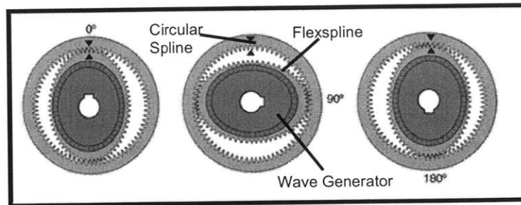
(Figure 3.5 20 : harmonic drive)
