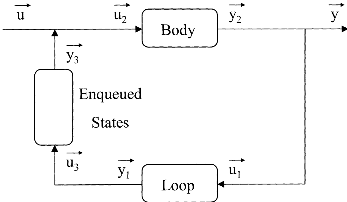
Figure 3-1: Labelled feedback loop
