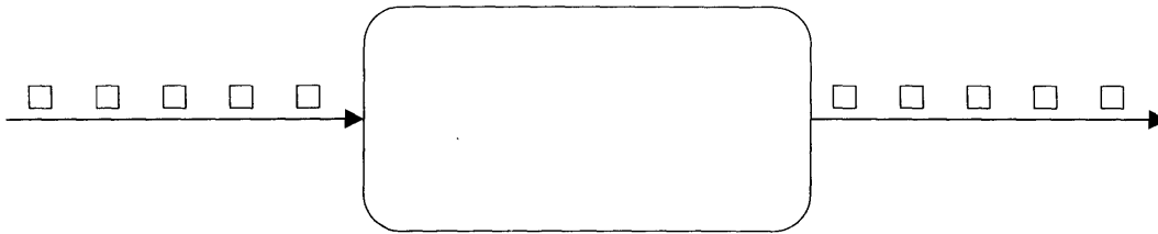
Figure 2-1: StreamIt filter
