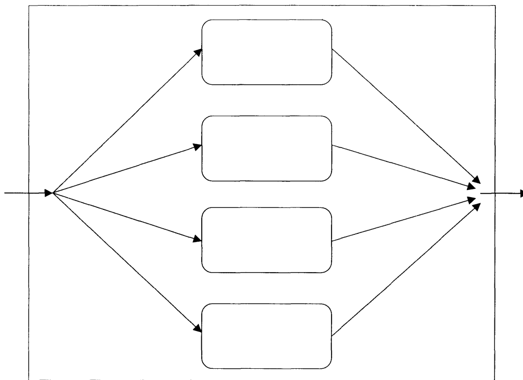
Figure 2-3: StreamIt splitjoin
