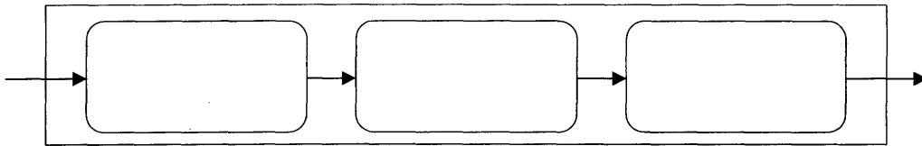
Figure 2-2: StreamIt pipeline
