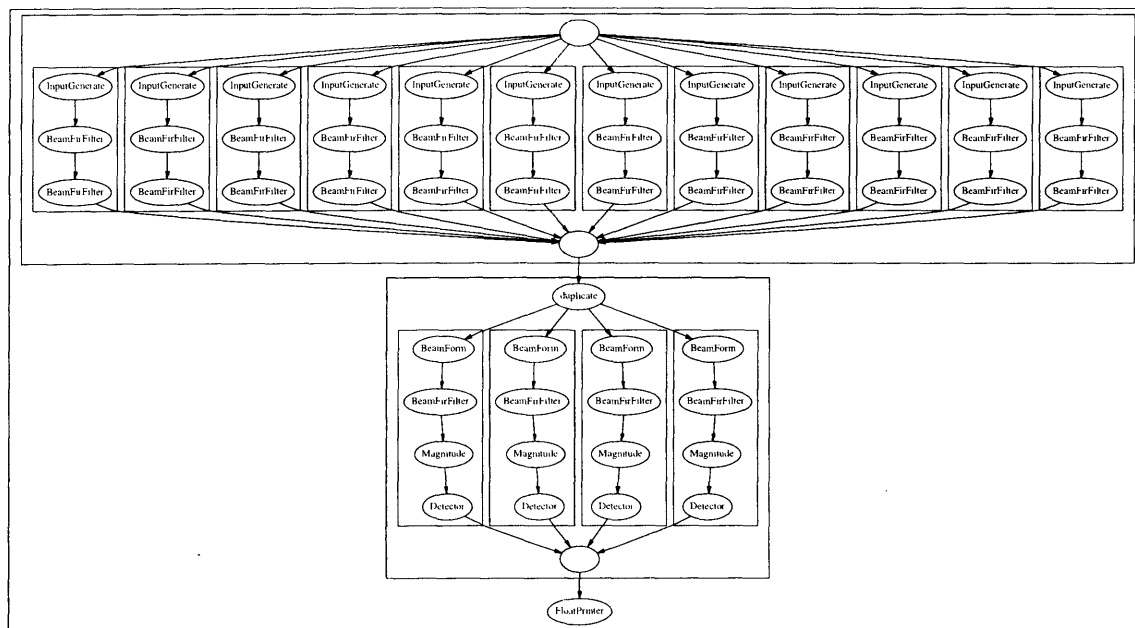
Figure 1-1: A DSP block diagram of the application Beamformer
