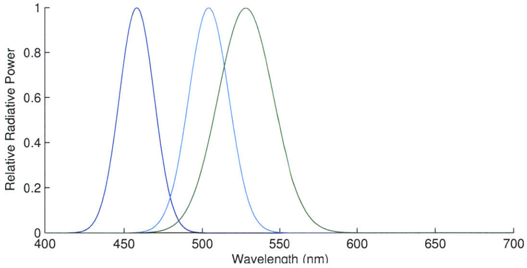
Figure C-2: Relative radiative power distribution for simulated Luxeon LED lights. From left to right, the curves represent the blue, cyan, and green LEDs
