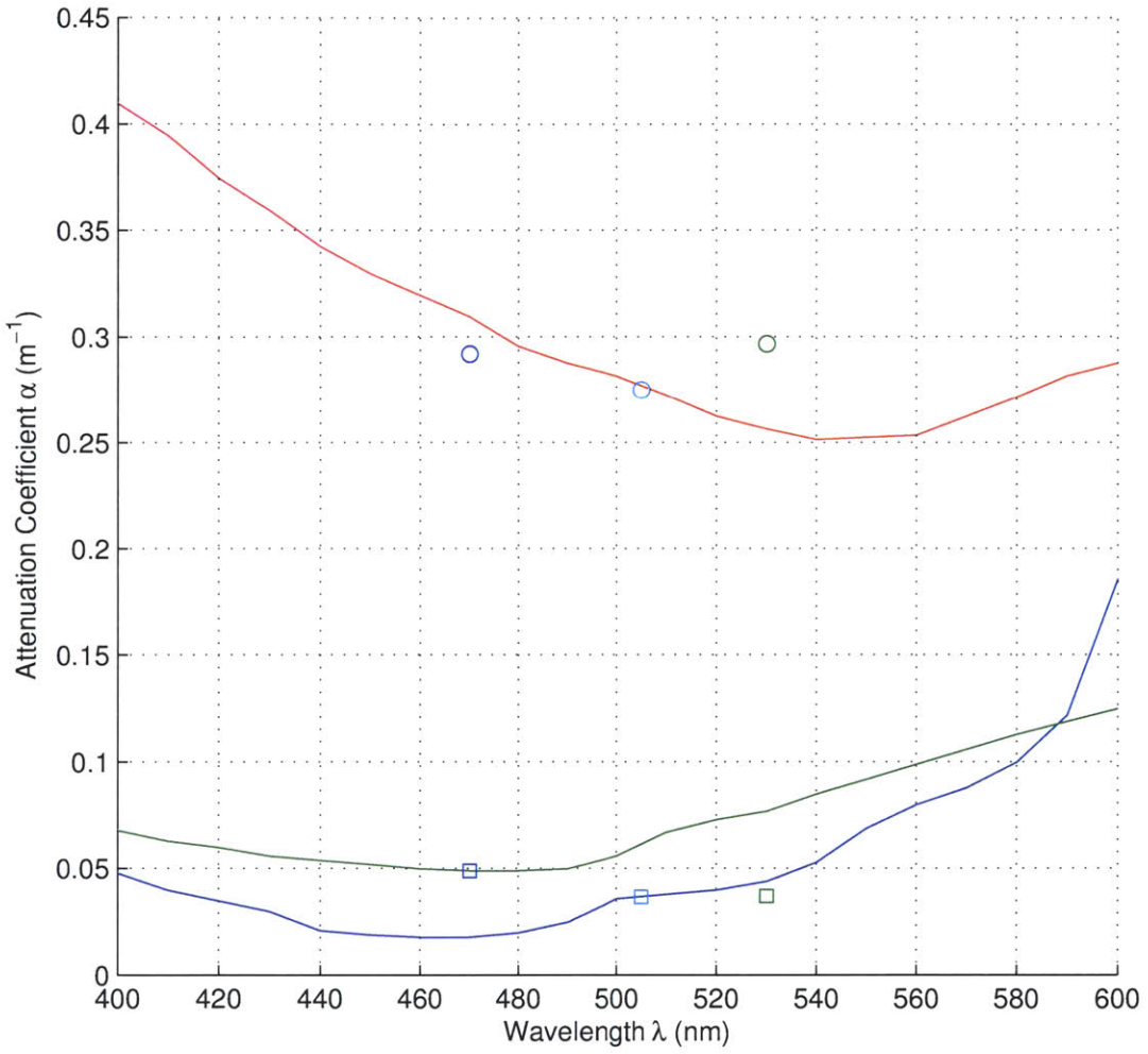
Figure 4-9: The attenuation coefficient measured in the MIT Towtank (squares) and at WHOI (circles) for three wavelengths. The data is presented with the distilled, deep ocean, and coastal water attenuation coefficient data from Figure 2-6. The wavelengths (470, 505, and 530 nm) correspond to the peak wavelengths of the Luxeon LEDs (blue, cyan, and green).
