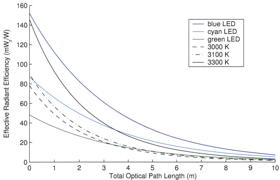
Figure 4-33: Total radiative efficiency of Luxeon 5W LEDs and simulated Halogen lights after propagating through simulated coastal ocean water similar to that seen at Woods Hole, MA.
