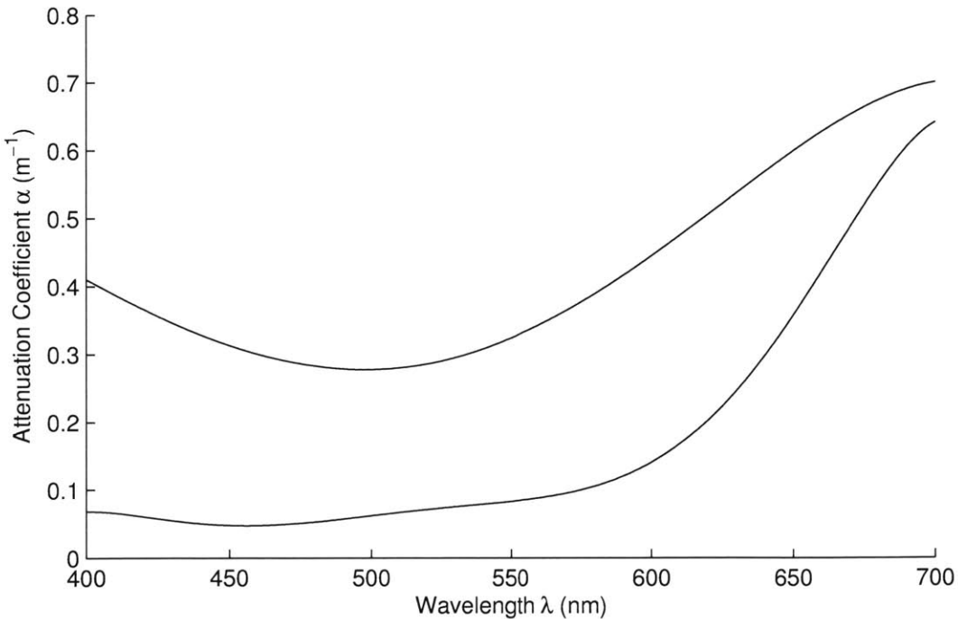
Figure C-5: Attenuation curves of simulated WHOI water(top) and simulated deep ocean water (bottom)
