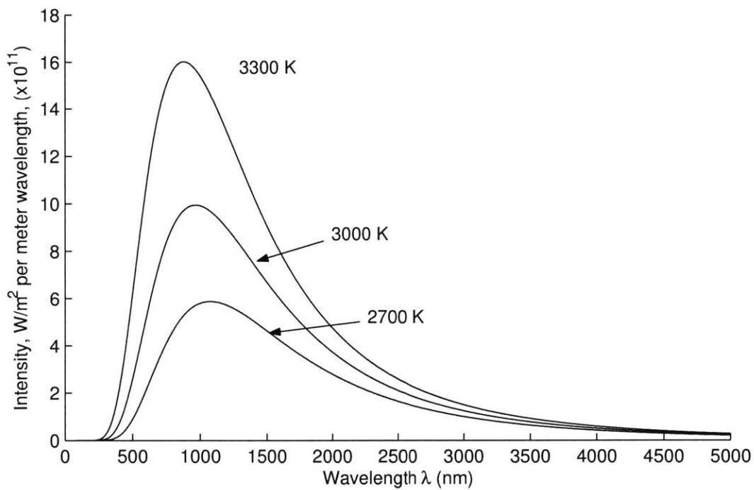
Figure 2-2: Intensity distribution for continuous spectrum blackbody radiation at color temperatures T = 2700 \text{ K} , T = 3000 \text{ K} , and T = 3300 \text{ K} .
