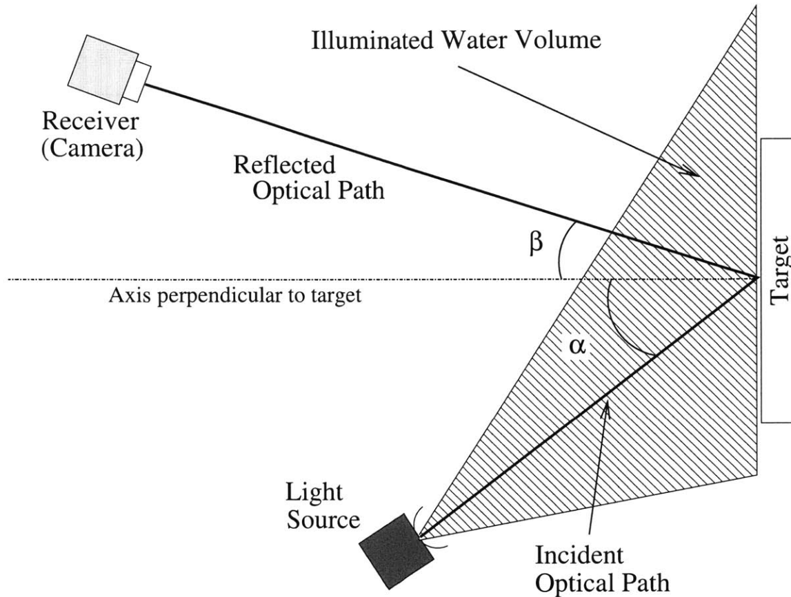
Figure 2-13: Diagram showing a typical underwater lighting and imaging arrangement. Light angle of incidence is shown as \alpha . The reflected angle is shown as \beta . The incident optical path from the light source to the center of the target is labeled. The length of this path, the incident optical path length, is often abbreviated incident OPL. The reflected optical path from the target to the camera is also labeled. The length of this path is the reflected OPL. The total optical path length is the total OPL.
