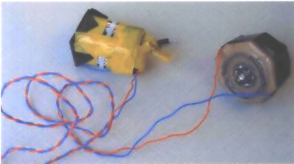
Figure 5-1: LED Candle Prototype
