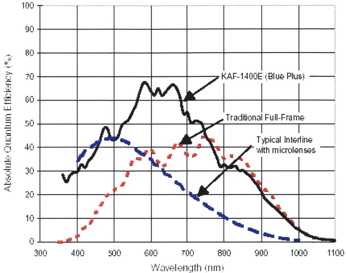
Figure 2-8: Spectral response of comparable image sensor technologies, from Kodak technical paper [10]
