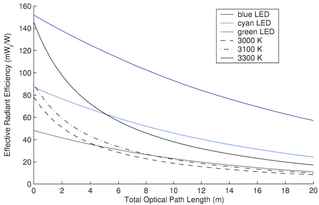
Figure 4-32: Total radiative efficiency of Luxeon 5W LEDs and simulated Halogen lights after propagating through simulated deep ocean water
