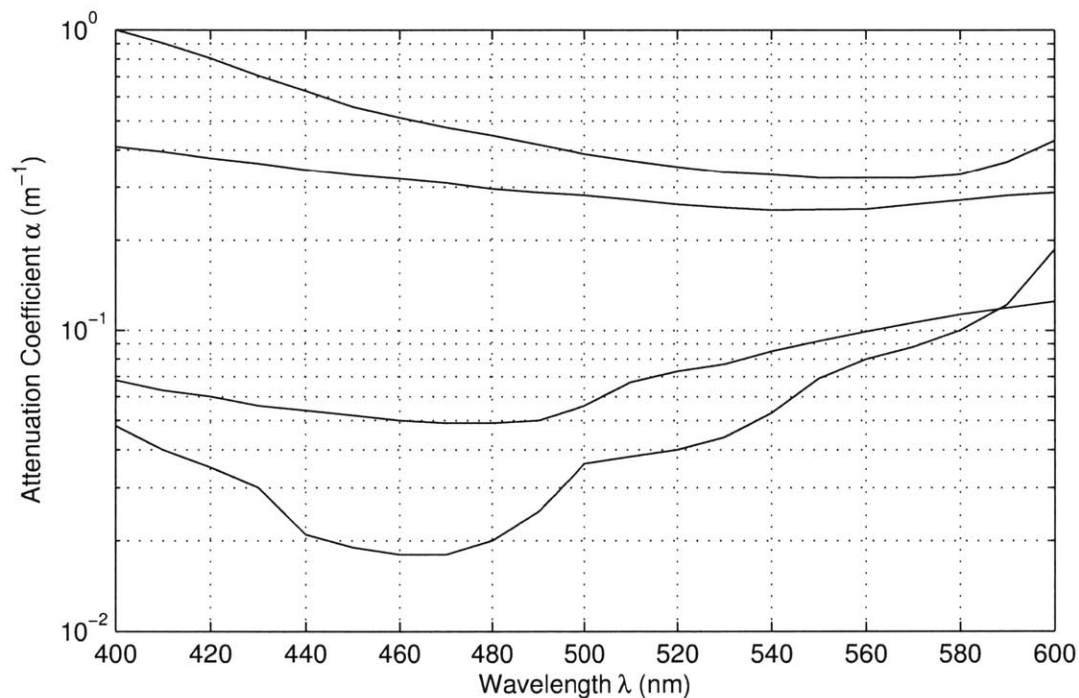
Figure 2-6: Attenuation coefficient for different water conditions adapted from Funk, et al. [9]. From top to bottom (dirtiest to cleanest) the curves correspond to bay water, coastal water, deep ocean water, and distilled water.
