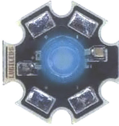
Figure 3-1: The Luxeon V Star, 5W LED light with hexagonal base, manufactured by Lumileds, San Jose, CA.
