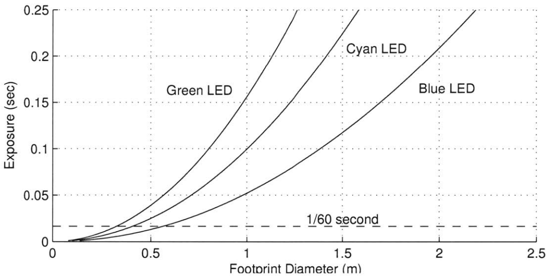
Figure 4-27: Predicted coverage of a single Luxeon 5W LED and the resulting required exposure of a Canon S230 digital camera for R = 0.1 . This represents a more reasonable estimate of an actual illuminated footprint. R = 0.1 was chosen to take into account off-axis illumination at the fringe and uneven illumination rather than a perfect distribution of flux.
