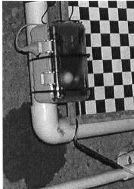
Figure 3-5: The Extech light meter inside its waterproof Otter Box housing. The exposed photodiode (under the white diffuser dome), the penetration for the serial cable, and the serial cable splice are visible. The Extech sits on the target used during the WHOI experiments.
