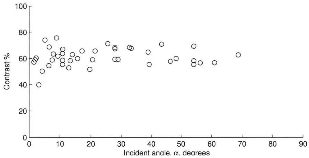
Figure B-15: Combined blue and green channel contrast response vs. incident angle of illumination, \alpha , of Canon S230 camera for Luxeon 5W cyan LED, with reflector , in the MIT Towntank. Camera is located 1.74 m from the target at an angle \beta = 6.1^\circ from perpendicular.
