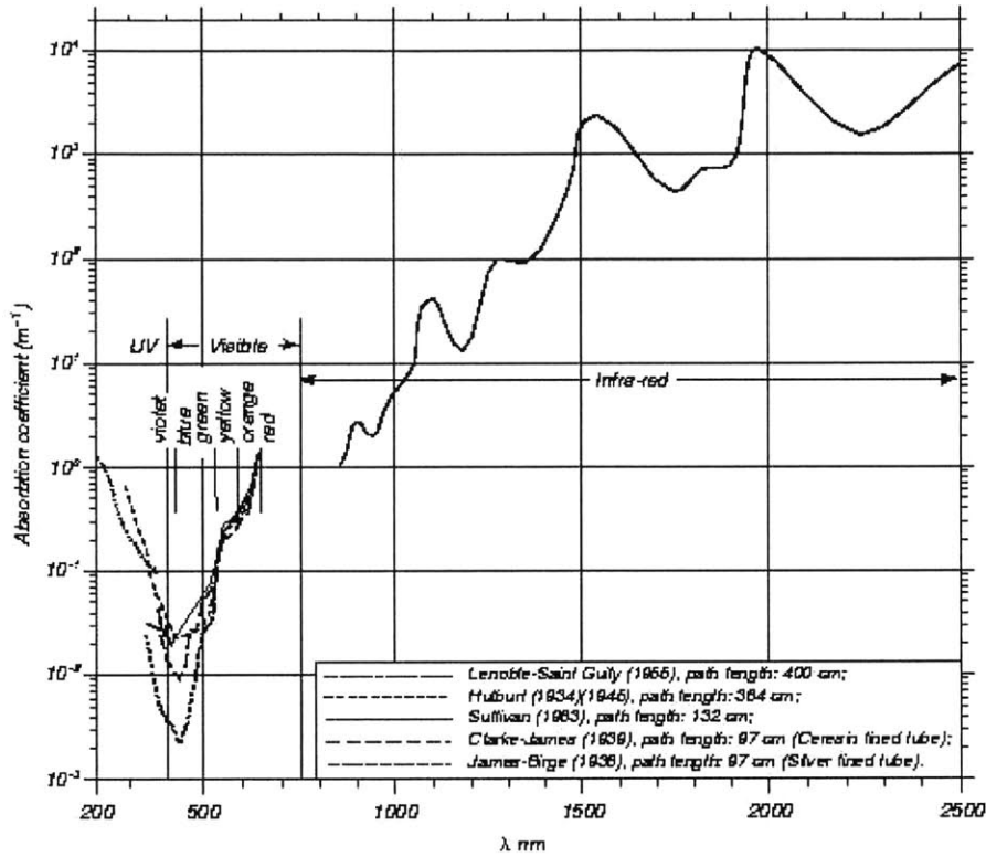
Figure 2-3: Absorption coefficient for pure water as a function of wavelength \lambda of the radiation. Taken from Morel [3] by way of Stewart [4].
