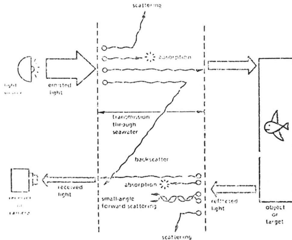
Figure 2-12: Block diagram of basic imaging situation, from [9]
