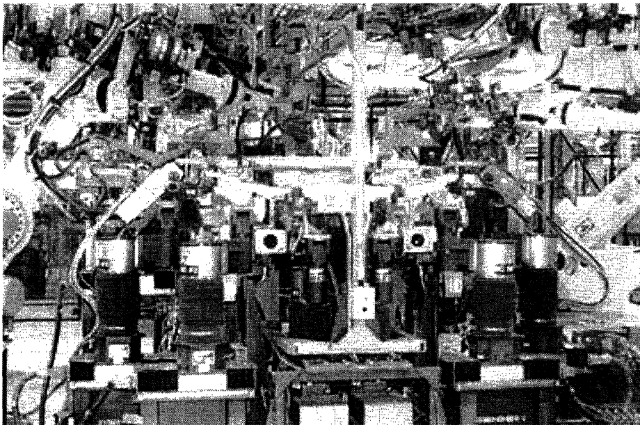
Figure 2.1: Station comprised of several PRRT units surrounded by RSW robots. The PRRTs are the smaller piston type arms 21 .
