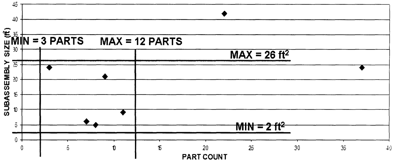
Figure 3.5: Auto weld 4 guns
