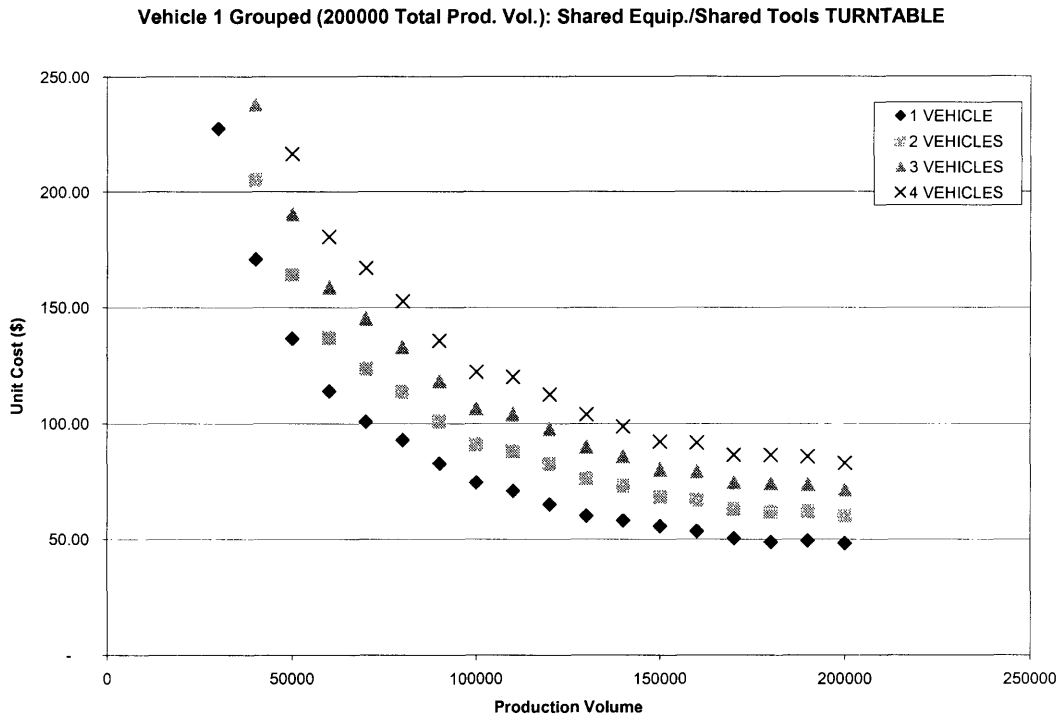
Figure 4.5: Cost outputs for the four vehicle counts with shared equipment and shared tools and turntable as the override.
