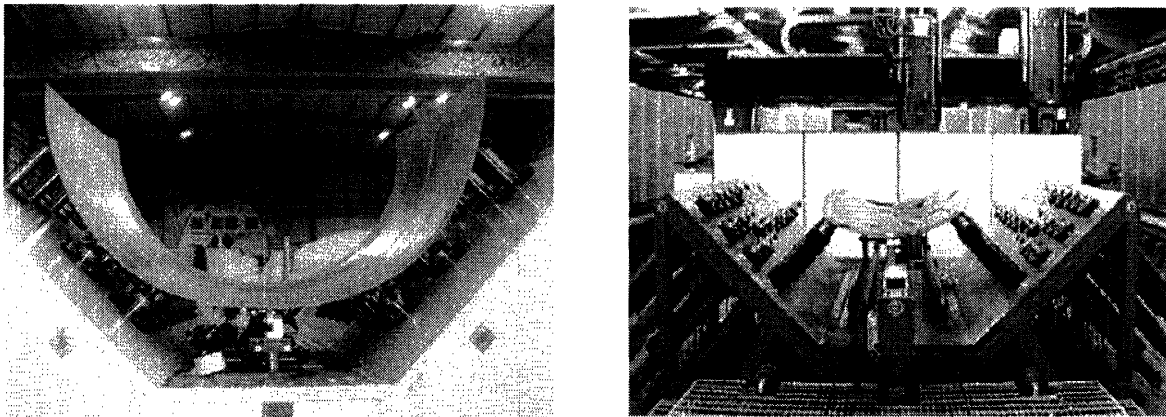
Figure 5.1: Bombardier Aerospace technology: a) tricept tooling and b) axis nacelle tooling 3 .
