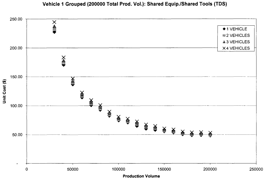
Figure 4.3: Cost outputs for the four vehicle counts with shared equipment and shared tools and TDS as the override.
