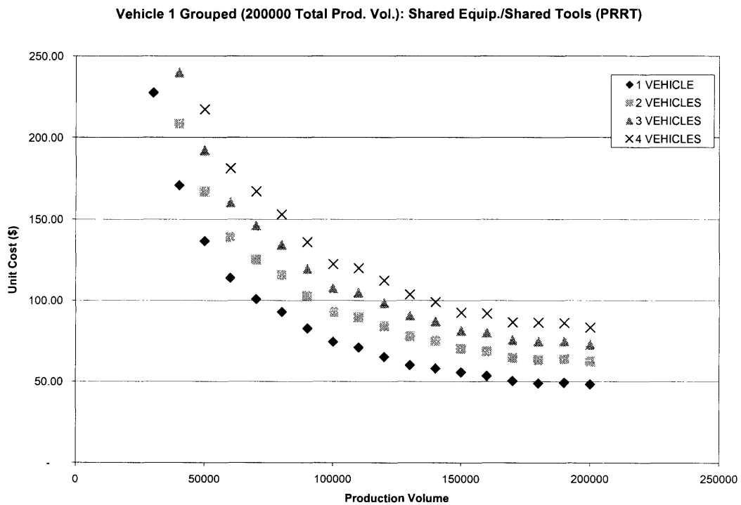
Figure 4.4: Cost outputs for the four vehicle counts with shared equipment and shared tools and PRRT as the override.
