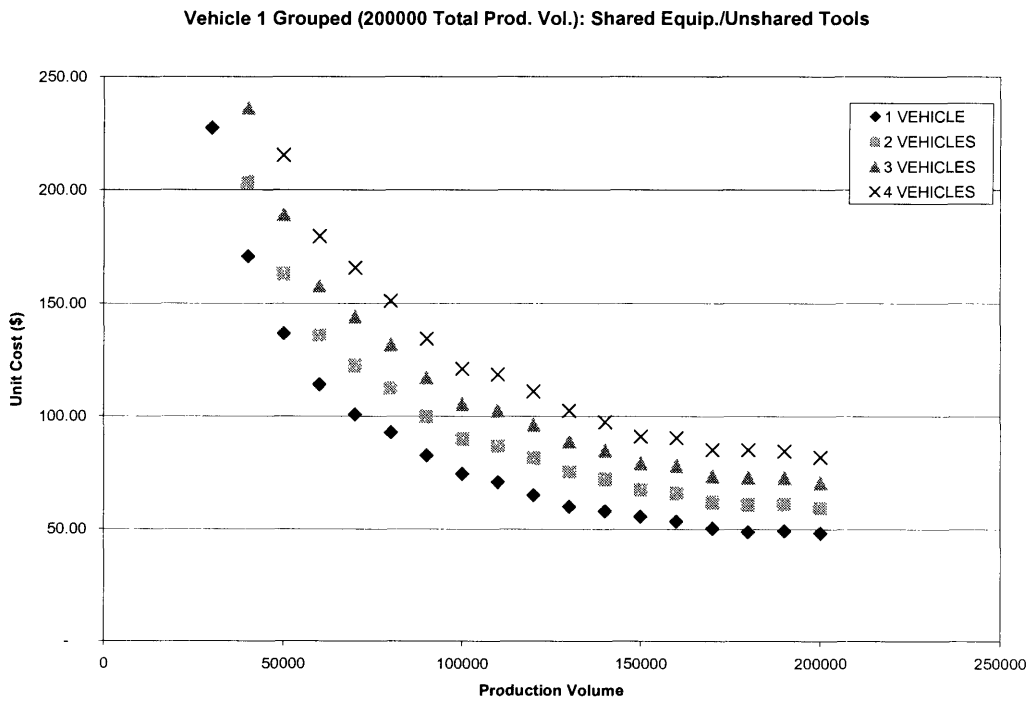
Figure 4.2: Cost outputs for the four vehicle counts with shared equipment and unshared tools.
