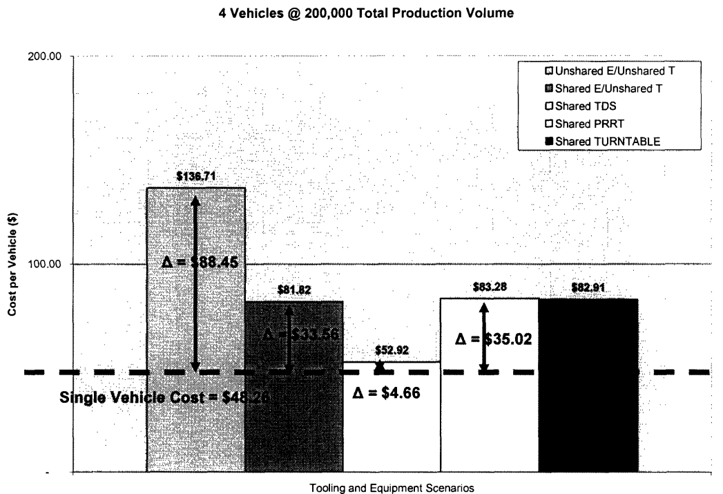
Figure 4.8: Graph of different sharing strategies for 4 vehicles at 200,000 total production volume
