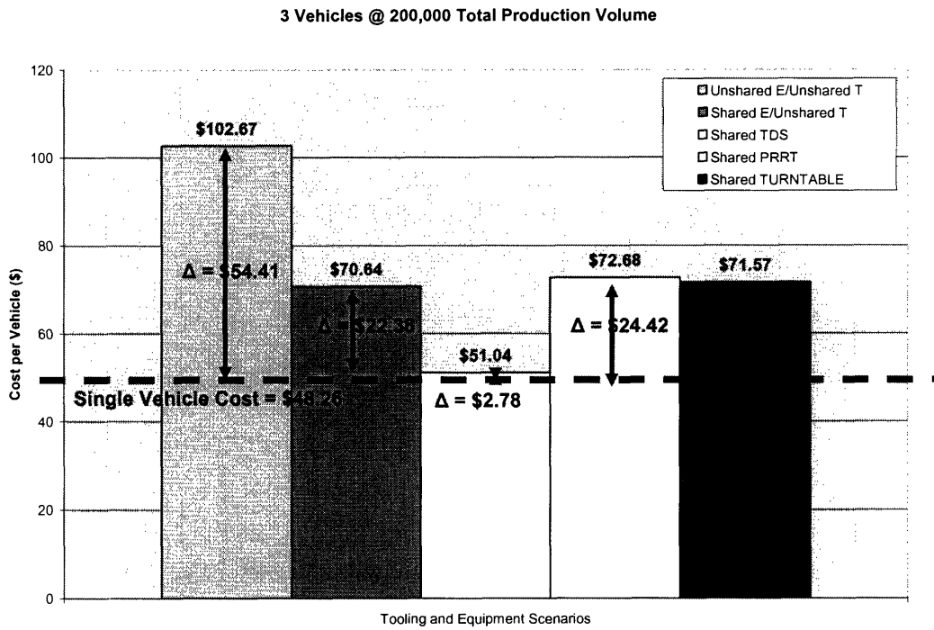
Figure 4.7: Graph of different sharing strategies for 3 vehicles at 200,000 total production volume
