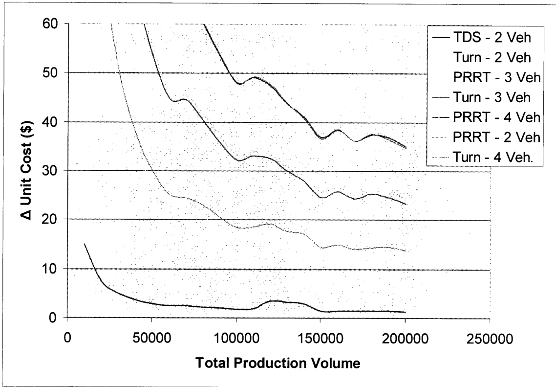
Figure 4.10: Graph showing the change in unit cost compared to single vehicle production as a function of total production volume.
