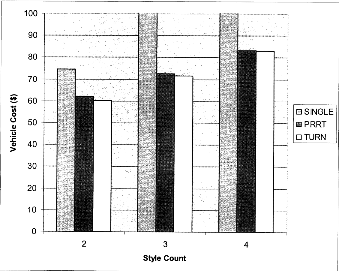
Figure 4.9: Comparison of single production, turntable, and PRRT vehicle costs vs. style count.
