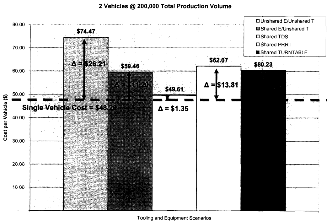
Figure 4.6: Graph of different sharing strategies for 2 vehicles at 200,000 total production volume.
