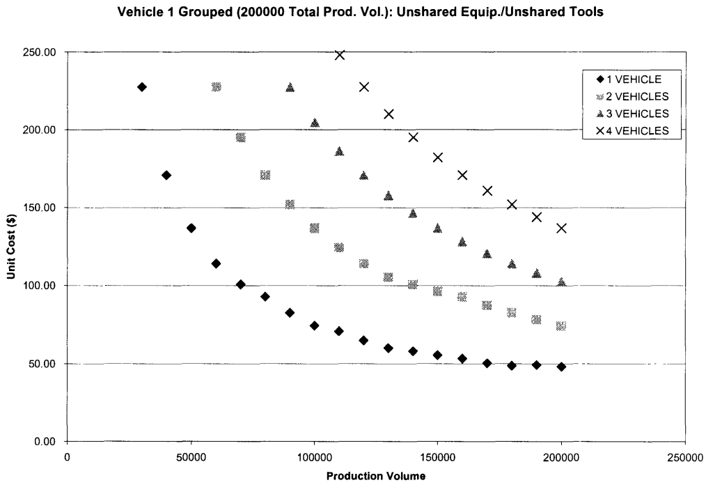
Figure 4.1: Cost outputs for the four vehicle counts with unshared equipment and unshared tools.
