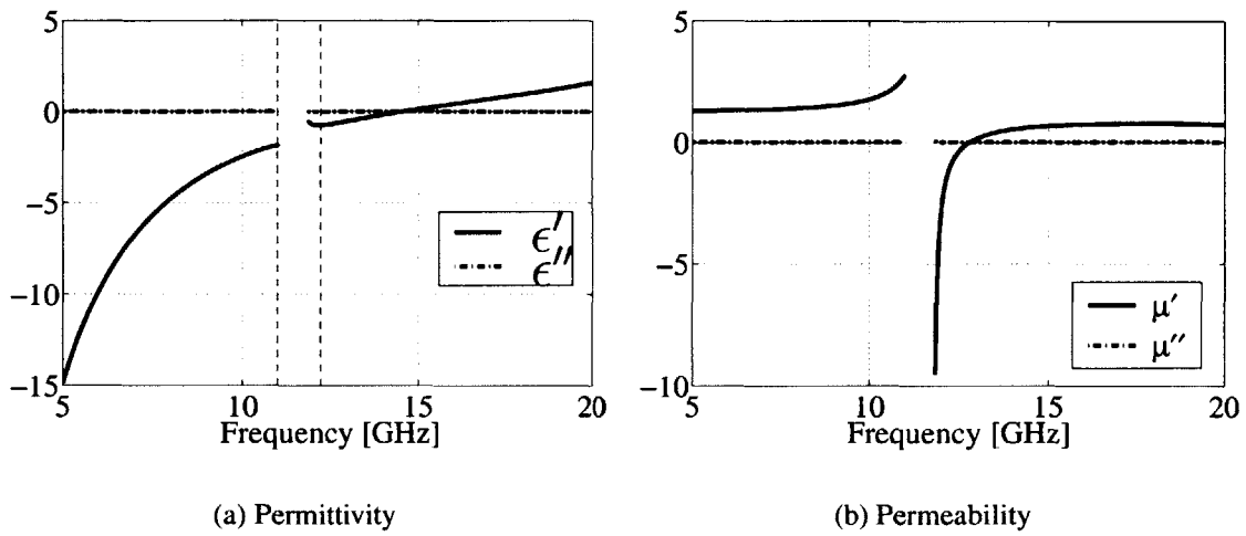
Figure 2-7: Retrieved \epsilon and \mu (real and imaginary parts) for a one-cell metamaterial shown in Fig. 2-1. The vertical dashed lines denote the limits of the resonance band.
