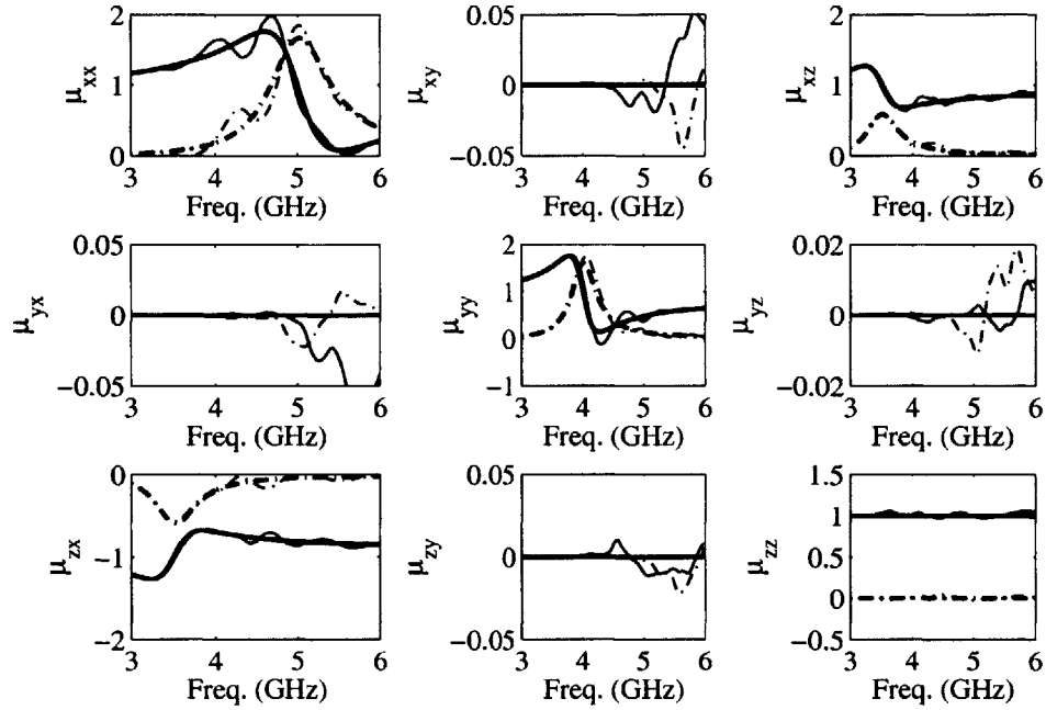
Figure 4-7: Comparison of the retrieved and the true \bar{\bar{\mu}} of an Omega ferrite medium (clean data). The solid and dotted-dashed lines are for the real and imaginary parts, respectively. The thick and thin lines are for the true and the retrieved results, respectively.
