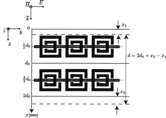
Figure 2-1: Illustration of the effective boundaries of a 2-cell metamaterial. The SRRs and rods are periodic along \hat{y} and \hat{z} directions with periodicity a_y = 4\text{mm} , a_z = 3\text{mm} . The unit-cell thickness ( d_0 ) in the direction of wave incidence is 4 mm. We choose the first and the last unit cell boundary as the reference plane for the parameters x_1 and x_2 , respectively. The value of x_1 and x_2 are positive/negative if the dash lines are below/above their reference planes. The thickness of the effective homogeneous medium is 2d_0 + x_2 - x_1 [mm].
