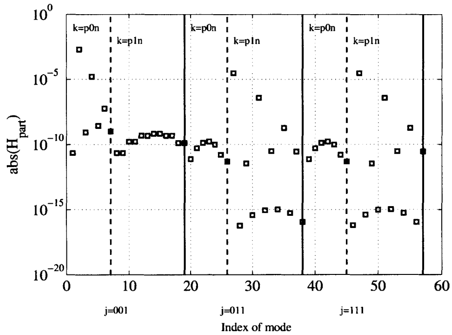
Figure 5-12: Magnitude of H_z in the oblate coordinate system
