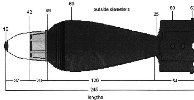
Figure 5-19: A UXO object labeled as U2 (Courtesy of Dr. K. O’Neill)
