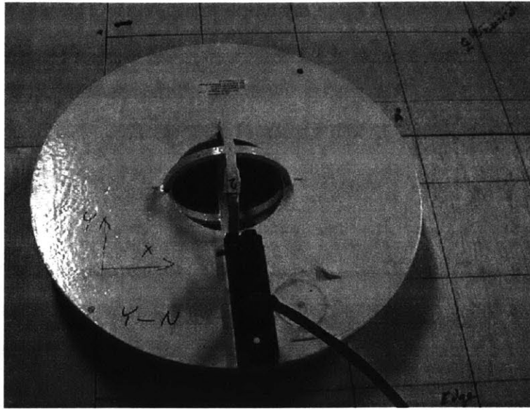
Figure 5-3: Geophex GEM-3 instrument sensor head (Courtesy of Dr. K. O'Neill)
