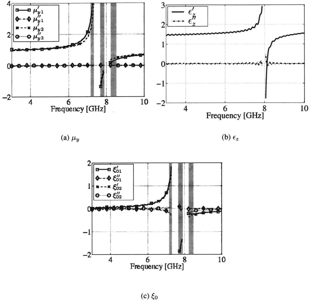
Figure 3-5: Retrieval results for a lossless edge-coupled SRR metamaterial whose unit cell is shown in Fig. 3-1(a), using a lossless retrieval for bianisotropic media. The subscripts ‘1’ and ‘2’ denote the results obtained from the proposed method 1 and method 2, respectively. Those results difficult to read within the resonance band are not shown here. The shaded region indicates the frequency range where the mismatch of either \mu_y or \xi_0 exceeds the threshold ( RM > 0.25 ).
