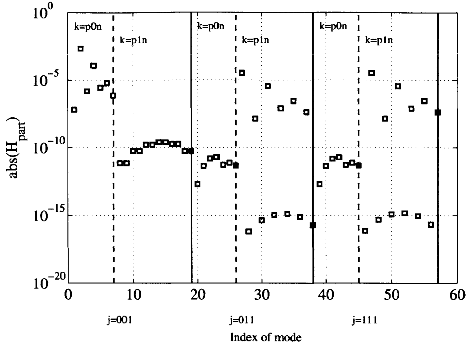
Figure 5-10: Magnitude of H_z in the prolate coordinate system for the oblate spheroidal body
