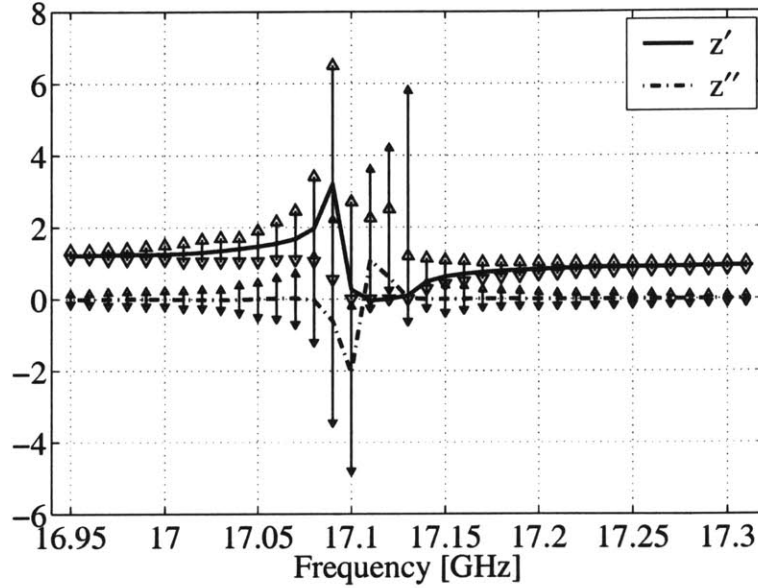
Figure 2-5: Range of z (real and imaginary parts) for tolerance \delta_r = 0.015 and \delta_t = 0.0 in Eqs. (2.11). The impedance is for a 3-cell metamaterial shown in Fig. 2-1.
