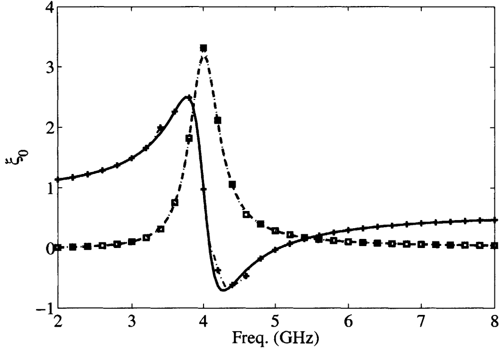
Figure 4-1: Comparison of the retrieved and the true \xi_0 of an Omega medium
