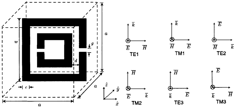
(a) Structure of the edge-coupled SRR: The unit cell is a cube of edge a = 5.25 mm. The parameters of the SRR are g = d = 0.125 mm, c = 0.25 mm, and w = 3.75 mm. The background medium is free space.
