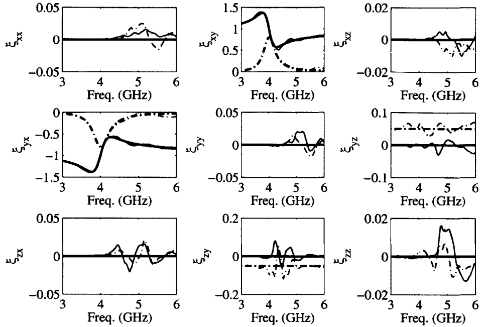
Figure 4-8: Comparison of the retrieved and the true \bar{\xi} of an Omega ferrite medium (clean data). The solid and dotted-dashed lines are for the real and imaginary parts, respectively. The thick and thin lines are for the true and the retrieved results, respectively.
