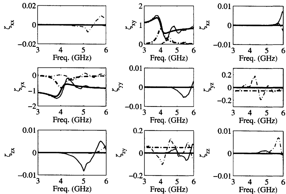
Figure 4-17: Comparison of the retrieved and the true \zeta of an Omega ferrite medium (5% noise). The solid and dotted-dashed lines are for the real and imaginary parts, respectively. The thick and thin lines are for the true and the retrieved results, respectively.
