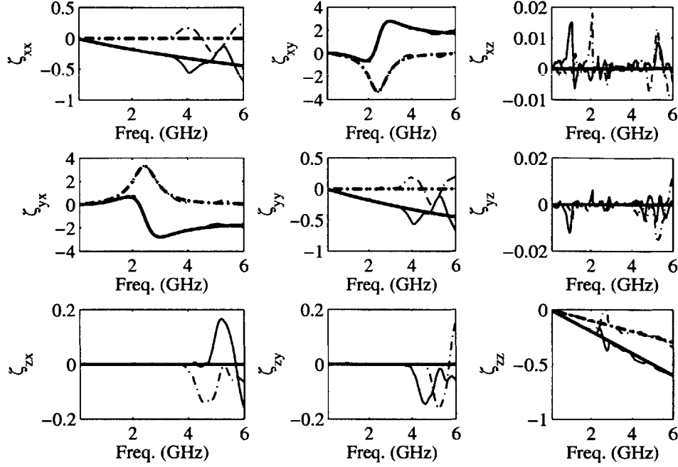
Figure 4-5: Comparison of the retrieved and the true \bar{\zeta} of a Chiroferrite medium. The solid and dotted-dashed lines are for the real and imaginary parts, respectively. The thick and thin lines are for the true and the retrieved results, respectively.
