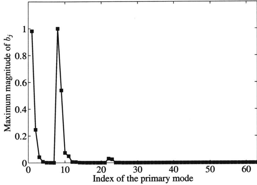
Figure 5-14: Maximum magnitude of b_j
