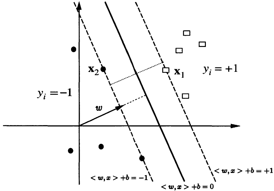
Figure 5-31: Canonical optimal hyperplane in the feature space
