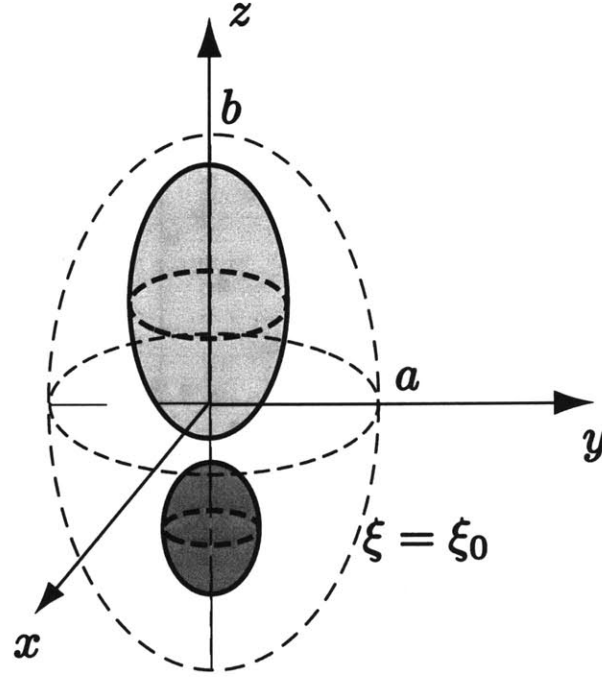
Figure 5-13: Composite object composed of two spheroids. We expand the fields in a spheroidal coordinate system with the surface of the spheroid \xi = \xi_0 enclosing the composite object. The interfocal distance d is 1.6 m in the simulation.
