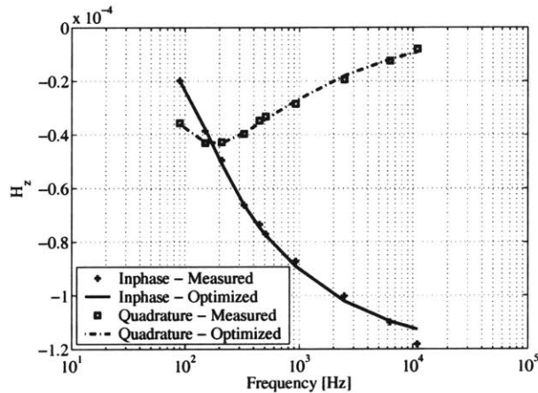
Figure 5-8: Comparison of the measured field and the optimized field at point (x, y, z) = (0.05, 0.05, 0.0) m for the spheroid shown in Fig. 5-7.
