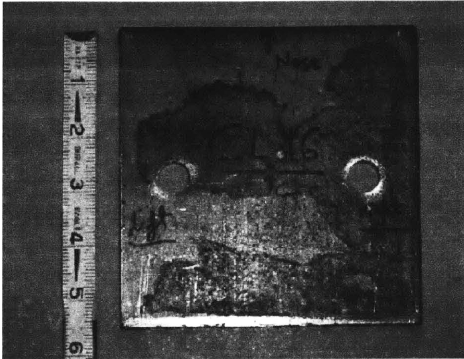
Figure 5-24: A square metallic plate labeled as CL16 (Courtesy of Dr. K. O'Neill)
