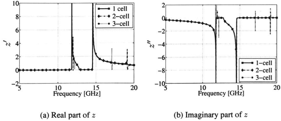
Figure 2-2: Optimized impedance z for 1, 2 and 3 cells of metamaterial of Fig. 2-1 in the direction of propagation.
