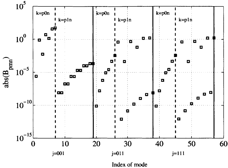
Figure 5-9: Magnitude of B_k^{(j)} in the prolate coordinate system for the oblate spheroidal body
