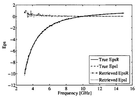
(a) Permittivity
