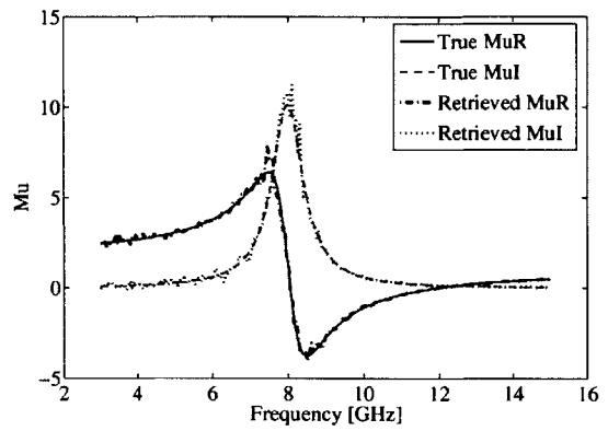
(b) Permeability
