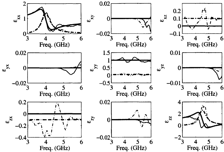
Figure 4-14: Comparison of the retrieved and the true \bar{\epsilon} of an Omega ferrite medium (5% noise). The solid and dotted-dashed lines are for the real and imaginary parts, respectively. The thick and thin lines are for the true and the retrieved results, respectively.
