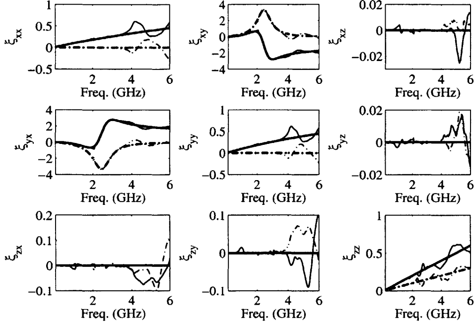
Figure 4-4: Comparison of the retrieved and the true \bar{\xi} of a Chiroferrite medium. The solid and dotted-dashed lines are for the real and imaginary parts, respectively. The thick and thin lines are for the true and the retrieved results, respectively.
