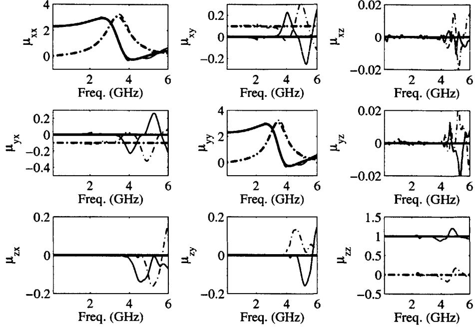
Figure 4-3: Comparison of the retrieved and the true \bar{\mu} of a Chiroferrite medium. The solid and dotted-dashed lines are for the real and imaginary parts, respectively. The thick and thin lines are for the true and the retrieved results, respectively.
