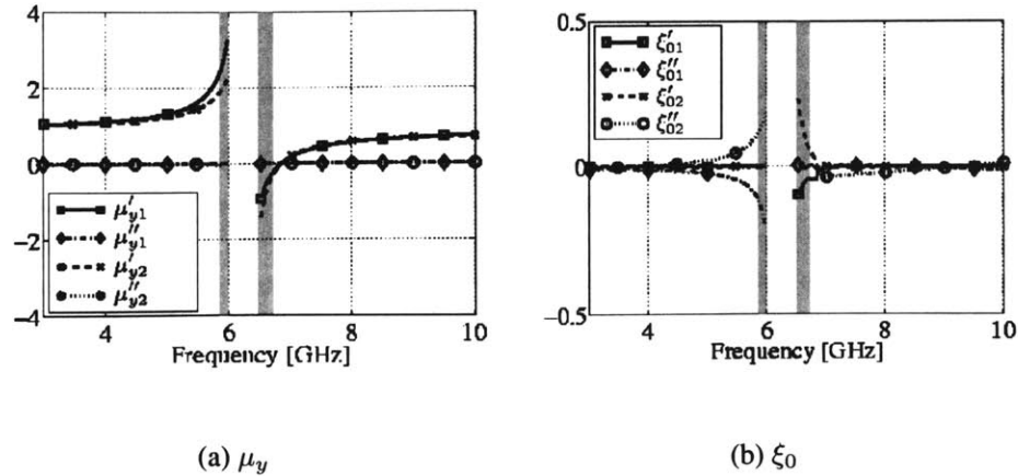
Figure 3-7: Retrieved results for a broadside-coupled SRR metamaterial, where a negligible \xi_0 is observed (except around the resonance: 5.9 GHz \sim 6.7 GHz. See Table 3.2). Those results difficult to read within the resonance band are not shown here. The shaded region indicates the frequency range where the mismatch of either \mu_y or \xi_0 exceeds the threshold ( RM > 0.25 ).
