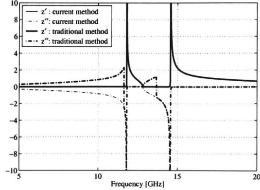
Figure 2-3: Comparison of the retrieved impedance z (real and imaginary parts) for one cell of metamaterial shown in Fig. 2-1 by the method presented in this chapter and a traditional method using only the requirement z' \geq 0 .
