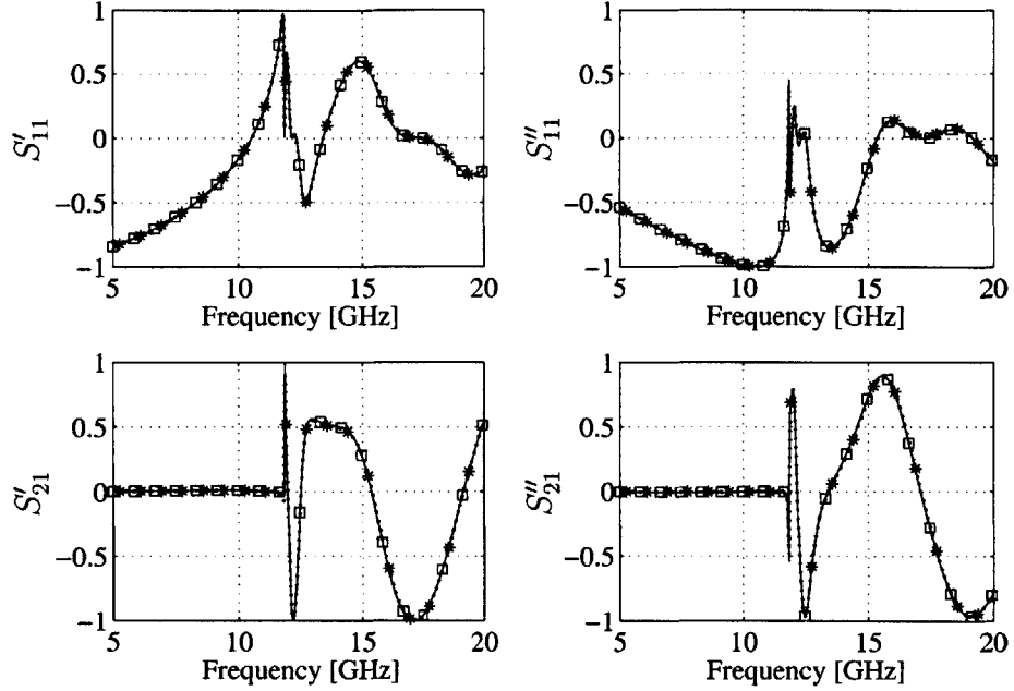
Figure 2-6: S_{11} and S_{21} (real and imaginary parts) for 3 cells: comparison between FDTD results (dot line with *) and calculated S parameters based on the retrieved \epsilon and \mu (solid line with \square ) for a one-cell metamaterial shown in Fig. 2-1.
