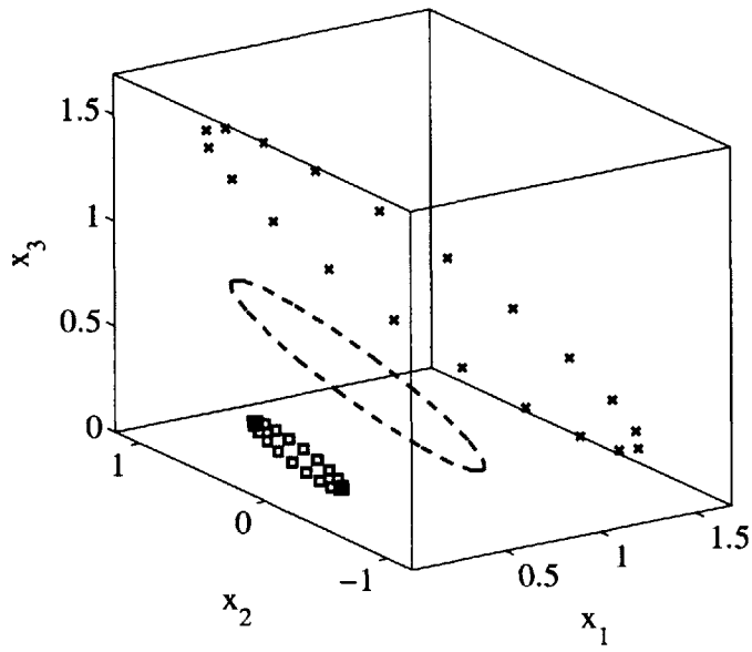
(b) Feature space
