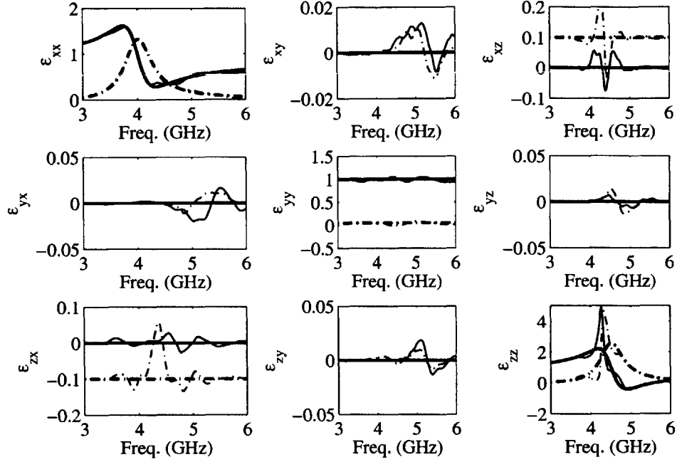
Figure 4-6: Comparison of the retrieved and the true \bar{\epsilon} of an Omega ferrite medium (clean data). The solid and dotted-dashed lines are for the real and imaginary parts, respectively. The thick and thin lines are for the true and the retrieved results, respectively.
