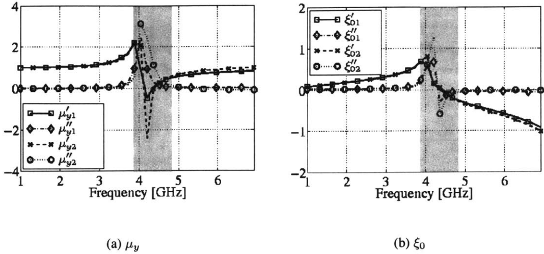
Figure 3-6: Retrieval results for a lossy edge-couple SRR metamaterial, whose unit cell is the same that in Fig. 3-1(a) except that the background material is lossy ( \sigma = 0.042 S/m, \epsilon_r = 3.4 ). Those results difficult to read within the resonance band are not shown here. The shaded region indicates the frequency range where the mismatch of either \mu_y or \xi_0 exceeds the threshold ( RM > 0.25 ).
