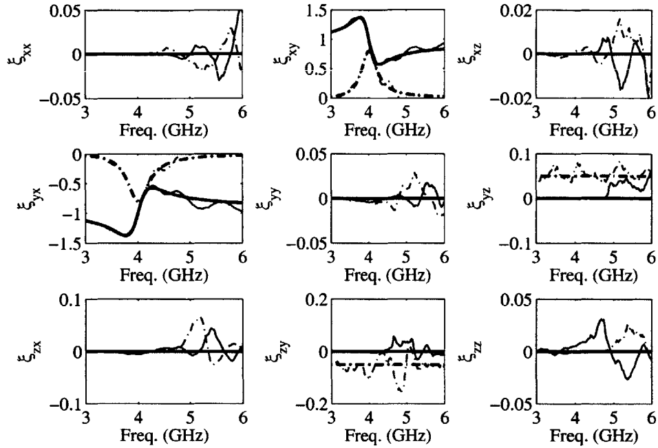
Figure 4-12: Comparison of the retrieved and the true \bar{\xi} of an Omega ferrite medium (2% noise). The solid and dotted-dashed lines are for the real and imaginary parts, respectively. The thick and thin lines are for the true and the retrieved results, respectively.
