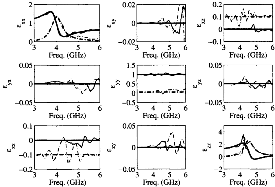
Figure 4-10: Comparison of the retrieved and the true \bar{\epsilon} of an Omega ferrite medium (2% noise). The solid and dotted-dashed lines are for the real and imaginary parts, respectively. The thick and thin lines are for the true and the retrieved results, respectively.
