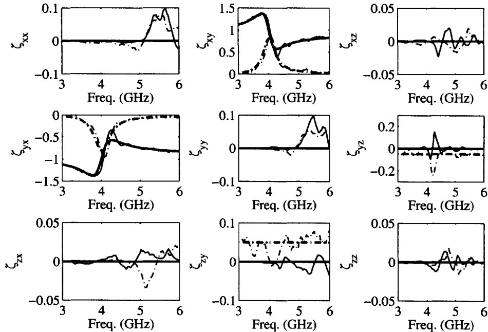
Figure 4-13: Comparison of the retrieved and the true \bar{\zeta} of an Omega ferrite medium (2% noise). The solid and dotted-dashed lines are for the real and imaginary parts, respectively. The thick and thin lines are for the true and the retrieved results, respectively.
