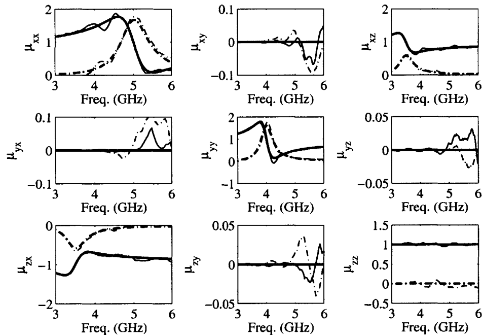
Figure 4-11: Comparison of the retrieved and the true \bar{\mu} of an Omega ferrite medium (2% noise). The solid and dotted-dashed lines are for the real and imaginary parts, respectively. The thick and thin lines are for the true and the retrieved results, respectively.
