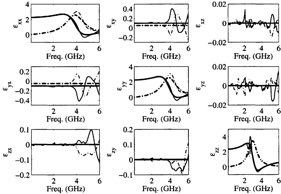
Figure 4-2: Comparison of the retrieved and the true \bar{\epsilon} of a Chiroferrite medium. The solid and dotted-dashed lines are for the real and imaginary parts, respectively. The thick and thin lines are for the true and the retrieved results, respectively.
