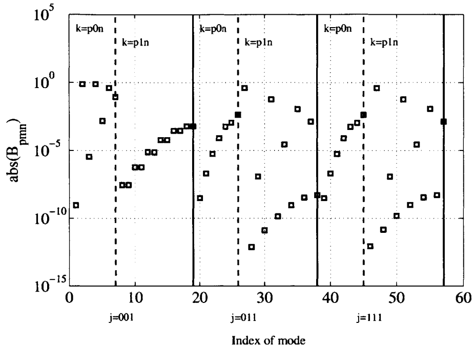
Figure 5-11: Magnitude of B_k^{(j)} in the oblate coordinate system
