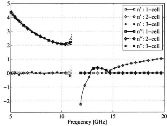
Figure 2-4: Retrieved refractive index n (real and imaginary parts) for 1, 2 and 3 cells of the metamaterial structure shown in Fig. 2-1.
