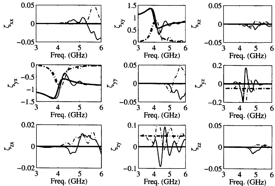
Figure 4-9: Comparison of the retrieved and the true \bar{\zeta} of an Omega ferrite medium (clean data). The solid and dotted-dashed lines are for the real and imaginary parts, respectively. The thick and thin lines are for the true and the retrieved results, respectively.
