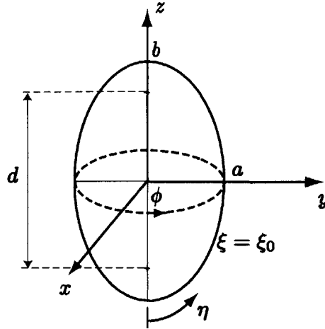
Figure 5-1: The prolate spheroidal coordinate system is specified by (\eta, \xi, \phi) , with -1 \leq \eta \leq 1, 1 \leq \xi \leq \infty , and 0 \leq \phi < 2\pi . The surface of a spheroid is given by \xi = \xi_0 = b/\sqrt{b^2 - a^2} , where a and b are minor and major semi-axis of the spheroid. The interfocal distance is given by d = 2\sqrt{b^2 - a^2} .
