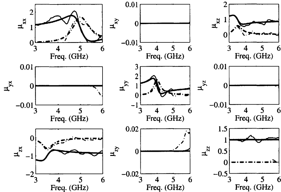
Figure 4-15: Comparison of the retrieved and the true \bar{\mu} of an Omega ferrite medium (5% noise). The solid and dotted-dashed lines are for the real and imaginary parts, respectively. The thick and thin lines are for the true and the retrieved results, respectively.
