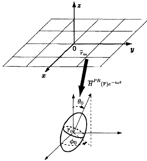
Figure 5-4: Illustration of the setup of the single spheroid inversion problem
