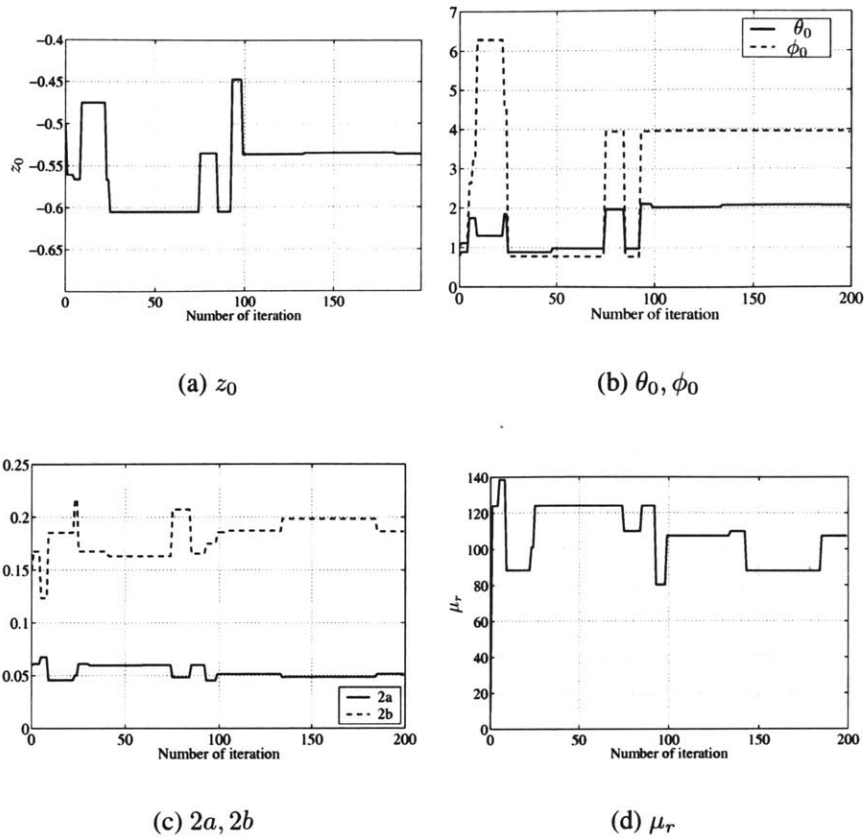
Figure 5-5: Optimization trajectory of parameters in the numerical model, in which the parameters of the hypothetical spheroid are z_0 = -0.55 m, \theta_0 = \frac{2\pi}{3} ( = 2.09 ), \phi_0 = \frac{5\pi}{4} ( = 3.93 ), 2a = 0.05 m, 2b = 0.20 m, and \mu_r = 100 .
