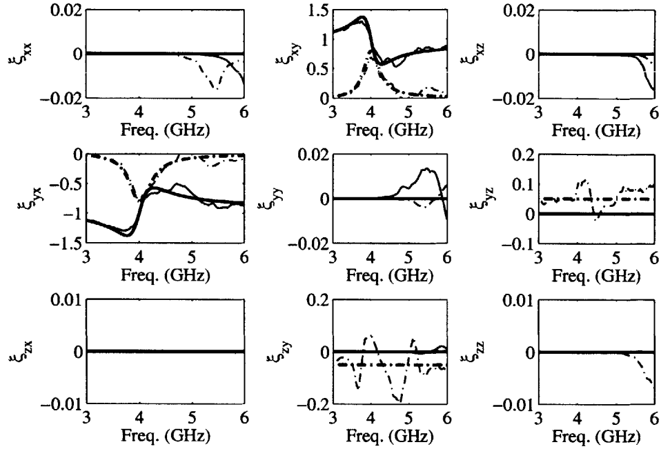
Figure 4-16: Comparison of the retrieved and the true \xi of an Omega ferrite medium (5% noise). The solid and dotted-dashed lines are for the real and imaginary parts, respectively. The thick and thin lines are for the true and the retrieved results, respectively.
