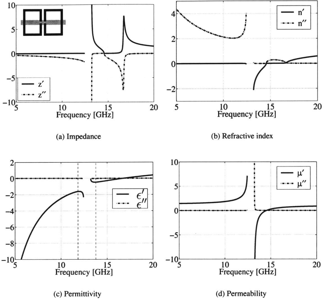
Figure 2-8: Retrieved z , n , \epsilon and \mu (real and imaginary parts) for a one-cell metamaterial structure taken from [82, 83] and shown in the inset of Fig. 2-8(a). The vertical dashed lines denote the limits of the resonance band.
