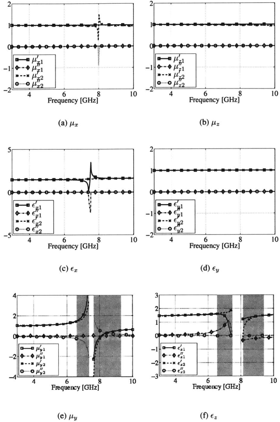
Figure 3-4: Retrieval results for a lossless edge-coupled SRR metamaterial whose unit cell is shown in Fig. 3-1(a), using a retrieval method not considering the bianisotropy. The retrieved \mu_x (Fig. 3-4(a)) and \epsilon_x (Fig. 3-4(c)) show negative imaginary parts around the resonance, which violates physical laws [84] and therefore indicates that the results are not reliable in the corresponding region. Those results difficult to read within the resonance band are not shown in Fig. 3-4(e) and Fig. 3-4(f). The shaded region indicates the frequency range where the mismatch of either \mu_y or \epsilon_z exceeds the threshold ( RM > 0.25 ).
