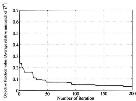
Figure 5-6: Trajectory of the optimized objective function value in the numerical model for the hypothetical spheroid.
