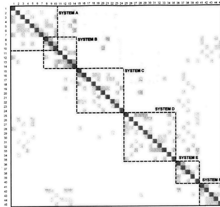
Figure 3-5: Clustering of a 45-variable DSM into 6 systems
