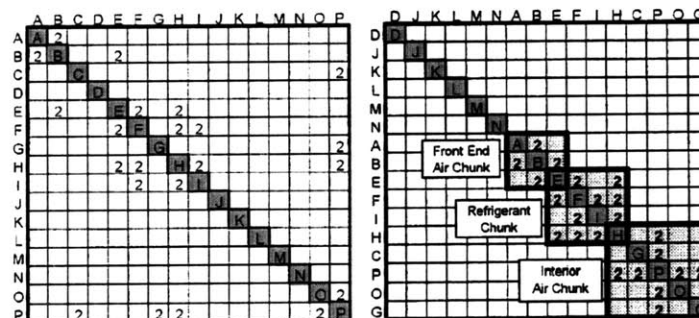
Figure 3-2: Original and clustered DSM (Browning 2001)
