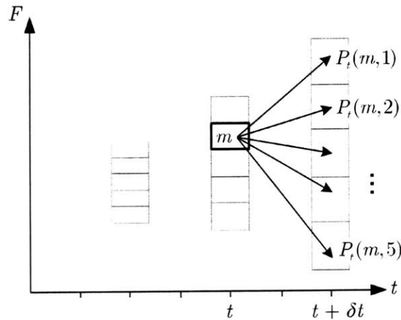
Figure 2-8: Bin definition and transition probabilities in SSAP algorithm
