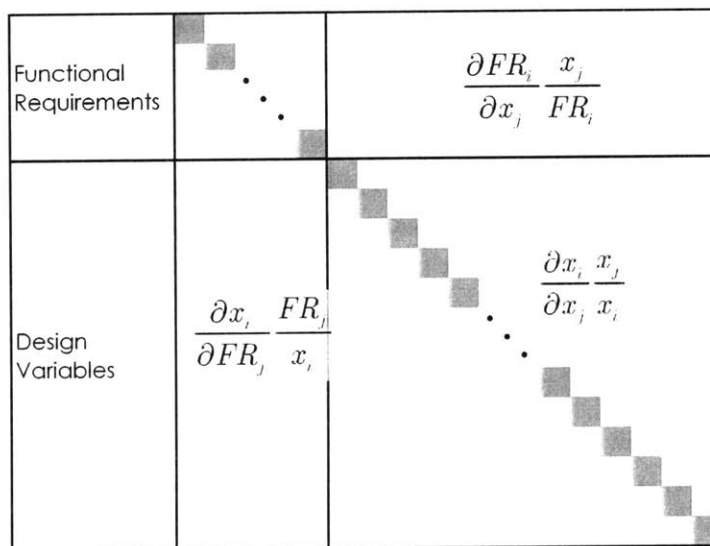
Figure 3-3: Normalized SDSM, extended to include exogenous functional requirements
