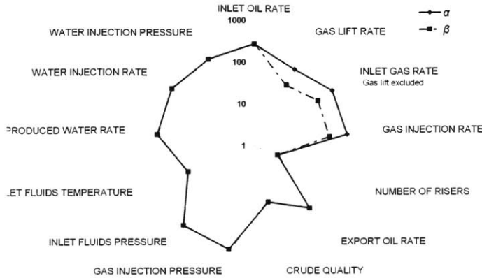
Figure 5-3: Comparison between assumed functional requirements of FPSOs \alpha and \beta
