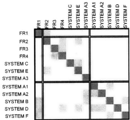
Figure 3-15: Re-partitioned SDSM, with platform that includes subsystem-level line items
