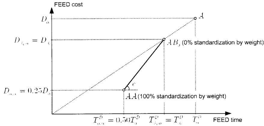
Figure 5-7: FEED cost and time as a function of standardization by weight
