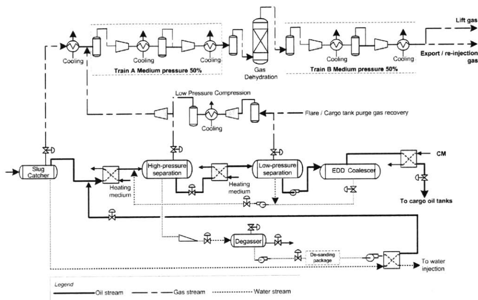
Figure 5-2: Main topsides facilities functions and equipment (simplified)
