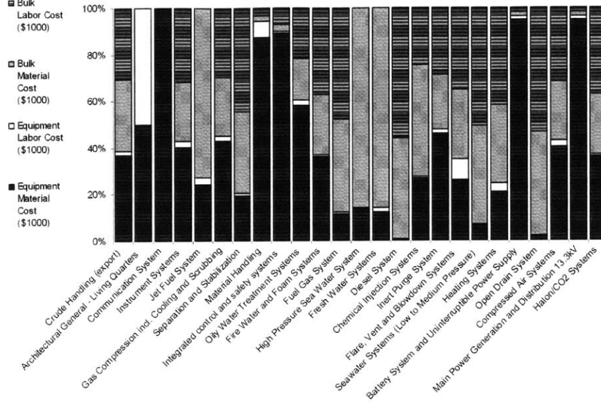
Figure 5-6: Assumed percent breakdown of development costs by system, FPSO \alpha
