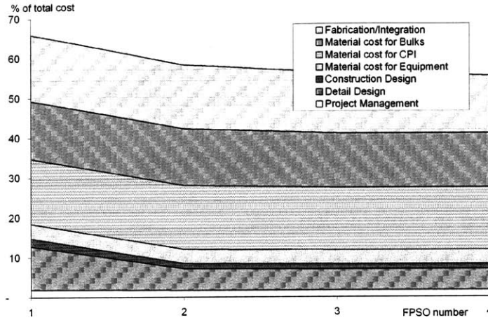
Figure 5-8: Assumed learning curves in FPSO construction costs
