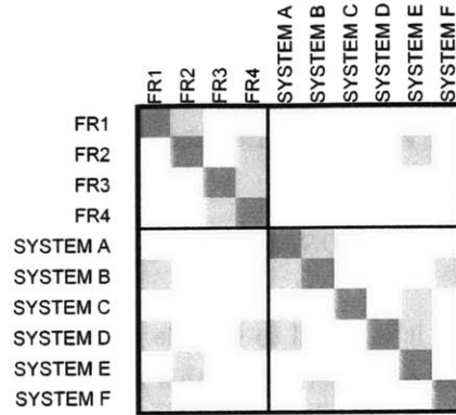
Figure 3-7: System-level DSM, extended to include functional requirements
