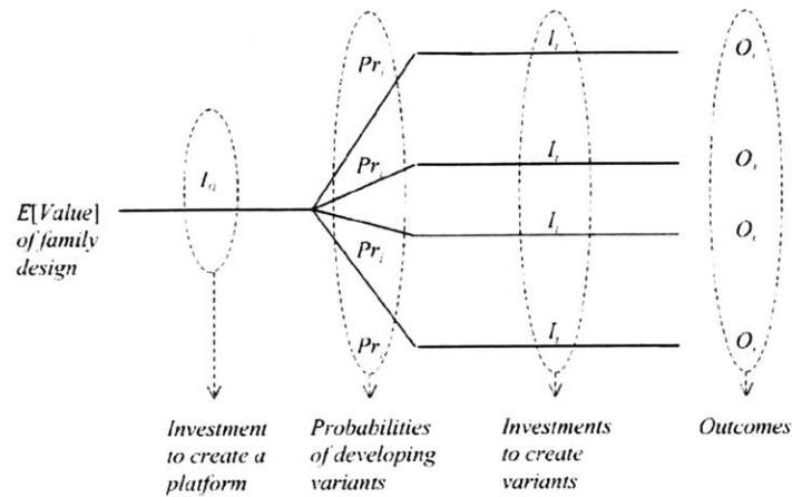
Figure 2-4: Two-step process for designing platform variants (Gonzalez-Zugasti et al. 2001)
