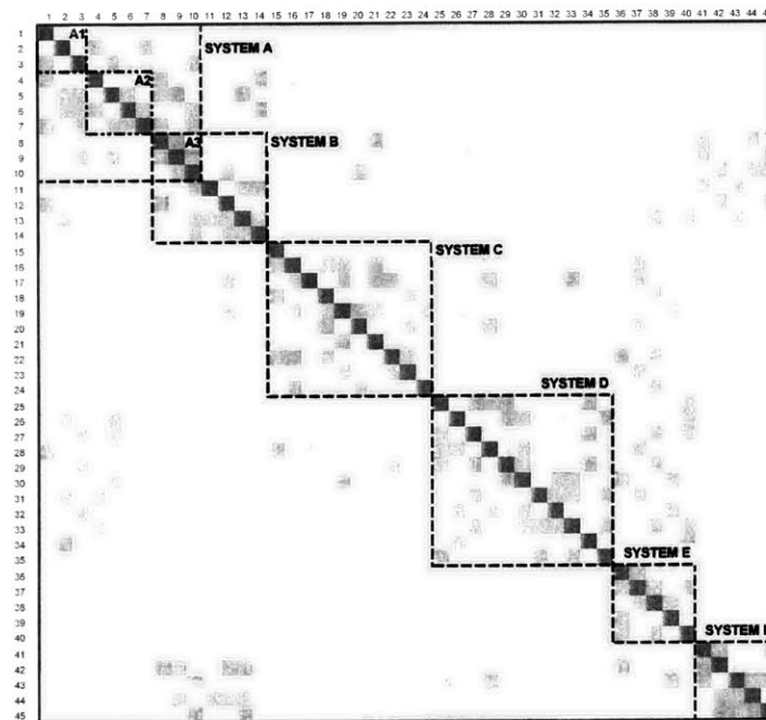
Figure 3-13: Decomposition of system A at the variable level
