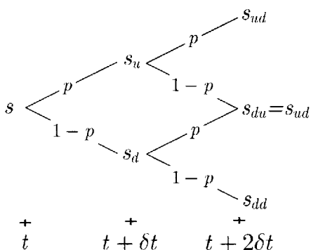
Figure 2-7: Two steps of a recombining binomial lattice of s
