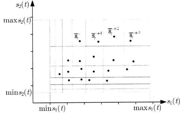
Figure 4-7: Two-dimensional bin definition and some representative values at time t
