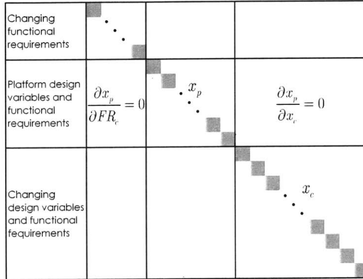
Figure 3-4: Invariant Design Rules on an S-DSM
