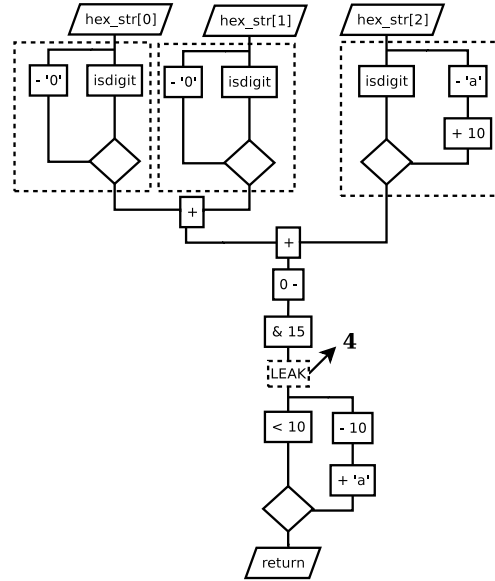
Figure 2: Preemptive leakage and enclosure of indirect flows. Here the hexadecimal checksum example of Figure 1 has been annotated to enclose computations that branch on secret data ( ENTER_ENCLOSURE and EXIT_ENCLOSURE in the code, dotted rectangles in the circuit), and to preemptively leak the value of the checksum while it is stored in binary ( LEAK code annotation and circuit operation). With these annotations, the amount of information leaked by the code is be precisely computed as 4 bits per execution.
