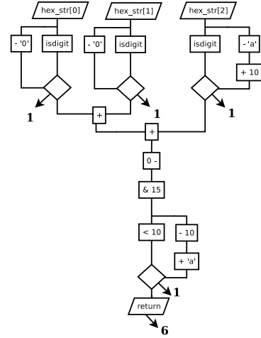
Figure 1: On the left, a C function to compute a checksum for data represented as a hexadecimal string. The output is a hex digit such that the sum of that digit and those in the input is a multiple of 16. On the right, a representation in the form of a circuit of the operations performed by an execution of the function. Data flows from inputs (top row parallelograms) through primitive computations (rectangles) to outputs (bottom row parallelograms). Values that depend on a control-flow branch are represented by diamonds, where the top input is the branch condition, the left or right inputs are the values when the condition is true and false, and the output is at the bottom. Diagonal arrows show the 10-bit information flow bound estimated by our tool when operating without annotations.
