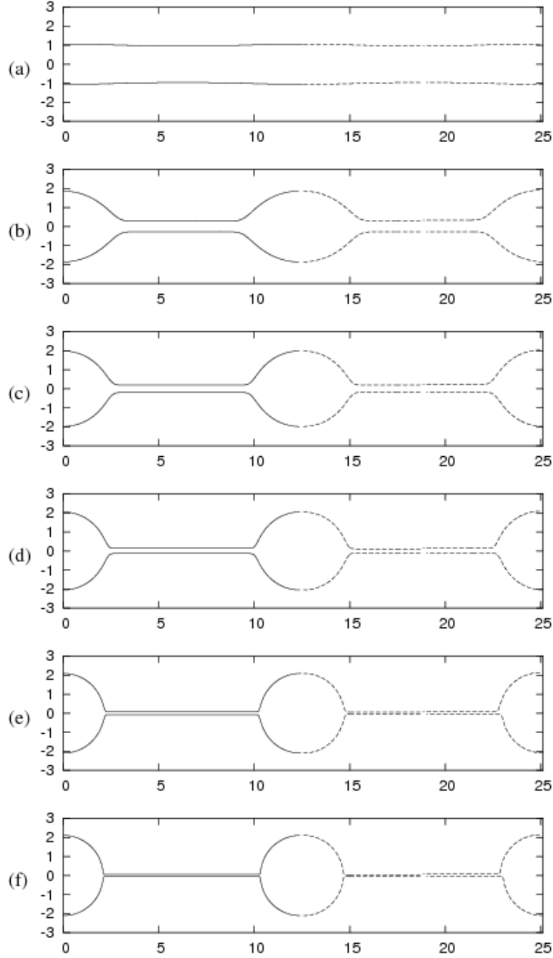
FIGURE 3. A typical series of profiles with periodic boundary conditions and period L = 4\pi . The dimensionless parameters are \nu_s = 0.79 , \nu_p = 2.37 , and De = 94.9 . A sinusoidal perturbation of amplitude 0.05 was added in order to make the filament collapse. After the rapid formation of the beads-on-string structure, one observes the slow thinning of the thread. The relative dimensionless times of each profile are (a) 0.0, (b) 31.6, (c) 158.1, (d) 316.2, (e) 632.5 and (f) 948.7. The left-hand-side of the graph (full lines) was produced using the explicit code, the right-hand-side using the implicit code with staggered grid.
