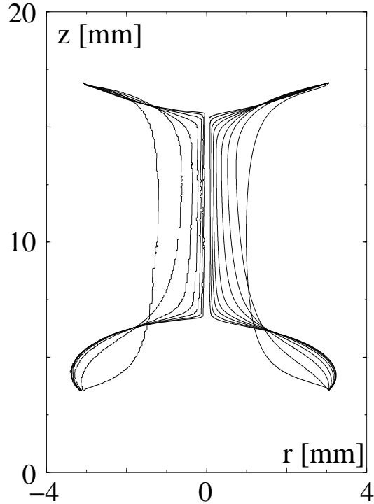
FIGURE 5. A comparison between experimental profiles (left), obtained from digitising the images of figure 1 and corresponding simulations (right), including the initial stretching and gravity (acting downward). The time difference between two consecutive images is 10 sec. The reduced variables corresponding to the experimental parameters are \nu_s = 193.2 , \nu_p = 29.04 , and De = 296 . Note that there are more profiles from simulation to reach approximately the same thread radius, corresponding to a slight overestimation of the experimental time scale.
