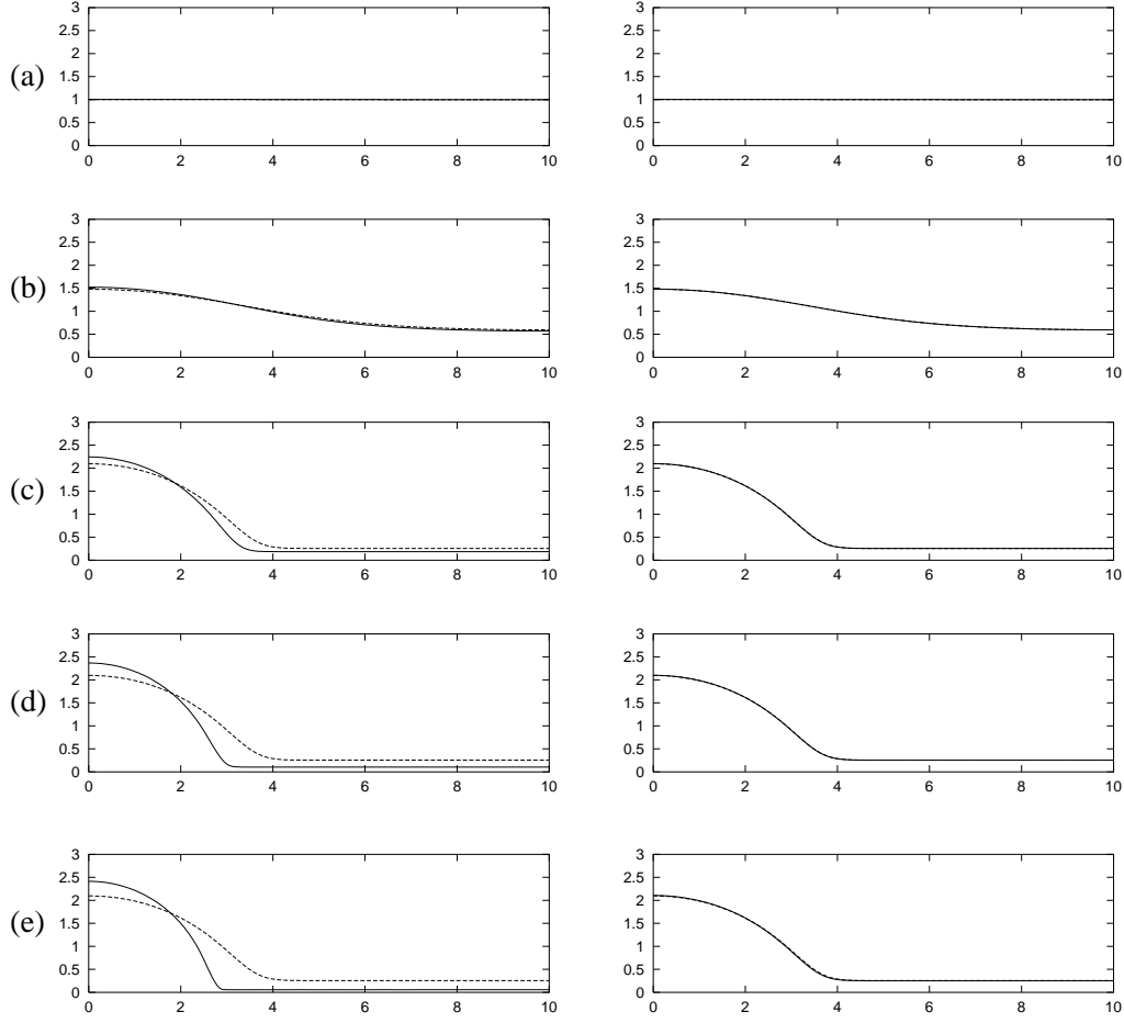
FIGURE 7. Comparison of interface profiles with period L = 20 and \nu_s = 0.79 between the full equations (full) and the local approximation (dashed lines): left column De = 94.9 and \nu_p = 2.37 , and right column De = 9490 and \nu_p = 237 . The relative times for each profile are (a) 31.6, (b) 79.1, (c) 158.1, (d) 316.2 and (e) 474.3. Evidently, for t \ll De the agreement is excellent (right column).
