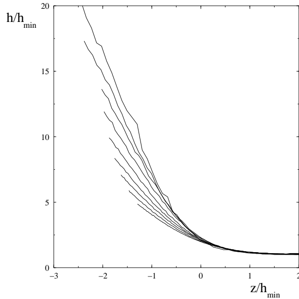
FIGURE 12. The last 9 experimental profiles (corresponding to figure 11), taken in time intervals of 0.5 sec, with both axes rescaled by the minimum thread radius.
