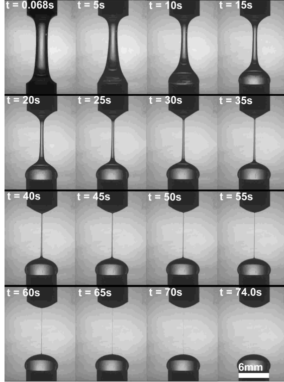
FIGURE 1. Experimental images of a collapsing liquid bridge of polymer solution in a viscous solvent (plate radius R_0 = 3 \text{ mm} , distance 13.8 \text{ mm} ). This state was obtained by rapidly stretching the liquid bridge from an initial gap of 3 \text{ mm} width, which was completely filled with fluid. The surface tension is \gamma = 37 \text{ mN/m} , the density \rho = 1026 \text{ kg/m}^3 . The solvent and polymeric contributions to the viscosity are \eta_s = 65.2 \text{ Pas} and \eta_p = 9.8 \text{ Pas} , respectively, the polymer timescale is \lambda = 8.1 \text{ s} . Relative to the capillary timescale \tau = \sqrt{\rho R_0^3 / \gamma} this results in a Deborah number of De = 296 .
