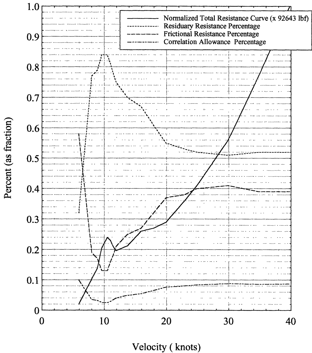
Figure 3-19: Model M-3 Resistance Components as a Percent of Total Resistance Based on Full Scale Results
