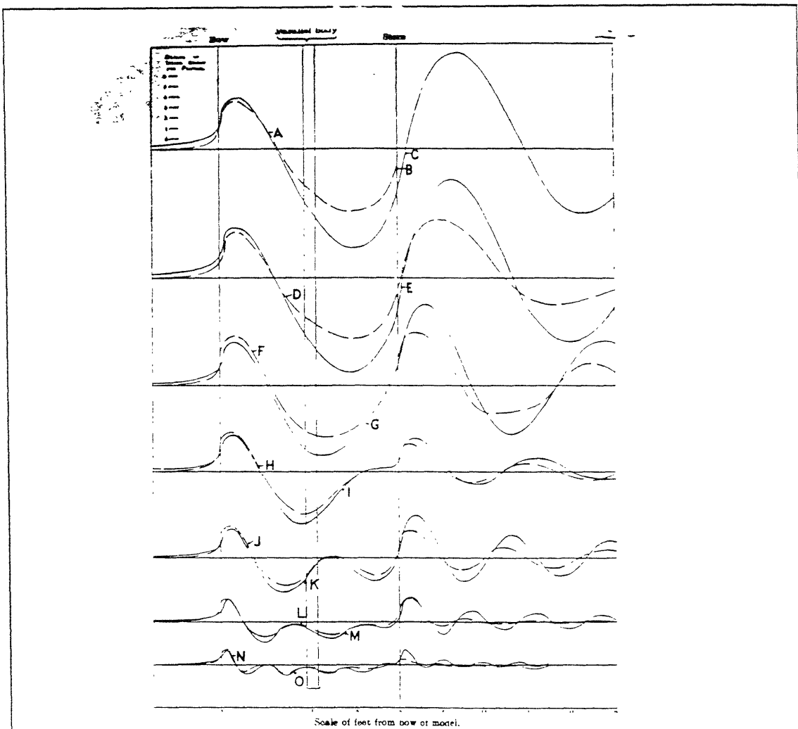
FIG. 2.—Model 1234. Comparison of calculated and observed wave-profiles.
