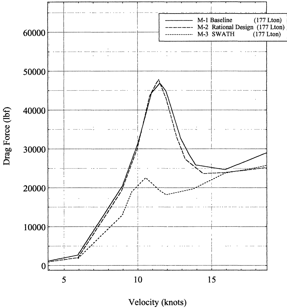
Figure 3-12: Models M-1/M-2 and M-3 Fixed in Pitch and Heave Full Scale Resistance Data
