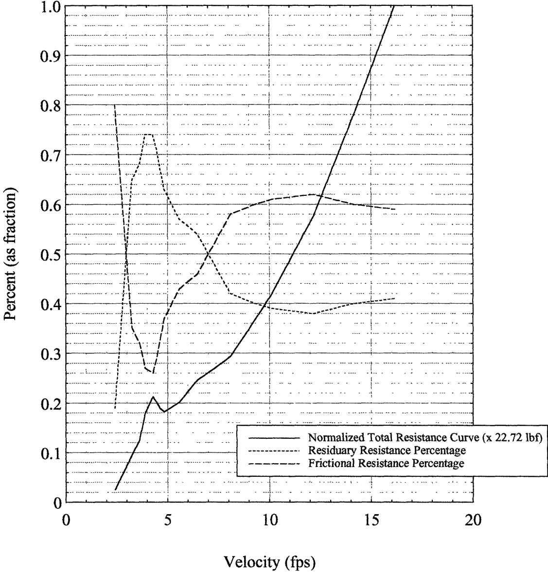
Figure 3-18: Model M-3 Resistance Components as a Percent of Total Resistance Derived from Unscaled Test Data
