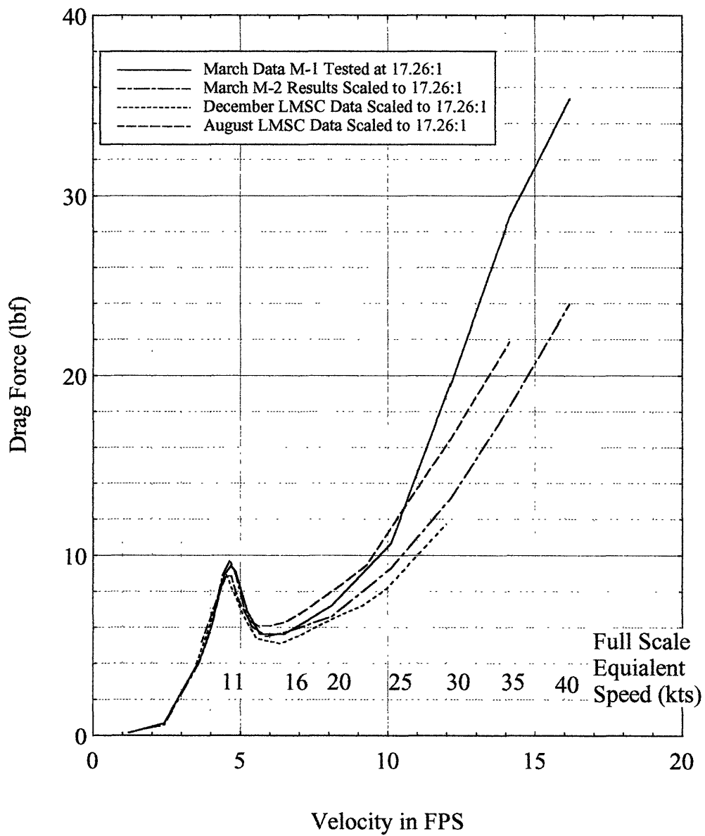
Figure 3-10: Models M-1 Performance Compared With LMSC Results Data Presented in 17.26:1 Scale
