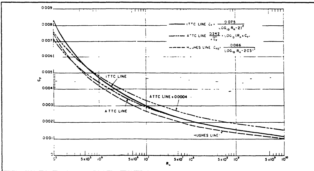
Figure 2-2: Standard Skin Friction Lines
