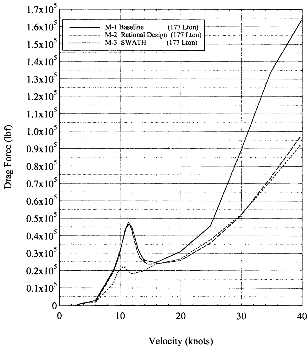
Figure 3-11: Models M-1/M-2 and M-3 Fixed in Pitch and Heave Full Scale Resistance Data
