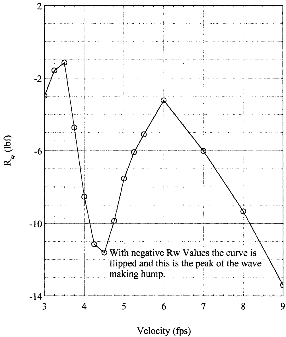
Figure 4-2: Wave Making Resistance of SLICE calculated from Thin Ship Theory
