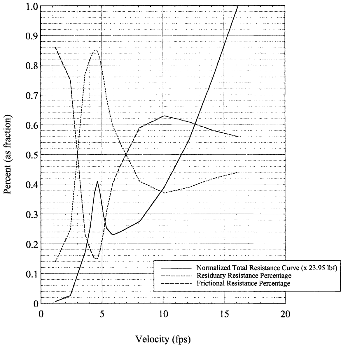
Figure 3-16: Model M-2 Resistance Components as a Percent of Total Resistance Derived from Unscaled Test Data
