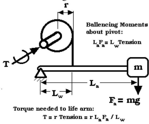
For a winch lifting an arm
