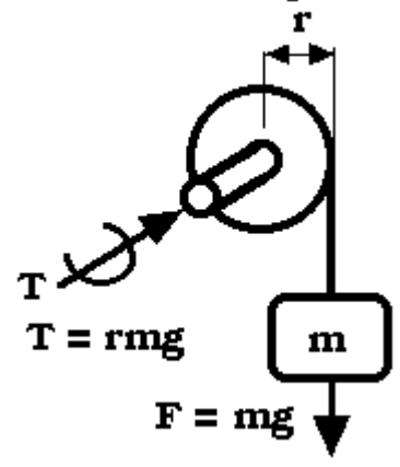
For a winch lifting a mass
