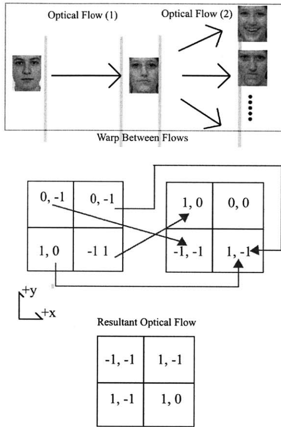
Figure 3-1: Visualization of Optical Flow Warp.
