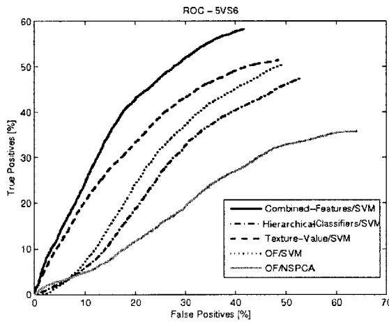
Figure 4-1: ROC curve for 5VS6.
