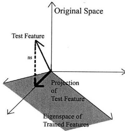
Figure 3-3: Visualization of the Projection and Resultant Distance Metric.
