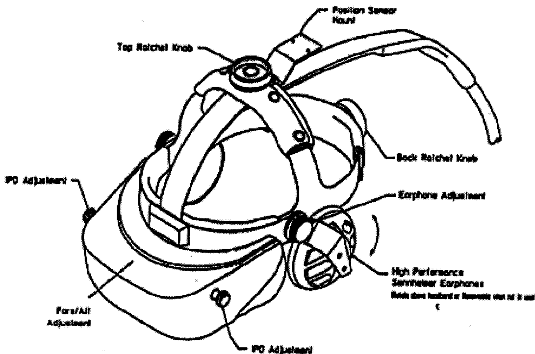
Figure 3.13 VR4 head-mounted display [Vir94].
