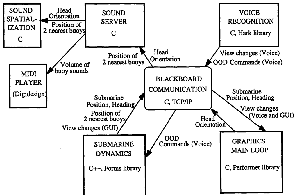
Figure 3.2 Software architecture for the OOD simulation.
