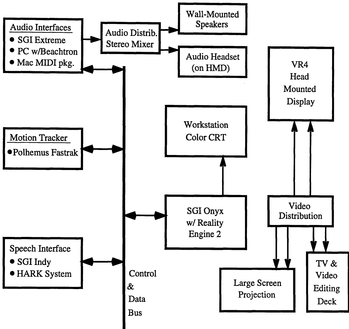
Figure 3.1 Hardware configuration for the OOD simulation. Figure adapted from VETT architecture slide by Walter Aviles.
