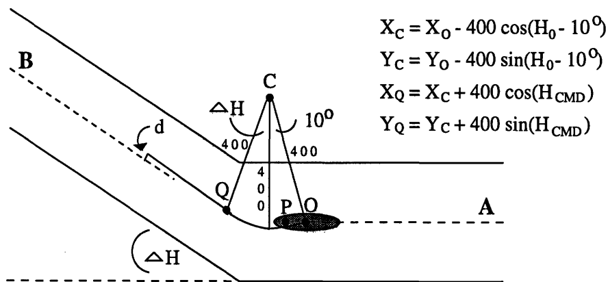
Figure 4.3 Simplified geometric modeling of a submarine turn.
