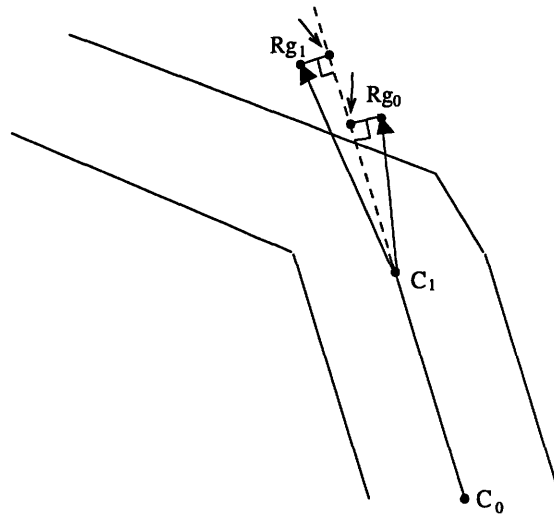
Figure 4.2 Verification of range marker locations. Erroneous locations Rg_0 and Rg_1 must be moved to the vector projection of vectors \overline{C_1Rg_0} and \overline{C_1Rg_1} into the extended centerline.
