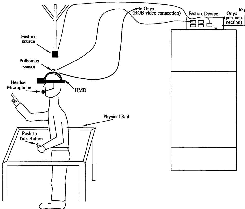
Figure 3.14 Polhemus Fastrak motion sensor. Figure also shows subject at physical rail station wearing HMD with microphone and push-to-talk button for voice commands.
