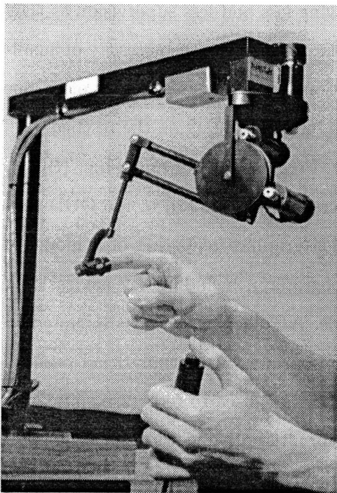
Figure 1.2a) PhanToM force-feedback device.
