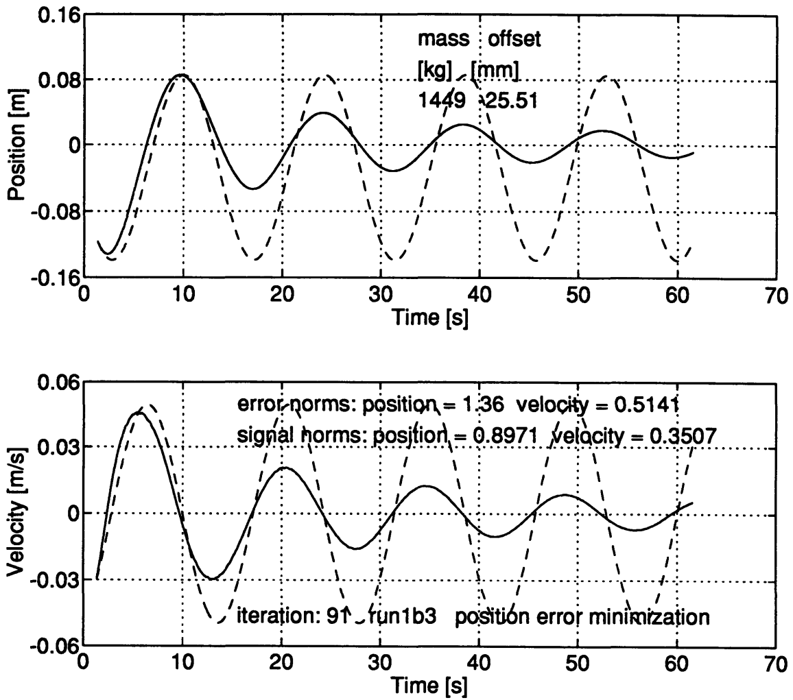
Figure A.26: NUMERICAL MINIMIZATION - INERTIA MODEL - RUN 1B3 - The vehicle trajectory is marked by the solid line. The dashed trace is the path followed by the model.
