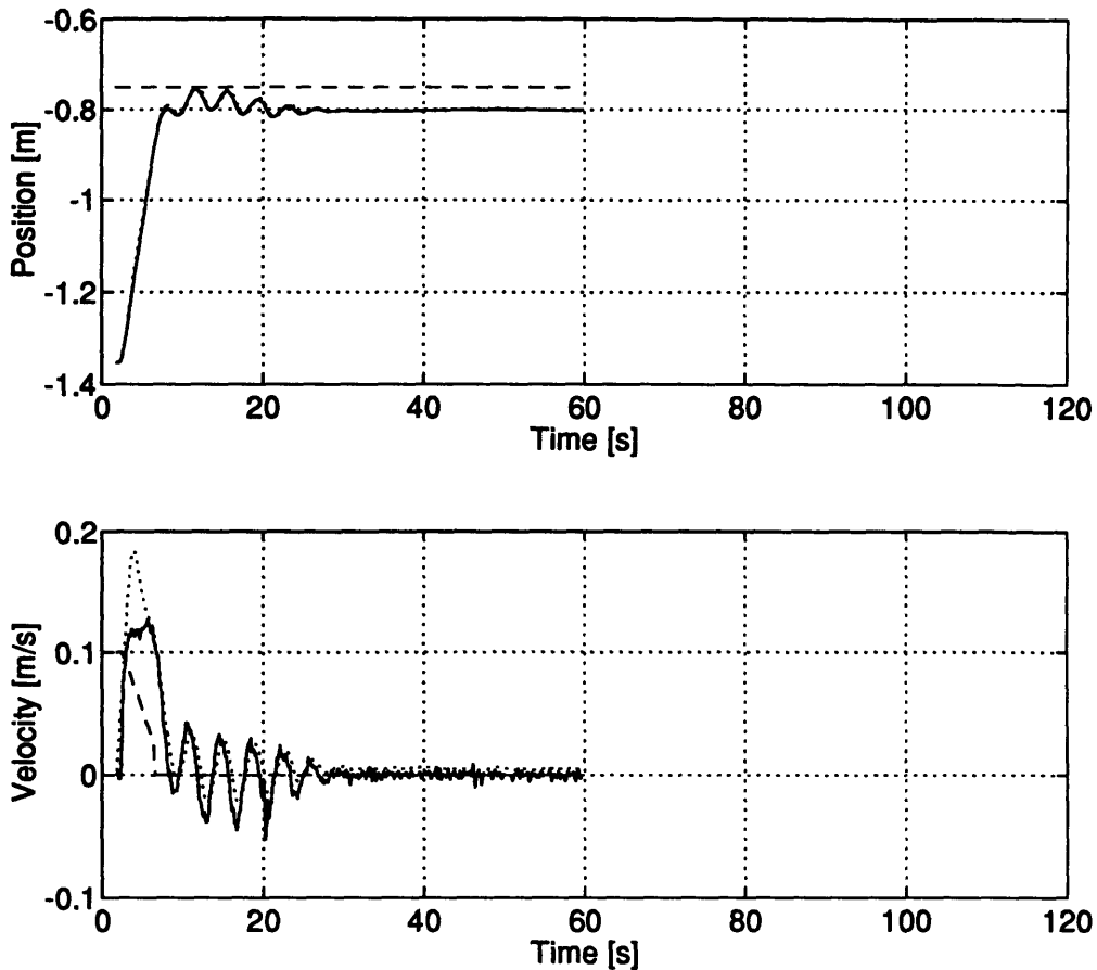
Figure 5.13: VEHICLE TRAJECTORY WITH DELAY, DEADBAND, AND SATURATION COMPENSATIONS AND THE OBSERVER FORCE INPUT ENABLED - The solid lines indicate the SHARPS position and its filtered derivative. The dashed lines mark the desired trajectory of the vehicle and the dotted curves are the state estimates.
