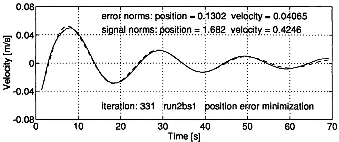
Figure A.34: NUMERICAL MINIMIZATION - INERTIA WITH QUADRATIC AND LINEAR DRAG MODEL - RUN 2BS1 - The vehicle trajectory is marked by the solid line. The dashed trace is the path followed by the model.
