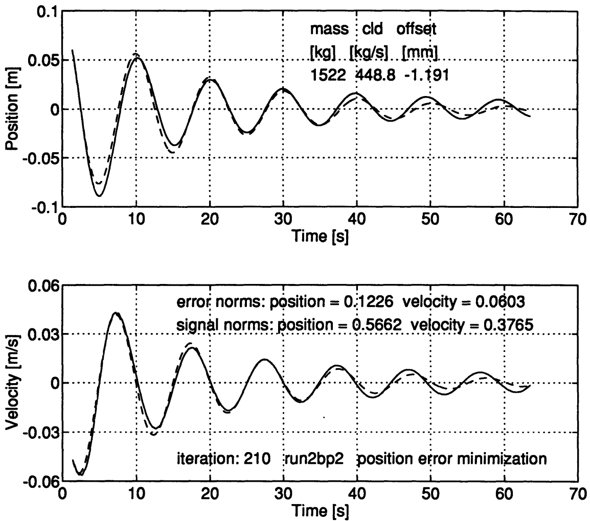
Figure A.7: NUMERICAL MINIMIZATION - INERTIA WITH LINEAR DRAG MODEL - RUN 2BP2 - The vehicle trajectory is marked by the solid line. The dashed trace is the path followed by the model.
