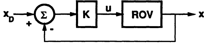
Figure 3.1: CLOSED LOOP TRAJECTORY FOLLOWING WITH FULL STATE FEEDBACK AND PD CONTROL
