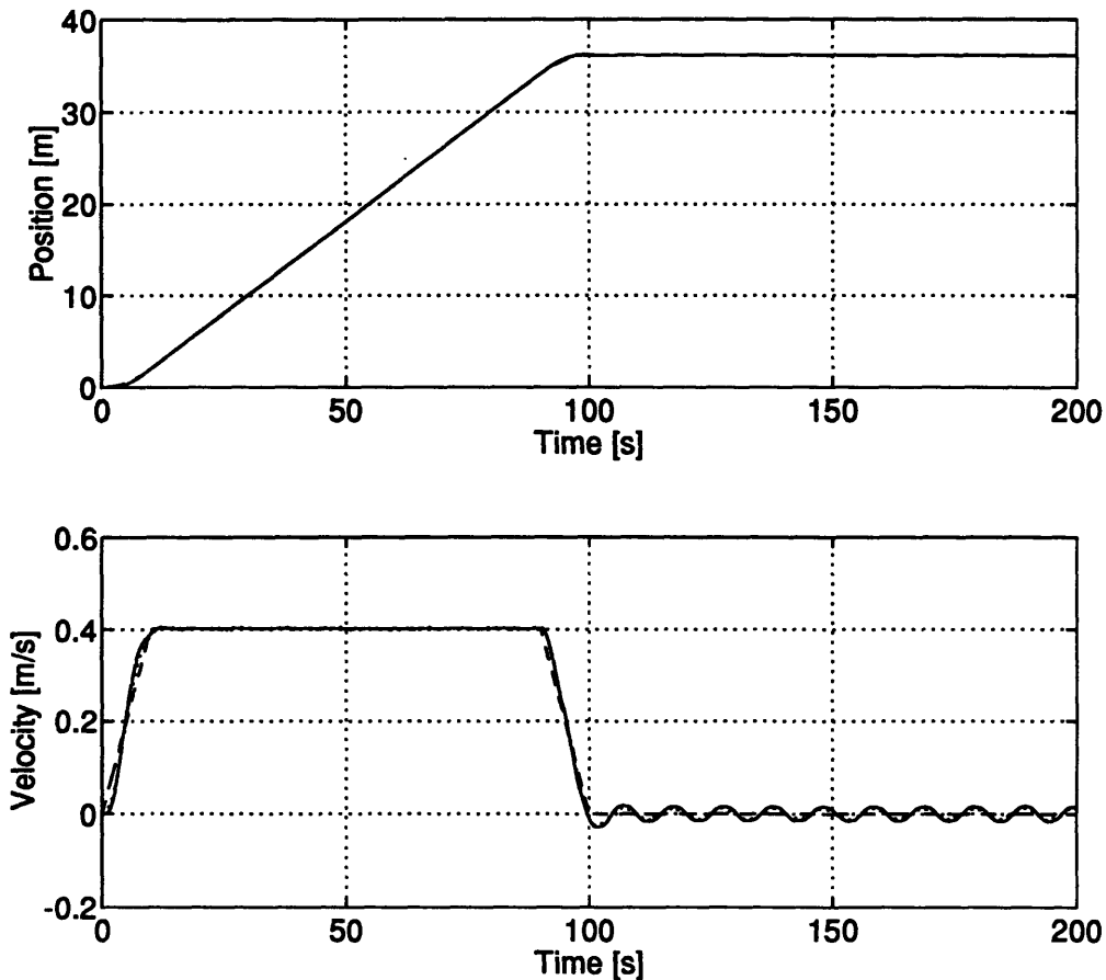
Figure 4.13: VEHICLE TRAJECTORY WITH THE COMPENSATION SUITE AND THE OBSERVER FORCE INPUT ENABLED - The solid lines mark the position and velocity of the simulated vehicle over time in response to the desired trajectory shown by the dashed lines. The state estimates are shown by the dotted lines. Even on this scale it is apparent that tracking errors have been reduced and state estimates have improved when compared to the previous configurations.
