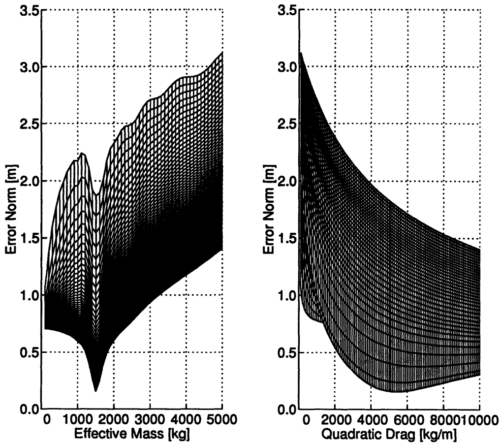
Figure 2.13: SIDE VIEWS OF THE ERROR NORM SURFACE - The global minimum identified by the simplex algorithm, m_{eff} = 1506 \text{ kg} and c_{qd} = 5431 \text{ kg/m} , is clearly visible.
