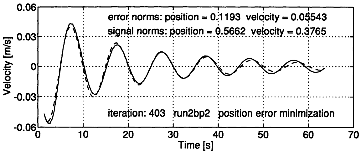
Figure A.9: NUMERICAL MINIMIZATION - INERTIA WITH QUADRATIC AND LINEAR DRAG MODEL - RUN 2BP2 - The vehicle trajectory is marked by the solid line. The dashed trace is the path followed by the model.
