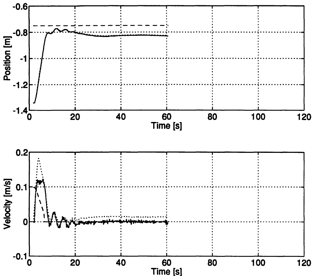
Figure 5.1: VEHICLE TRAJECTORY WITH DELAY AND DEADBAND COMPENSATIONS DISABLED AND SATURATION COMPENSATION AND THE OBSERVER FORCE INPUT ENABLED - The solid lines indicate the SHARPS position and its filtered derivative. The dashed lines mark the desired trajectory of the vehicle and the dotted curves are the state estimates. The constant position error and suppression of the limit cycle during hover are caused by the negative ballasting of the vehicle. The 5 cm/s error in the velocity estimate during the short translation matches the error recorded in the simulation (Figure 4.4).
