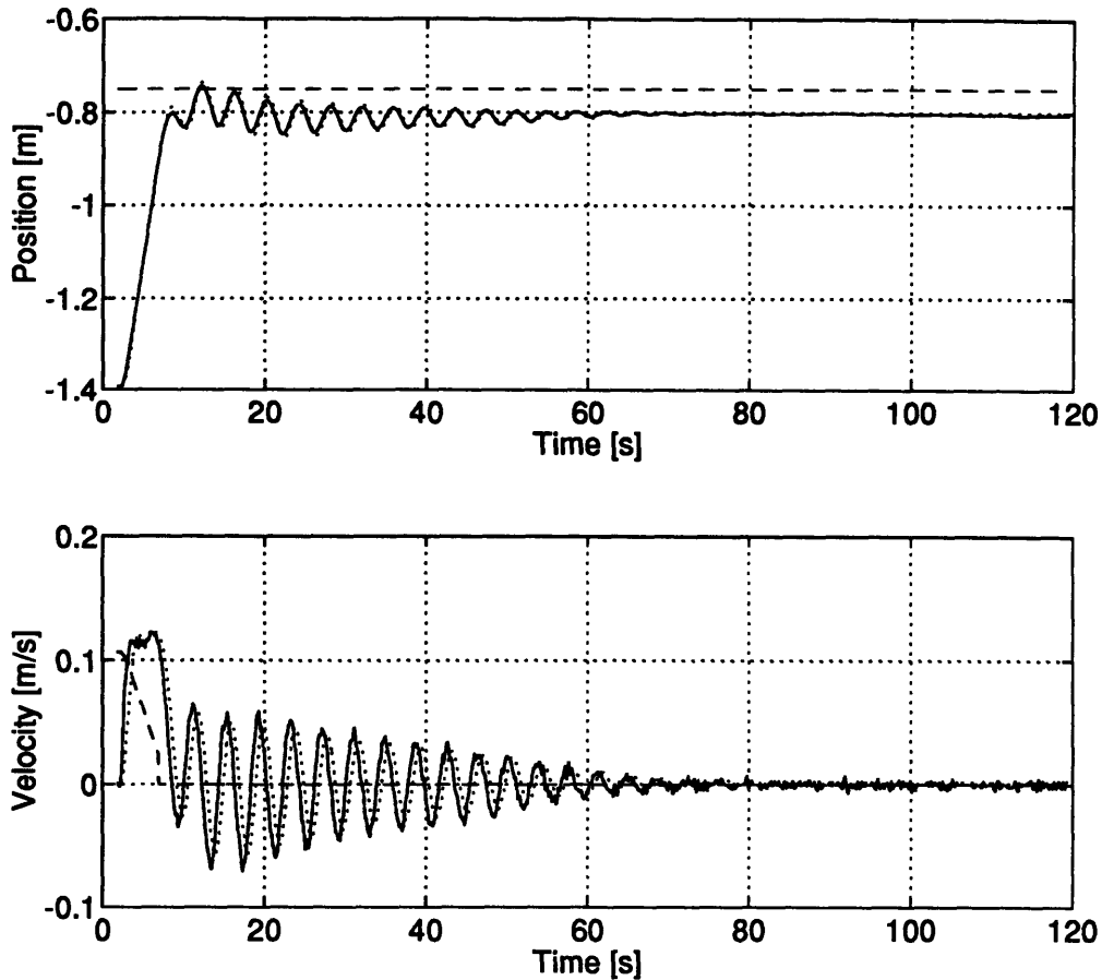
Figure 5.4: VEHICLE TRAJECTORY WITH SATURATION COMPENSATION ENABLED AND DELAY AND DEADBAND COMPENSATIONS AND THE OBSERVER FORCE INPUT DISABLED - The solid lines indicate the SHARPS position and its filtered derivative. The dashed lines mark the desired trajectory of the vehicle and the dotted curves are the state estimates.
