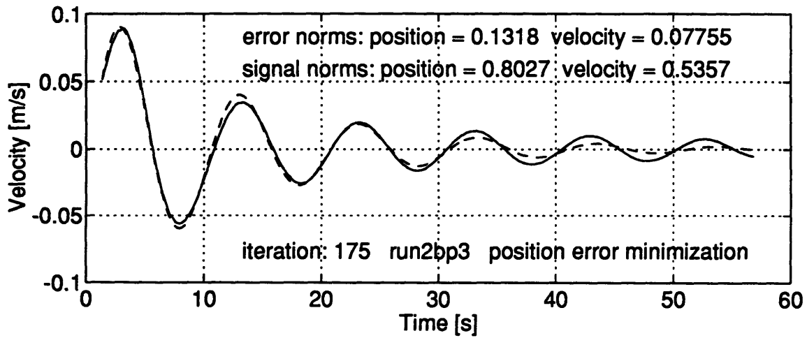
Figure A.12: NUMERICAL MINIMIZATION - INERTIA WITH LINEAR DRAG MODEL - RUN 2BP3 - The vehicle trajectory is marked by the solid line. The dashed trace is the path followed by the model.
