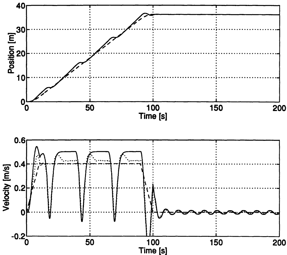
Figure 4.17: VEHICLE TRAJECTORY DUE TO AN INACCURATE HYDRODYNAMIC MODEL - The solid lines mark the position and velocity of the simulated vehicle over time in response to the desired trajectory shown by the dashed lines. The state estimates are shown by the dotted lines. The errors occur during translation when the drag coefficient of the vehicle is C_D^* = 1 while the vehicle controller quadratic drag compensation is calculated based on C_D^* = 8 . Error extrema are smaller and more frequent as the controller coefficient is reduced.
