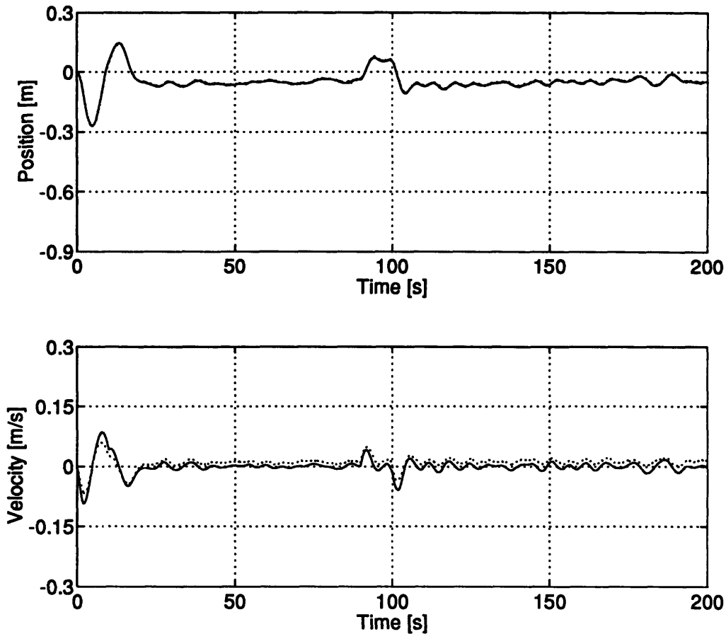
Figure 4.24: TRAJECTORY FOLLOWING ERROR IN THE PRESENCE OF ENVIRONMENTAL FORCING, COMPENSATED SYSTEM UNDER PID CONTROL, OBSERVER FORCE LOOP ENABLED, REAL CLOSED LOOP POLE AT -0.007 s^{-1} - The desired trajectory has been subtracted from the actual (solid lines), estimated (dotted lines), and measured (dash-dot, position plot only) trajectories and plotted here against time. The real valued closed loop pole has been placed at -0.007 s^{-1} to satisfy a quadratic performance index that emphasizes position tracking over actuator use. The ringing has been eliminated, but the steady tracking error has the same magnitude as the PD case.
