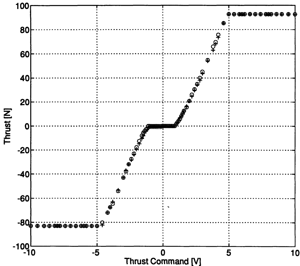
Figure 3.4: SINGLE THRUSTER STEADY STATE INPUT-OUTPUT RELATION - The response shown here is for a single thruster mounted in a test rig. \circ symbols mark the response as the input magnitude was increased away from zero. + symbols mark the response as the input magnitude was decreased towards zero.
