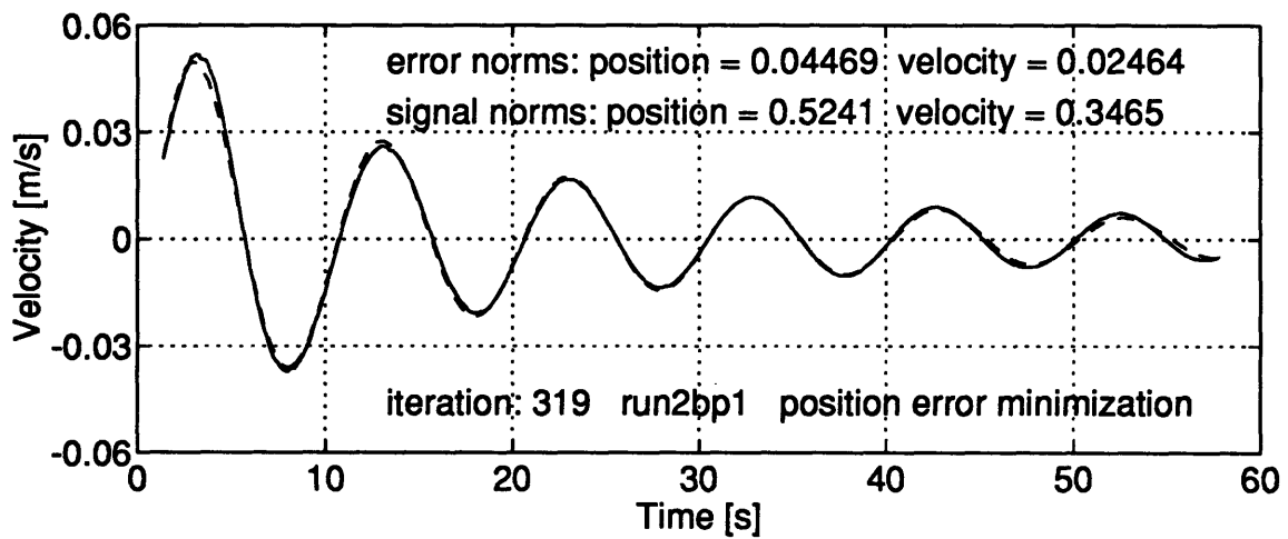
Figure A.4: NUMERICAL MINIMIZATION - INERTIA WITH QUADRATIC AND LINEAR DRAG MODEL - RUN 2BP1 - The vehicle trajectory is marked by the solid line. The dashed trace is the path followed by the model.
