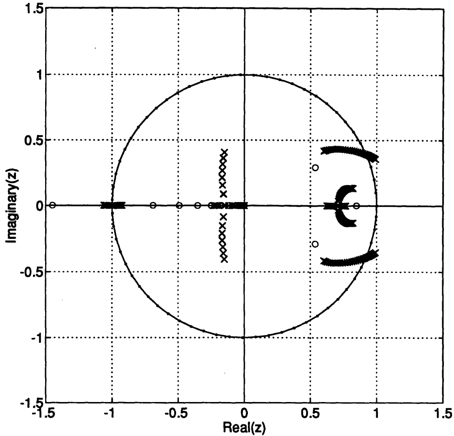
Figure 3.6: ROOT LOCUS STABILITY ANALYSIS - System poles are denoted by \times , system zeros are denoted by \circ . As the time delay is increased, the system poles migrate across the z -plane and eventually cross the unit circle, signalling the onset of instability. In the case shown the observer force input has been disconnected. Instability occurred when the delay reached approximately three full SHARPS periods. When the observer force input is used the delay reaches six or more full SHARPS periods before the onset of instability. The pole near -1 may be ignored.
