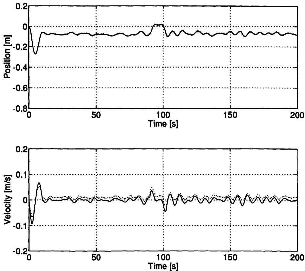
Figure 4.21: TRAJECTORY FOLLOWING ERROR IN THE PRESENCE OF ENVIRONMENTAL FORCING, COMPENSATION SUITE AND OBSERVER FORCE INPUT ENABLED - The desired trajectory has been subtracted from the actual (solid lines), estimated (dotted lines), and measured (dash-dot, position plot only) trajectories and plotted here against time. Note the change of scale on the vertical axes compared to the earlier trajectory following error plots. Note also the constant position offset and the suppression of the limit cycle. Movement about the mean offset is caused by the random component of the environmental forcing, not by the thruster dynamics.
