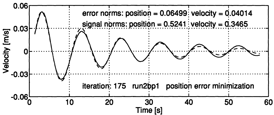
Figure A.2: NUMERICAL MINIMIZATION - INERTIA WITH LINEAR DRAG MODEL - RUN 2BP1 - The vehicle trajectory is marked by the solid line. The dashed trace is the path followed by the model.
