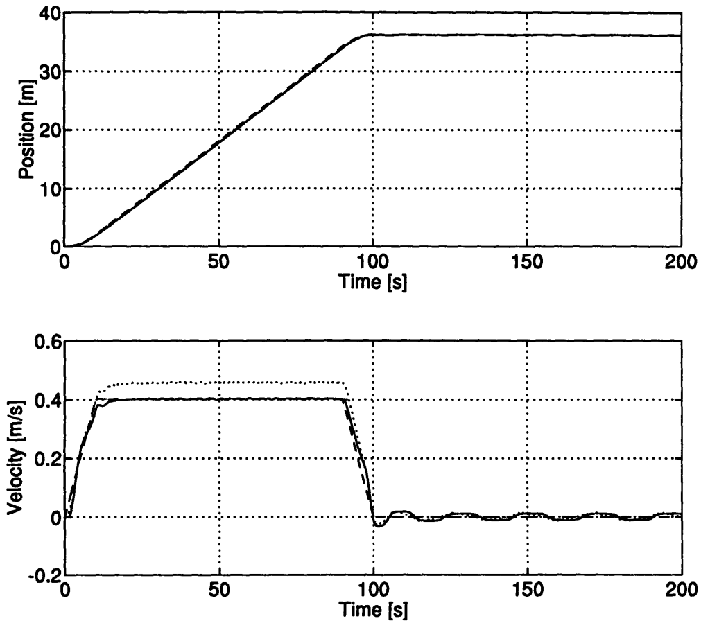
Figure 4.3: VEHICLE TRAJECTORY WITH COMPENSATION DISABLED AND THE OBSERVER FORCE INPUT ENABLED - The solid lines mark the position and velocity of the simulated vehicle over time in response to the desired trajectory shown by the dashed lines. The state estimates are shown by the dotted lines. Details of the position plot are obscured by the scale of the translation; small features can be seen more clearly in the trajectory error plot below (Figure 4.4). The limit cycle behavior caused by the thruster dynamics during hover is visible in the velocity plot.
