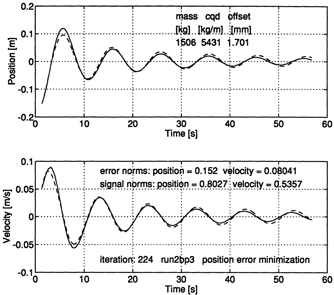
Figure A.13: NUMERICAL MINIMIZATION - INERTIA WITH QUADRATIC DRAG MODEL - RUN 2BP3 - The vehicle trajectory is marked by the solid line. The dashed trace is the path followed by the model.
