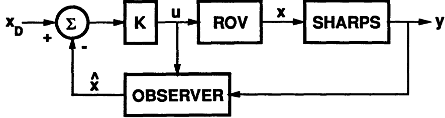
Figure 3.2: CLOSING THE CONTROL LOOP WITH A STATE ESTIMATOR
