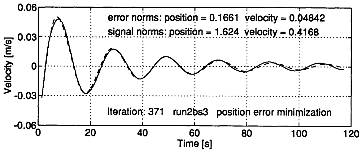
Figure A.44: NUMERICAL MINIMIZATION - INERTIA WITH QUADRATIC AND LINEAR DRAG MODEL - RUN 2BS3 - The vehicle trajectory is marked by the solid line. The dashed trace is the path followed by the model.
