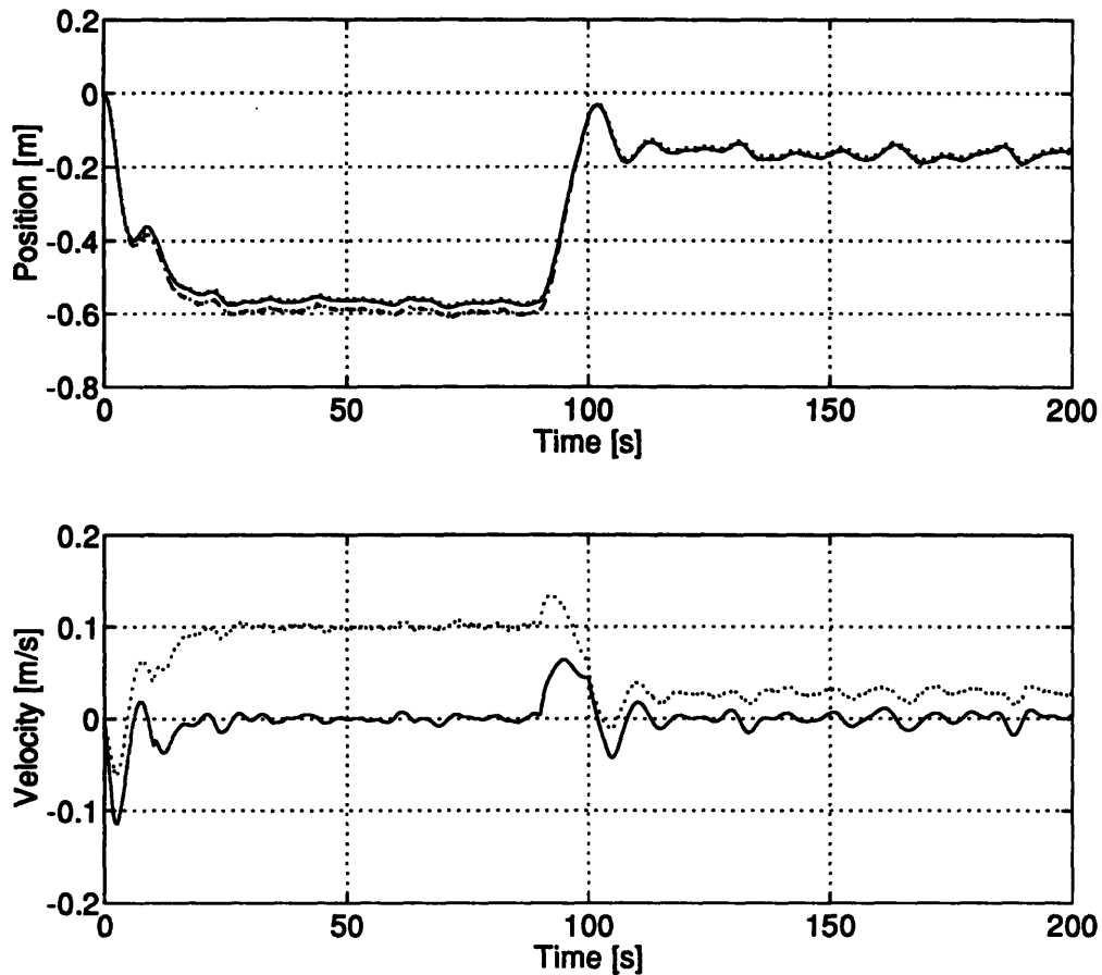
Figure 4.22: TRAJECTORY FOLLOWING ERROR IN THE PRESENCE OF ENVIRONMENTAL FORCING, COMPENSATION DISABLED AND OBSERVER FORCE INPUT ENABLED - The desired trajectory has been subtracted from the actual (solid lines), estimated (dotted lines), and measured (dash-dot, position plot only) trajectories and plotted here against time. Note the change of scale on the vertical axes compared to the earlier trajectory following error plots. Controller gains were calculated assuming steady translation values for the hydrodynamic coefficients, C_M^* = 1 , C_D^* = 1 . The position error is 55 cm during translation and 15 cm during hover. The position errors drop to 35 cm during translation and 10 cm during hover when the limit cycle values of the hydrodynamic coefficients ( C_M^* = 2 , C_D^* = 8 ) are used to compute the controller gains. Compare these values to the 5 cm offsets observed in the compensated case. The tracking errors can be reduced, but not eliminated, using PID control. Movement about the mean offset is caused by the random component of the environmental forcing, not by the thruster dynamics.
