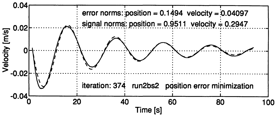
Figure A.39: NUMERICAL MINIMIZATION - INERTIA WITH QUADRATIC AND LINEAR DRAG MODEL - RUN 2BS2 - The vehicle trajectory is marked by the solid line. The dashed trace is the path followed by the model.
