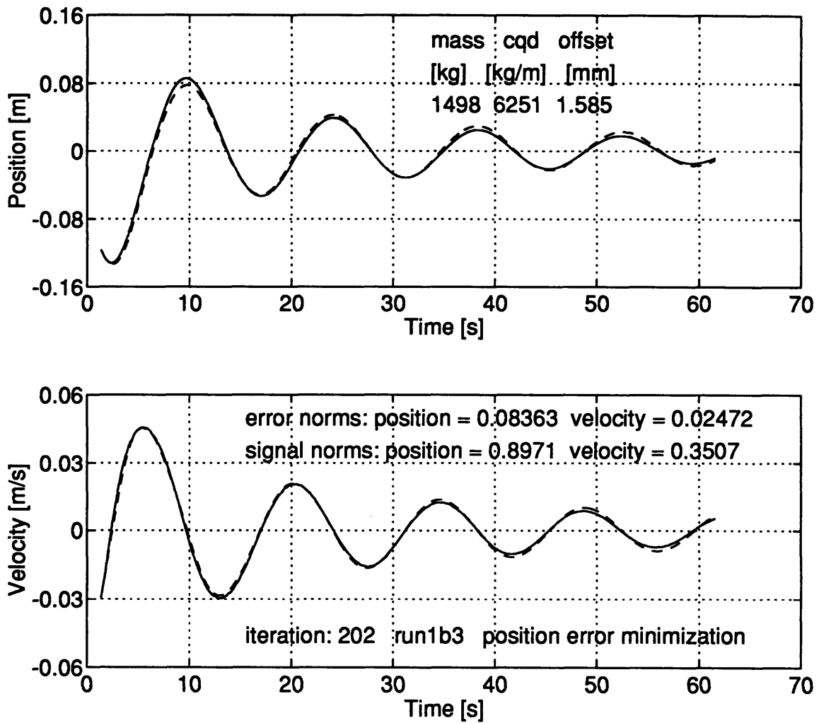
Figure A.28: NUMERICAL MINIMIZATION - INERTIA WITH QUADRATIC DRAG MODEL - RUN 1B3 - The vehicle trajectory is marked by the solid line. The dashed trace is the path followed by the model.
