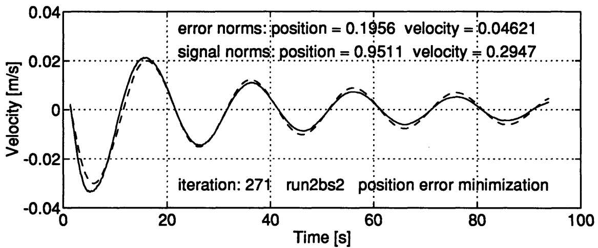
Figure A.38: NUMERICAL MINIMIZATION - INERTIA WITH QUADRATIC DRAG MODEL - RUN 2BS2 - The vehicle trajectory is marked by the solid line. The dashed trace is the path followed by the model.
