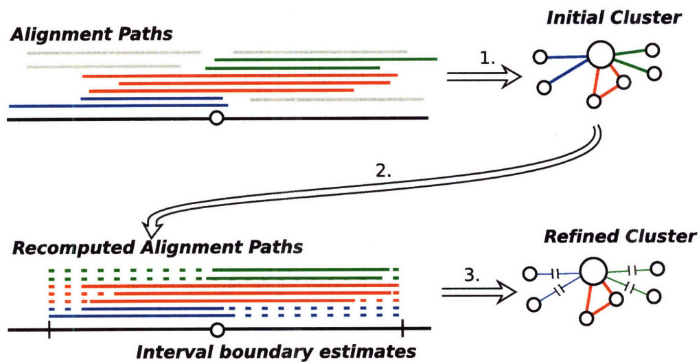
Figure 8-2: Cluster refinement using path re-estimation. 1. Alignment paths are used to generate an initial clustering as described in the original word acquisition algorithm. 2. Interval end-points for each node are estimated based upon the alignment paths present in the current cluster. These new end-points are used to re-calculate alignment path distortions. 3. The new distortions are used to re-cluster the original graph.
