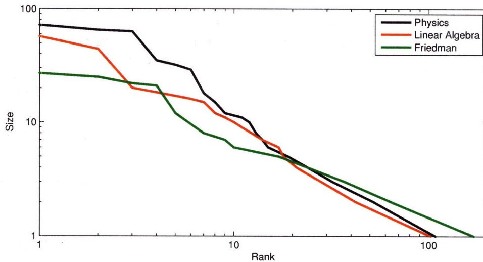
Figure 5-6: Log-log plot of cluster size versus size rank for the Physics, Algebra, and Friedman lectures.
