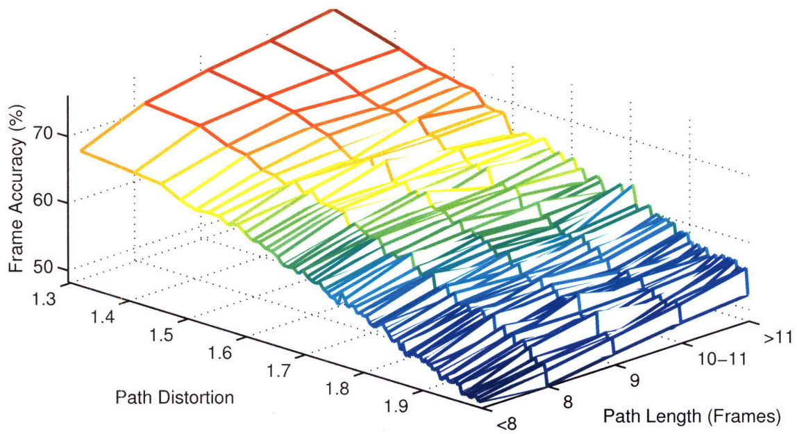
Figure 4-3: Phone accuracy in terms of percentage of frames correctly matched versus path distortion and path length.
