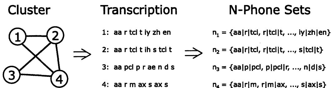
Figure 6-2: Conversion of cluster nodes into groups of n-phones. The intervals under the nodes are phonetically transcribed, then separated into sets of n-phone sequences. In this example, n = 3 .
