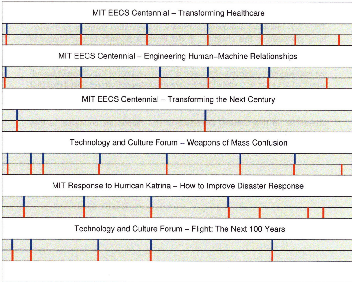
Figure 7-10: Comparison of human generated segmentation with automatic segmentation for the 6 lectures used in this chapter. For each lecture, the reference boundaries are shown as blue lines in the upper panel, and the automatically generated boundaries are shown as red lines in the lower panel.
