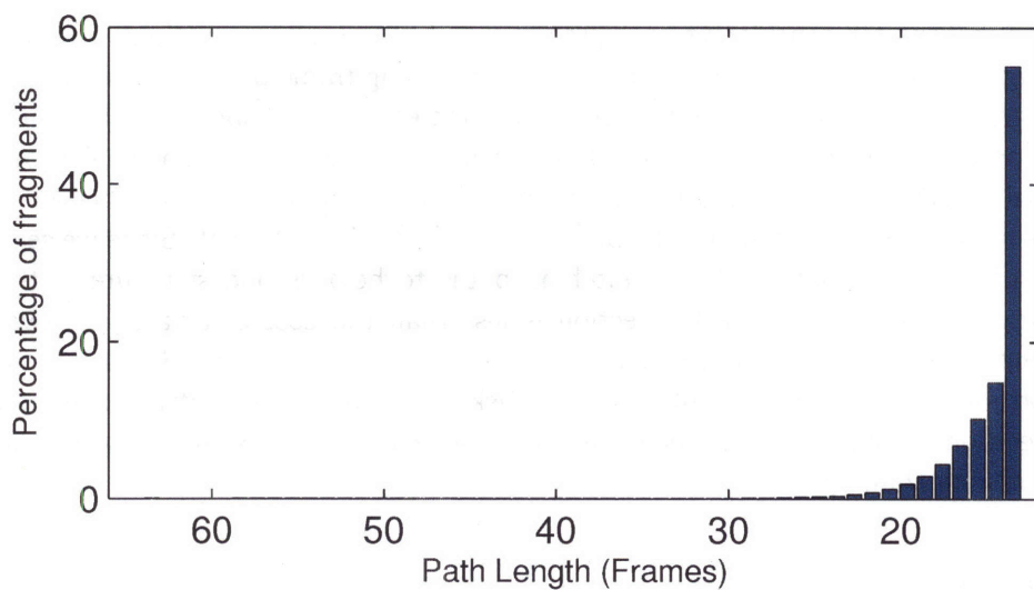
Figure 4-1: Histograms showing the distribution of the 921K path fragments according to average path distortion and path length. The distortion threshold of 2 was used to prune the generated fragments and is therefore the upper limit for fragments in the distortio histogram.
