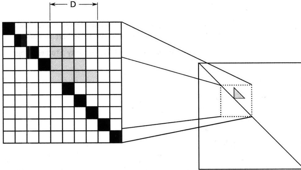
Figure 7-3: The diagonal region used to compute the segmentation profile. In this example, D = 4 .
