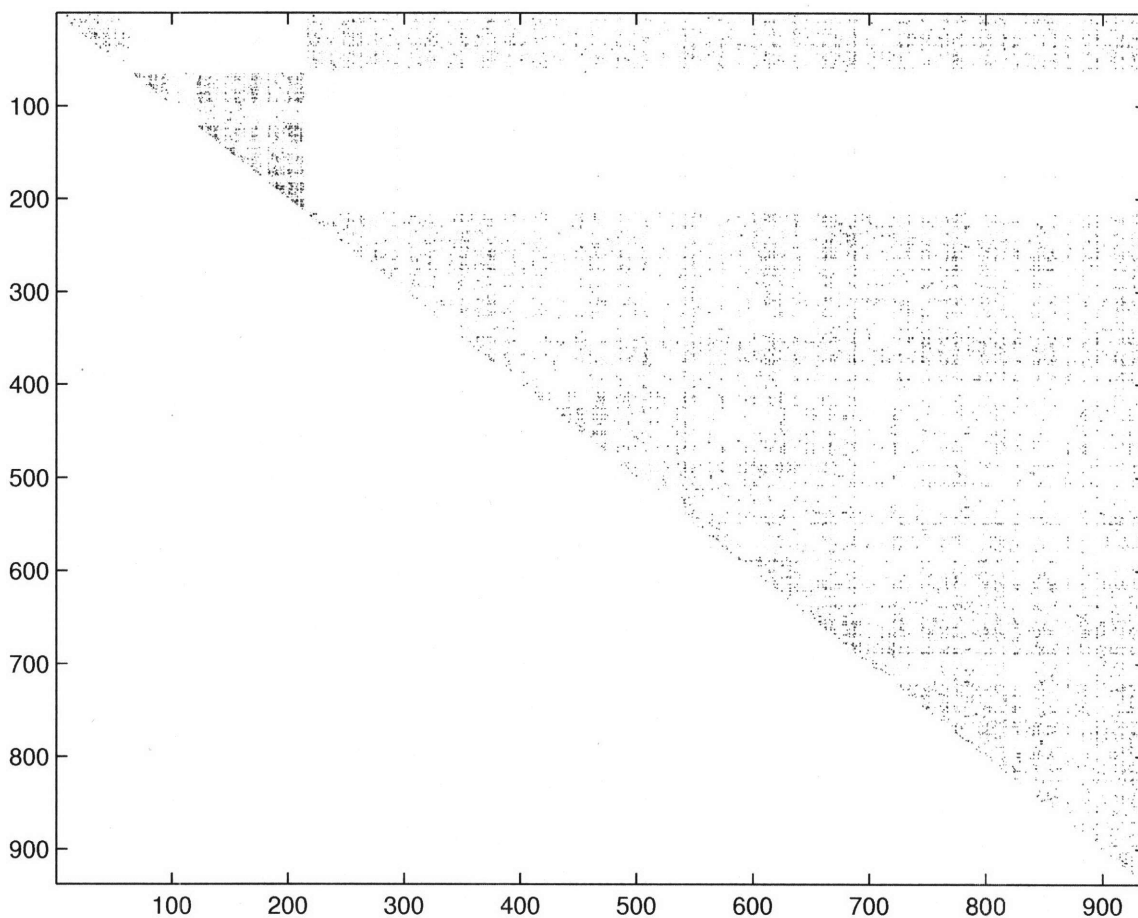
Figure 7-1: Utterance level similarity matrix for a physics lecture consisting of two main speakers and three main segments. The intensity of a cell (i, j) indicates the similarity of utterance i and utterance j using the minimum distortion alignment path fragment computed by the segmental DTW algorithm. Darker cells indicate higher similarity.
