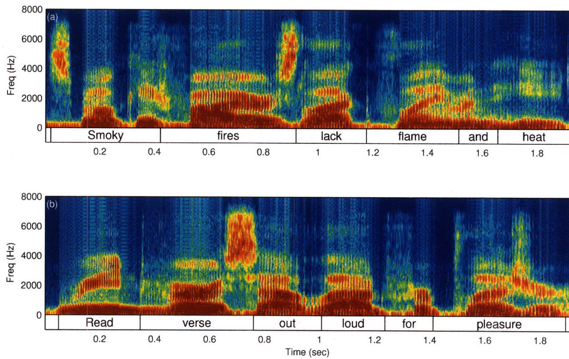
Figure 2-1: Two example ICC sentences with time aligned orthographies.
