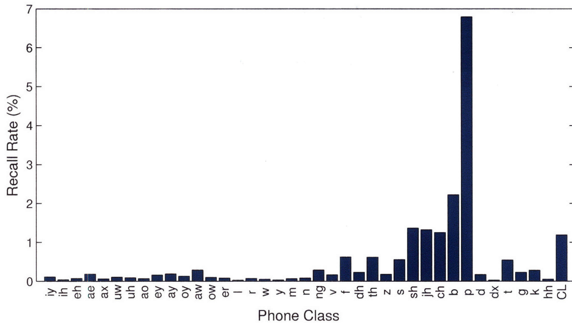
Figure 4-4: Frame level recall rates for each phone class.
