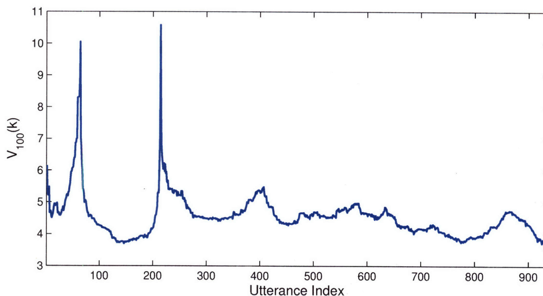
Figure 7-2: The log dissimilarity profile for the physics lecture from Figure 7-1. The width of the diagonal band considered is D = 100 utterances.
