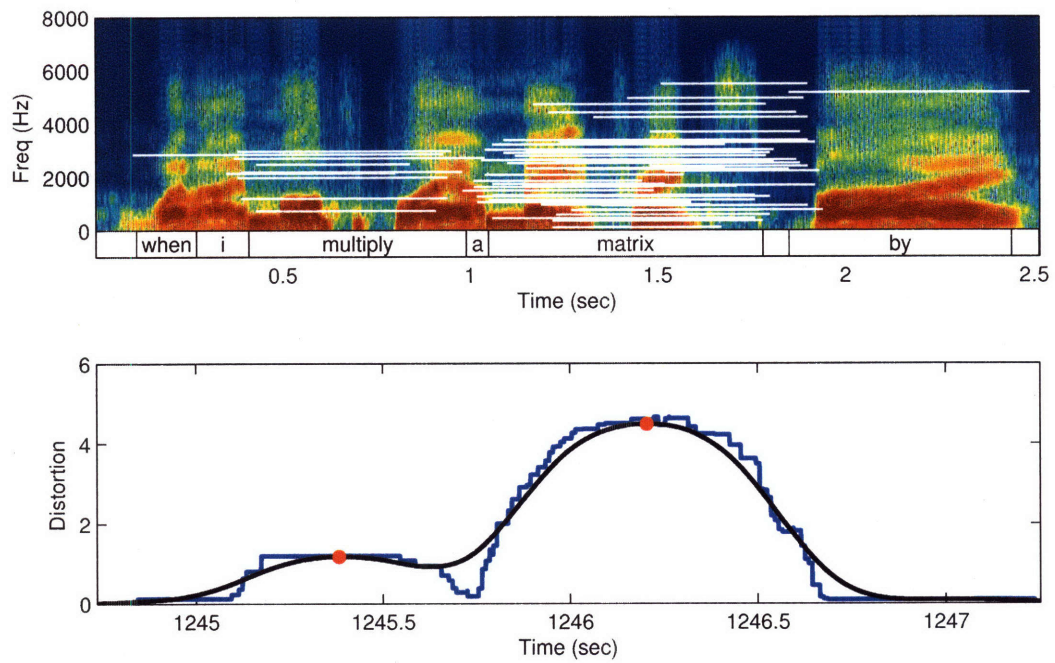
Figure 5-4: Top - An utterance from the Algebra lecture with the time regions from its associated path fragments shown in white. Paths are ordered from bottom to top in increasing order of distortion. Bottom - Similarity profile is shown in blue with the smoothed version shown in black. The extracted time index is shown as a red dot.
