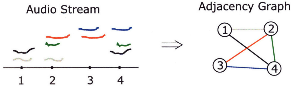
Figure 5-2: Production of an adjacency graph from alignment paths and extracted nodes. The audio stream is shown as a timeline, while the alignment paths are shown as pairs of colored lines at the same height above the timeline. Node relations are captured by the graph on the right, with edge weights given by the path similarities.
