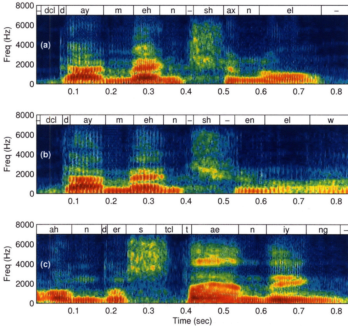
Figure 3-1: Spectrograms for three isolated word utterances spoken in a conversational context. The first two utterances are of the word “dimensional”. The third utterance is of the word “understanding”.
