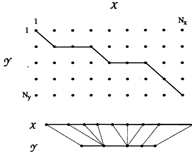
Figure 3-2: An example warp path aligning sequences \mathcal{X} and \mathcal{Y} of lengths N_x and N_y , respectively. The warp path \phi in this case is the sequence of ordered pairs: (1,1) (2,2) (3,2) (4,2) (5,3) (6,3) (7,3) (8,4) (9,5). The alignment corresponding to the warp path is displayed in the lower part of the figure.
