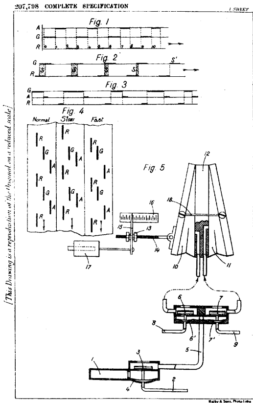
Fig. 1.4: The 1924 Pleyel patent for synchronizing multiple player pianos.
