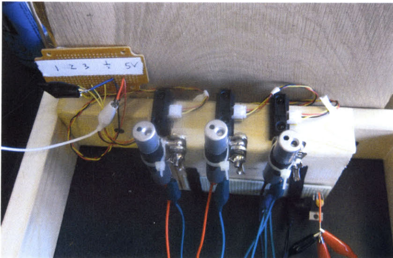
Fig. 5.5: Lasers, IR sensors, and power supply.
