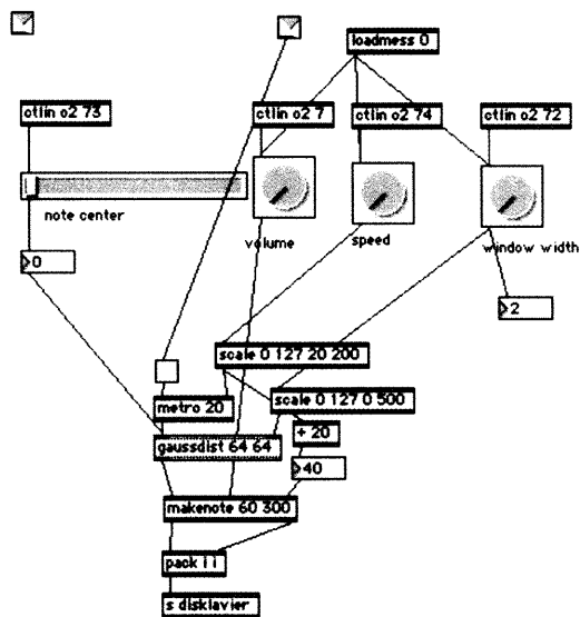
Fig. 3.10: Knob-blob patch
