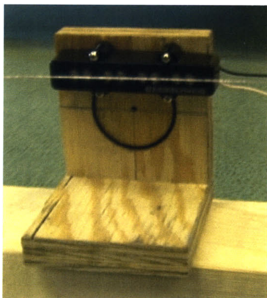
Fig. 4.12: The mounted pickup of the electromonochord.
