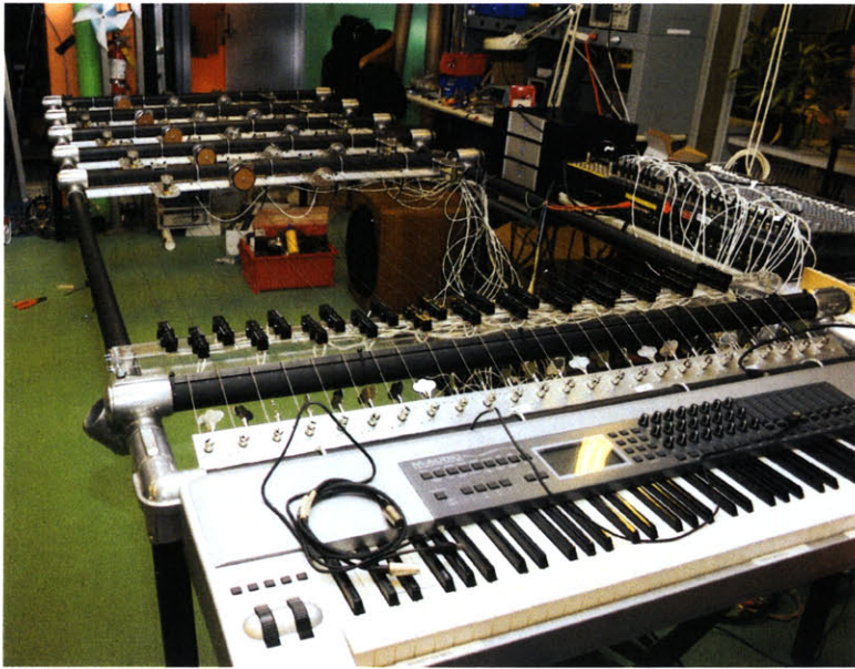
Fig. 4.17: The Chandelier prototype, with keyboard controller.
