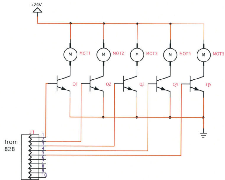
Fig. 4.26: Control electronics schematic
