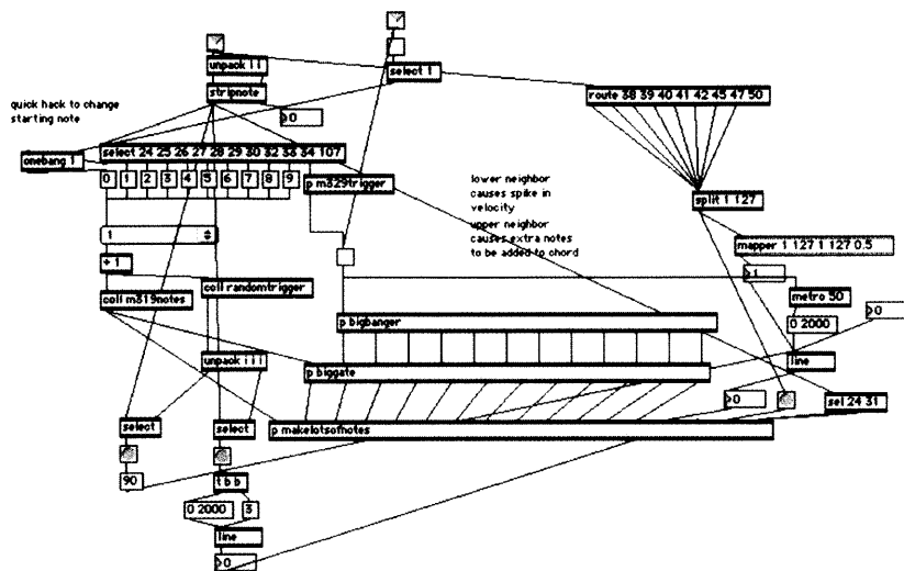
Fig. 3.9: Texture blob 3 - swirling polyrhythms patch
