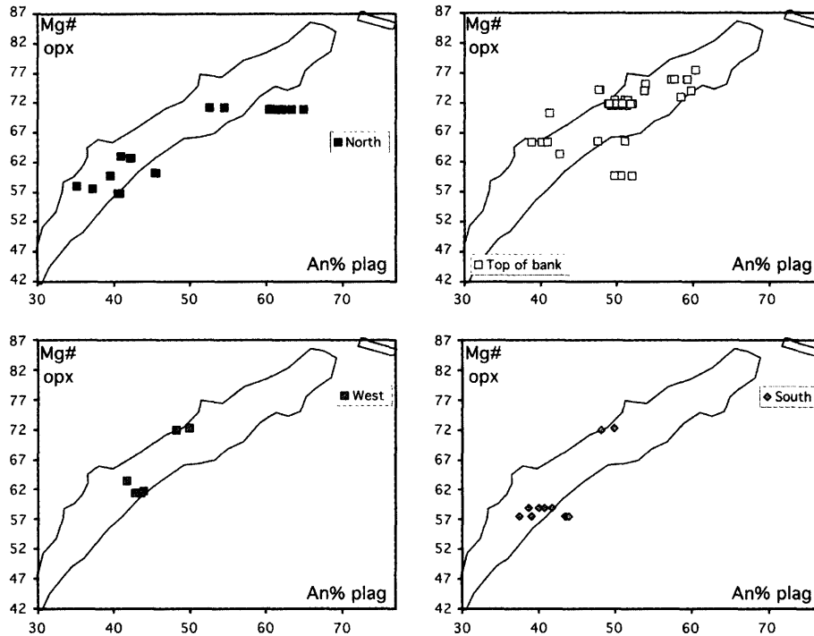
Figure 5-8: C: The composition of coexisting plagioclase (plag) and orthopyroxene (Mg#). The fields represent Hole 735B gabbronorites.
