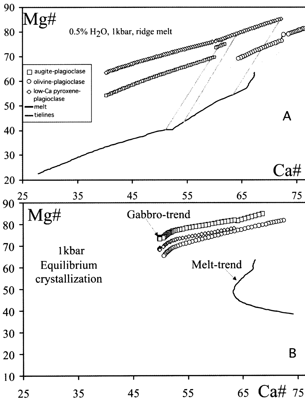
Figure 3-4: A : Crystallization of RC27-9-44-14 with 0.5 wt% H 2 O at 1kbar and QFM. B : Bulk crystallization of the same melt, where the solid is not separated from the liquid. Note how the melt compositions turns around and becomes higher in Ca# with crystallization.
