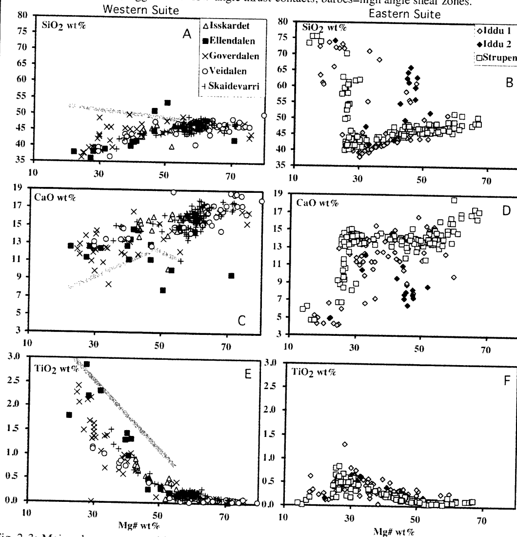
Fig. 2-3: Major element compositions of gabbroic whole-rocks sampled from seven different areas in the Lyngen Gabbro. Figures A, C, and E show Harker diagrams for the Western suite, and B, D, and F the Eastern suite, respectively. Iddu has been separated into Iddu-1, the general sampling of the area, and Iddu-2, a detailed transition. The inserts in E (Ellendalen) and F (Iddu 2) show the difference between the two suites. The gray fields in A, C and E indicates the field for the South West Indian Ridge.
