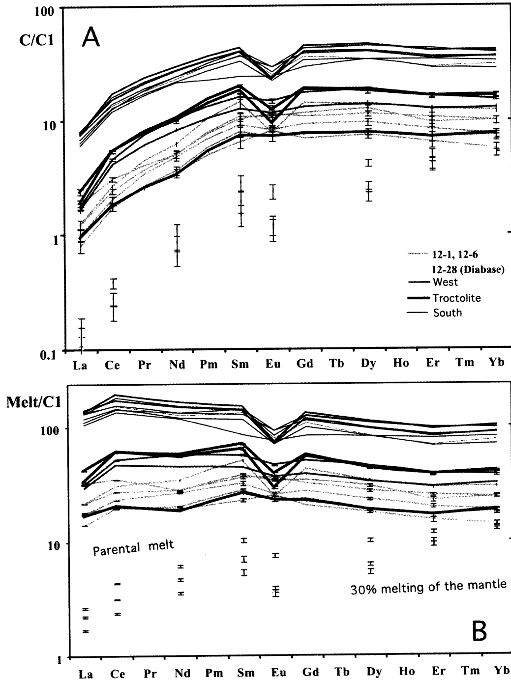
Figure 6-2: A: REE-plots for the augites in this study. The error-bars indicate 1\sigma . B: The hypothetical melts in equilibrium with the gabbro augite-crystals. Two parental melts, made from 5.5 and 30% batch equilibrium melting of the depleted upper mantle (Workman, in prep) are also shown. The partition coefficients used are from Bédard (1994).
