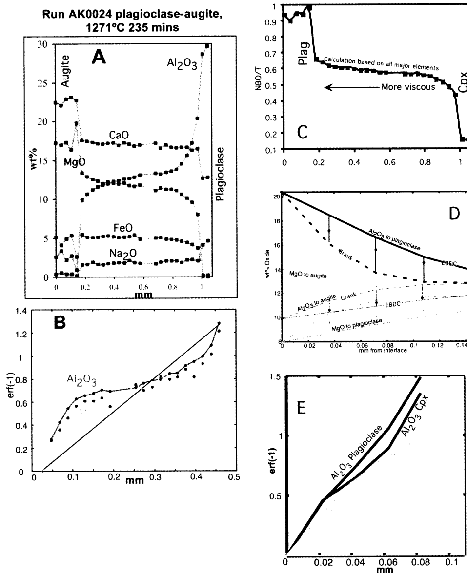
Figure 4-8: A: Chemical profiles across the augite-melt-plagioclase interface in sample AK0024. SiO 2 is not included as the concentrations are similar in both minerals. B: If the entire profile is diffusion controlled, \text{erf}^{-1}\left(\frac{x}{2\sqrt{Dt}}\right) should follow a straight line through the origin. C: The non-bridging oxygens per tetrahedrally coordinated cation (NBO/T) (Mysen, 1988) are inversely related to the polymerization of the melt and melts to plagioclase are more viscous than those to augite. D: Fits to the data, using diffusion-coefficients calculated from only the melts closest to the interface. Broken lines are calculated using the classical method from Crank (1975), the full lines are using the effective binary diffusion coefficients (EBDC) from Zhang et al., (1989). Thick black lines are Al 2 O 3 in the melt to plagioclase, thin black lines are Al 2 O 3 in the melt to augite, thick grey lines are MgO in the melt towards plagioclase, thin grey lines are MgO to augite. The data are dots in the respective colors, connected to the corresponding diffusion-profiles by vertical lines. E: The melts close to the mineral interfaces follow a near straight line for erf -1 .
