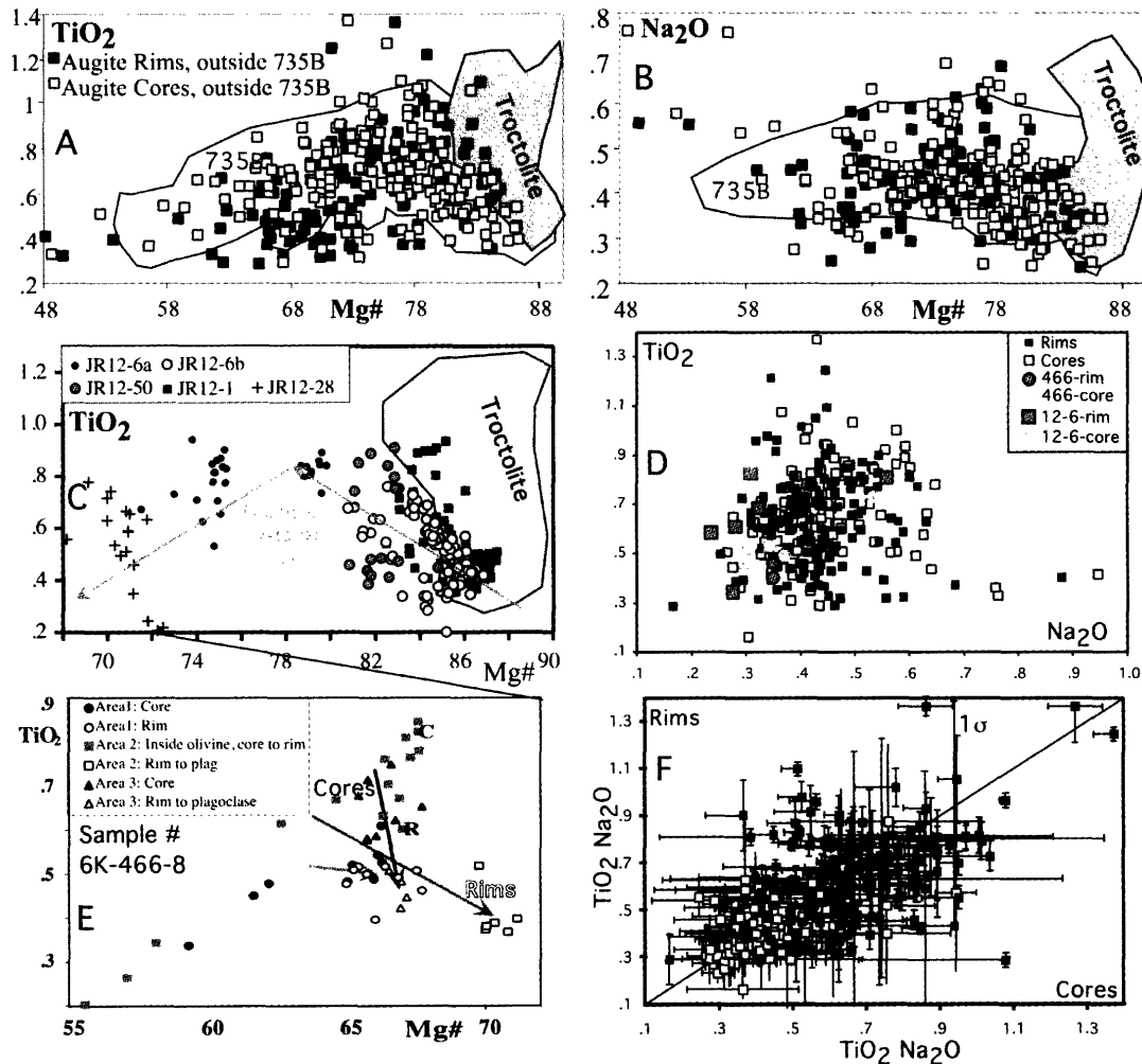
Figure 5-11: Minor element chemistry of augites analyzed in this study, compared to the upper 550-m of Hole 735B. A: Average Mg\# - TiO_2 of augites from our study compared to the general outline of Hole 735B and the cross-cutting Hole 735B troctolites from the upper 550 meters of the core. B: Average Mg\# 's vs. Na_2O for the same rocks. C: Rocks in a single dredge in the northern showing wide ranges of compositions in augite (individual analyses). In addition, single samples can have dramatically different augite compositions between grains (JR12-6a and 6b). The more evolved JR12-28 sample plot perpendicular to a normal fractionation trend. D: There is no direct linear relationship between Na_2O and TiO_2 in augite. E: Augites from a single, evolved oxide-olivine gabbro has more refractory cores than rims, plotting perpendicular to the fractional crystallization trend in C. F: There are as many reversely zoned augites as there are normally zoned ones: true both for Na_2O (open squares with bars indicating 1\sigma variation) and for TiO_2 (closed squares with bars indicating 1\sigma variation).
