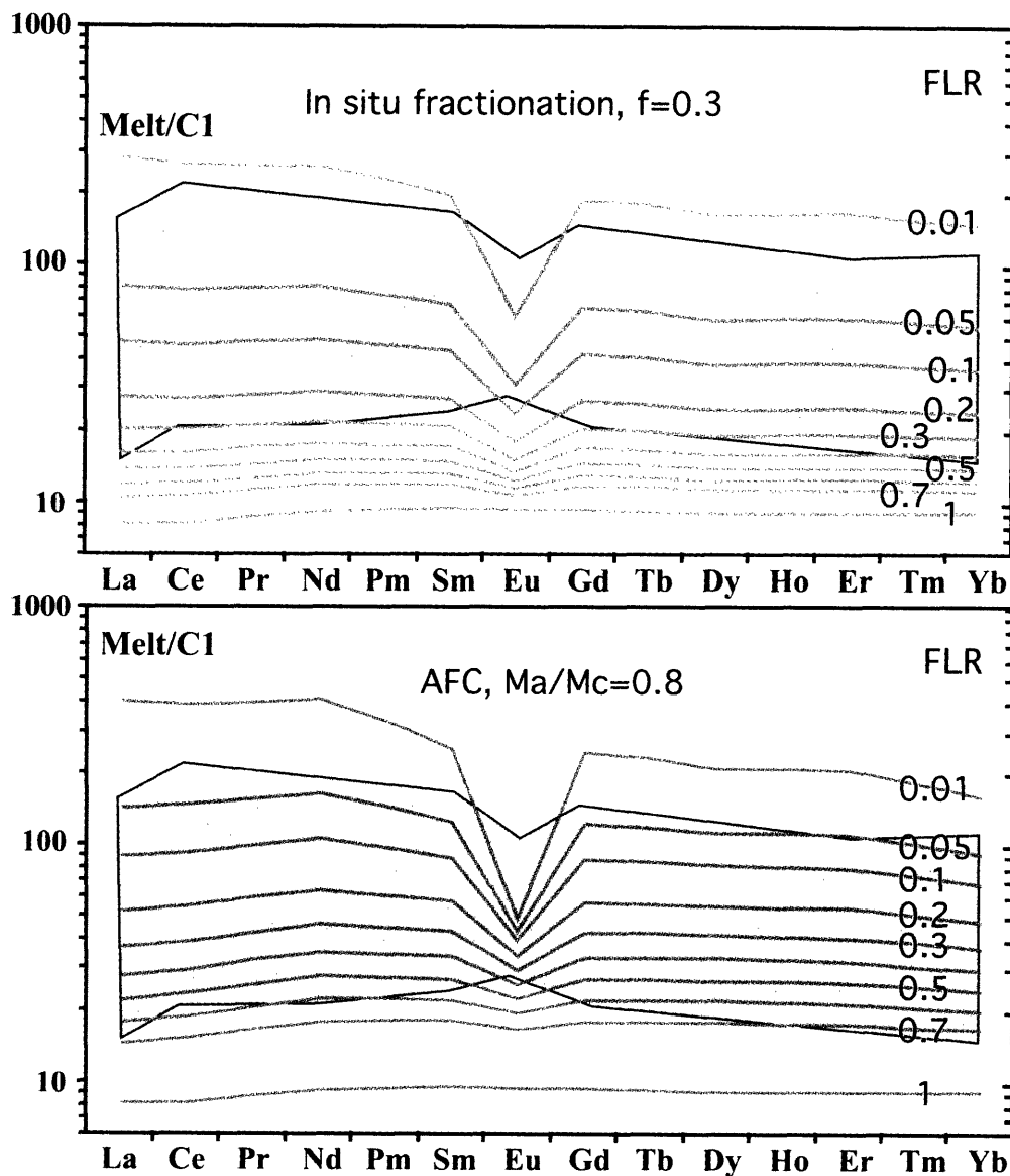
Figure 6-4: REE-element plots for crystallization models (normalized to the CI chondrite of Taylor and MacLennan (1995)). FLR=Fraction of liquid remaining, the gray lines describe degree of fractionation. FLR(0.05) = 95% crystallized relative to the original melt. The gray field outlines the theoretical melt compositions based on the composition of augite in the gabbros (note that the diabase-data are excluded). A: In-situ fractionation, where only 30% of the interstitial melt is returned from the mush-zone to the central magma. B: The fractionation and crystallization of the DMM-derived melt happens during bulk-assimilation of the average olivine gabbro from Hole 735B (Natland and Dick, 1992). The diagram demonstrates that even if the melt experienced assimilation of pre-existing olivine-gabbros, the gabbros represent melts that first fractionated 50% elsewhere, but then crystallized to near completion.
