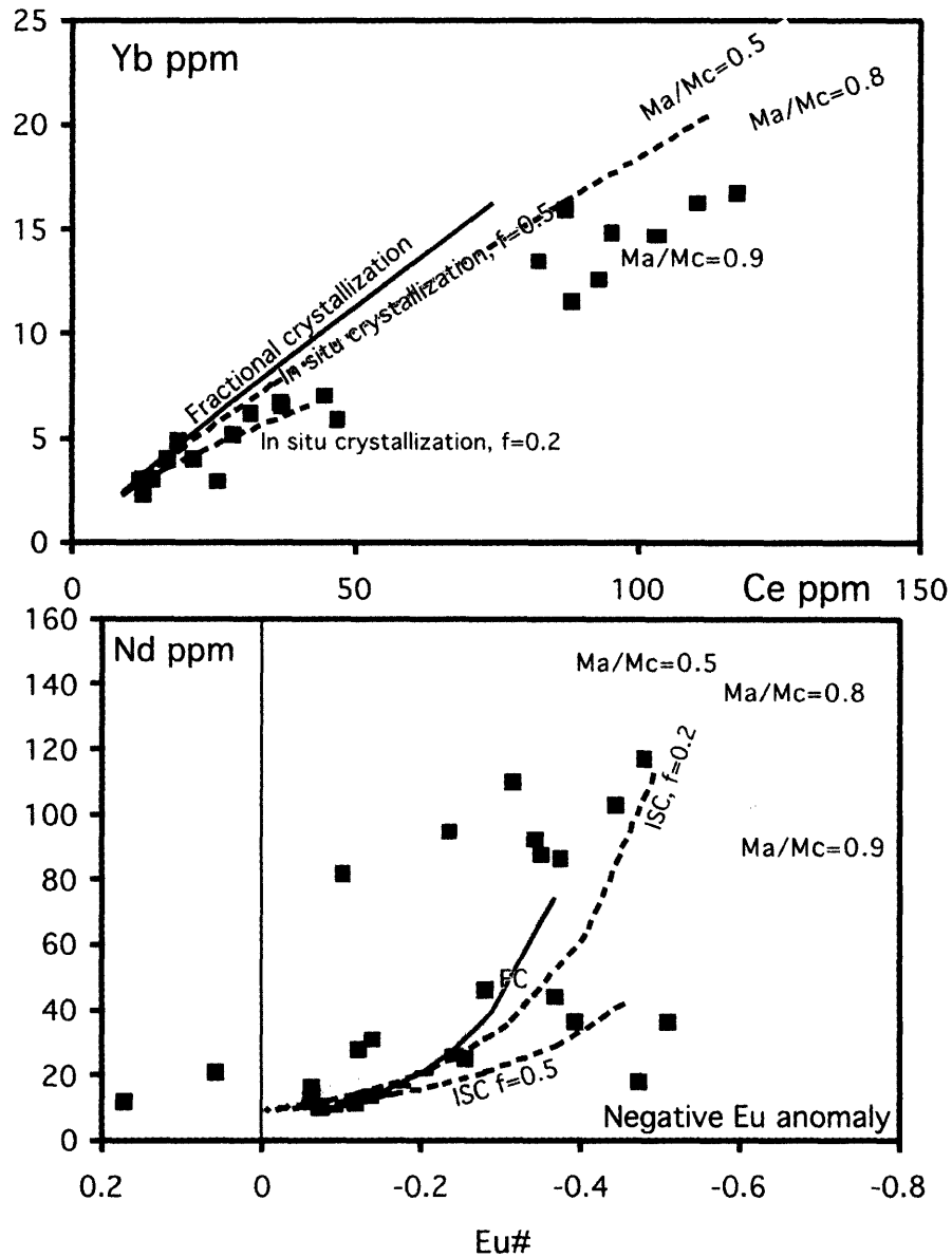
Figure 6-3: Crystallization models for our samples compared to the hypothetical melts in equilibrium with the augites. A: It appears that the AFC-models and in-situ fractionation fit the augite-melts better than a pure fractional crystallization model. “Ma”=Mass assimilated; “Mc”=Mass crystallized; “f” = fraction of melt returned from the mush-zone to the magma chamber; Eu\# = (Eu^* - ([Sm^* + Gd^*] \times 0.5) - 1) , where Eu^* , Sm^* and Gd^* represent chondrite-normalized values. Negative Eu\# 's are negative Eu-anomalies, indicating fractionation of plagioclase from the melt.
