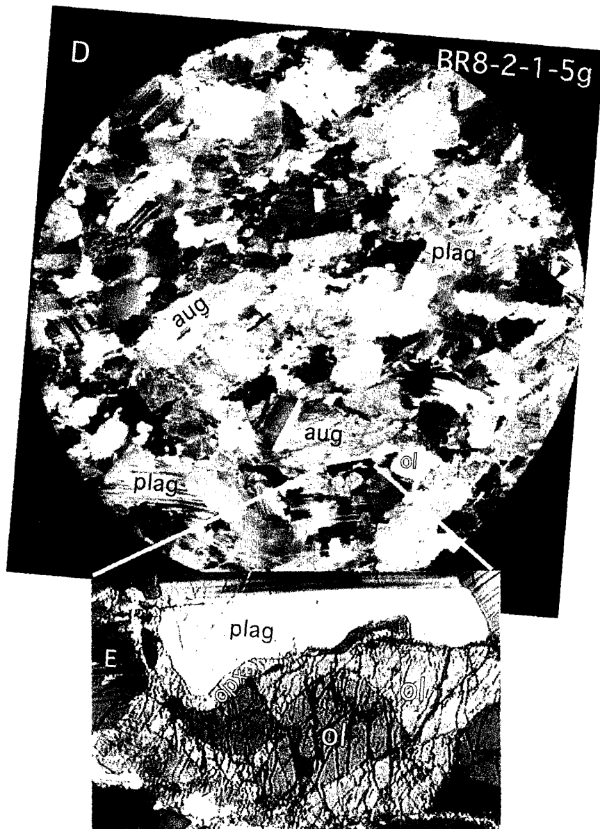
Figure 5-3: A: Sample # JR31-12-1: Sub-ophitic augite surrounds plagioclase-laths with interstitial olivine. Cross-polarized light. Plag=plagioclase, aug=augite, ol=olivine. Field of view is 3" from left to right. B: Same slide in parallel light. C: Sample 6K-466-8, field of view is 1" across. An olivine-gabbro-norite-oxide-gabbro-norite contact, as seen by the extensive interstitial oxide-crystals to the right. The boundaries between the lithologies are indicated by the white line. The picture is taken using a combination of reflected and parallel light to distinguish the different minerals. Three areas (indicated) have been analyzed. D: Sample # BR8-2-1-5g: The sample has been partially deformed at high temperatures, as seen in the kink-banded plagioclase and rounded augite. Cross-polarized light, the slide is 1" across. E: Detail of C: a thin orthopyroxene-grain lies between an olivine grain (with the characteristic cracking-pattern) and plagioclase
