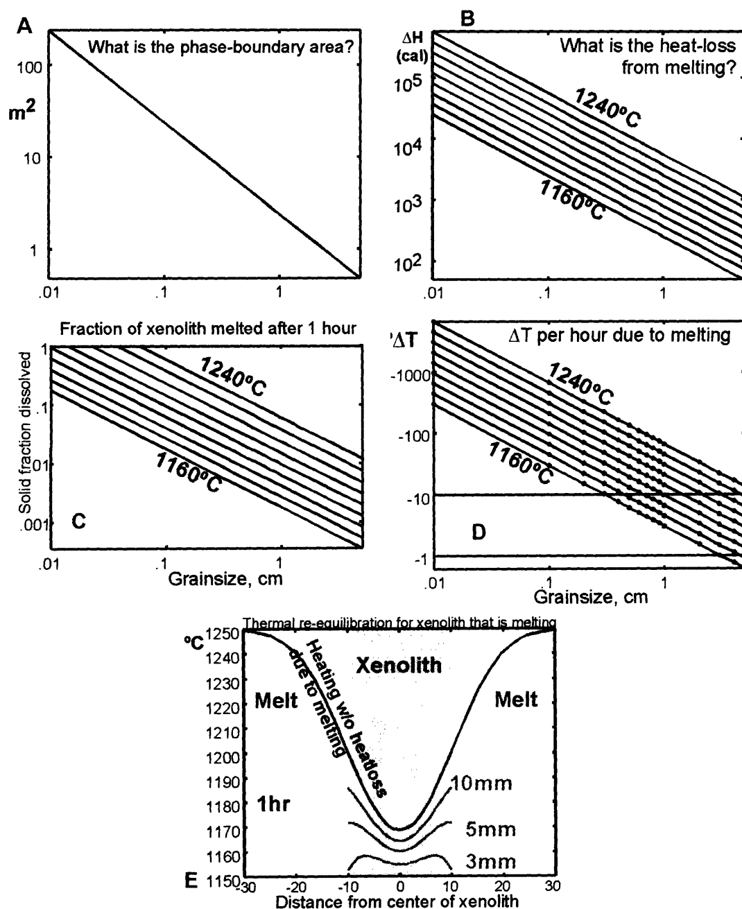
Figure 4-12: A: The geometric area of contact between the minerals of a 20cm bimineralic (50:50) cube for varying grainsizes. B: The heat-loss from melting after one hour at different temperatures and grainsizes. C: The fraction of melting relative to the volume of the original xenolith after one hour. D: the temperature drop calculated per hour due to melting on the boundaries. E: The thermal re-equilibration of the xenolith calculated with and without the heat-loss due to dissolution for varying grain sizes in one hour. The results for grain-sizes less than 3mm yield heat-losses so large that they prevent the heat from penetrating the xenolith.
