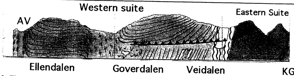
Fig. 2-2: The three areas sampled in the southern part of the Lyngen Gabbro, Ellendalen, Governalen and Veidalen, represent a composite cross-section through the Western suite. The profile is drawn to scale and is about 10-km long as the crow flies. Yellow=The sedimentary Balsfjord Group; green=Aksla Volcanics; orange = Western suite of Lyngen Gabbro, with lines = layering in the gabbro, with hatches=varitextured gabbro; brown=Eastern suite of the Lyngen Gabbro; tan=Rypdalen Shear Zone; red=Kjosens Greenschist; purple=ultramafic rocks; tagged lines=low-angle thrust-contacts; barbes=high angle shear zones.
