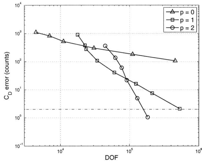
Figure 5-29: NACA 0012 wing: AR=2 , M = 0.1 , \alpha = 0^\circ . Drag output error versus degrees of freedom. Dashed line indicates prescribed tolerance of e_0 = 2 counts.
