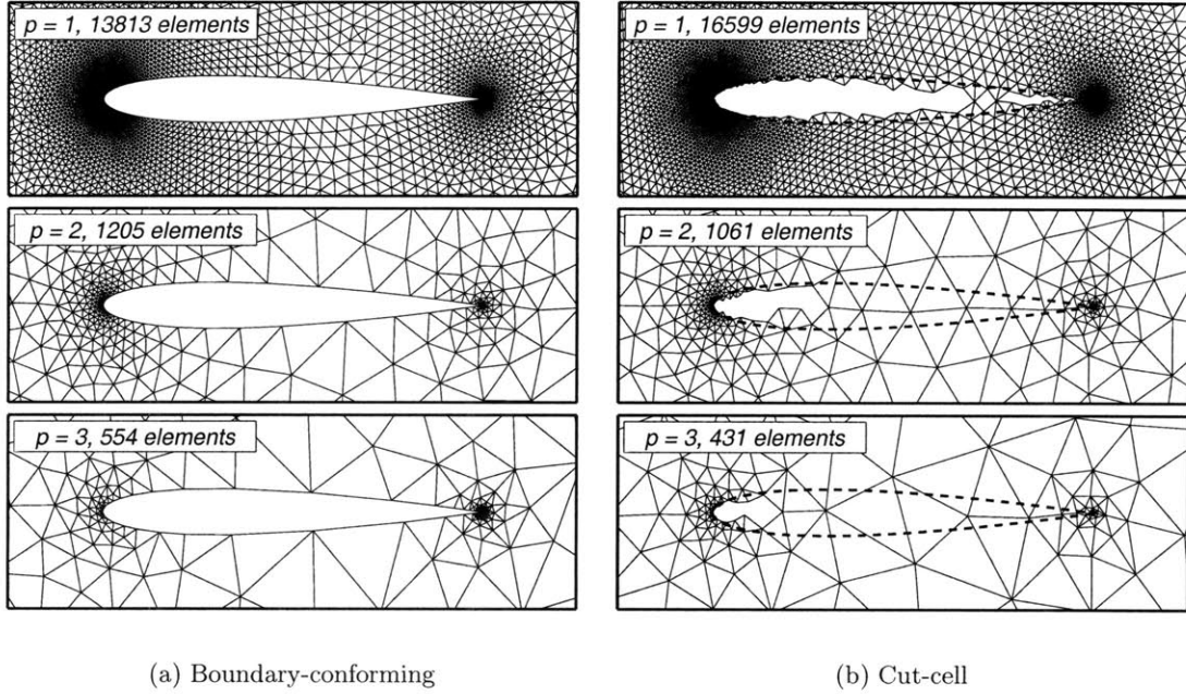
Figure 4-12: NACA 0012: M_\infty = 0.5 , inviscid, \alpha = 2^\circ . Final boundary-conforming and cut-cell meshes for p = 1, 2, 3 , adapted to a drag tolerance of e_0 = 0.1 counts.
