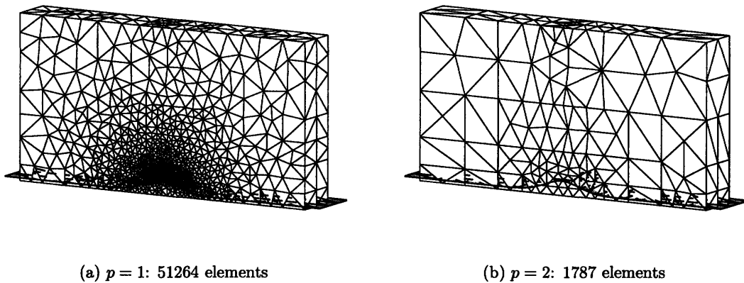
Figure 5-22: Gaussian bump channel: M = 0.3 . Final adapted meshes for p = 1 and p = 2 .
