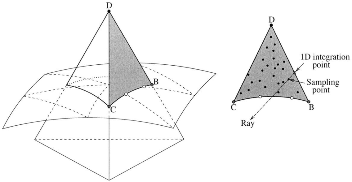
Figure 5-16: Three cut faces result from the intersection depicted in Figure 5-4. This figure highlights one of these cut faces. Sampling points generated by ray-casting in the plane of the cut face are also shown.
