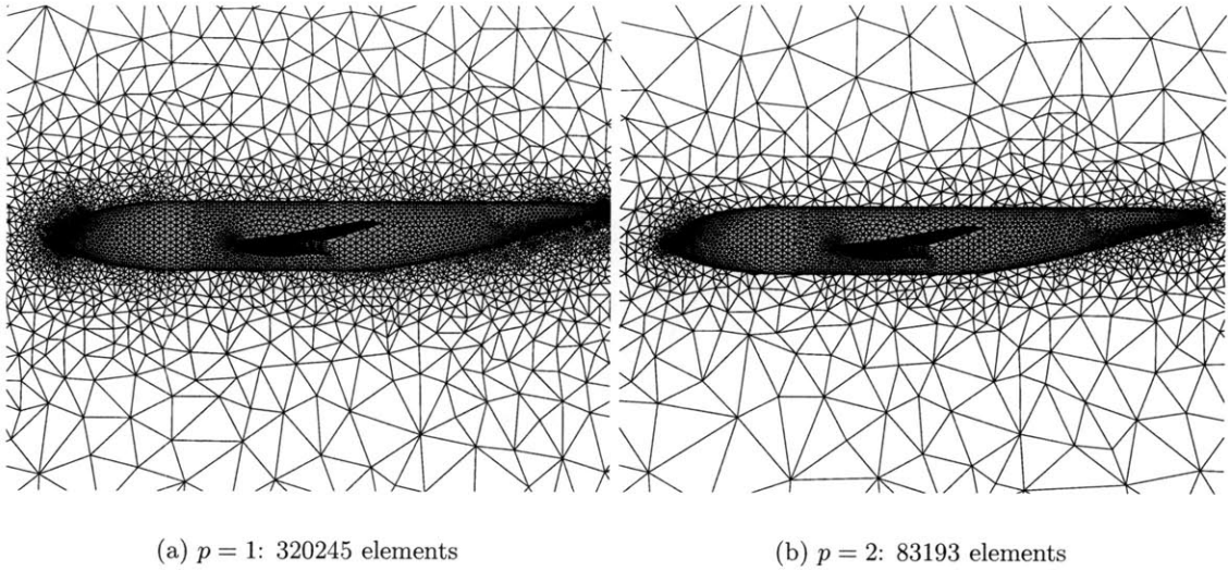
Figure 5-34: Wing-body: M = 0.1, \alpha = 0^\circ . Finest adapted meshes for p = 1 and p = 2 .
