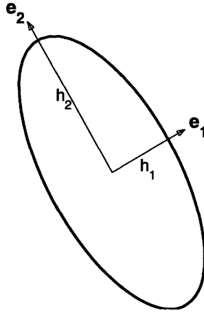
Figure 3-3: Ellipse representing requested mesh sizes implied by equal measure under a Riemannian metric \mathbf{M} . Also shown are the principal directions, \mathbf{e}_i , and the associated principal stretching magnitudes, h_i .
