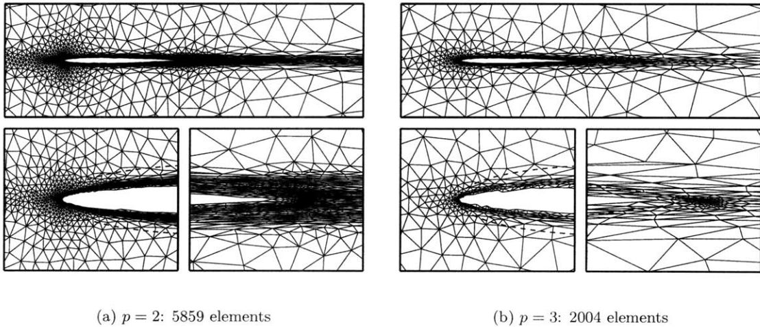
Figure 4-27: NACA 0005: M_\infty = 0.4, Re = 50000, \alpha = 0^\circ . Final cut-cell meshes adapted on drag.
