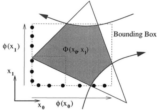
Figure 4-6: Construction of the \Phi_i(\mathbf{x}) functions for use in defining the integration basis, \zeta_i(\mathbf{x}) . The \Phi_i(\mathbf{x}) are tensor products of one-dimensional Lagrange functions, \phi_{i_k}(x) , in each spatial direction on the cut-cell bounding box.
