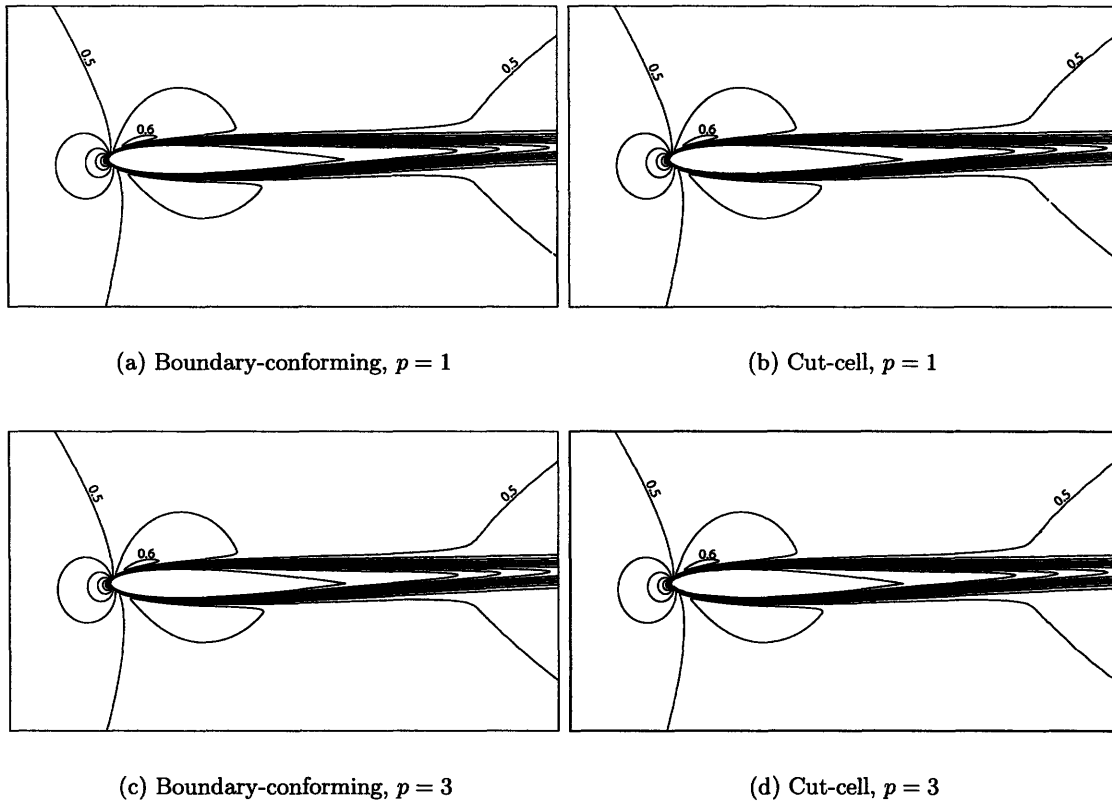
Figure 4-17: NACA 0012: M_\infty = 0.5 , Re = 5000 , \alpha = 2^\circ . Mach number contours for p = 1 and p = 3 on the final adapted boundary-conforming and cut-cell meshes.
