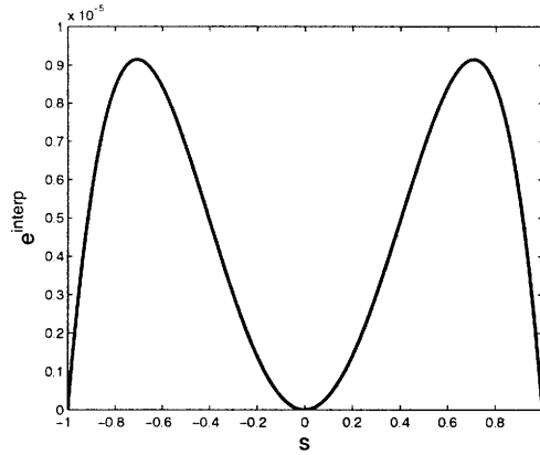
Figure F-2: Geometry interpolation error along a quadratic panel for \Delta\theta = \pi/12 . The maximum interpolation error is 9.1 \times 10^{-6} .
