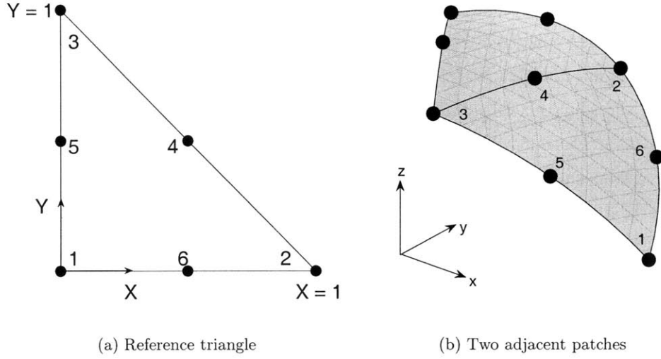
Figure 5-1: Patch reference triangle (a) and an example of two adjacent patches (b). The first three nodes in the numbering are the “linear nodes”, whereas the latter three are the “high-order nodes.”
