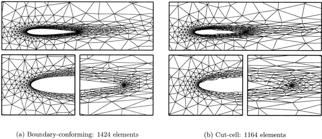
Figure 4-21: NACA 0012: M_\infty = 0.5 , Re = 5000 , \alpha = 2^\circ . Final p = 3 meshes adapted on lift with tolerance e_0 = 1 count.
