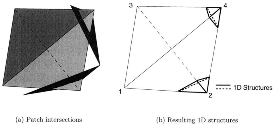
Figure 5-10: Two cut cells arising from the cutting of one tetrahedron. The two corners adjacent to nodes 2 and 4 of the original tetrahedron lie inside the computational domain. In addition, two of the original tetrahedron's faces are cut into multiple (two) disjoint regions.
