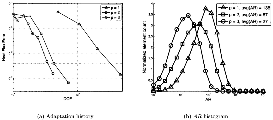
Figure 4-36: Joukowski airfoil: Pe = 4 \times 10^8 . Output error versus DOF adaptation history and a histogram of element aspect ratio in the final adapted meshes.
