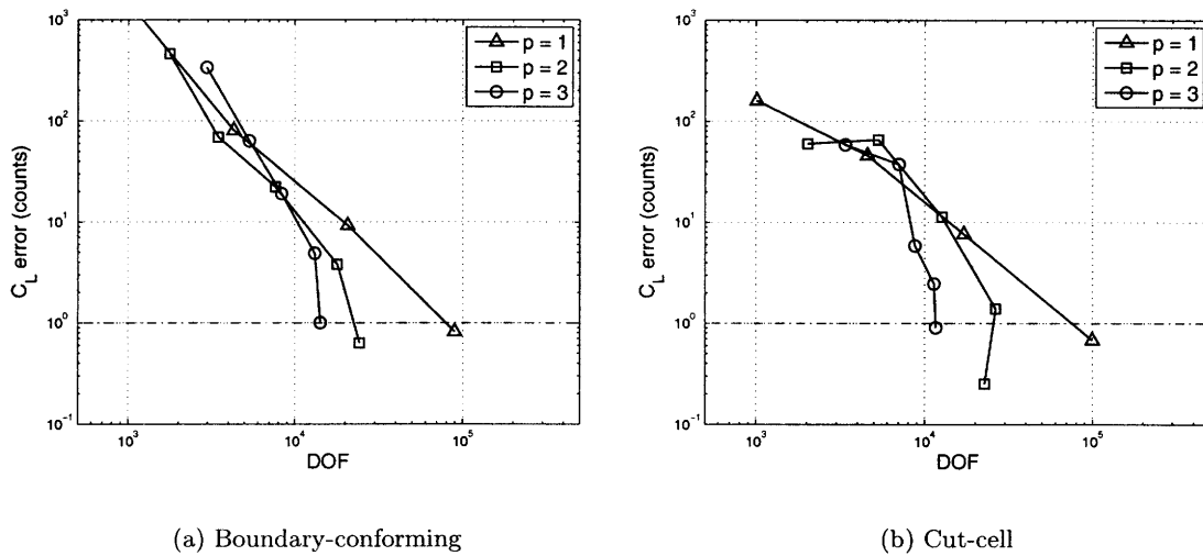
Figure 4-19: NACA 0012: M_\infty = 0.5 , Re = 5000 , \alpha = 2^\circ . Lift error versus degrees of freedom. Dashed line indicates prescribed tolerance of e_0 = 1 lift counts.
