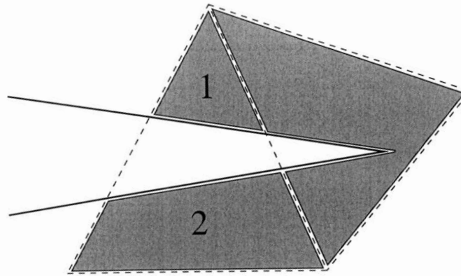
Figure 4-3: Example of cut cells formed at an airfoil trailing edge. The background triangle on the left is split into two cut cells, as indicated by the labels “1” and “2.” The triangle on the right becomes one cut cell with four neighbors.
