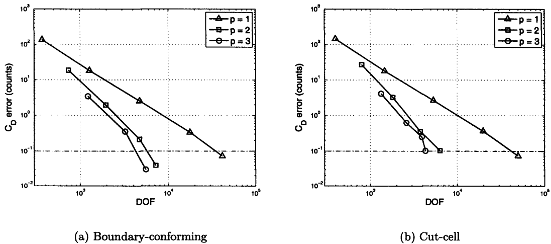
Figure 4-11: NACA 0012: M_\infty = 0.5 , inviscid, \alpha = 2^\circ . Drag error versus degrees of freedom. Dashed line indicates prescribed tolerance of e_0 = 0.1 counts.
