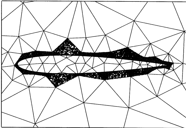
(a) Entire airfoil
