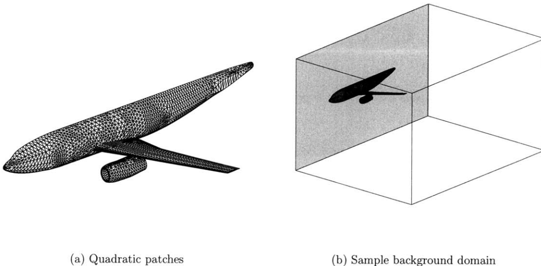
Figure 5-3: Quadratic patch surface representation of a wing-body-nacelle geometry (a) and one possible choice for the background domain (b). The shaded side of the background domain indicates a symmetry boundary condition. Farfield boundary conditions are applied on the other sides.
