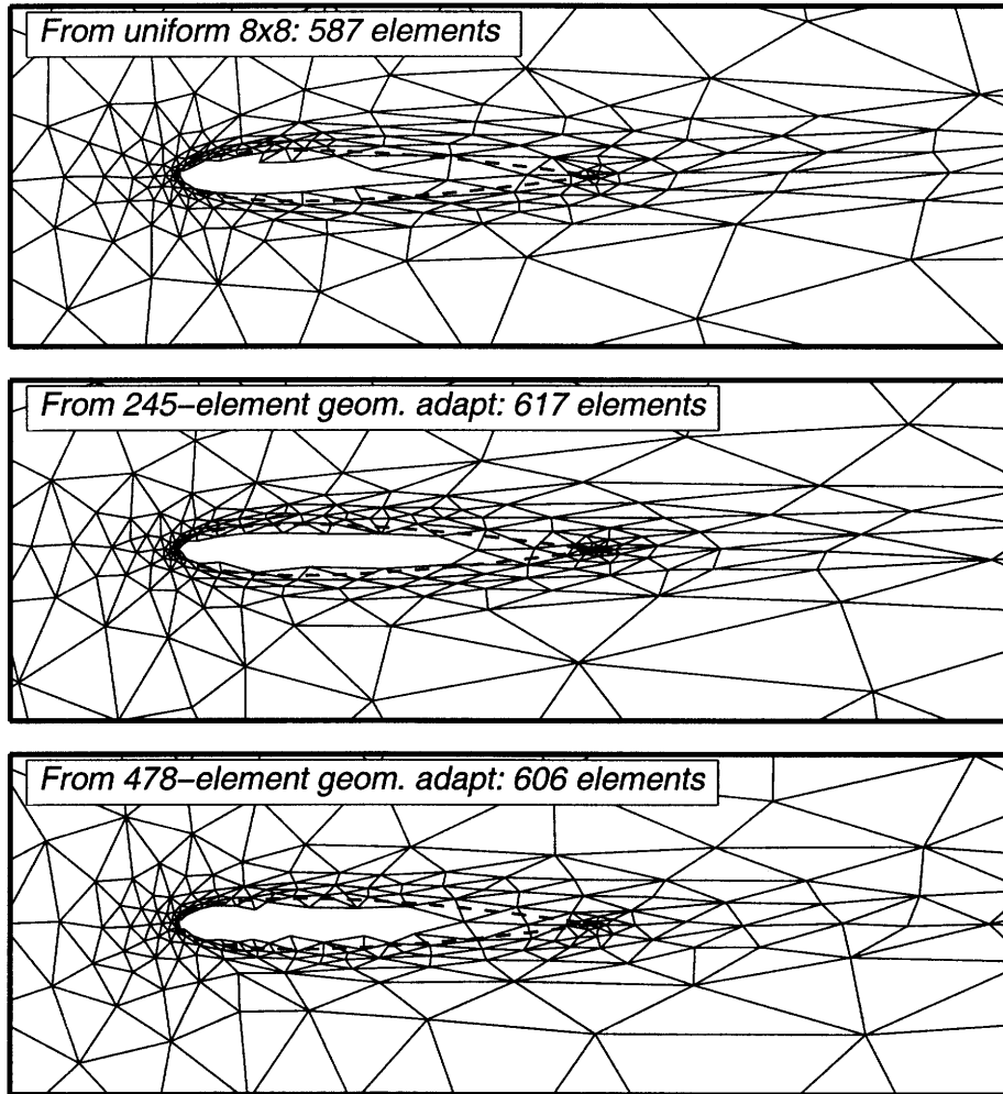
Figure 4-24: Mesh-sensitivity study: final p = 3 meshes for the three initial meshes shown in Figure 4-22.
