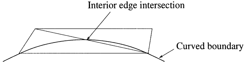
Figure 1-4: Example of a curved boundary intersecting an interior edge adjacent to two anisotropic triangles. Attempting to curve the boundary edge introduces a negative Jacobian in the mapping from the reference triangle to the curved element and hence renders the triangulation invalid.
