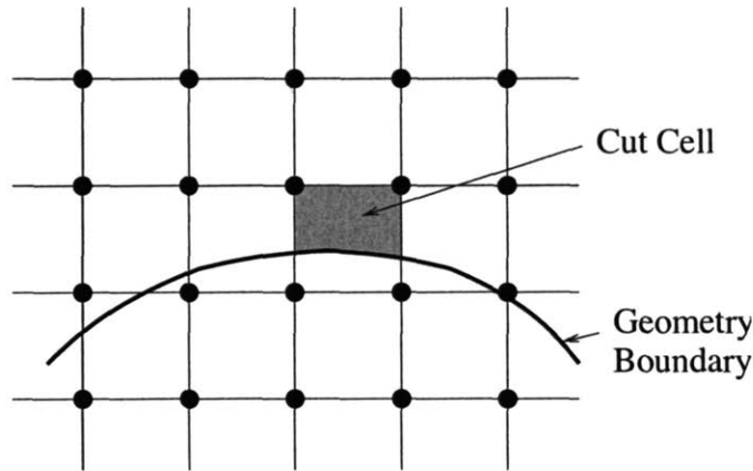
Figure 1-5: Sample Cartesian mesh in two dimensions. The square lattice mesh does not conform to the geometry. Cut cells are portions of intersected elements that lie inside the computational domain (above the geometry boundary in this case).
