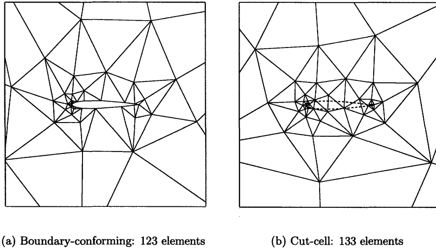
Figure 4-10: NACA 0012: M_\infty = 0.5 , inviscid, \alpha = 2^\circ Initial meshes for adaptive runs.
