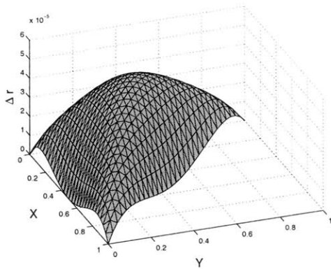
(a) Interpolation error over patch
