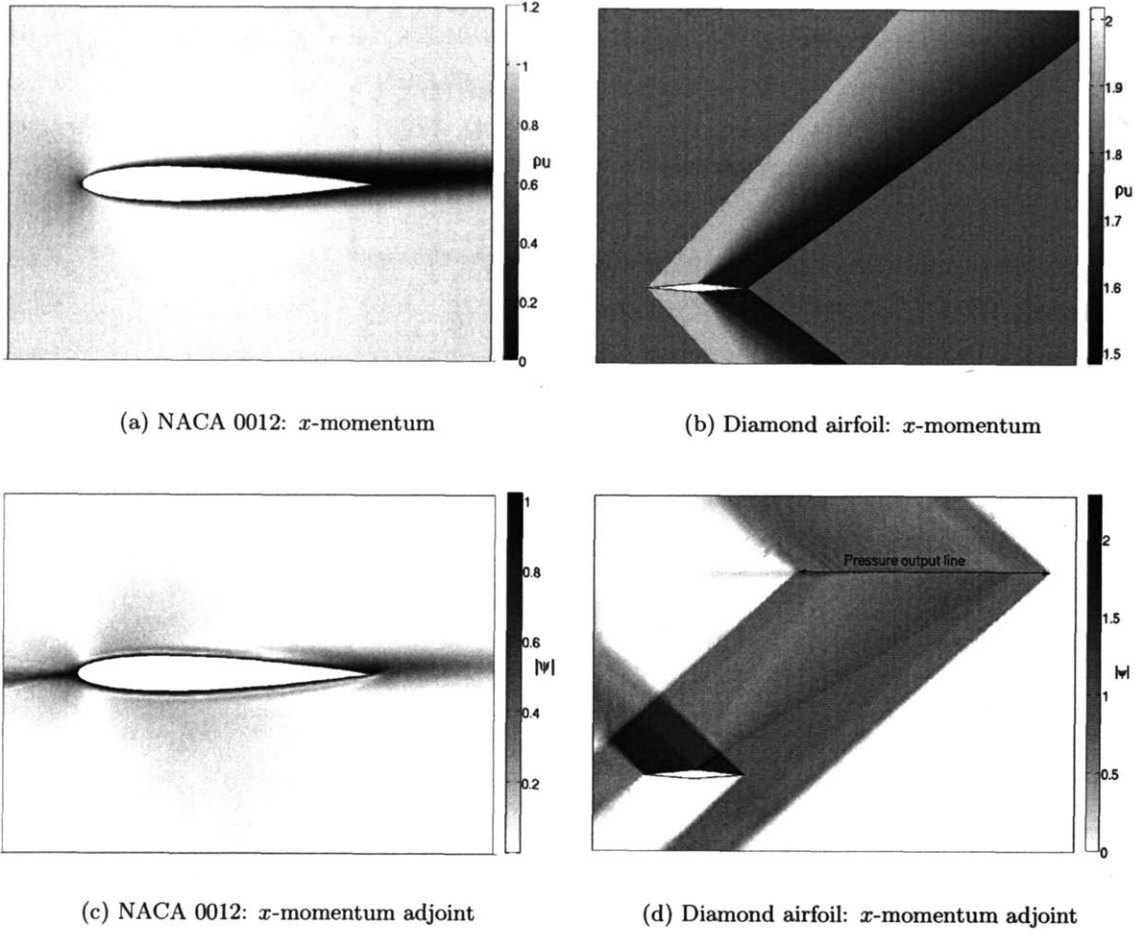
Figure 3-1: Sample flow and adjoint solutions: (a) x -momentum for a NACA 0012 in subsonic, viscous flow; (b) x -momentum for a diamond airfoil in supersonic, M = 1.5 flow; (c) x -momentum adjoint associated with a drag output on the NACA 0012; (d) x -momentum adjoint for a pressure line integral output computed several chords away from the diamond airfoil. For the adjoint, the absolute value is plotted with dark areas indicating large magnitudes.
