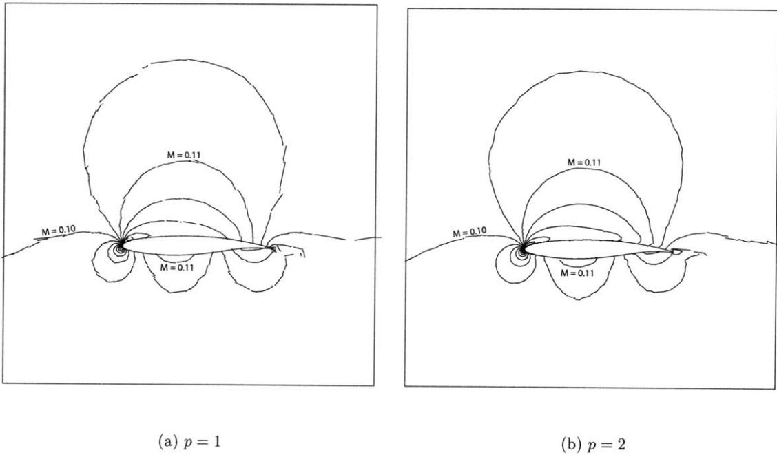
Figure 5-35: Wing-body: M = 0.1, \alpha = 0^\circ . Mach number contours on the finest meshes for p = 1 and p = 2 . The cut is parallel to the x-z plane and is situated at 50% of the half-span.
