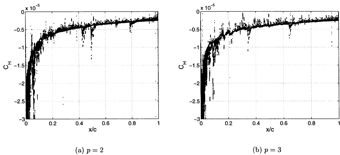
Figure 4-41: Joukowski airfoil: Pe = 4 \times 10^{10} . Heat transfer coefficient along the airfoil surface on the final adapted p = 2 and p = 3 meshes.
