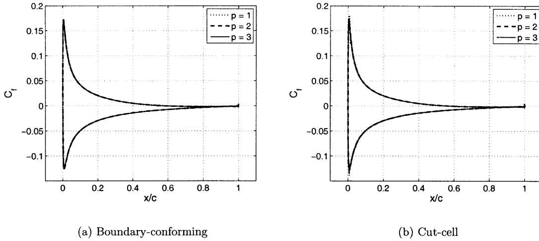
Figure 4-18: NACA 0012: M_\infty = 0.5 , Re = 5000 , \alpha = 2^\circ . Surface skin friction coefficient distributions for solutions on the final adapted boundary-conforming and cut-cell meshes. These plots were generated by evaluating C_f at the quadrature points on the embedded boundary edges.
