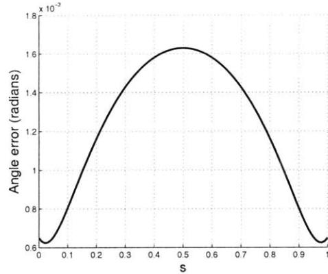
(b) Slope error along edge
