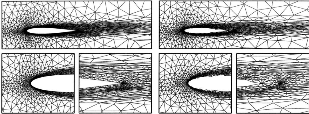
(a) Boundary-conforming: 4068 elements
