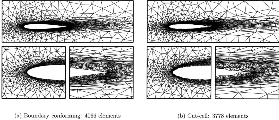
Figure 4-20: NACA 0012: M_\infty = 0.5 , Re = 5000 , \alpha = 2^\circ . Final p = 2 meshes adapted on lift with tolerance e_0 = 1 count.
