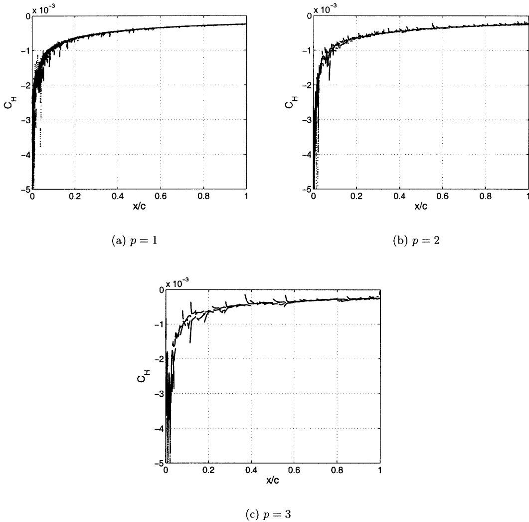
Figure 4-34: Joukowski airfoil: Pe = 4 \times 10^6 . Heat transfer coefficient along the airfoil surface on the final adapted p = 1, 2, 3 meshes. Negative heat transfer corresponds to heat flux into the flow, out of the airfoil.
