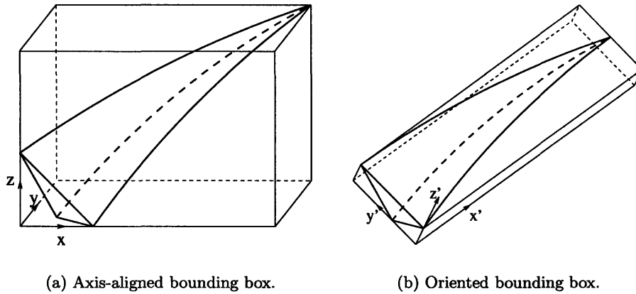
Figure 5-18: Numerical conditioning improvement of element-interior integration via bounding-box rotation for the case of a sliver element.
