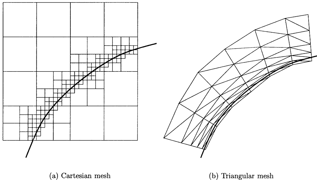
Figure 1-6: Comparison of Cartesian and triangular cut-cell meshes of a curved boundary layer. As the boundary is not aligned with the grid, isotropic refinement is required for the Cartesian mesh (a). With triangular cut cells, anisotropic refinement is possible in general directions (b).
