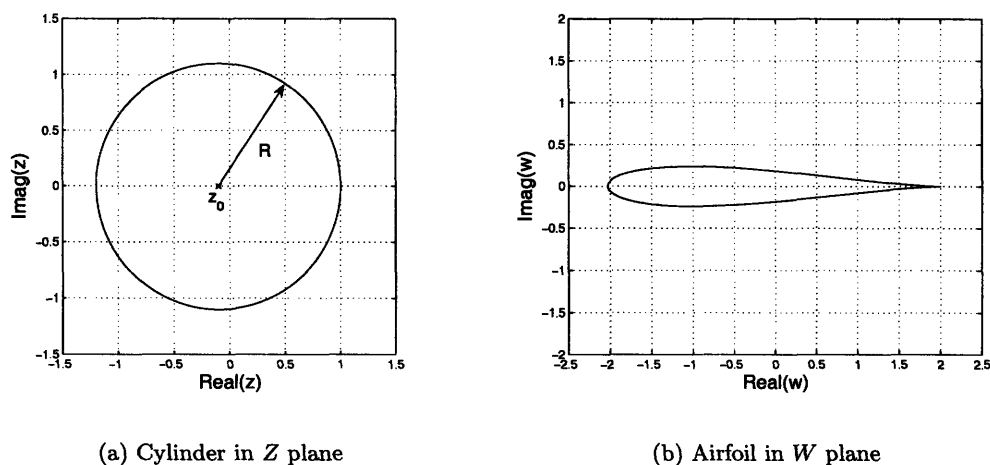
Figure 4-30: Joukowski transformation from a cylinder to an airfoil with a cusped trailing edge. The origin of the cylinder is on the real axis, which means that the resulting Joukowski airfoil is symmetric.
