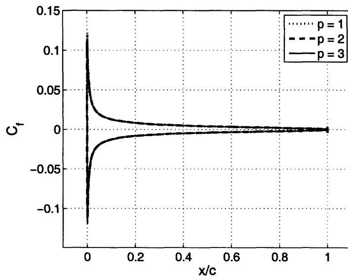
Figure 4-29: NACA 0005: M_\infty = 0.4 , Re = 50000 , \alpha = 0^\circ . Skin friction coefficient distributions on the final adapted meshes.
