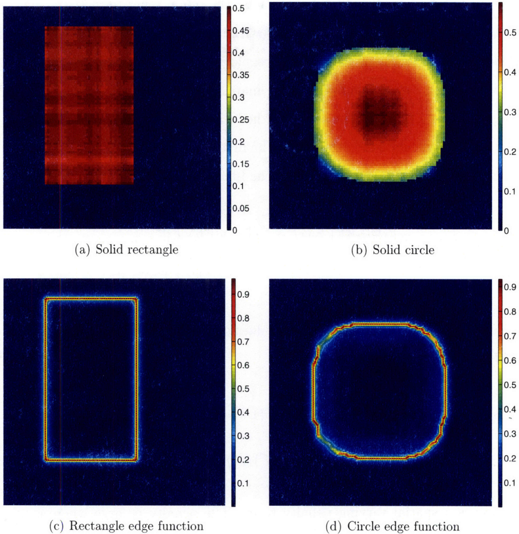
Figure 5-4: 2D reconstruction using convexity term – Reconstructed data and edge functions found using gradient descent to find a minimum of Equation 5.3. The artifacts found in Figure 5-3 are removed.
