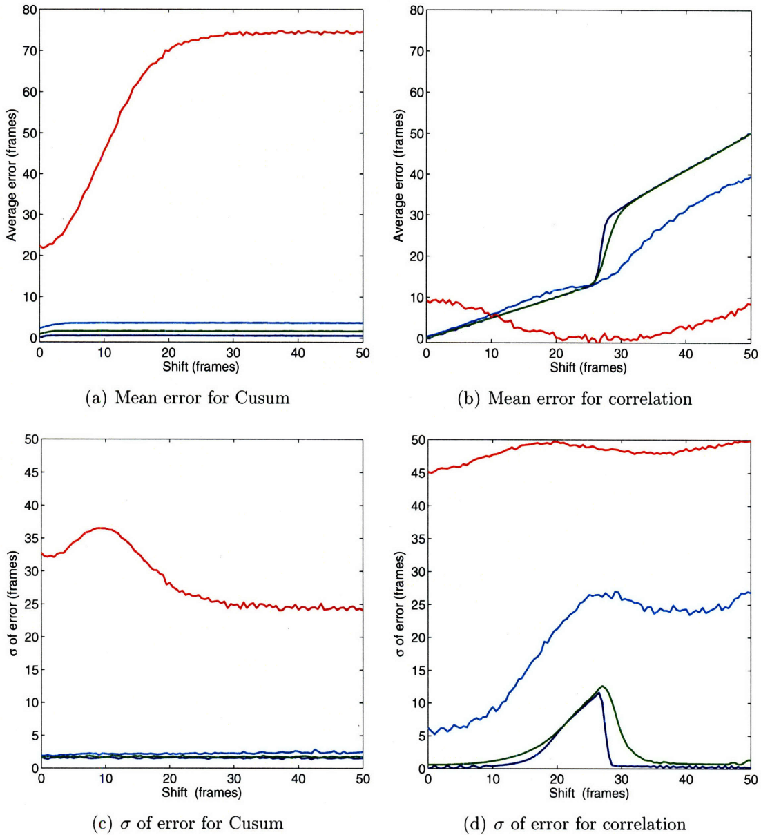
Figure 4-8: Performance of the two arrival time algorithms – Plots are shown for both the mean (top) and standard deviation \sigma (bottom) of the error after 10,000 iterations of both the Cusum-based algorithm (left) and the minimum square difference of correlation based algorithm (right) as a function of the shift applied to the second template. Shifts from zero to fifty are applied on the second template, some examples are shown in Figures 4-6 and 4-7. The results are shown for four levels of zero mean Gaussian noise with standard deviation of 0.0065 (blue), 0.02 (green), 0.065 (cyan), and 0.2 (red).
