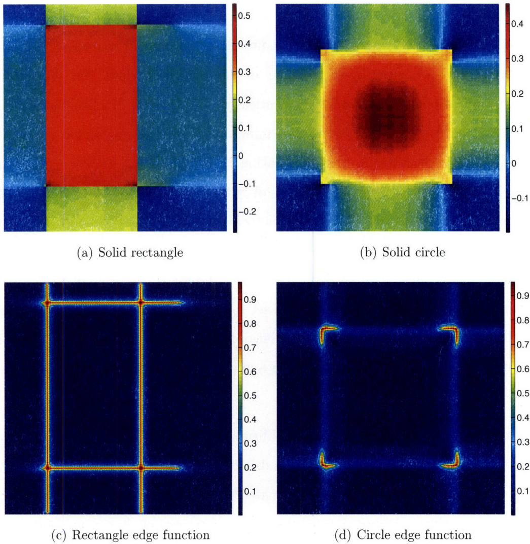
Figure 5-3: 2D reconstruction using edge term – Reconstructed data and edge functions using a numerical solution to equation 5.2.
