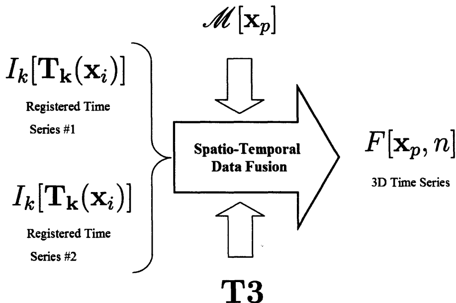
Figure 5-1: Spatio-Temporal Data Fusion – Flowchart showing the Spatio-Temporal Data Fusion process. The prepared data in Chapter 3, the two registered time series I_k[\mathbf{T}_k(x_i)] , the constraint map \mathcal{M} , and the 3D orientation information \mathbf{T}_3 , is combined to produce a time series of 3D volumes.
