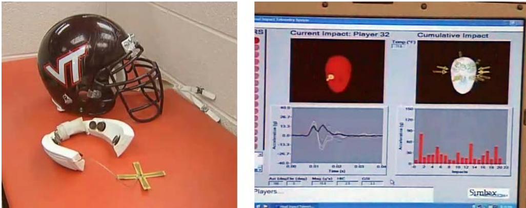
Figure 3. Virginia Tech helmet with accelerometers and data visualization software.
