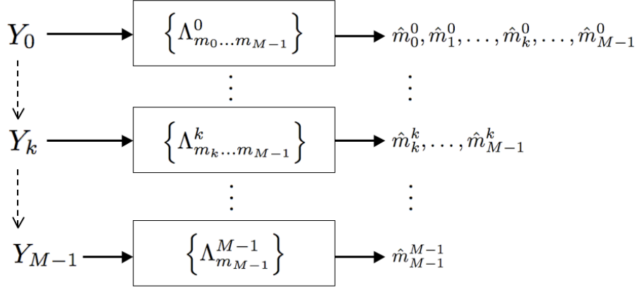
Degraded receivers | Quantum measurement (POVM elements) | Decoded messages (estimates)
