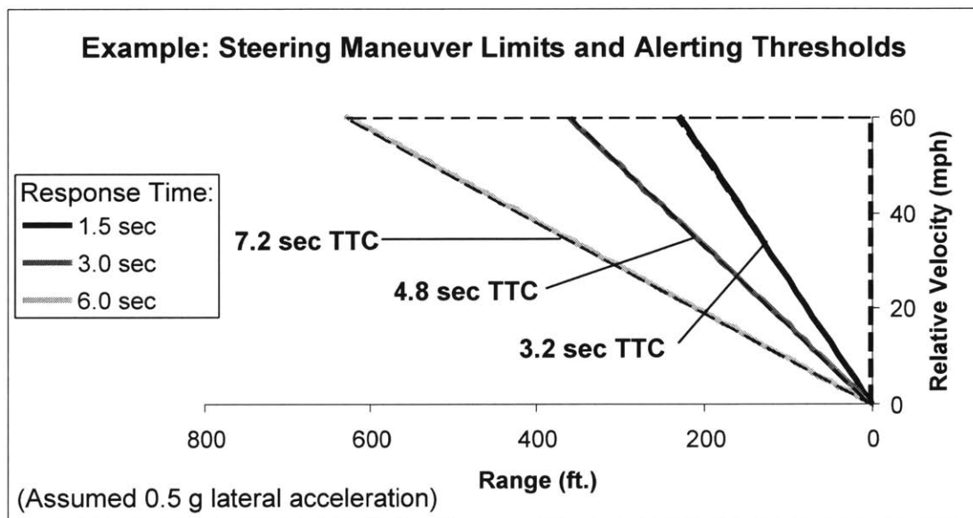
Figure 2-11: Example steering maneuver limits and corresponding notional alerting thresholds.
