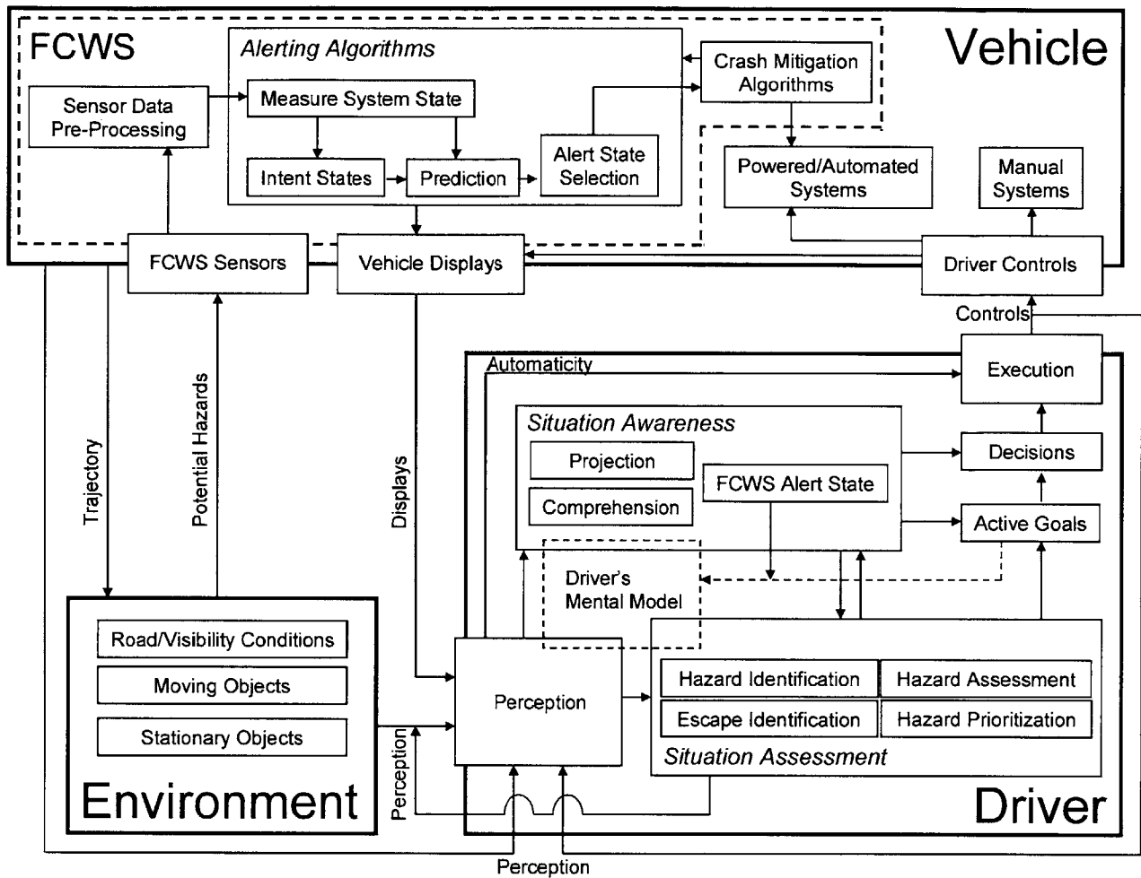
Figure 2-2: Detailed FCWS closed loop feedback process.
