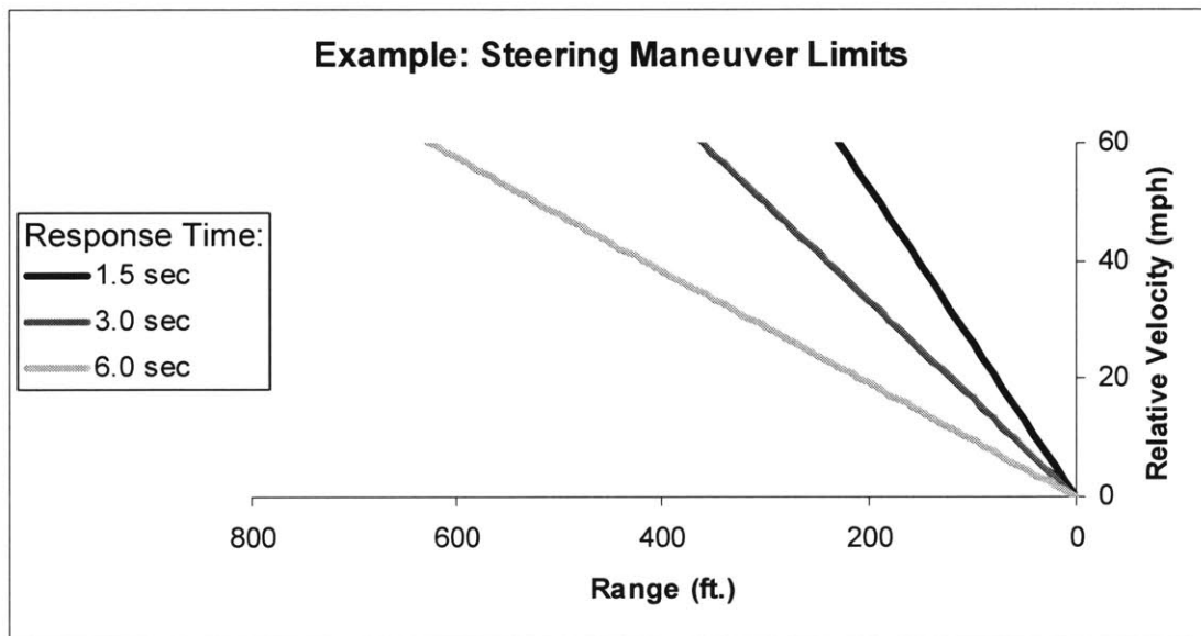
Figure 2-9: Example: steering maneuver limits for response times of 1.5, 3.0, and 6.0 seconds.
