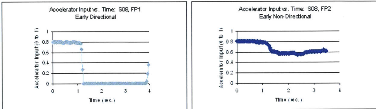
Figure 4-12: Example: accelerator input during unnecessary alert activations; first exposure to the Early Directional FCWS (1 of 2).
