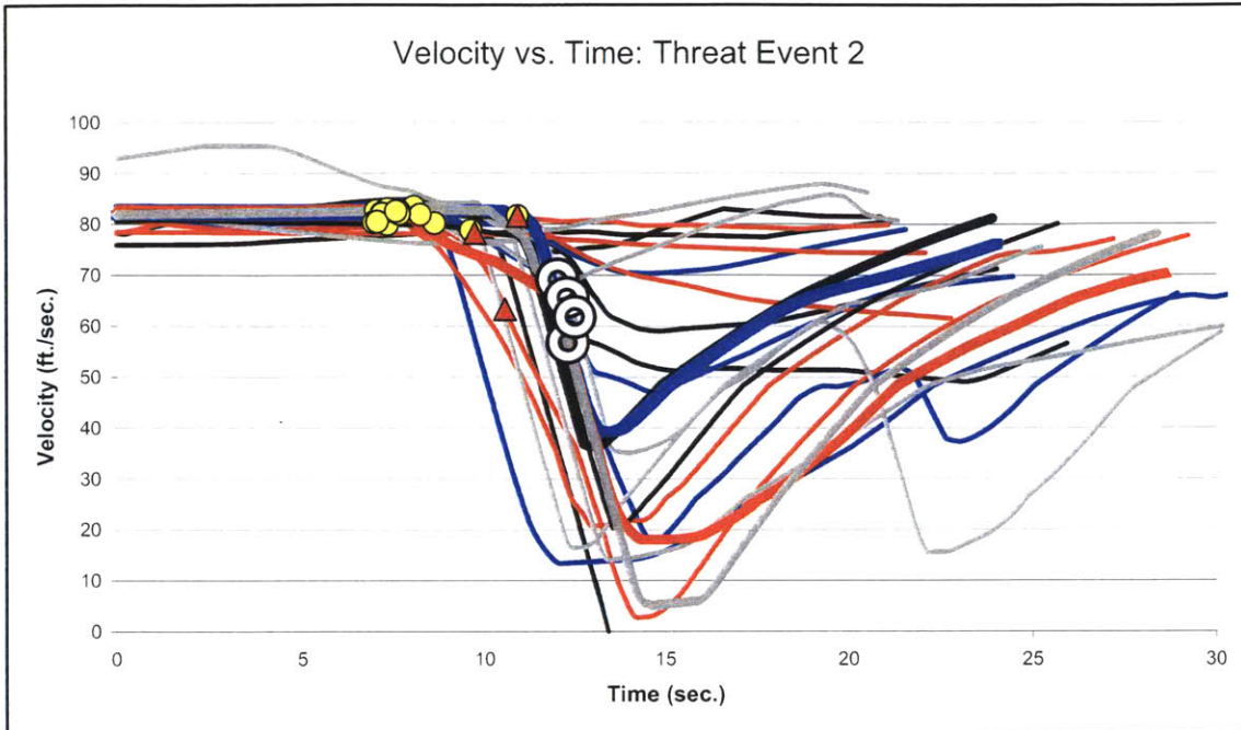
Figure 4-5: Velocity profile for TE2 (key to the right).
