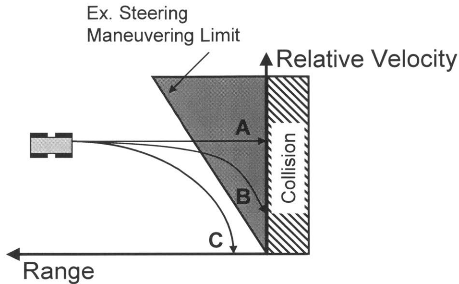
Figure 2-5: An example state-space representation of collision avoidance (steering to avoid).
