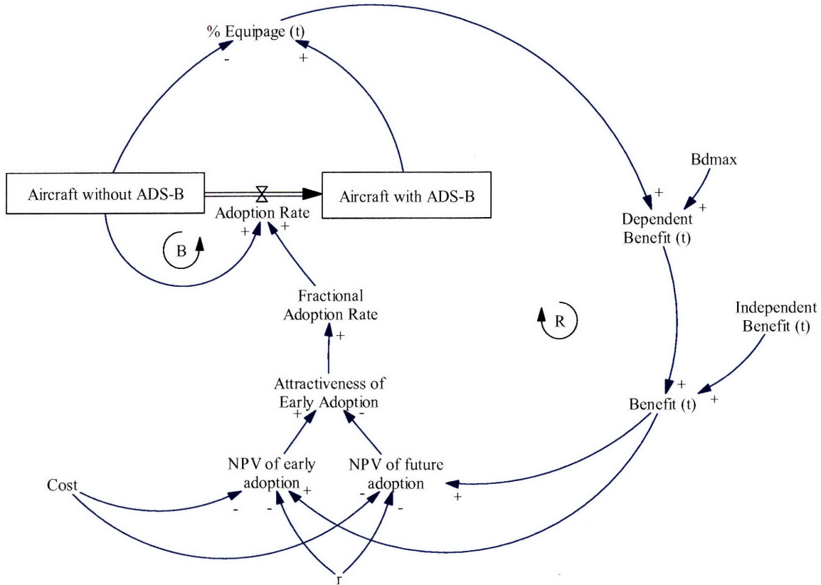
Figure 4-4: Basic Model of ADS-B Out Equipage
