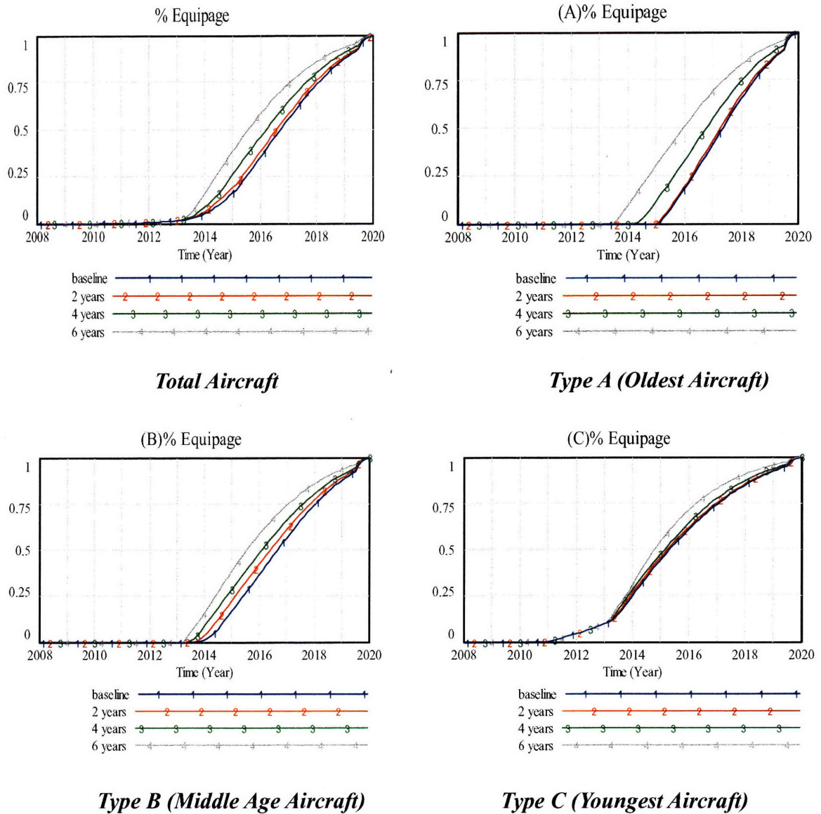
Figure 5-3: Change of Equipage Curve by Acceleration of Benefit (High Benefit Rate Type)
