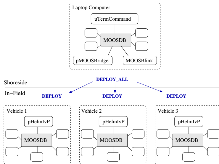
Figure 10: A common usage of the uTermCommand application for command and control.
