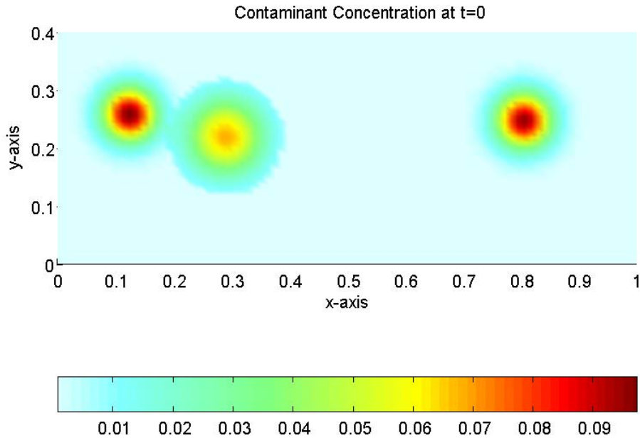
Figure 3-2: This figure depicts the sample test initial condition used to compare reduced model to full model in the forward problem.
