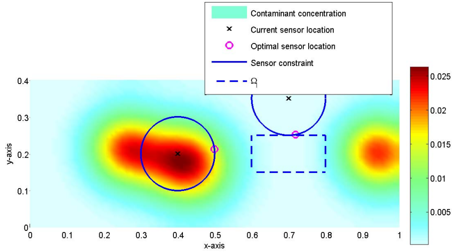
Figure 5-1: Contaminant concentration at t_f = 0.2 , current and optimal sensor locations of cycle one of the online stage with parameterized velocity field by \mu = \{0.75, 0.25, 0, 0, 0, 0, 0, 0\} .
