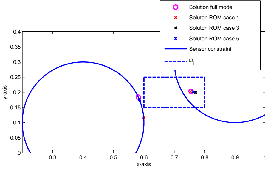
Figure 3-10: This figure contains the new sensor locations computed by the full model and several reduced-order models in the constrained case.
