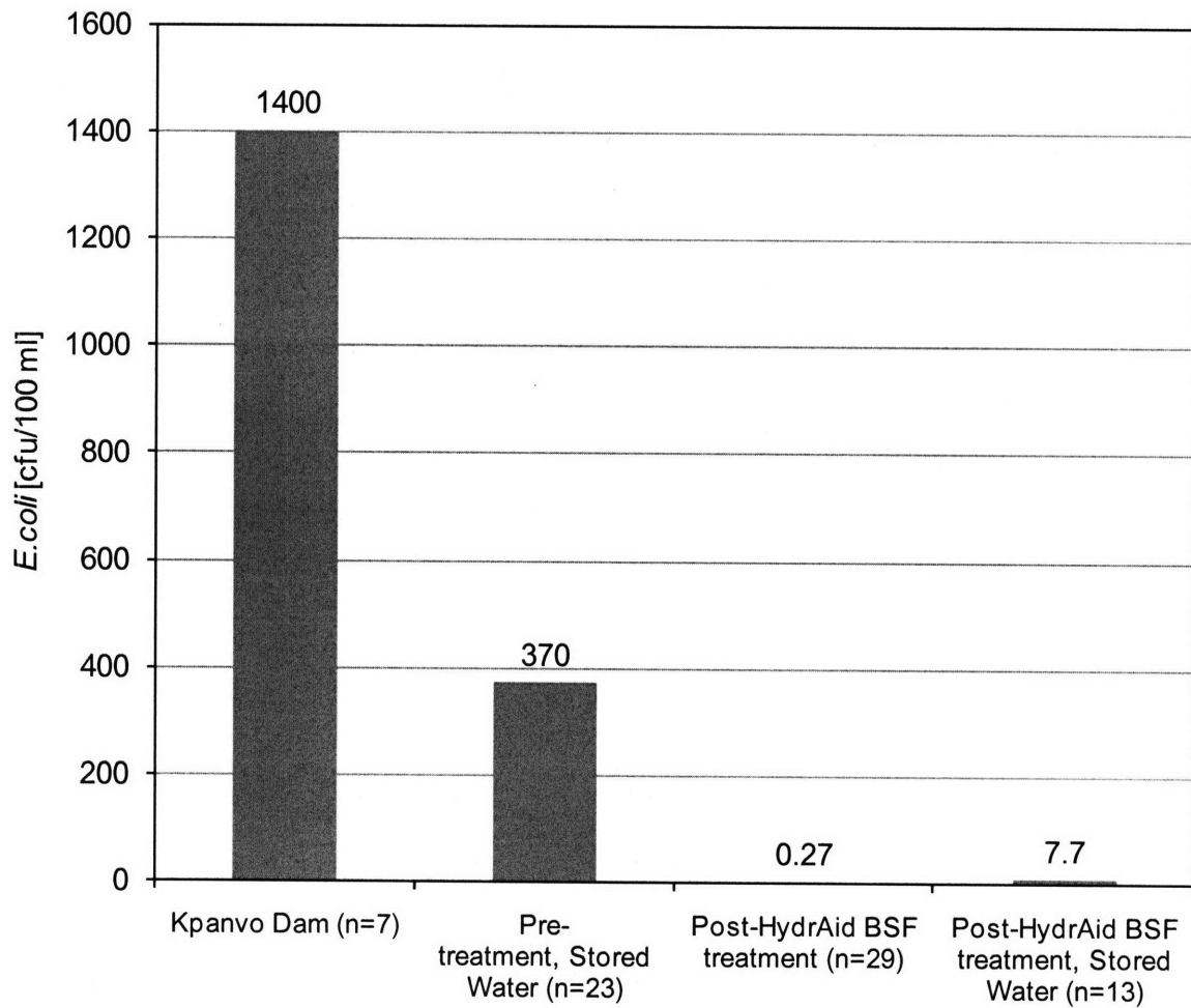
Figure 6-17 Average E. coli Concentrations at Different Stages of Treatment
