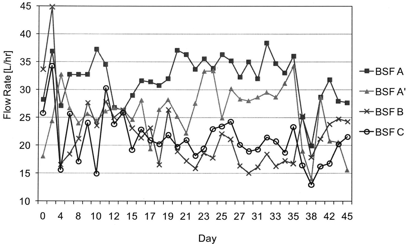
Figure 5-7 Flow Rate of Unmodified (BSF A & A') and Modified BSFs (BSF B & C)
