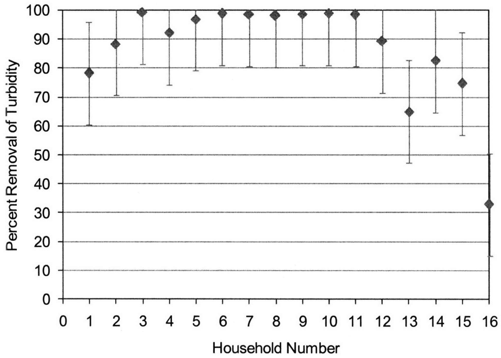
Figure 6-9 Turbidity Percent Removal of HydrAid BSFs
