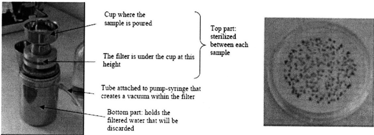
Figure 3-3 Membrane Filtration Method: Milipore portable membrane filtration assembly unit (left) and a sample showing results (right) (Source: Ngai & Walewijk, 2003)
