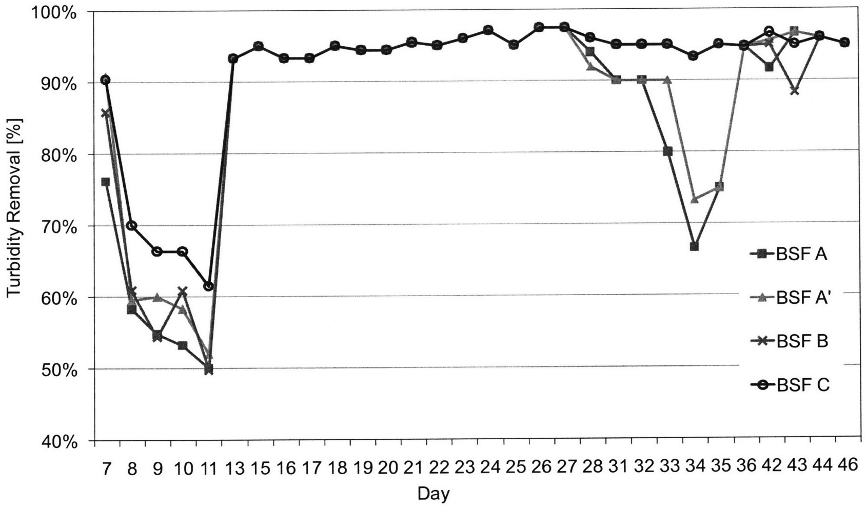
Figure 5-10 Turbidity Removal of the LPD BSFs
