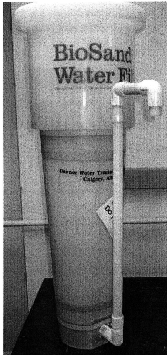
Figure 4-4 Picture of the Plastic Davnor BSF
