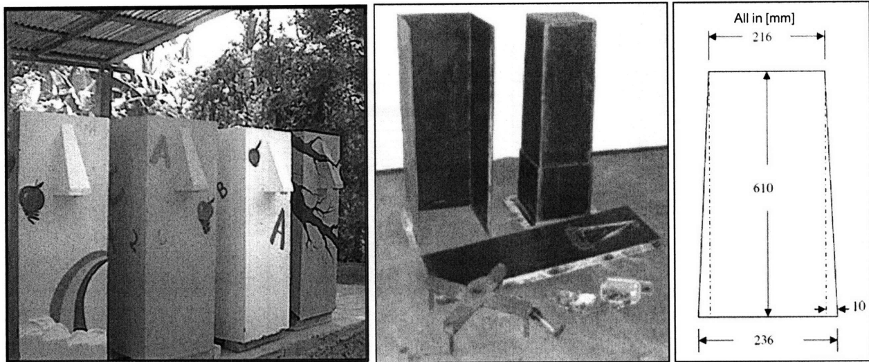
Figure 4-2 Concrete Rectangular BSF; Picture of Concrete BSFs in Haiti (left), Picture of Inner and Outer Mold (middle), Dimension of the Walls of the Inner Mold (right)
