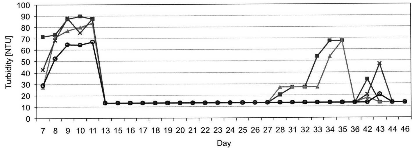
Figure 5-9 Turbidity of the Ghanasco Dam and Effluents of the LPD BSFs (Day 7 – Day 46; TU units converted to NTU)
