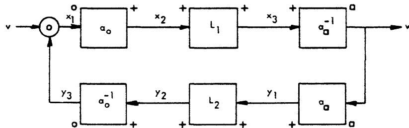
Fig. 11. Equivalent representation of a homomorphic feedback system.
