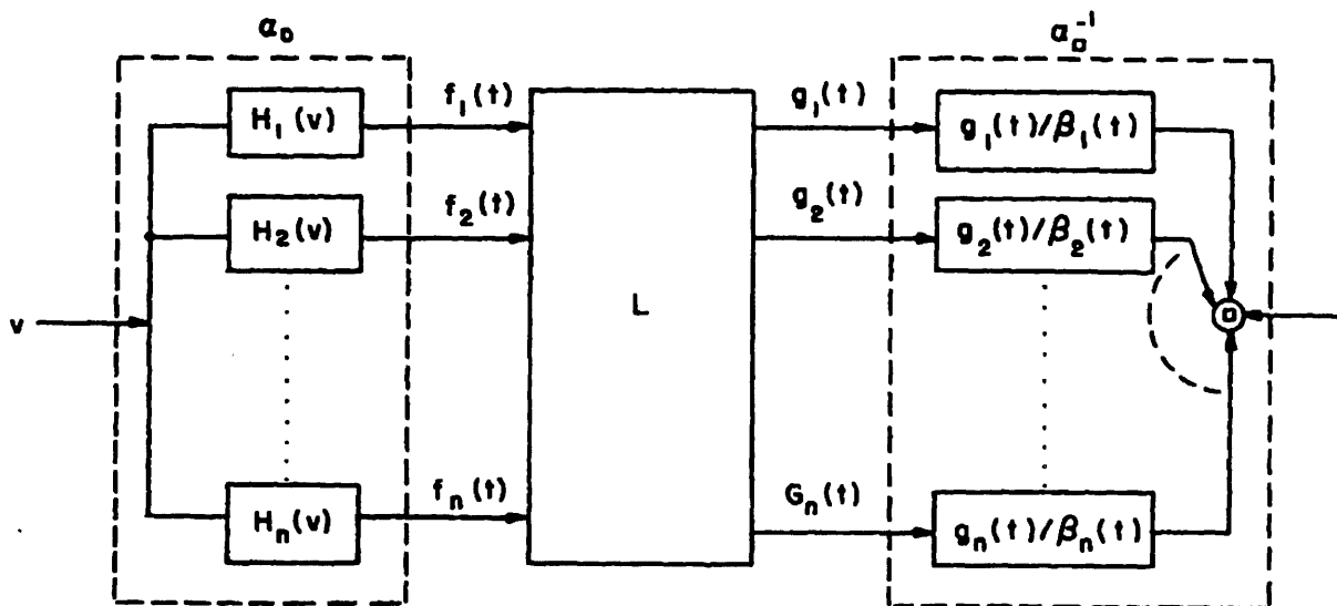
Fig. 9. Canonic representation of a homomorphic system with memoryless input and output operations, illustrating the construction of the characteristic systems.
