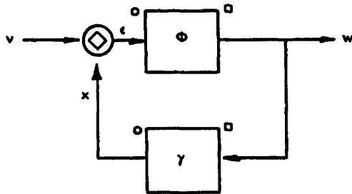
Fig. 13. Nonadditive feedback system with homomorphic systems in the forward and feedback paths.
