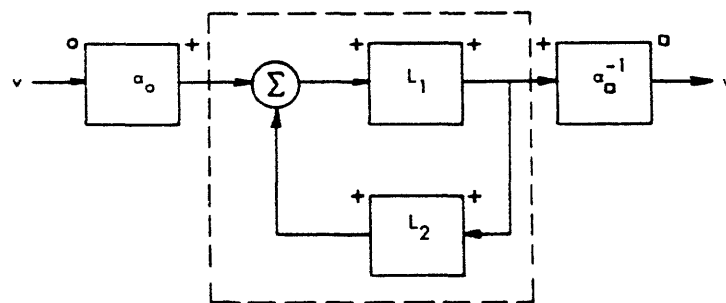
Fig. 12. Canonic representation of a homomorphic feedback system.
