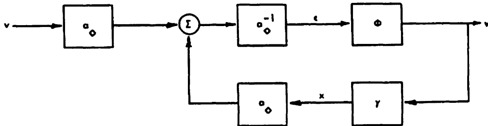
Fig. 14. Equivalent representation of the feedback system of Fig. 13.
