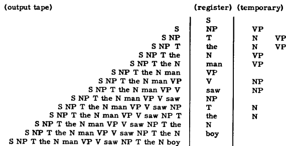
FIG. 2. Steps in producing a sentence.
