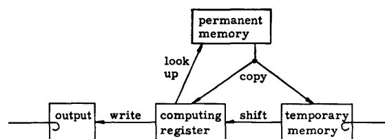
FIG. 1. How the mechanism is organized.
