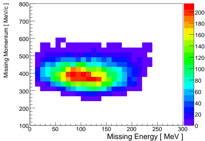
Figure 5-13: Distribution of missing momentum versus missing energy for kinematic II after all cuts applied.
