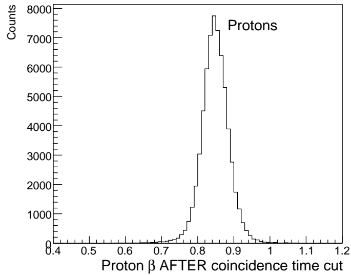
Figure 5-3: Comparison of the \beta value of particles detected in the proton spectrometer before (upper plot) and after (lower plot) the coincidence time cut is applied. Events corresponding to detected deuterons, protons and pions are shown in the upper plot. After applying the coincidence time cut, only the distribution corresponding to protons survives and so no further proton particle identification cut was necessary.
