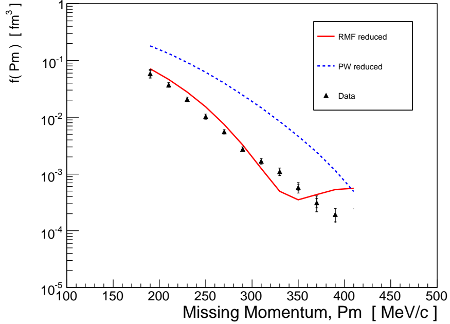
Figure 6-3: Extracted distorted momentum distribution from kinematic I data for ^{12}\text{C}(e, e'p)^{11}\text{B} reaction. The solid line (red online) is the reduced cross-section from the relativistic mean full calculation of the cross-section. The dotted line is the reduced cross-section for the plane wave calculation.
