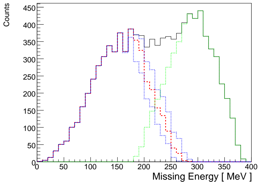
Figure 5-11: Upper Plot: Two-dimensional distribution of events in kinematic III of \omega versus y-scaling variable, with empirical cut selected; dotted lines give limits of the systematic check of this cut on the final cross-section result. Lower Plot: Full missing energy distribution for kinematic III; dashed line (red online) shows the distribution after the \omega -y cut is applied; dotted line (green online) shows the data rejected by this cut. The two dotted (blue) lines around the dashed (red) line show the effect of the upper and lower limits of the \omega - y cut and are used to evaluate the systematic error associated with this cut.
