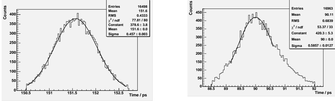
Figure 4-7: The coincidence time calibration for the left and right spectrometers; note the left arm measurement (left figure) has better resolution than the right arm measurement.
