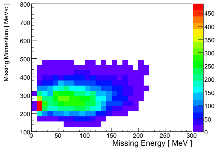
Figure 5-12: Distribution of missing momentum versus missing energy for kinematic I after all the described cuts have been applied. Note that this dataset shows clearly the bound state peak at low missing energy and momentum.
