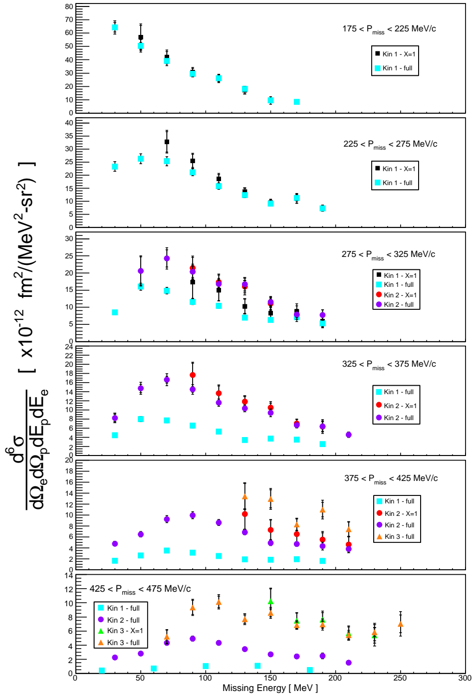
Figure 6-19: A comparison of the quasielastic cross-section extracted using x_B = 1 \pm 1\% and the continuum cross-sections extracted without using this constraint on Bjorken- X . For the same missing momentum bin, the full cross-section (not using the x_B cut) has a tail arising from the data at x_B = 1 .
