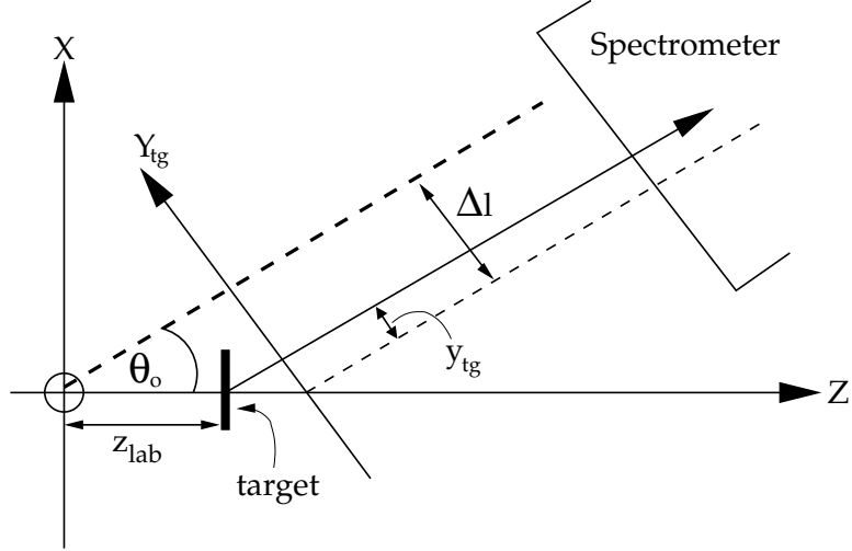
Figure 4-6: Definition of the mispointing variables, in the Hall coordinate system; the Y-axis in the hall frame is pointing out of the page.
