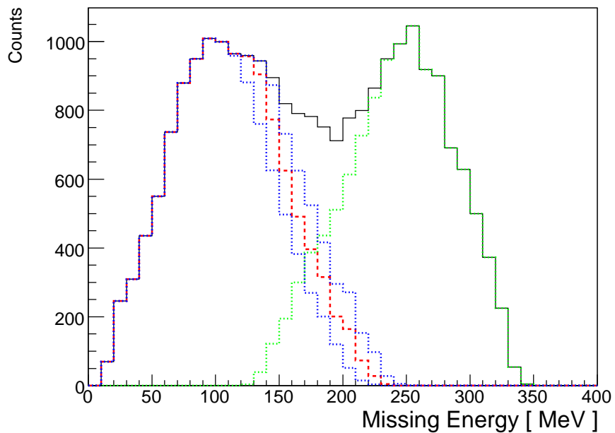
Figure 5-10: Upper Plot: Two-dimensional distribution of events in kinematic II of \omega versus y -scaling variable, with empirical cut selected; dotted lines give limits of the systematic check of this cut on the final cross-section result. Lower Plot: Full missing energy distribution for kinematic II; dashed line (red online) shows the distribution after the \omega - y cut is applied; dotted line (green online) shows the data rejected by this cut. The two dotted (blue) lines around the dashed (red) line show the effect of the upper and lower limits of the \omega - y cut and are used to evaluate the systematic error associated with this cut.
