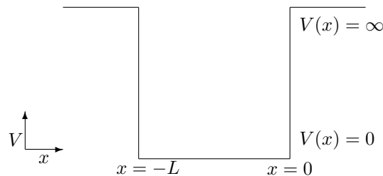
Figure 9-1: Infinite square well
