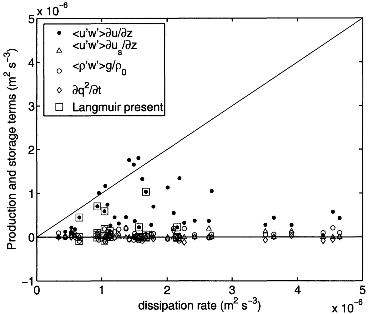
FIG. 10. Estimates or upper bounds (on shear production only) on production, growth, and dissipation terms in the turbulent kinetic energy budget. The dissipation term is usually larger than the sum of the other terms, suggesting that the terms not included here—the transport terms—are important in the TKE balance. Boxes show times when Langmuir turbulence was detected.
