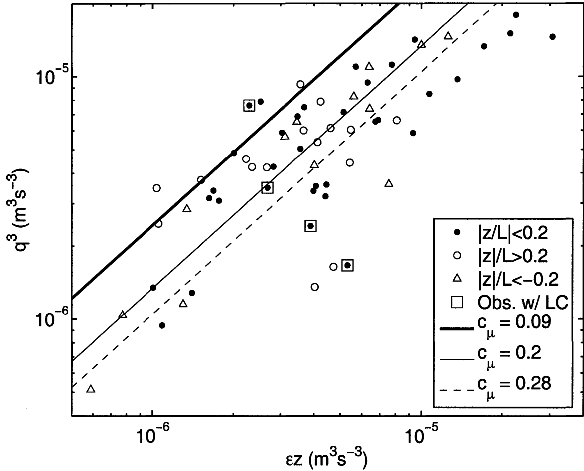
FIG. 11. Test of a standard rigid-boundary relationship between TKE, dissipation rate, and a turbulent length scale. For clarity we have shown lines with varying c_\mu^o , but they could have been drawn equally well by varying \kappa . The observed value of c_\mu^o is larger than the standard value of 0.09, meaning that the observed size of the energy-containing eddies is smaller than in standard rigid-boundary turbulence. c_\mu^o = 0.2 is the median of the observations and c_\mu^o = 0.28 is the least squares linear fit to the observations.
