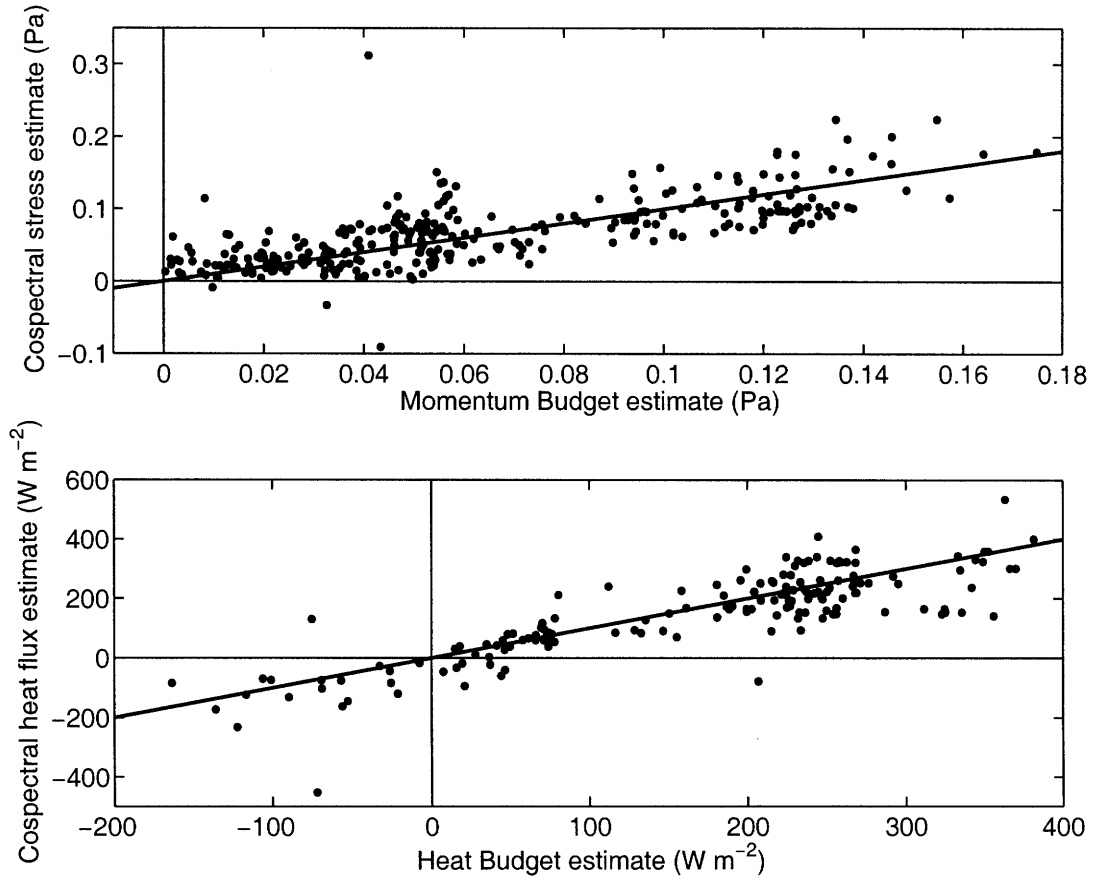
FIG. 8. Cospectral estimates of momentum flux (top) and heat flux (bottom) vs independent estimates from budgets. Dots are individual burst measurements. Data from both 1.7 and 2.2 m are shown here. A preliminary version of this figure appeared in Edson et al. (2007).
