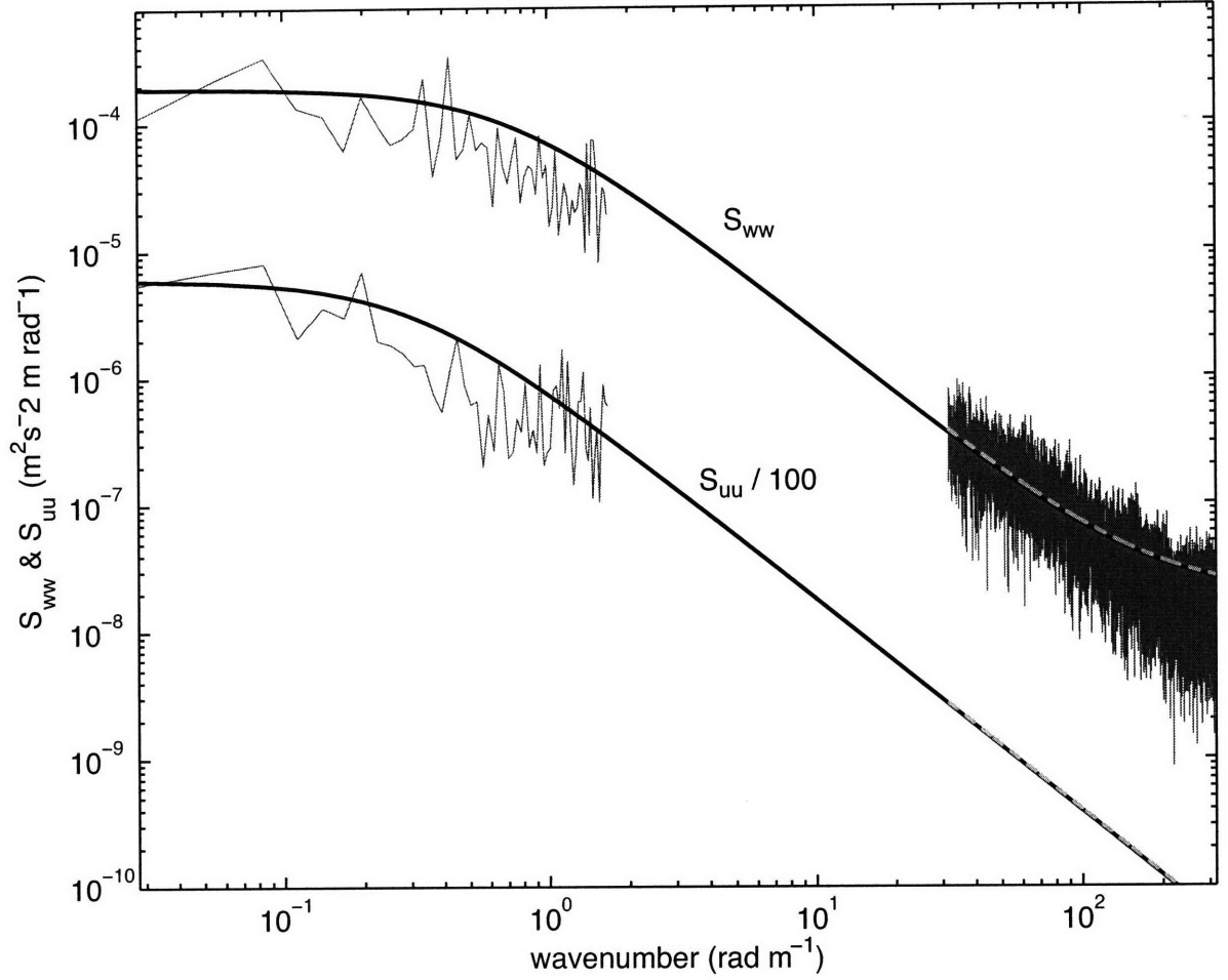
FIG. 4. Example autospectra of velocity fluctuations. Gray: observed. Black: best fit to full spectrum model. Dashed: best fit to inertial range model. Top spectrum is S_{ww} and bottom spectrum is S_{uu} , reduced for clarity by a factor of 100. As explained in the text, because of noise, the inertial ranges in S_{uu} and S_{vv} were determined from the inertial range w spectra and not from inertial range observations of u and v .
