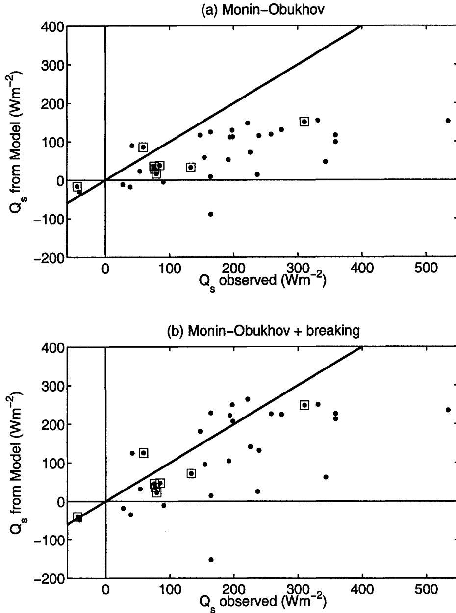
FIG. 13. Vertical heat flux, from cospectral observations (Gerbi et al. 2008) and models. The turbulent diffusivities used in modeling the temperature flux are explained in the text. The Monin-Obukhov model underpredicts the temperature fluxes. The composite model accounting for shear instability, buoyancy flux, and wave breaking gives much better agreement with the observations. Boxes show times when Langmuir turbulence was detected at the surface.
