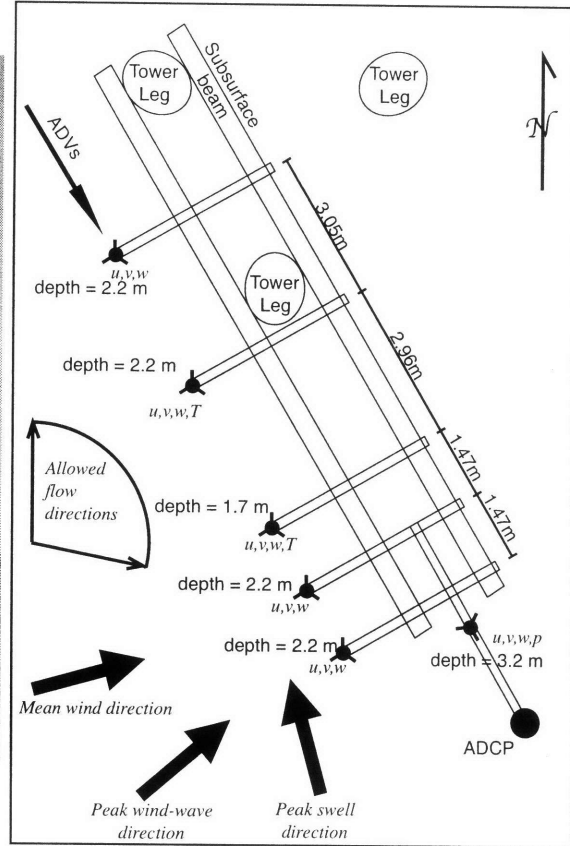
FIG. 2. Photograph, looking north, and schematic drawing of the Air Sea Interaction Tower at MVCO. The platform is 12 m above the sea surface. In the schematic diagram of the instrument tower, ellipses represent the tilted tower legs (which join above the sea surface). Small filled circles with three arms each represent ADVs and thermistors. The large filled circle represents the mid-depth ADCP. Mean wind and wave directions are shown by bold arrows, and the range of flow directions ( 0\text{-}120^\circ ) used in this study is shown to the left.
