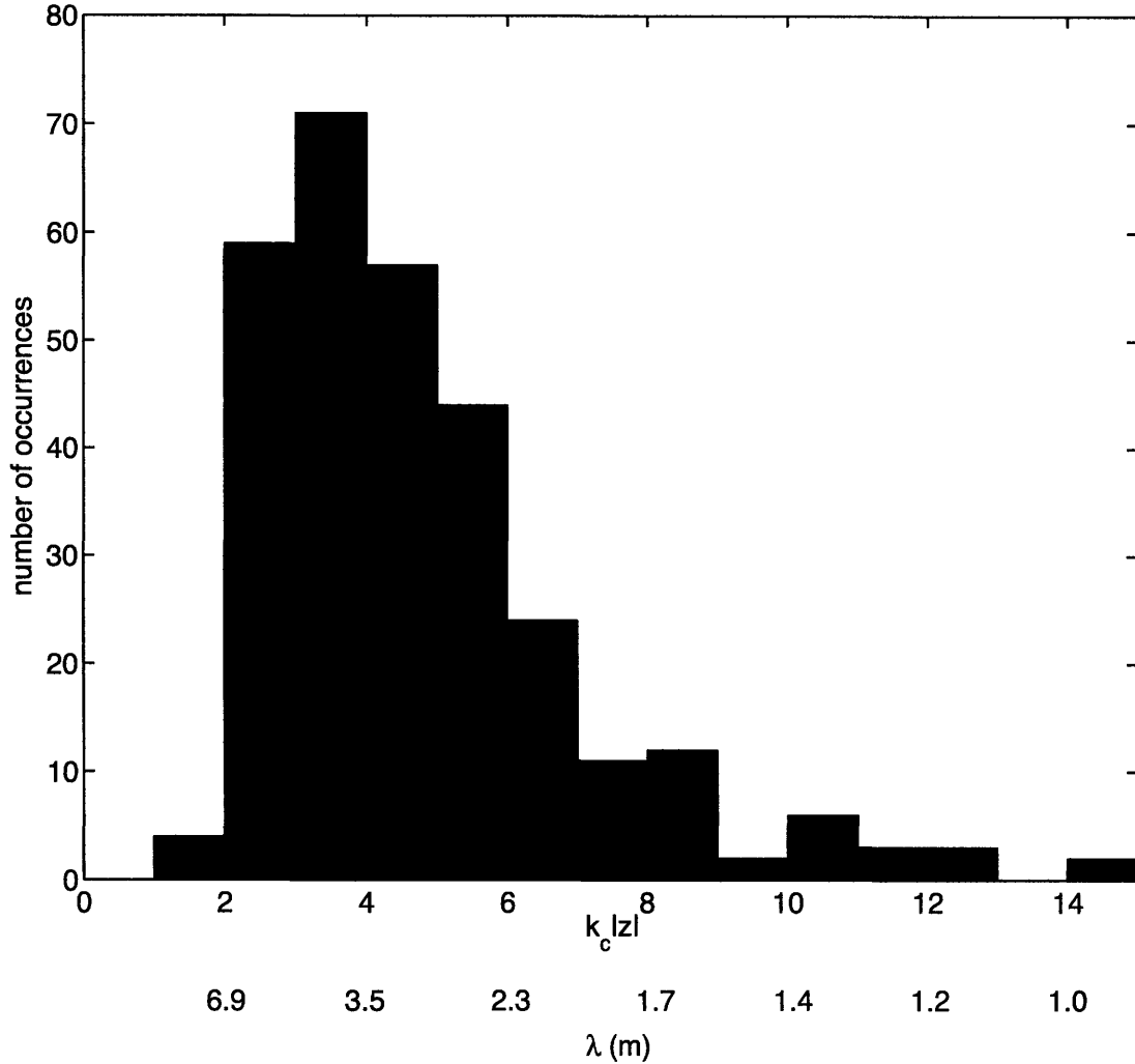
FIG. 4. Histogram of nondimensional cutoff wavenumber, k_c|z| , the scale of the smallest turbulent eddies measured by the below-waveband cospectral method, normalized by depth. A second x-axis scale gives the equivalent cutoff length scales, \lambda = 2\pi/k_c , at a nominal depth of 2.2 m.
