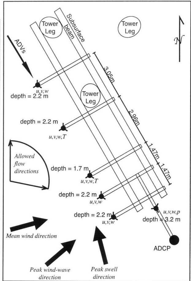
FIG. 3. Photograph, looking north, and schematic plan-view drawing of the Air Sea Interaction Tower at MVCO. In the photograph, the platform is 12 m above the sea surface. In the schematic diagram of the instrument tower, ellipses represent the tilted tower legs (which join at the platform). Small filled circles with three arms each represent ADVs and thermistors. The large filled circle represents the mid-depth ADCP. Mean wind and wave directions are shown by bold arrows, and the range of flow directions (0-120°) used in this study is shown to the left. This figure is reprinted from Gerbi et al. (2008).
