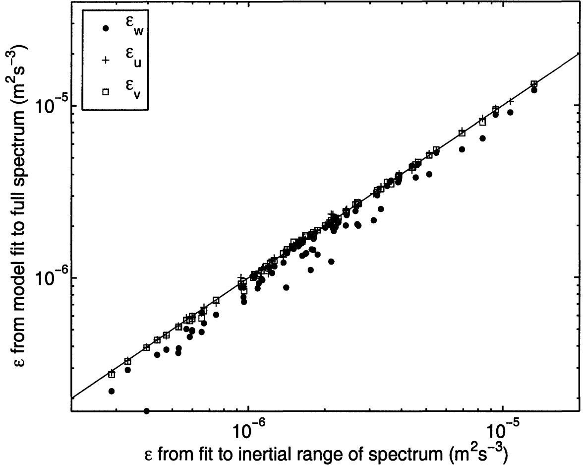
FIG. 5. Comparison of estimates of dissipation rate as a test of internal consistency of two-parameter fits of the model spectrum to observed spectra. Vertical axis: estimates derived from fitting model to the full spectrum (3.13); horizontal axis: estimates derived using only the inertial range of the spectrum (3.5). Line is 1:1.
