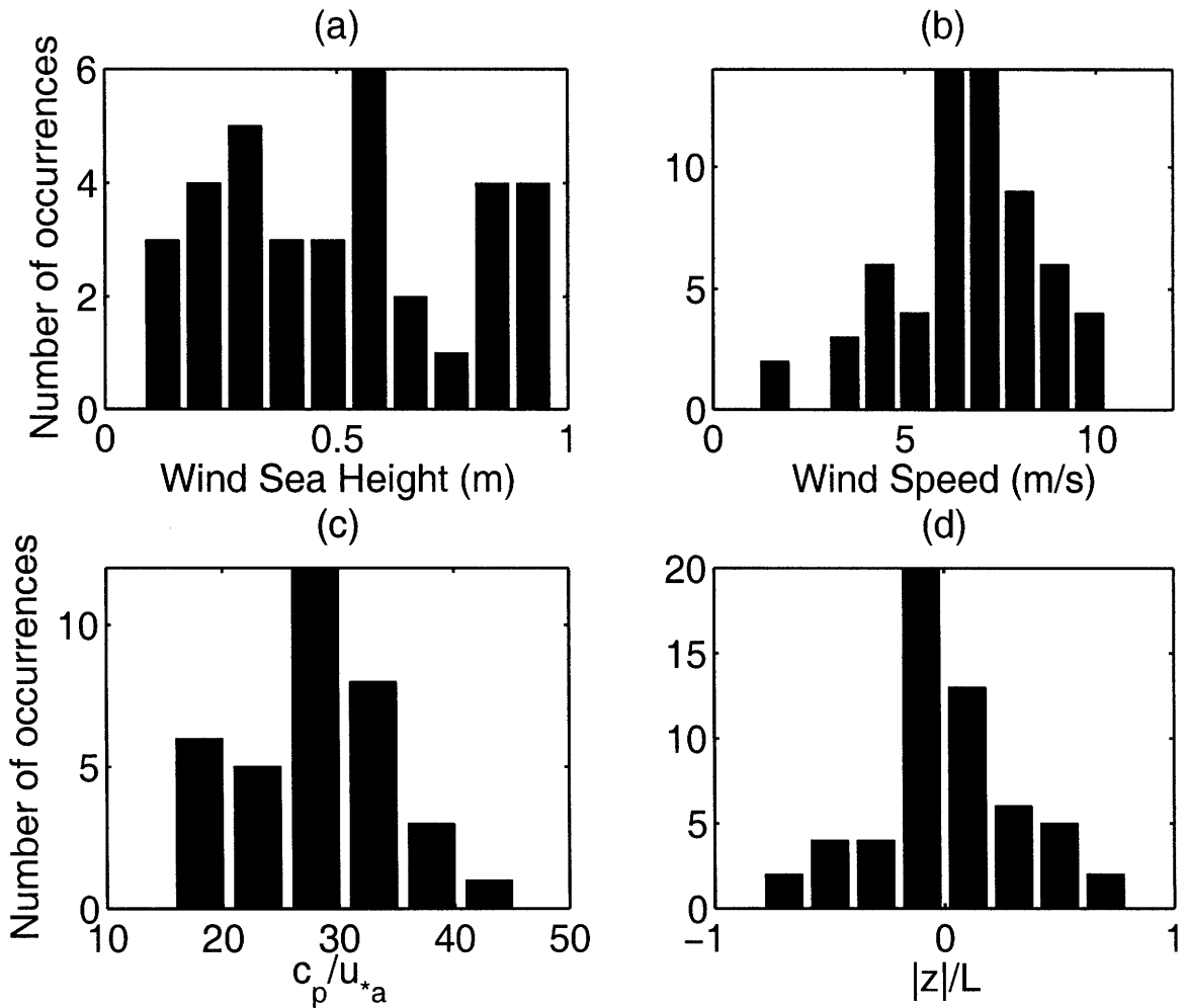
FIG. 8. Environmental conditions during times of dissipation and TKE observations. (a) Significant height of the wind waves. (b) Wind speed at 10 m height. (c) Age of wind waves. (d) Monin-Obukhov parameter at lower (2.2 m) ADV computed from surface fluxes. Four points with values between -6 and 10 have been omitted from the histogram of |z|/L .
