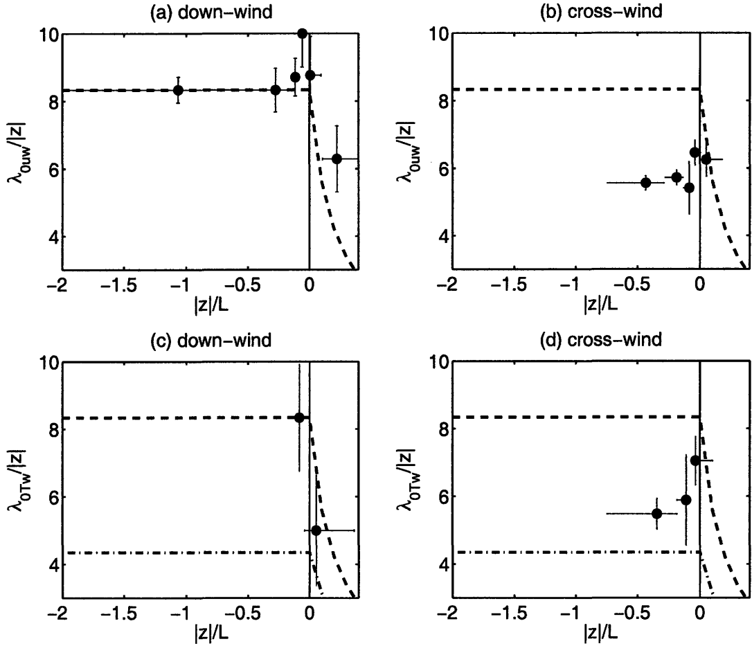
FIG. 9. \lambda_0/|z| vs |z|/L . Dots are bin medians of observations, formed from a constant number of observations per bin, the dashed lines are the momentum results of Wyngaard and Coté (1972) (this study's (2.15)), and the dash-dot lines in the lower panels are the temperature results of Wyngaard and Coté (1972) (this study's (2.16)). Vertical error bars show two standard errors of the distribution of observations within each bin, and horizontal bars show the range of |z|/L in each bin. Left panels, (a) and (c), show \lambda_0/|z| when the wind was aligned with the drift, and right panels, (b) and (d), show \lambda_0/|z| when the wind was across the drift. Upper panels, (a) and (b), show \lambda_{0uw}/|z| , and lower panels, (c) and (d), show \lambda_{0Tw}/|z| . At a nominal depth of 2.2 m, the dominant length scales shown in this figure range between \sim 10 and 20 m. This size range is consistent with the horizontal scales attributed to Langmuir circulations based on observations of surface convergence velocities at the site.
