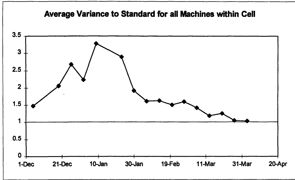
Figure 4.2 Average Variance to Standard for all Cell Machines for First Quarter of Operation
