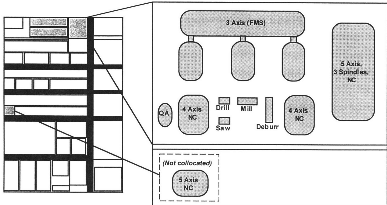
Figure 4.1 Cell Layout
