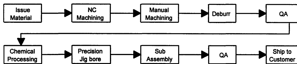
Figure 1.2 Typical Part Process Flow
