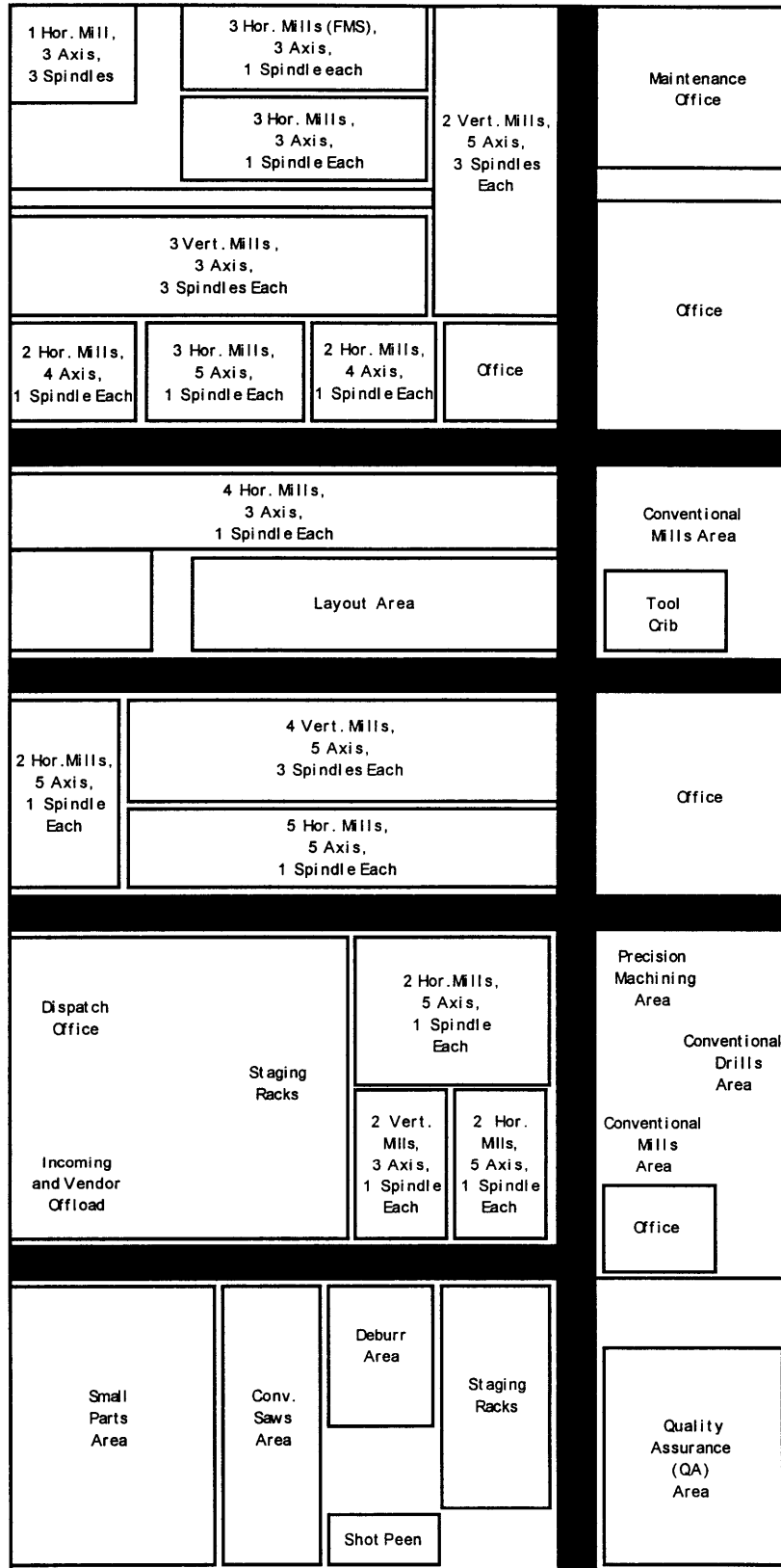
Figure 1.1 Machining Center Layout
