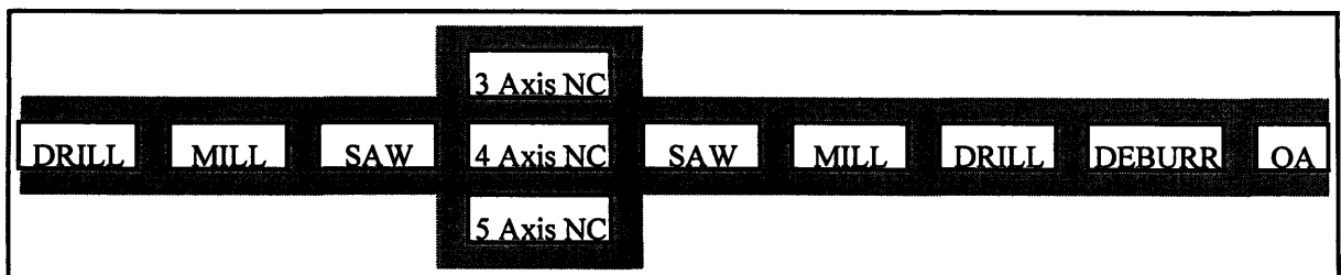
Figure 3.3 Cell Process
