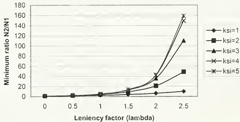
Figure 2: Minimum ratio of "redeeming" to "deceiving" transactions needed in order to restore one's good reputation following a period of quality over-reporting.
