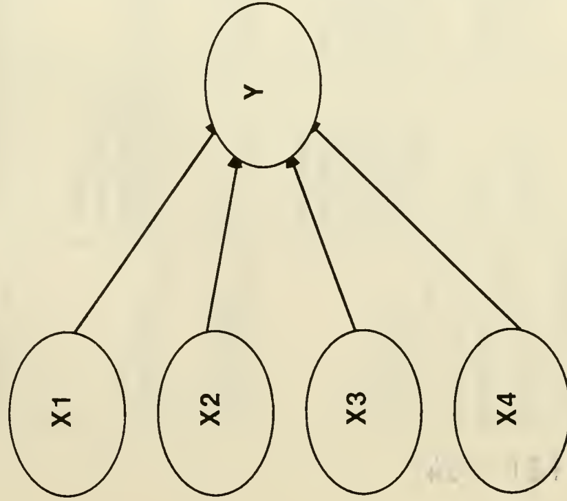
Figure 5(a): Main Effects Model
