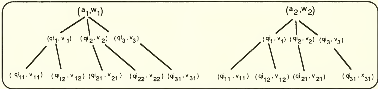
Figure 12: QIV-Equal Example
