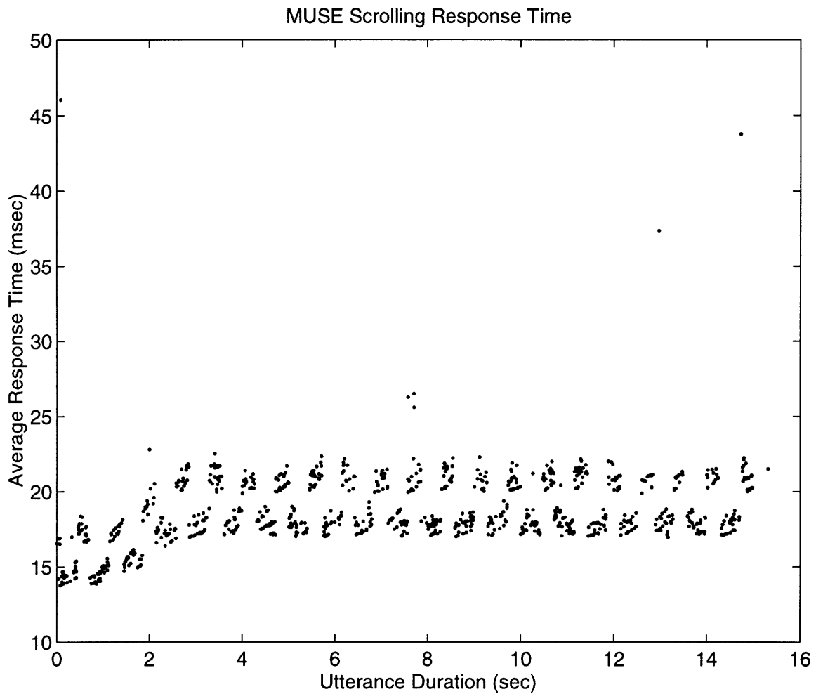
Figure 5-12: Average response time for 1000 scrolling trials for MUSE.
