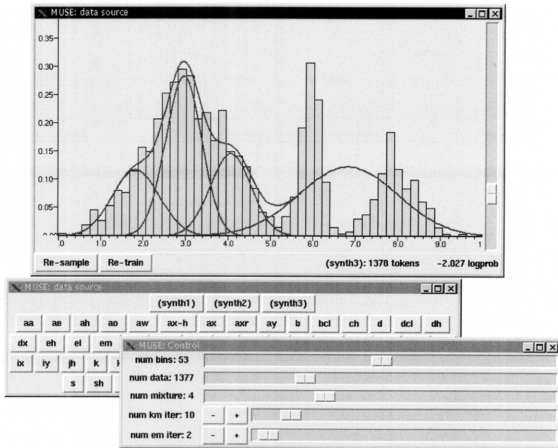
Figure 5-3: An interactive one-dimensional Gaussian mixture training tool.
