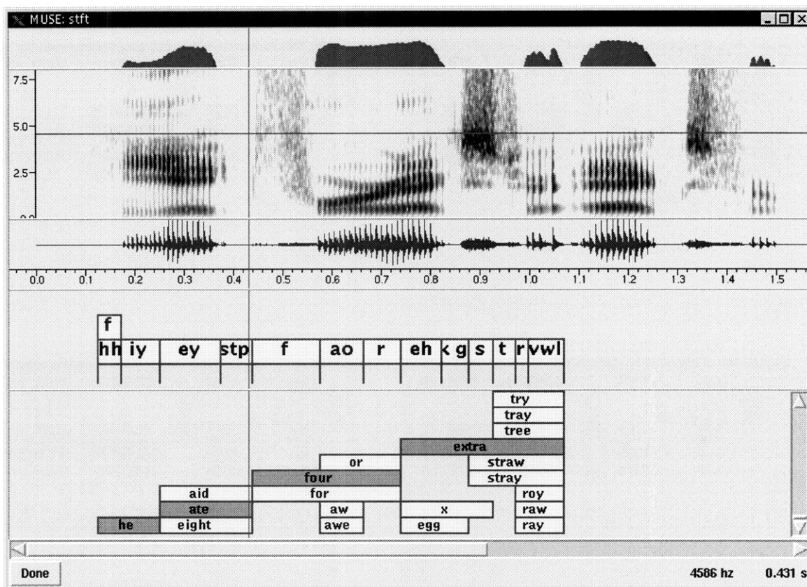
Figure 5-6: An interactive lexical-access tool.
