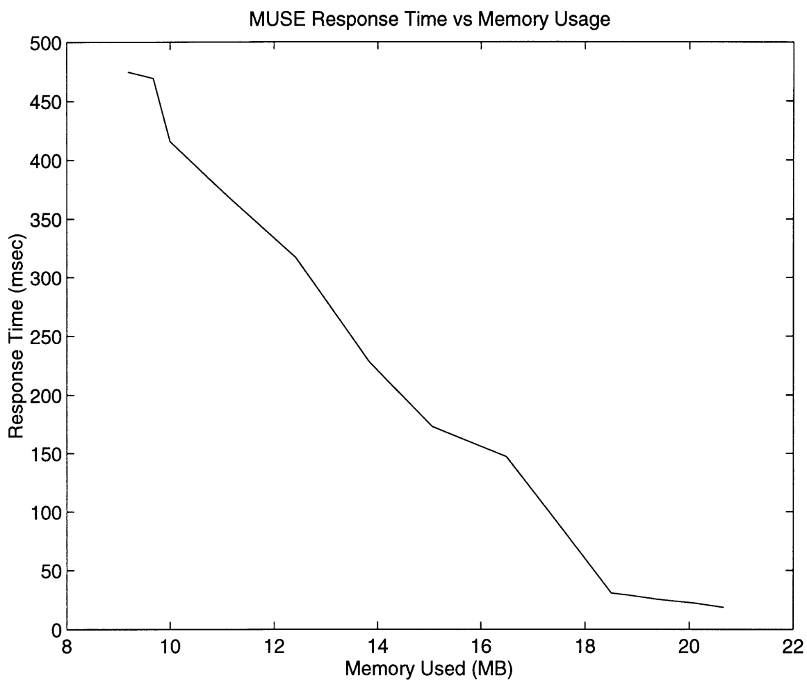
Figure 5-22: The tradeoff of average response time for scrolling versus memory usage, for the MUSE speech analysis tool.
