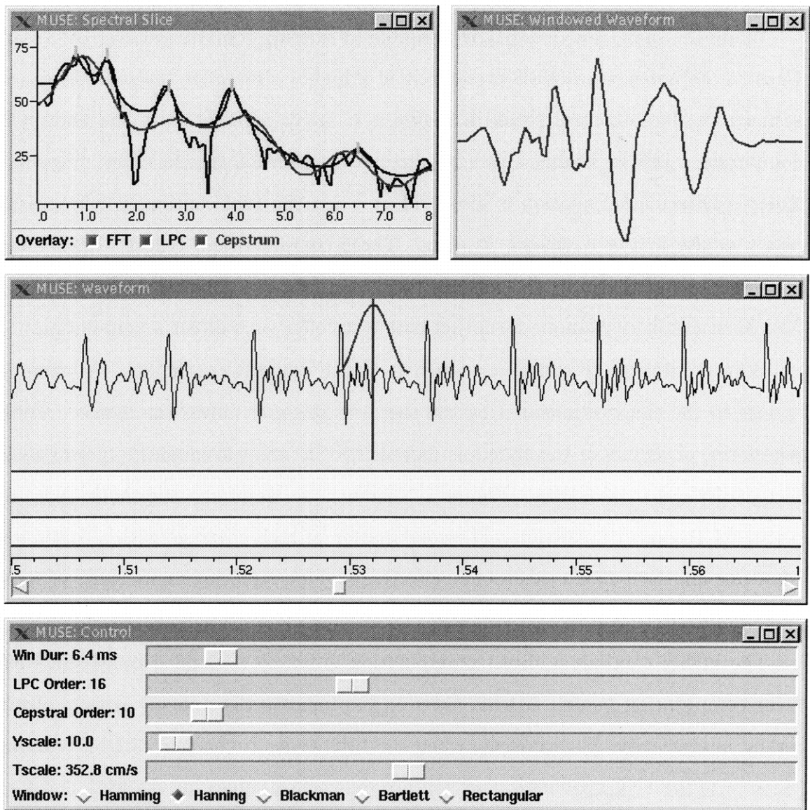
Figure 1-1: An interactive FFT, LPC and Cepstrum spectral slice tool.
