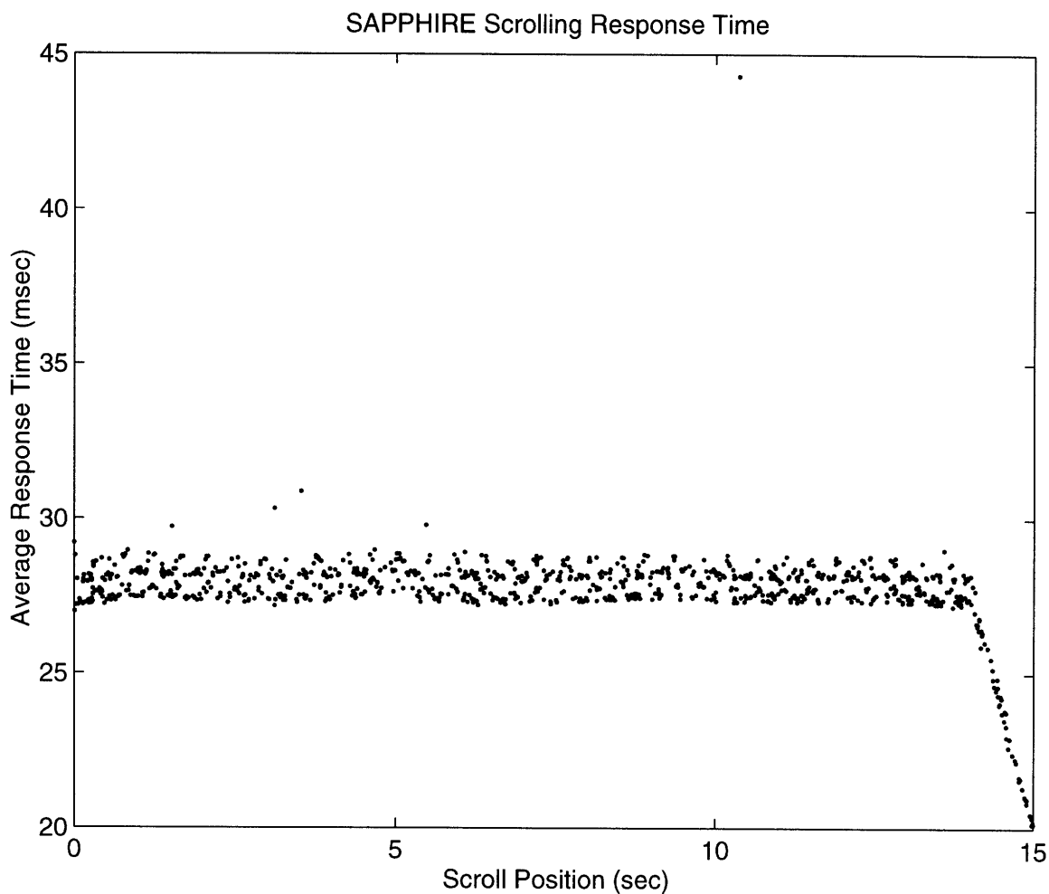
Figure 5-13: Average response time for 1000 scrolling trials for Sapphire.
