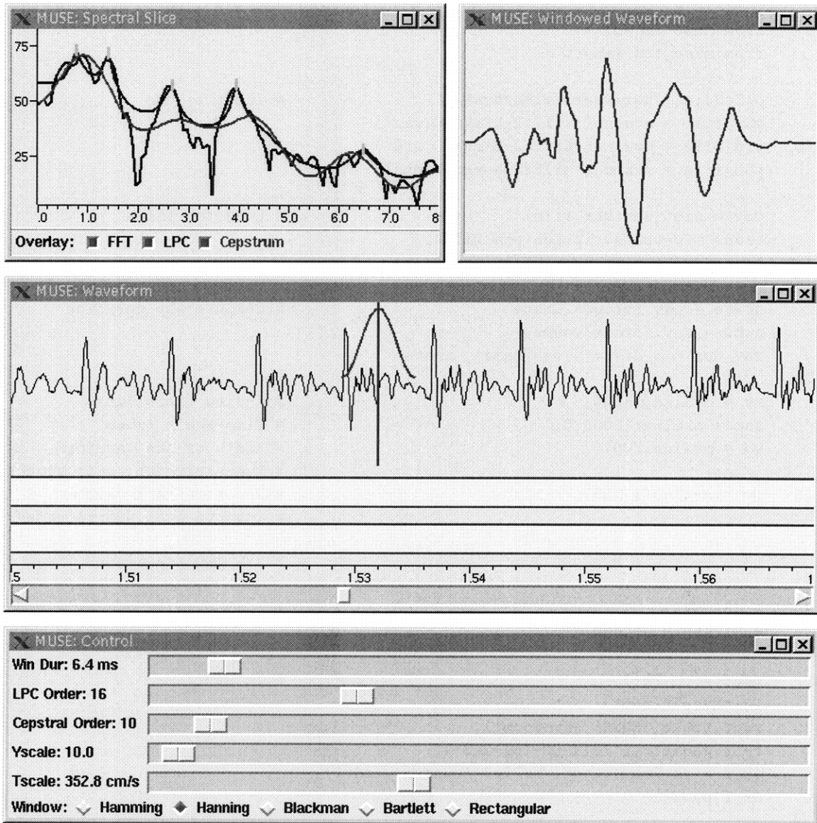
Figure 6-1: An interactive FFT, LPC and Cepstrum spectral slice tool.
