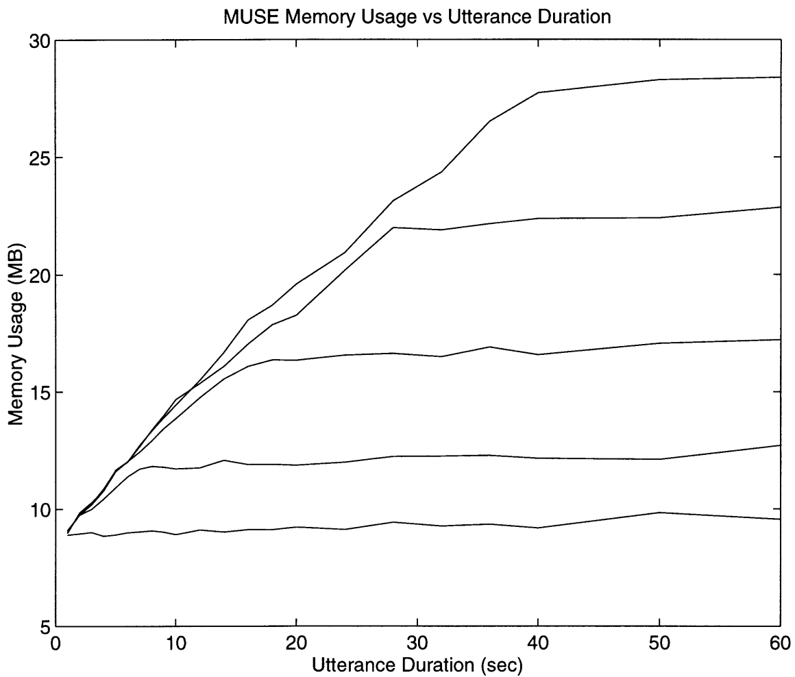
Figure 5-18: MUSE memory consumption for the speech analysis tool as a function of utterance length.
