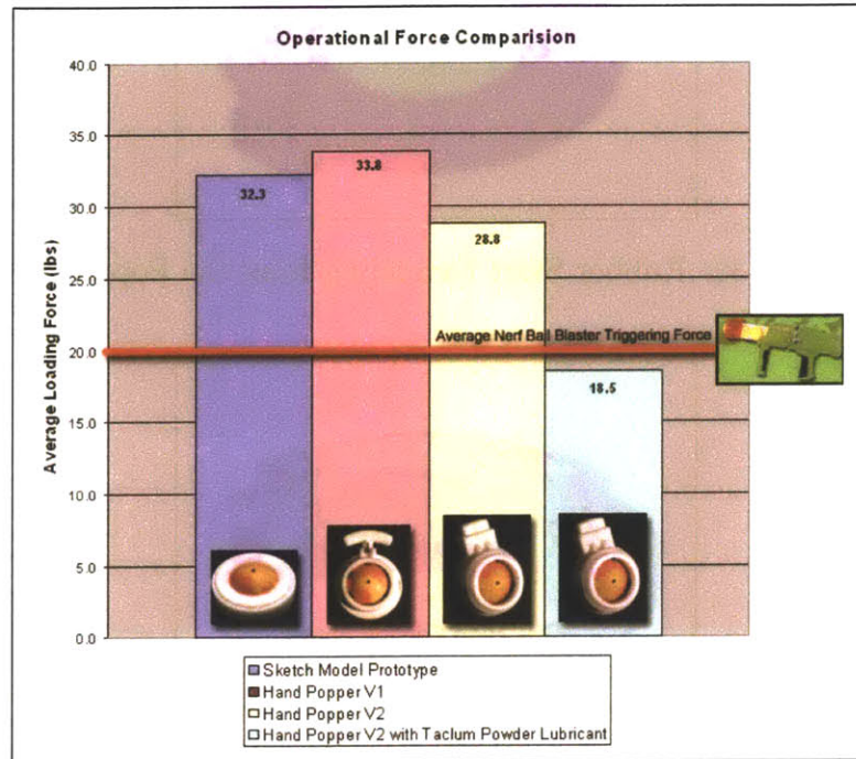
Figure 4-34: Operational Force Comparison
