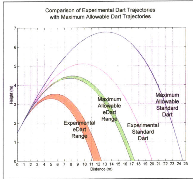
Figure 5-28: Maximum Allowable Trajectories of Standard Dart and 2nd Iteration eDarts
