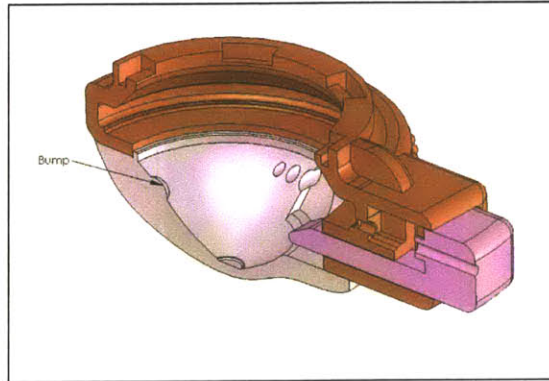
Figure 4-12: Bump Located in the Backing Plate
