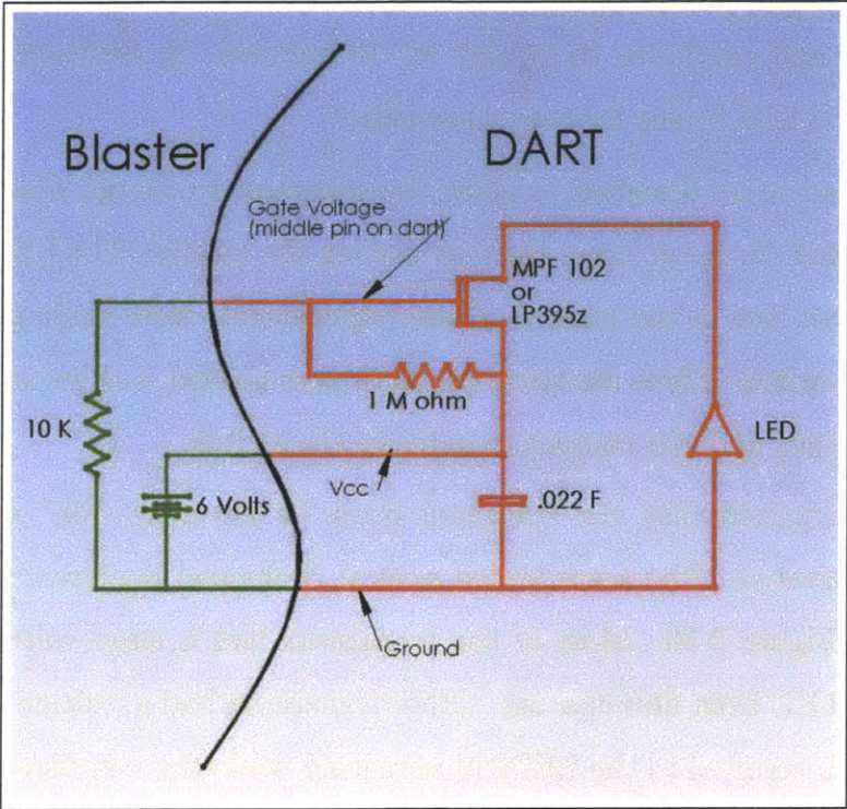
Figure 3-31: The Optimized Circuit for the LED Dart Sketch Model
