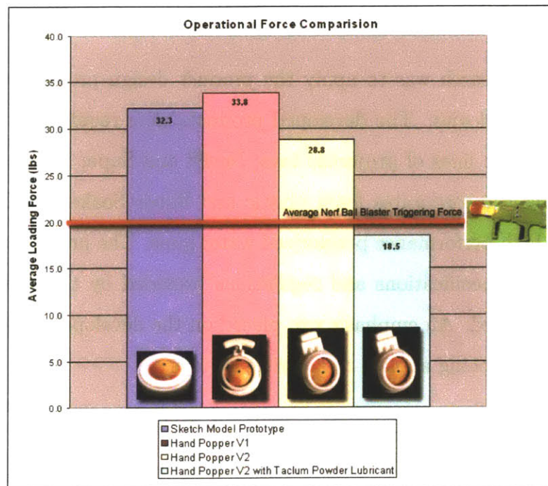
Figure 1-2: Operational Force Comparison
