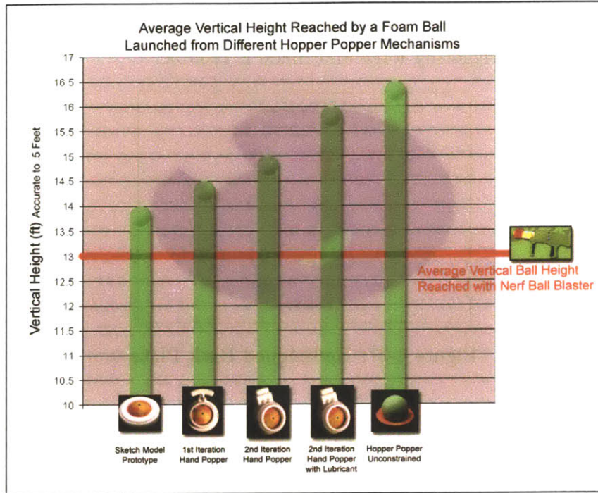
Figure 4-35: Vertical Distances Achieved by Foam Ball Launched with Various Mechanisms
