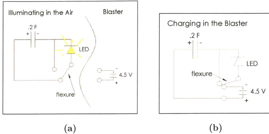
Figure 5-32: Final Circuit
