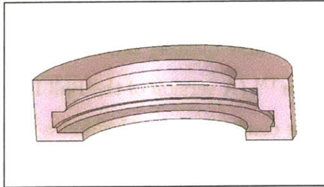
Figure 3-16: Cross Section of the Popper Holder
