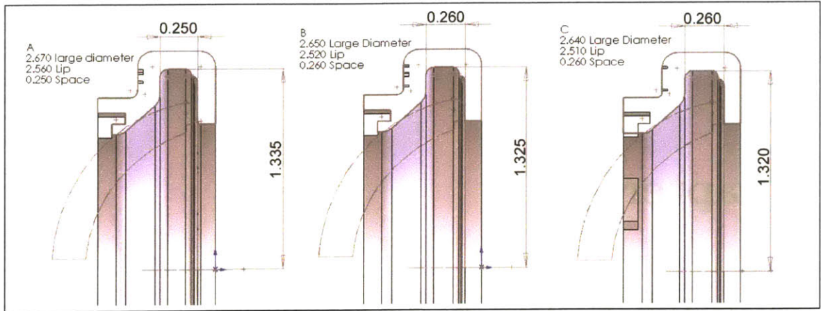
Figure 4-1: Alternative Inner Geometries of the Popper Holder
