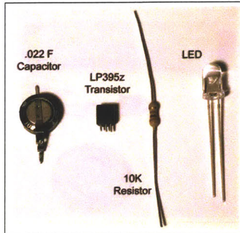
Figure 3-32: The Electronic Components of the LED Dart Sketch Model
