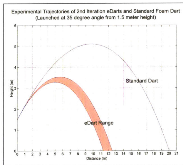
Figure 5-27: Trajectories of Standard Dart and 2nd Iteration Darts
