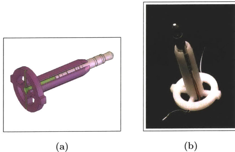
Figure 5-21: Redesigned Blaster Post
