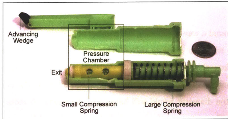
Figure 5-37: PowerClip™ Pressure Release Mechanism
