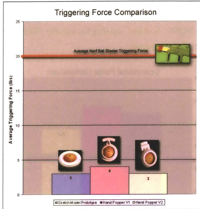
Figure 4-18: Average Triggering Force Comparison
