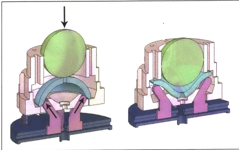
Figure 4-27: Loading Motion of a Cross-Sectioned Unconstrained Holder
