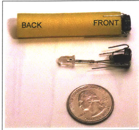
Figure 3-33: The Assembled LED Dart Sketch Model
