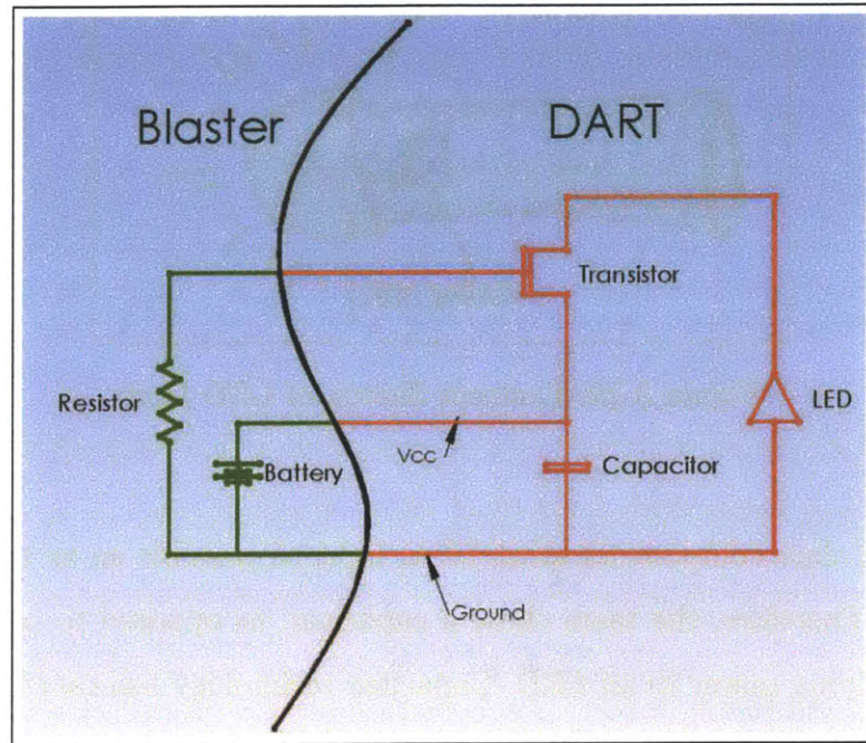
Figure 3-30: The General Circuit for the LED Dart
