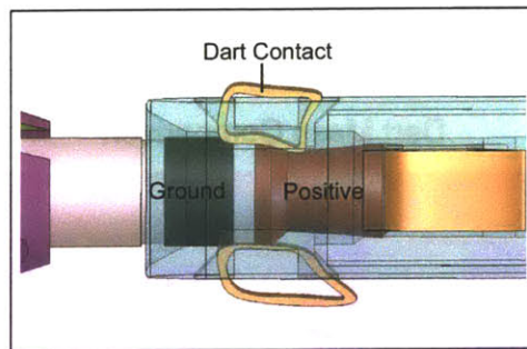
Figure 5-23: Dart Contact Bridging Blaster Contacts
