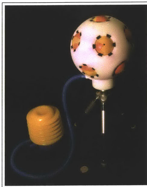
Figure 4-5: The Assembled Stomp Grenade
