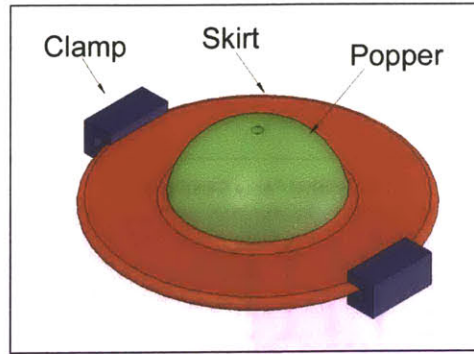
Figure 4-32: Rubber Skirt Extending from the Popper Rim
