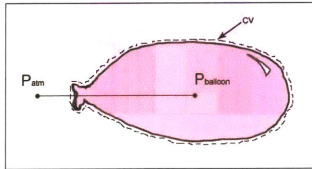
Figure 3-7: Streamline of Air Exiting Balloon
