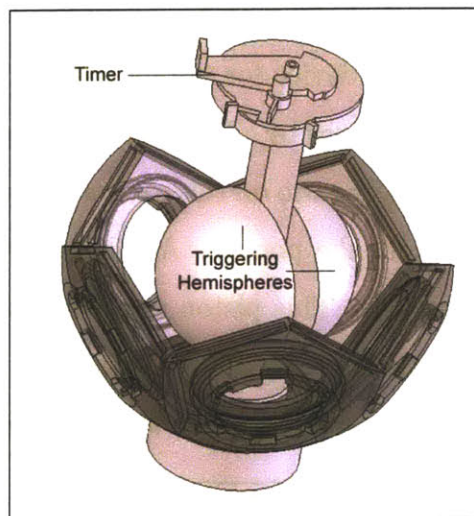
Figure 4-6: Model of a Grenade with Timer Mechanism
