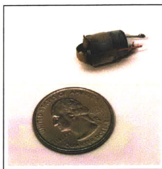
Figure 5-13: Shim Stock Switch for Impact Dart
