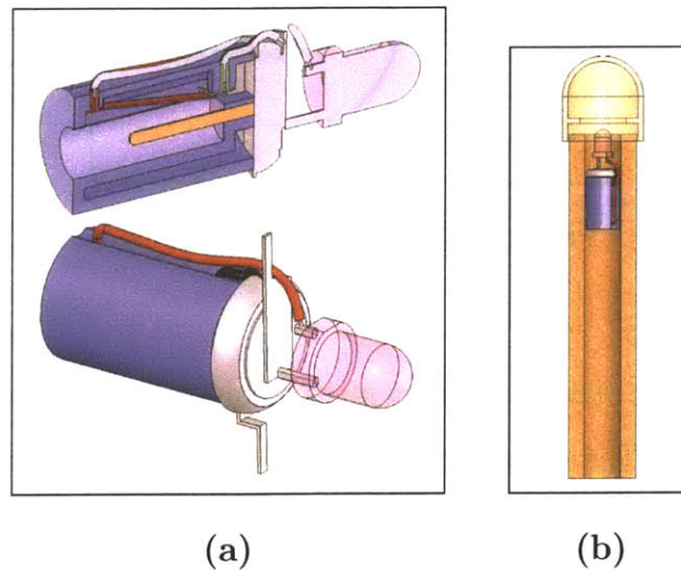
Figure 5-33: The Final eDart
