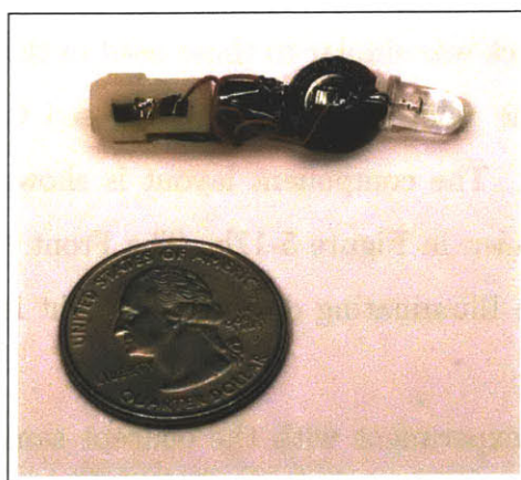
Figure 5-18: Contact Component for Alternating Color Blinking Dart
