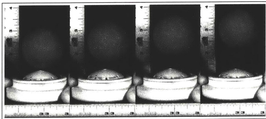
Figure 4-22: High Speed Photography of a Constrained Popper Launching a Foam Ball
