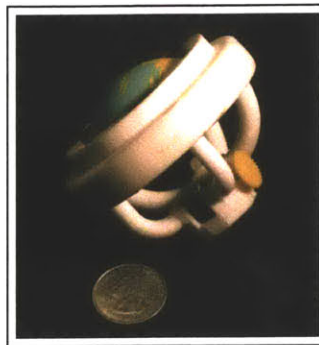
Figure 4-7: Customized Drive Assembly in SLS Housing for the RC Grenade
