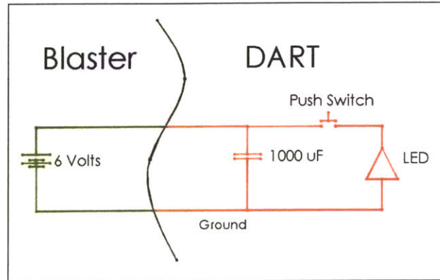
Figure 5-14: Impact Dart Circuit
