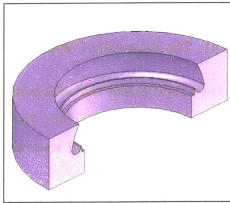
Figure 4-30: CAD Cross-Section of the Casted Silicone Ring
