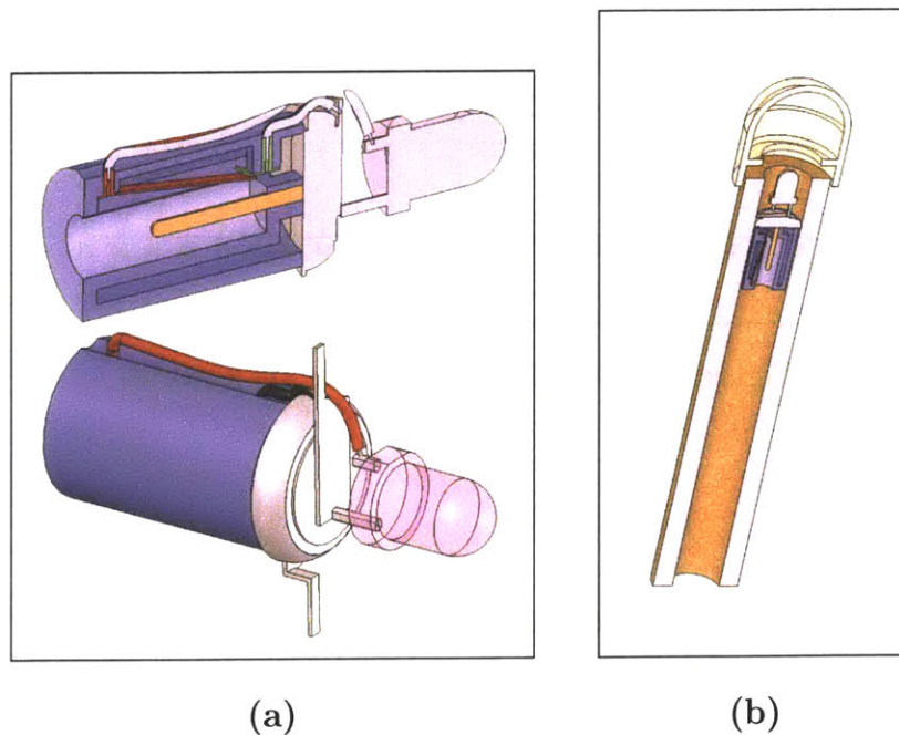
Figure 1-3: The Final eDart
