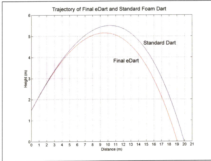
Figure 5-36: Standard and eDart Trajectories
