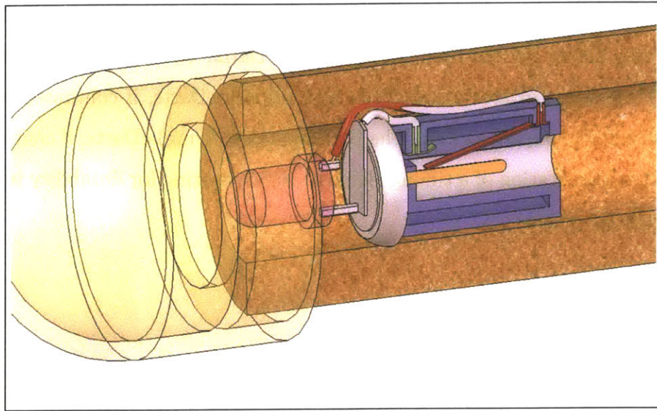
Figure 6-2: Final eDart Cross Section
