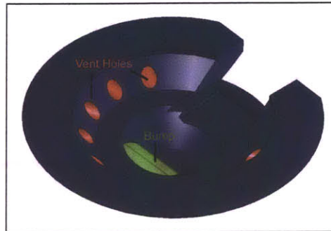
Figure 4-37: Redesigned Back Plate
