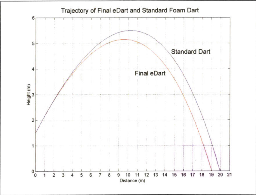
Figure 1-4: Standard and eDart Trajectories
