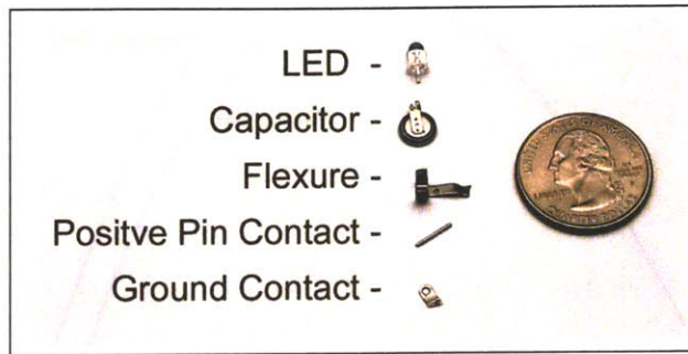
Figure 5-34: Final eDart Components
