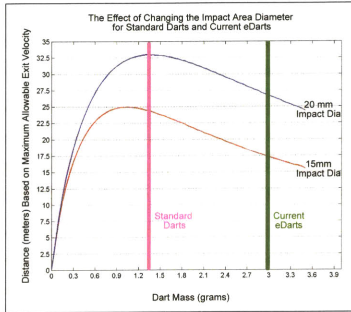
Figure 5-30: Effect of Changing the Impact Area for Standard Dart and 2nd Iteration Darts
