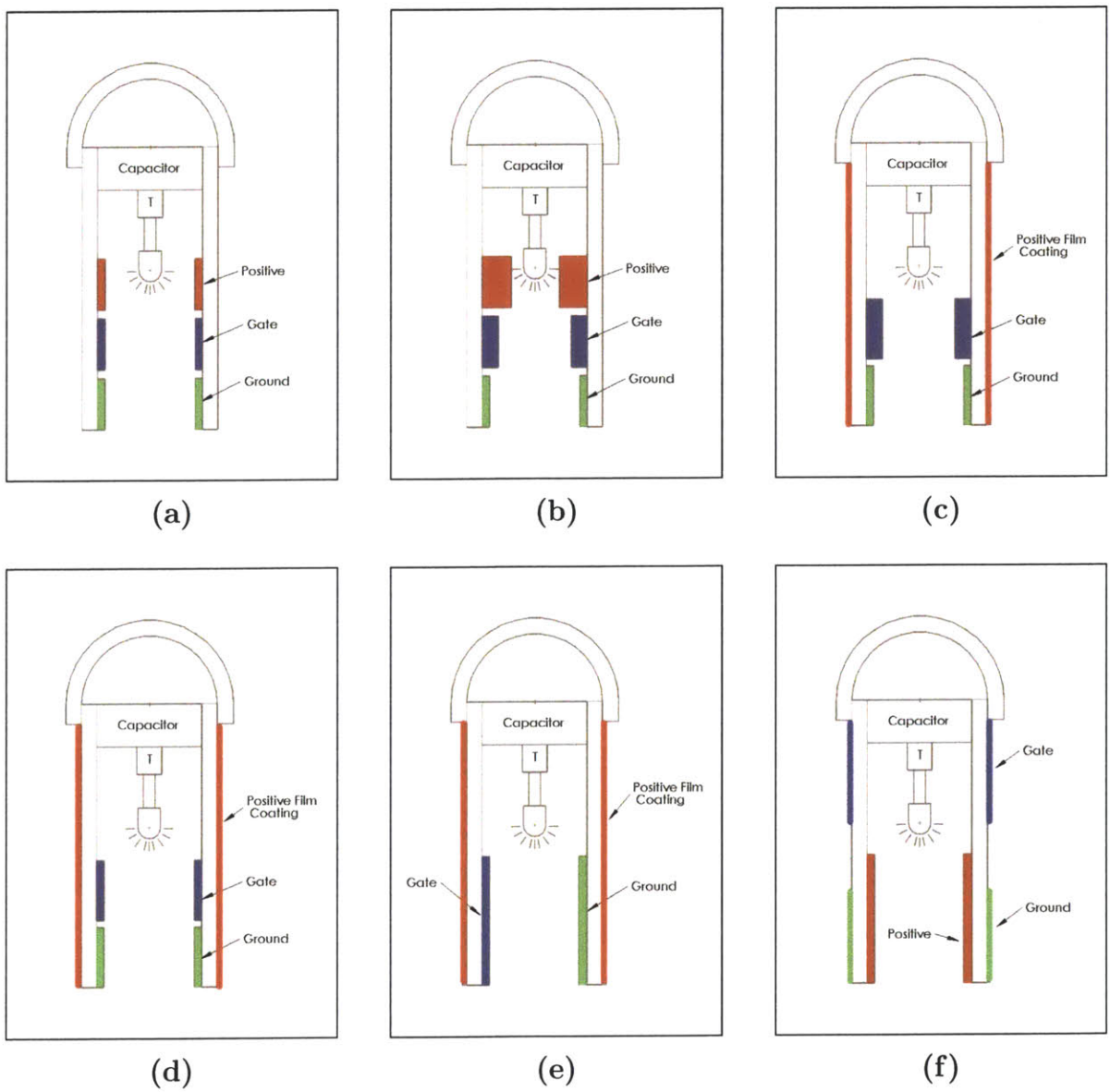
Figure 5-1: Various Dart Contact Layouts
