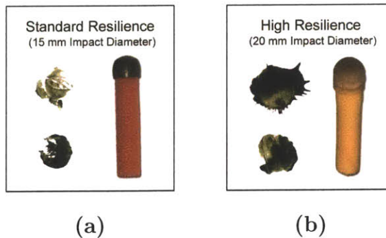
Figure 5-29: Standard and High Resilience Dart Impact Markings
