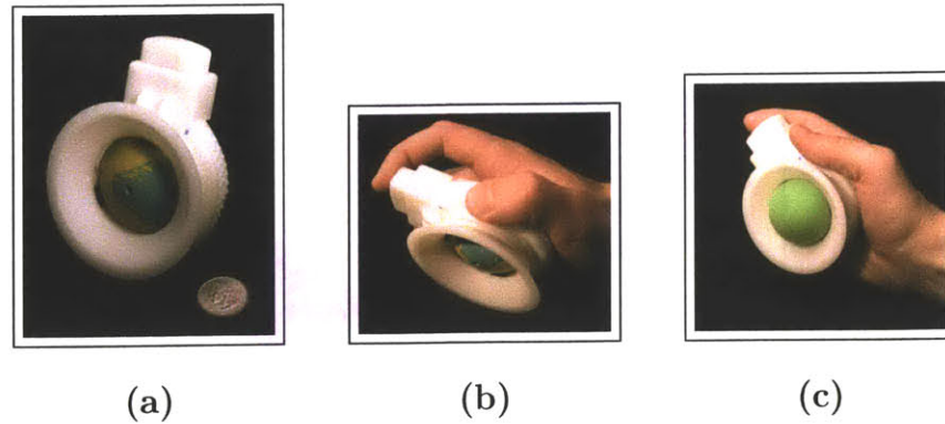
Figure 4-14: 2nd Iteration of the Hand Popper with Flared Channel
