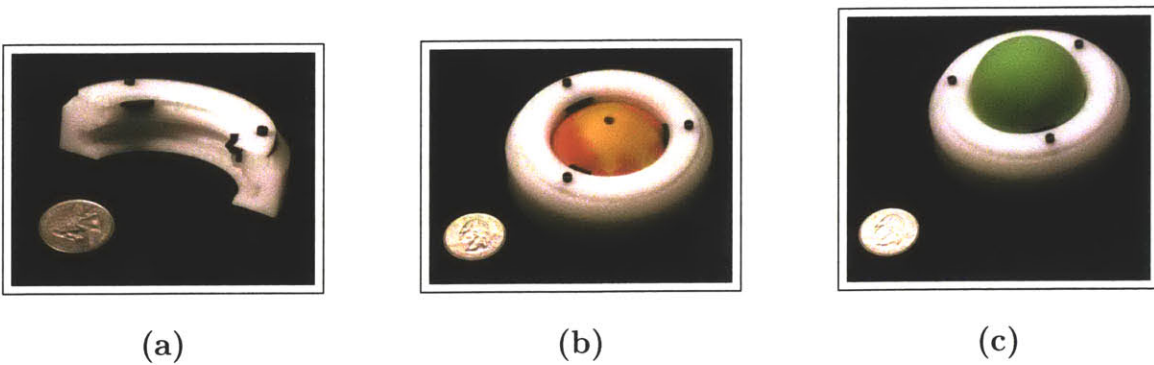
Figure 3-27: Refined Popper Holder
