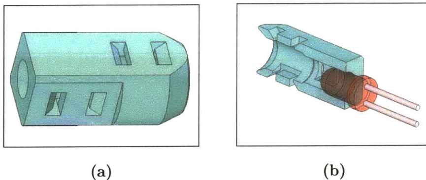
Figure 5-11: Contact Component for Back Illuminating Dart
