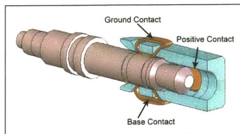
Figure 5-8: Revised Contact Orientation
