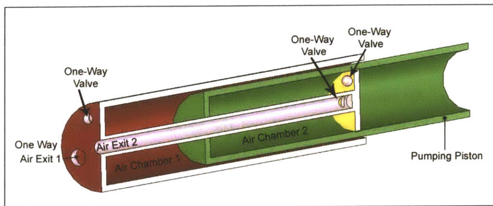
Figure 5-38: Piston Pump with Four One-Way Valves
