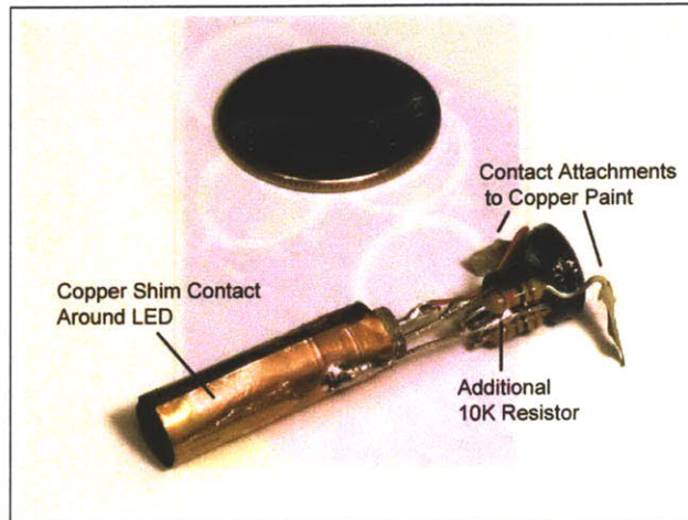
Figure 5-3: Revised Dart Component Layout
