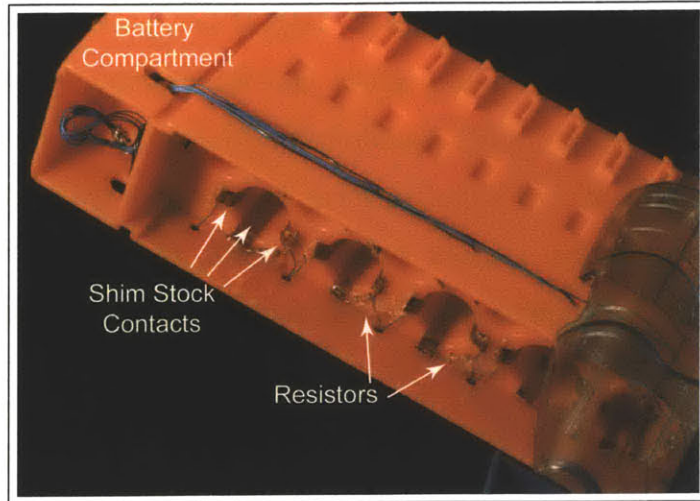
Figure 3-35: The Modified Clip with Shim Stock Contacts
