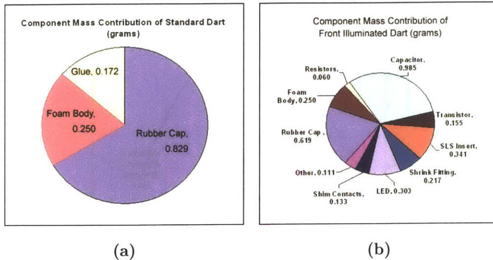
Figure 5-26: Dart Component Mass Contribution
