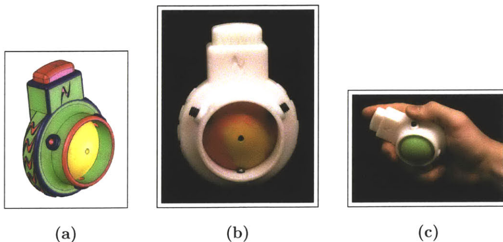
Figure 4-38: Final Iteration of the Hand Popper
