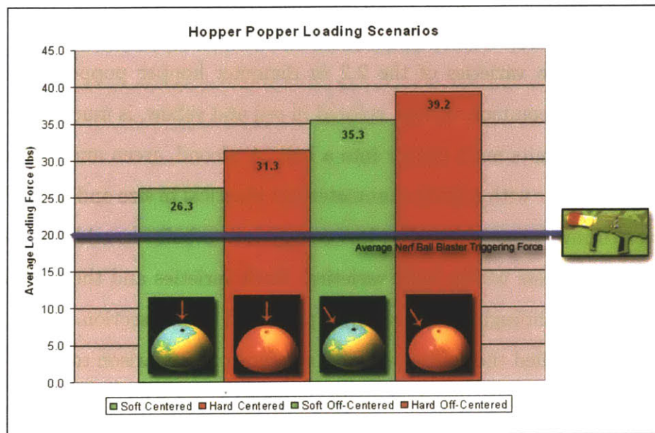
Figure 4-16: Average Loading Forces for Various Popper Scenarios
