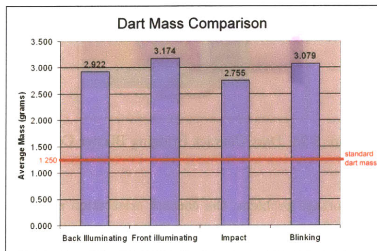
Figure 5-25: 2nd Iteration Dart Mass Comparison
