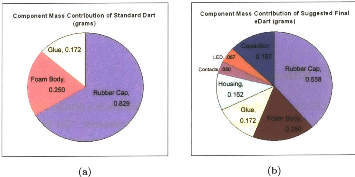
Figure 5-39: Comparison of Dart Component Mass Contribution
