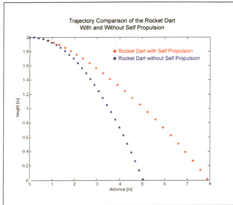
Figure 3-9: Trajectory of Rocket Dart with and without Self-Propulsion
