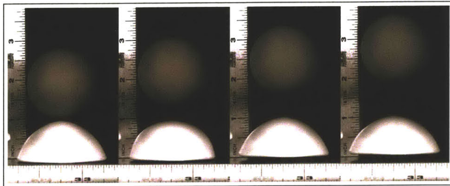
Figure 4-21: High Speed Photography of an Unconstrained Popper Launching a Foam Ball
