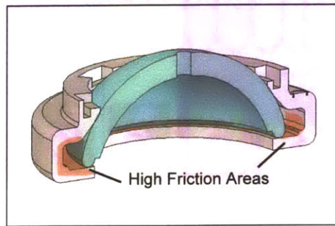
Figure 4-33: High Friction Areas inside the Popper Holder
