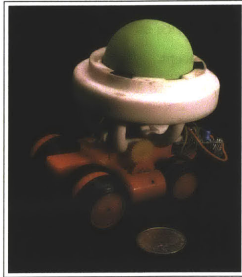
Figure 4-8: The Assembled RC Grenade
