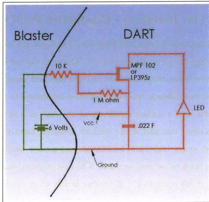
Figure 5-2: Redesigned Circuit with Two Blaster-Side Contacts
