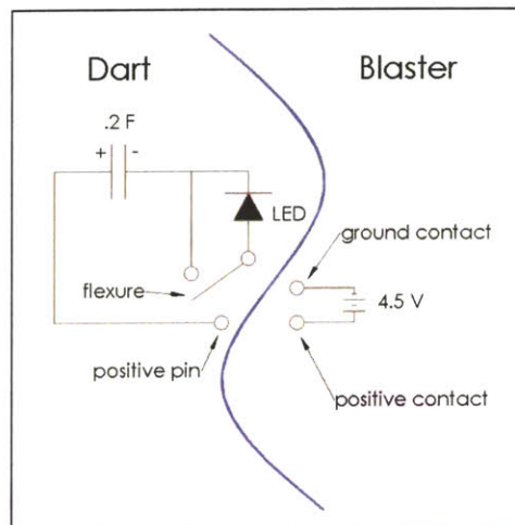
Figure 5-31: Final Circuit Design
