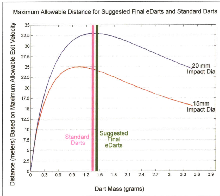
Figure 5-40: Maximum Allowable Distances of Final eDart and Standard Dart
